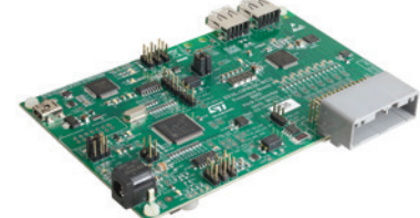
L9963E evaluation board (EVAL-L9963E-MCU) with on-board SPC5 MCU and preloaded firmware
