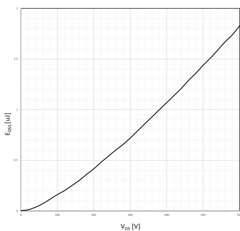
Figure 9. Typ. E_{OSS} vs. V_{DS}
