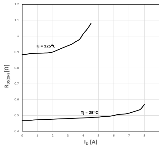
Figure 5. Typ. R_{DS(on)HS}
