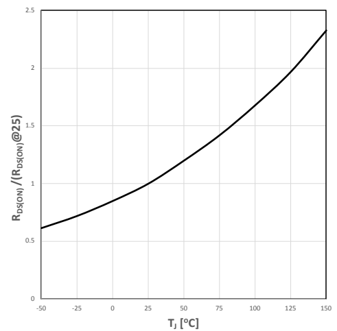
Figure 6. Typ. R_{DS(on)HS} vs. T_J
