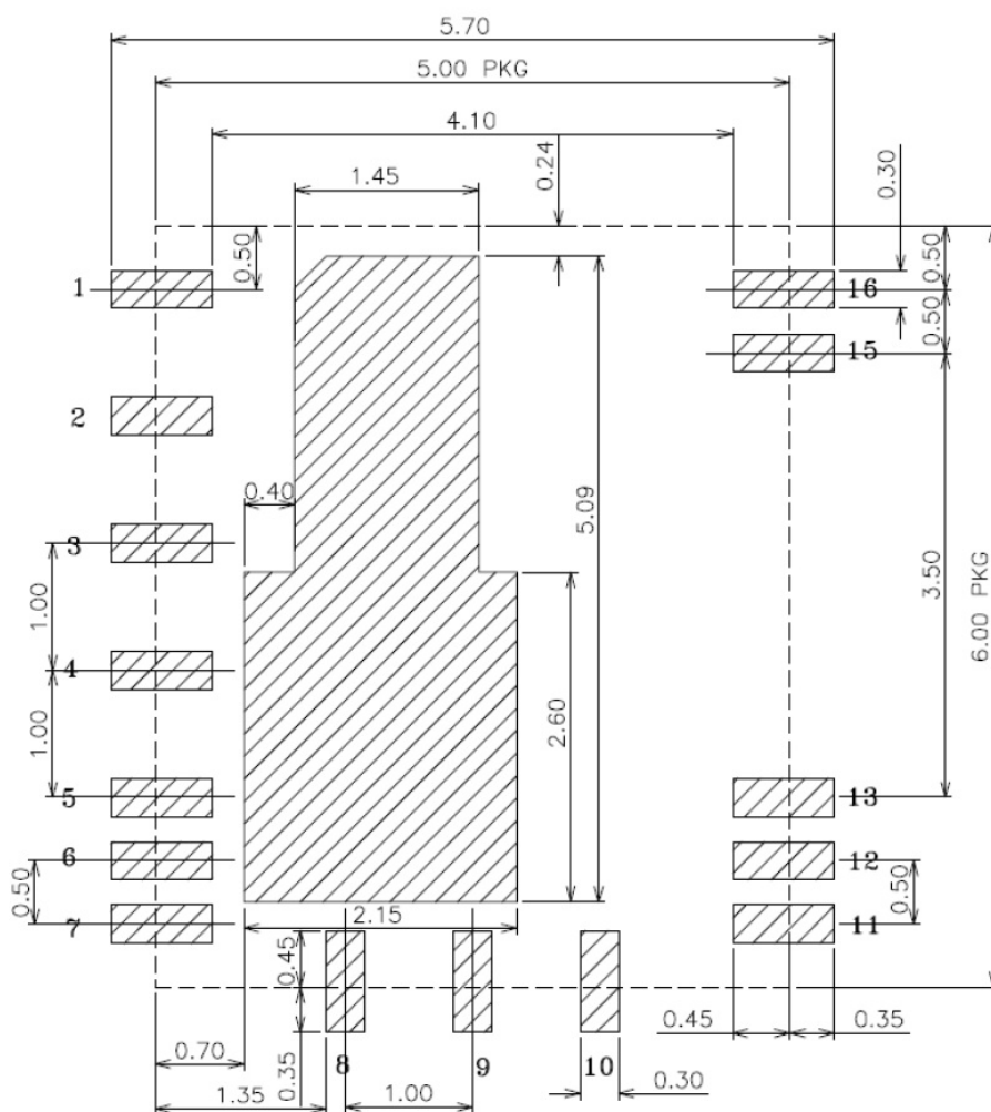
Figure 36. QFN 5x6 package information
