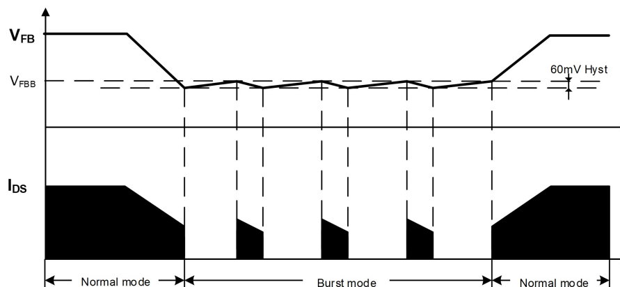
Figure 14. Burst-mode operation
