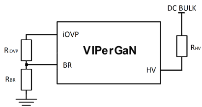
Figure 28. Brown-In/Out and input OVP: external configuration (Input OVP and BR)
