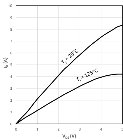
Figure 7. Typ. I_D vs. V_{DS}
