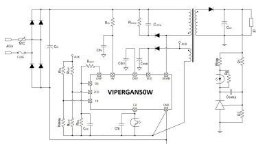
Figure 1. Typical application
