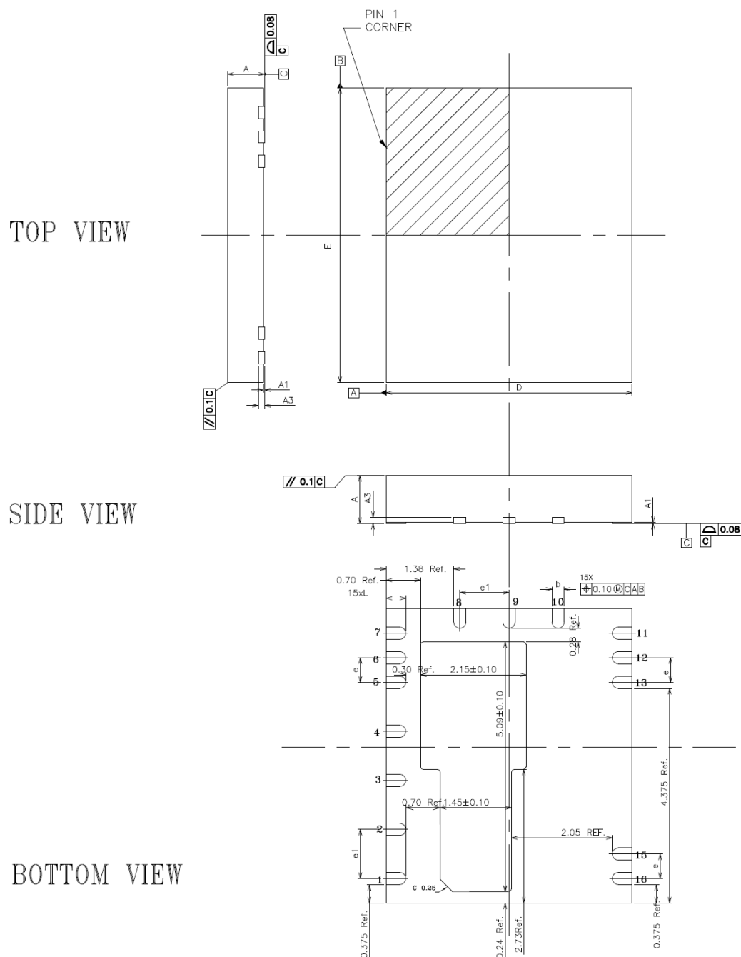
Figure 35. QFN 5x6 package information
