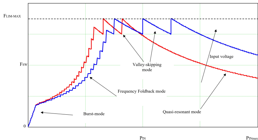
Figure 10. Multi-mode operation of VIPERGAN50W
