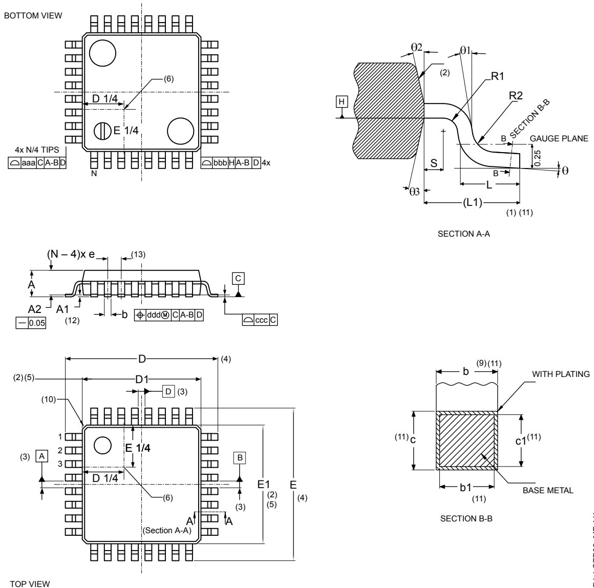
Figure 45. LQFP32- Outline
