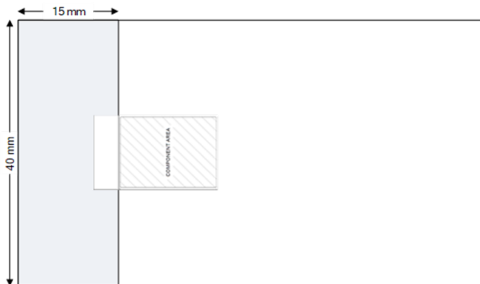
Figure 14. RF layout guideline
