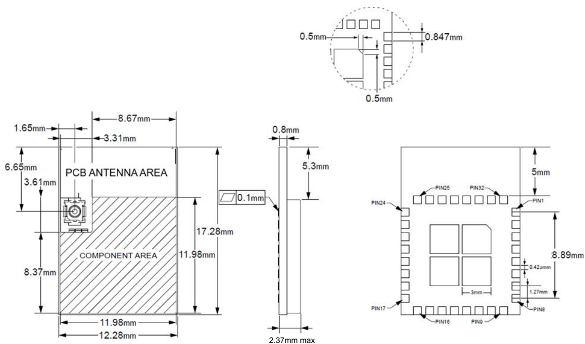
Figure 8. ST67W611M1 LGA module PCB antenna landing pad
