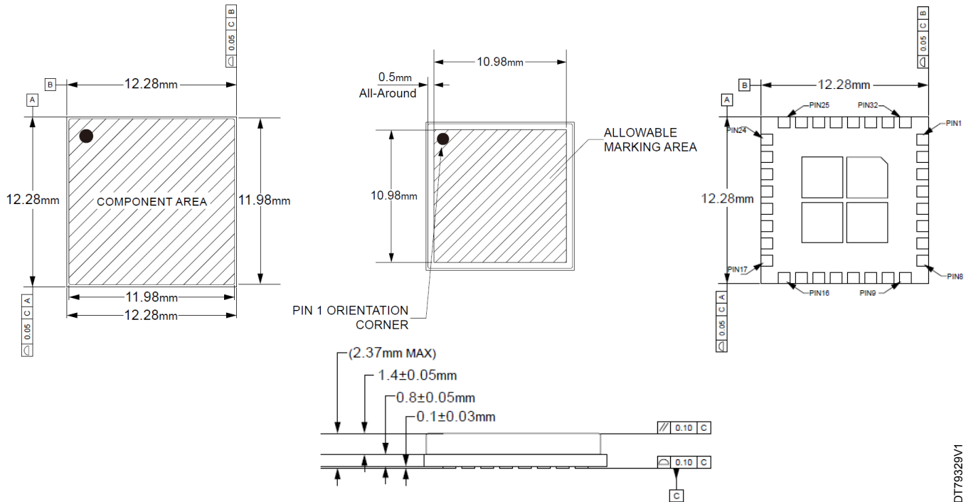
Figure 11. ST67W611M1 LGA module RF pin dimension
