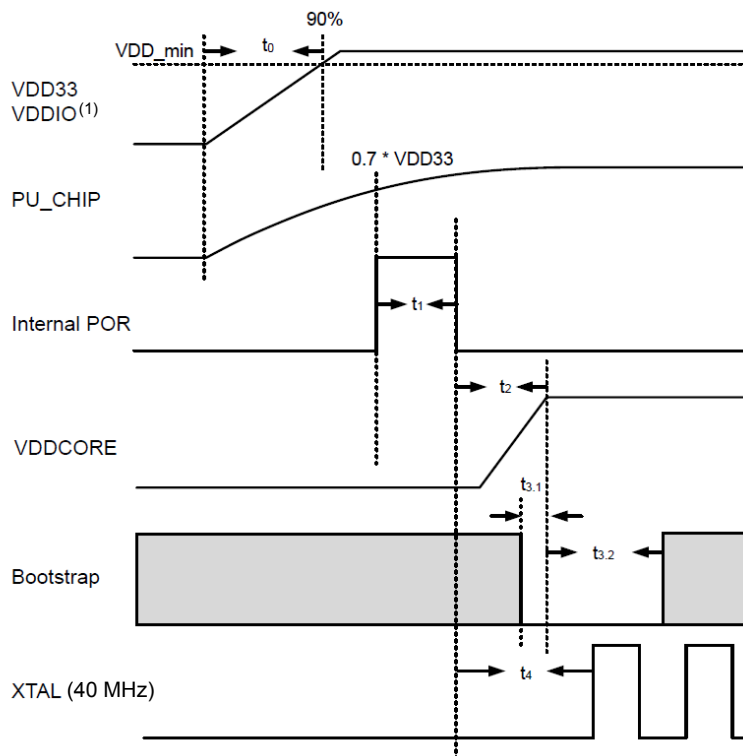
Figure 5. Power-on sequence
