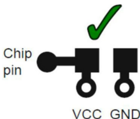
Figure 13. Power layout guideline
