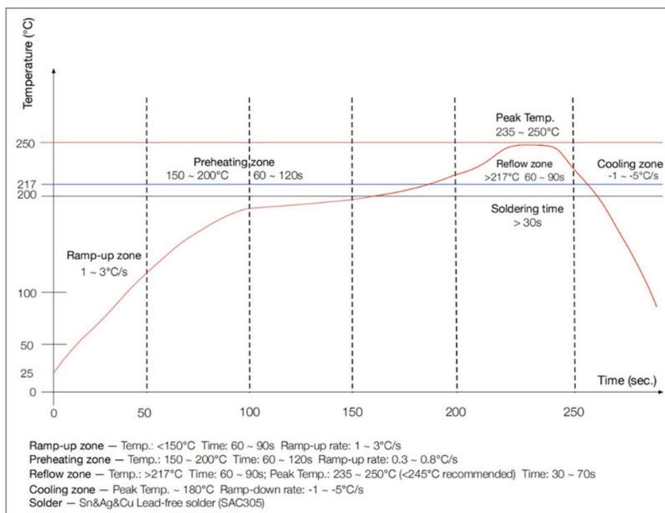
Figure 15. Soldering guideline
