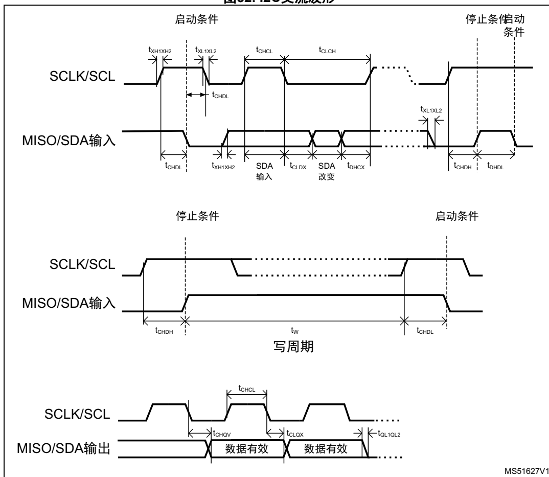
图33. I2C AC measurements
