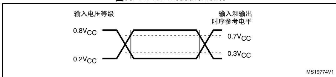
图33. I2C AC measurements
