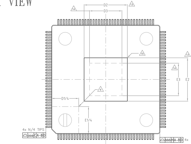
Figure 28. eTQFP144 package outline
