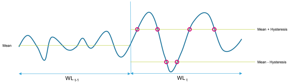
Figure 9. Zero-crossing
