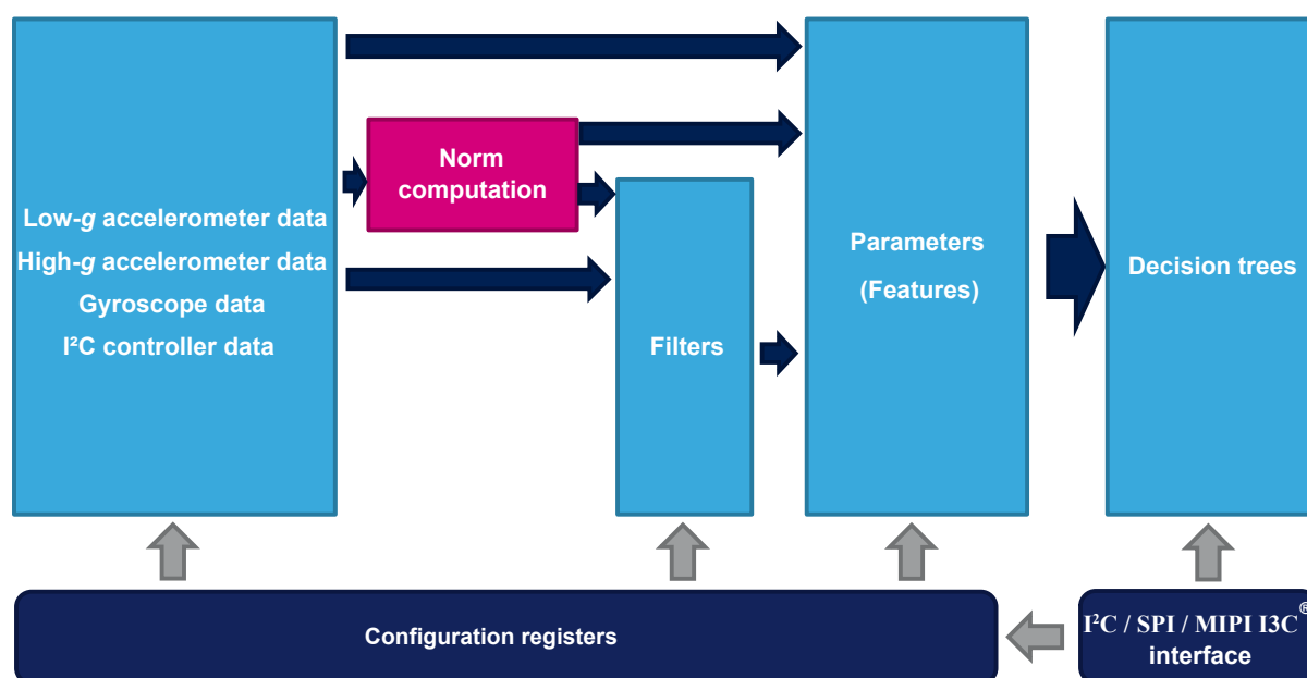
Figure 2. Machine learning core in the LSM6DSV320X
