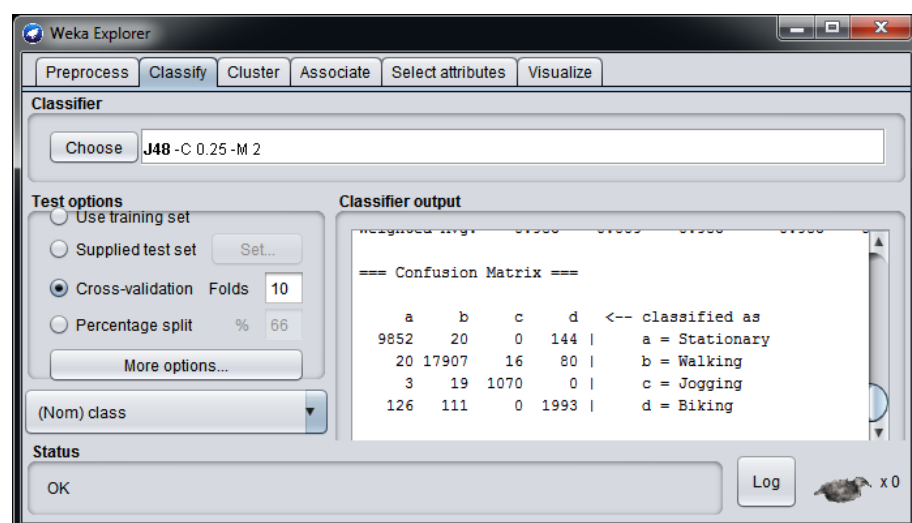
Figure 52. Confusion matrix
