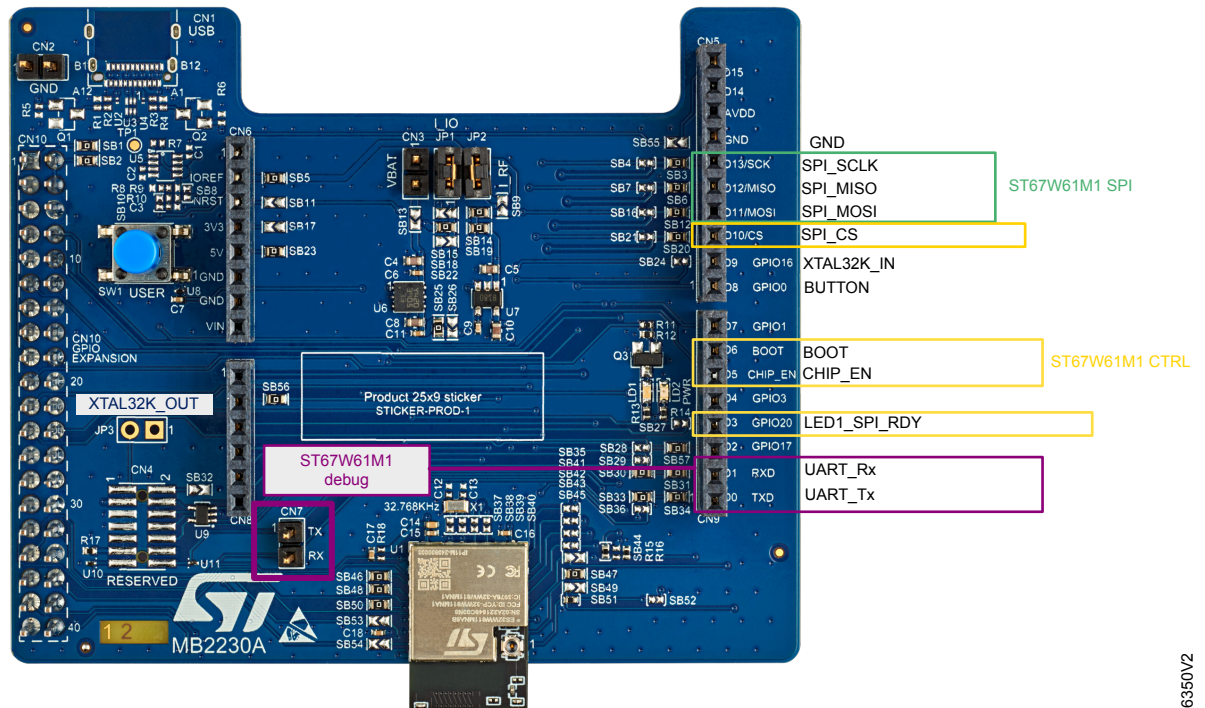
Figure 4. Pin mapping
