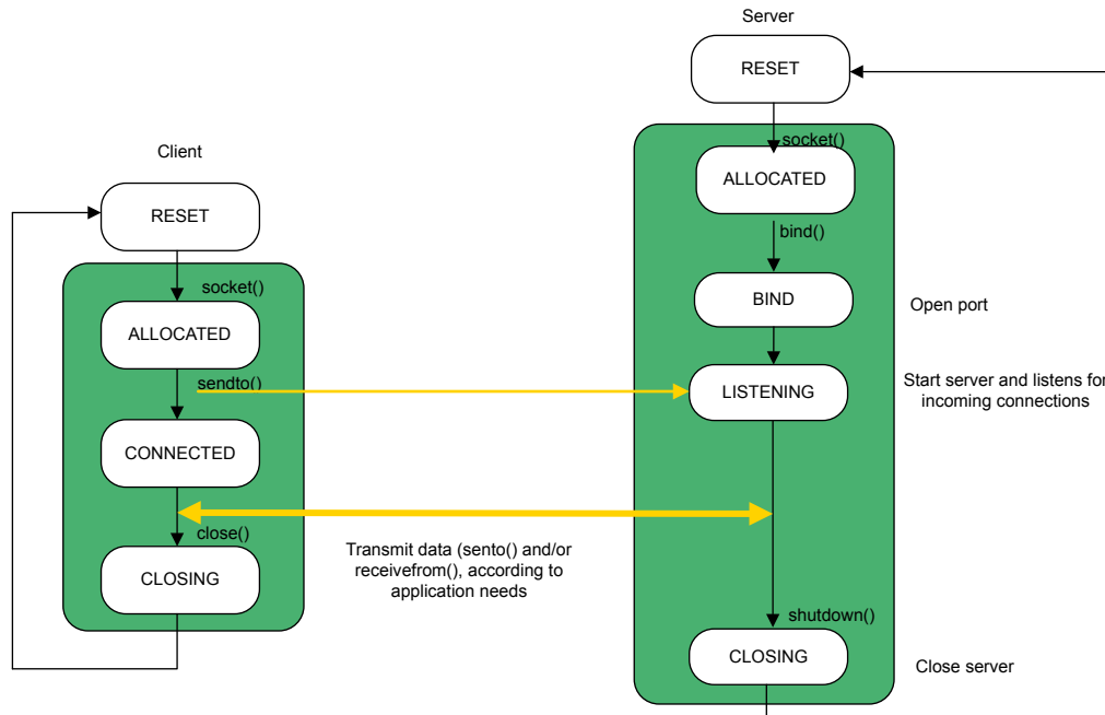
Figure 23. UDP sockets FSM
