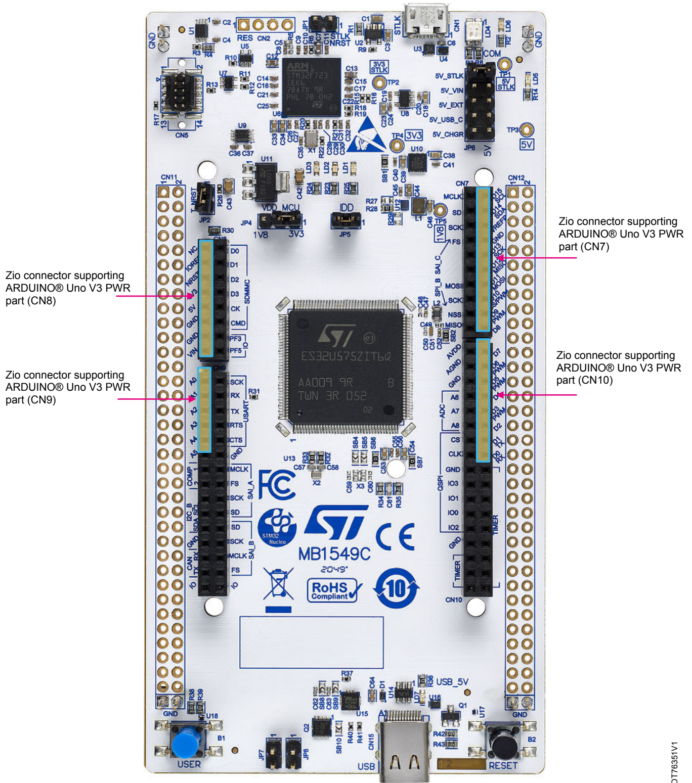
Figure 5. NUCLEO-U575ZI-Q connections
