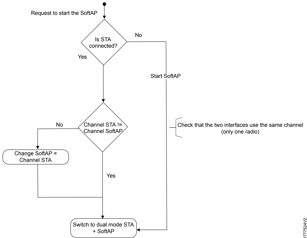
Figure 21. Wi-Fi® STA + SoftAP behavior chart
