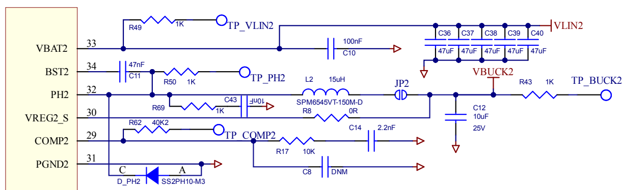
Figure 3. BUCK2 schematic circuit
