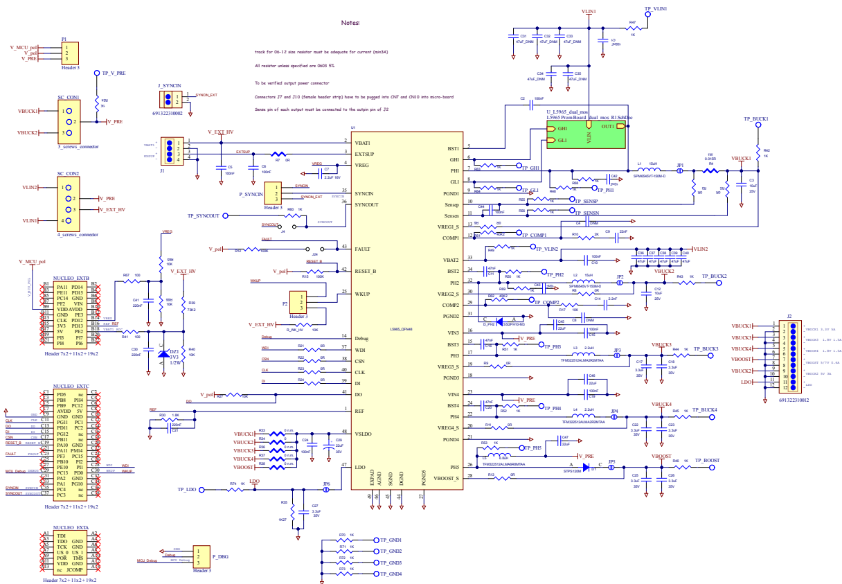
Figure 11. Board schematic
