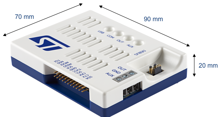
Figure 3. Product dimensions
