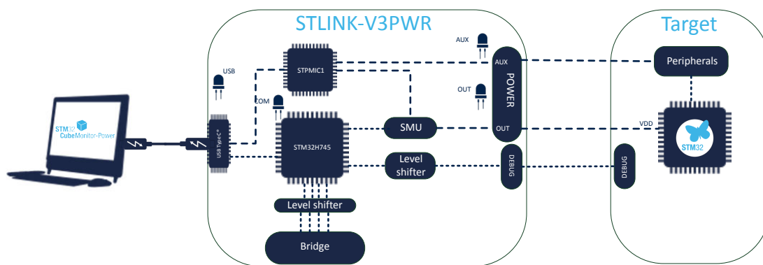
Figure 6. STLINK-V3PWR block diagram
