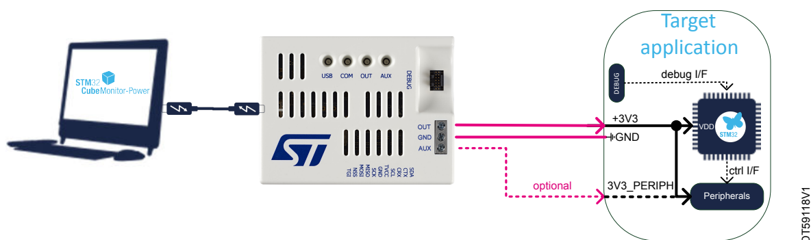
Figure 4. STLINK-V3PWR connection
