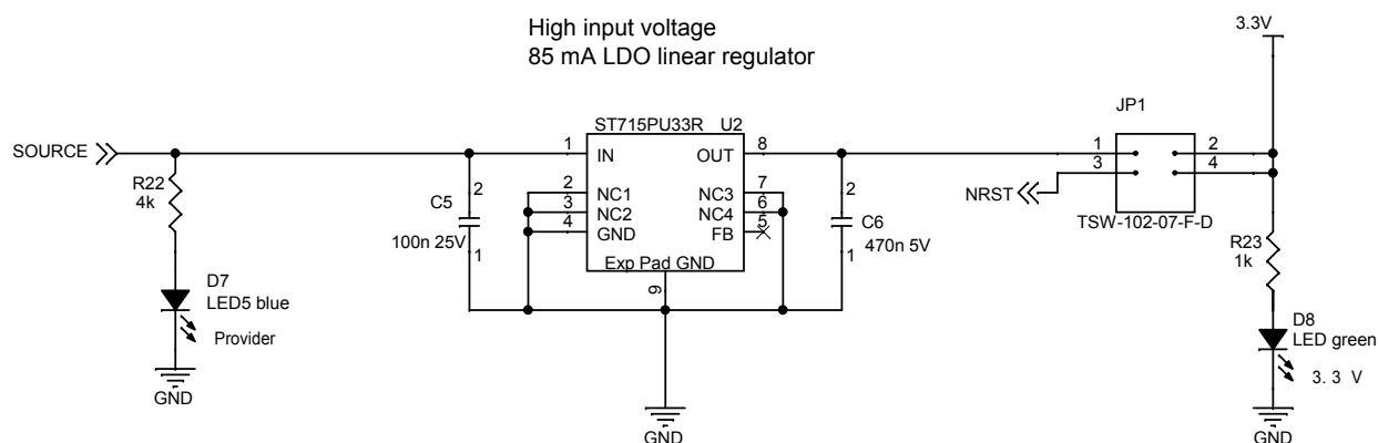
Figure 12. LDO configuration
