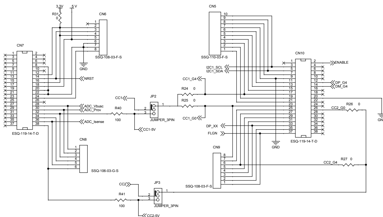
Figure 8. ST morpho and Arduino UNO V3 connectors
