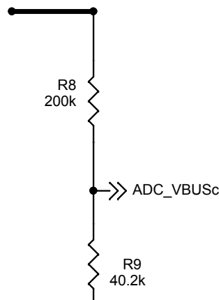
Figure 10. V_{BUS} voltage sense for the STM32 ADC
