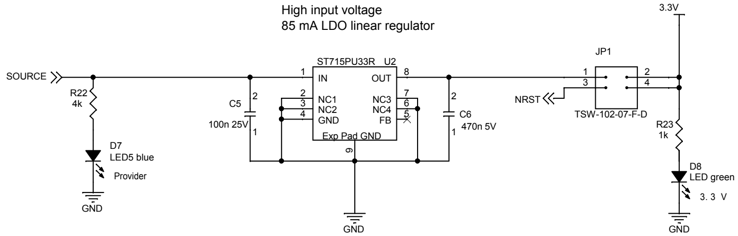
Figure 16. X-NUCLEO-SRC1M1 circuit schematic (3 of 3)
