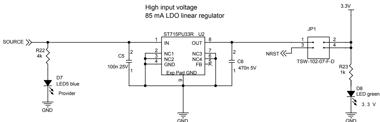
Figure 13. TCPP02-M18
