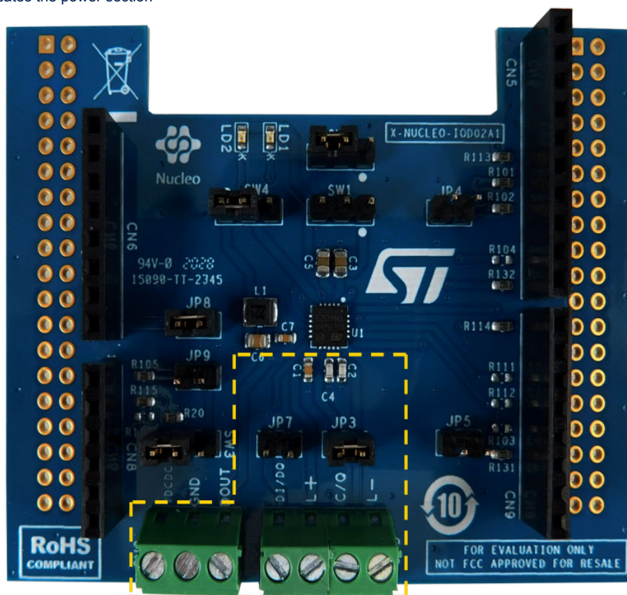
Figure 3. X-NUCLEO-IOD02A1 expansion board
