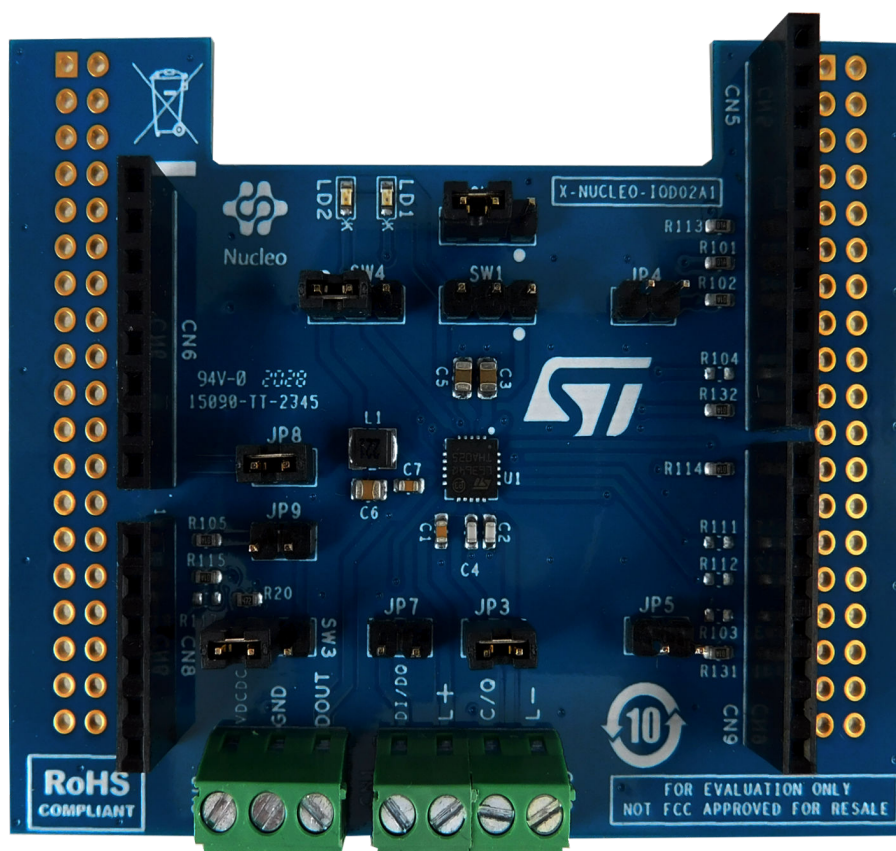
Figure 1. X-NUCLEO-IOD02A1 expansion board
