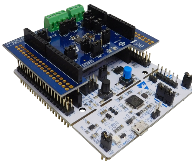
Figure 4. X-NUCLEO-IOD02A1 and STM32 Nucleo stack
