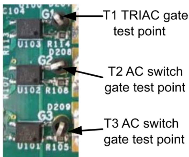
Figure 14. STEVAL-GLA001V1 evaluation board AC switch gate control (secondary side) components
