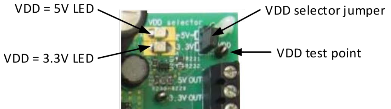
Figure 9. STEVAL-GLA001V1 evaluation board VDD selector components
