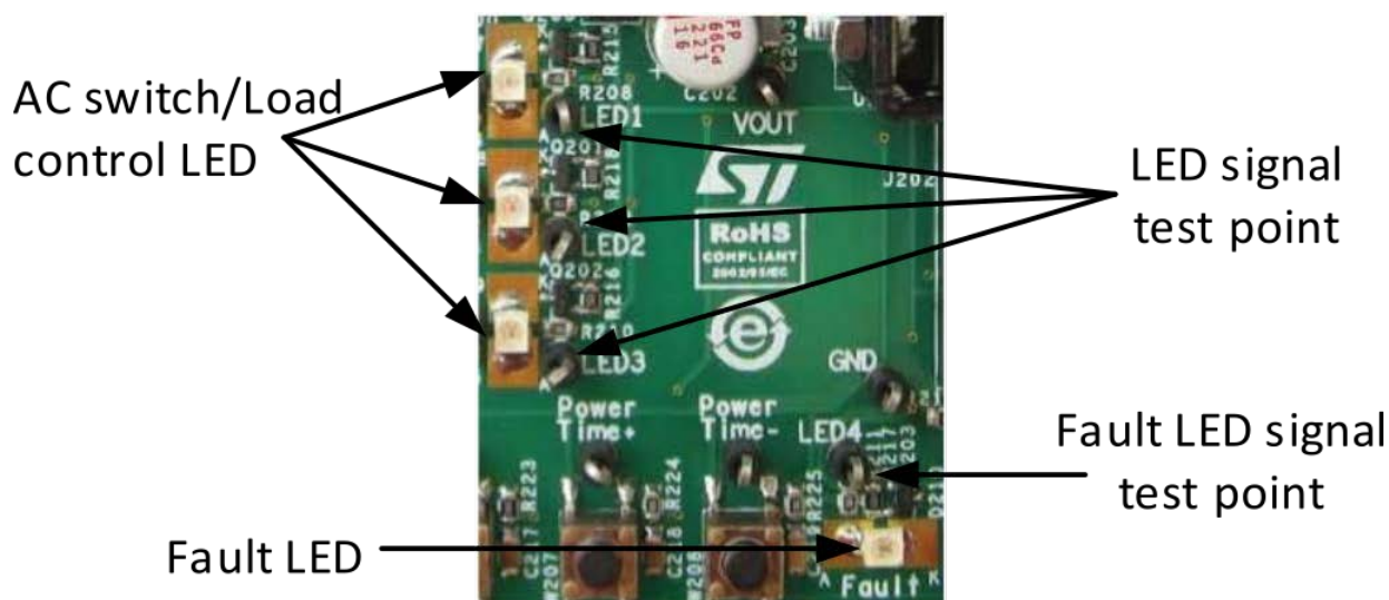
Figure 11. STEVAL-GLA001V1 evaluation board LED components
