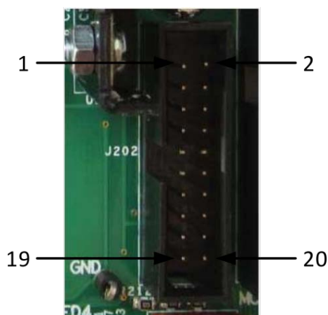
Figure 29. User connector pinning
