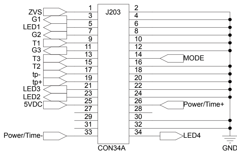
Figure 39. 34-Pin ST board connector
