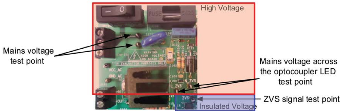
Figure 16. STEVAL-GLA001V1 evaluation board ZVS components
