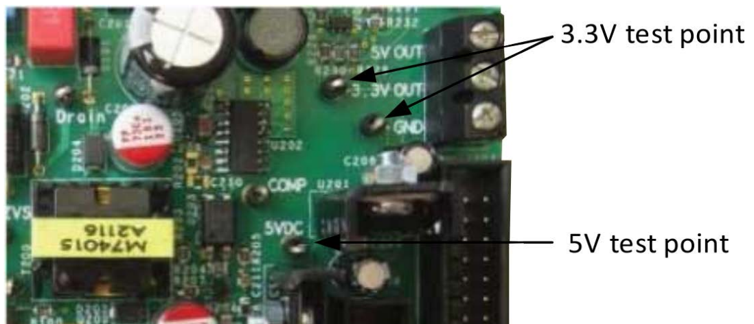
Figure 8. STEVAL-GLA001V1 evaluation board power supply secondary side components
