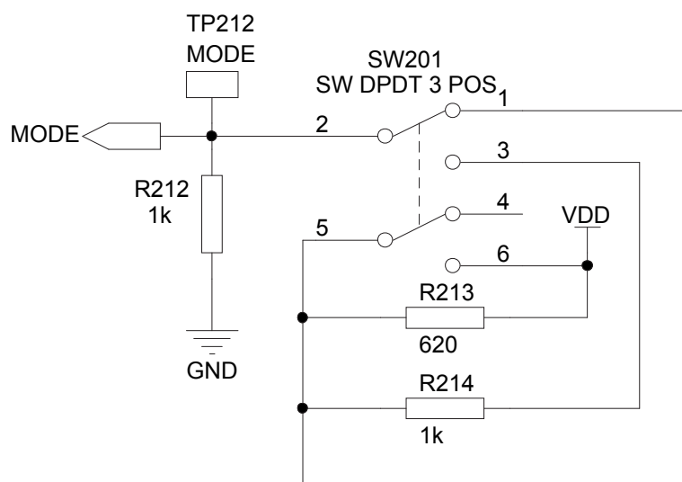
Figure 37. STEVAL-GLA001V1 - Mode selector switch
