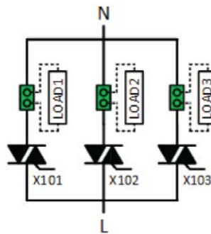
Figure 3. Loads connection versus AC switches
