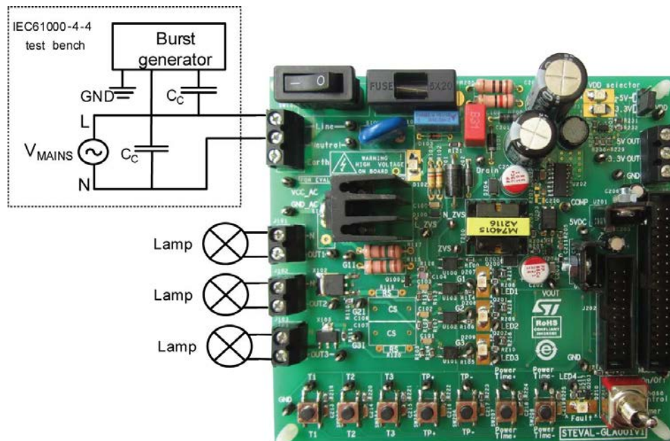
Figure 44. IEC61000-4-4 test with STEVAL-GLA001V1
