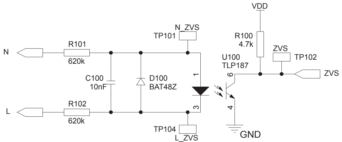
Figure 31. STEVAL-GLA001V1 - ZVS detection
