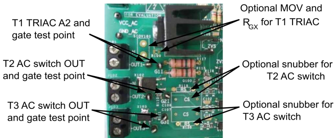
Figure 13. STEVAL-GLA001V1 evaluation board AC switch gate control (primary side) components
