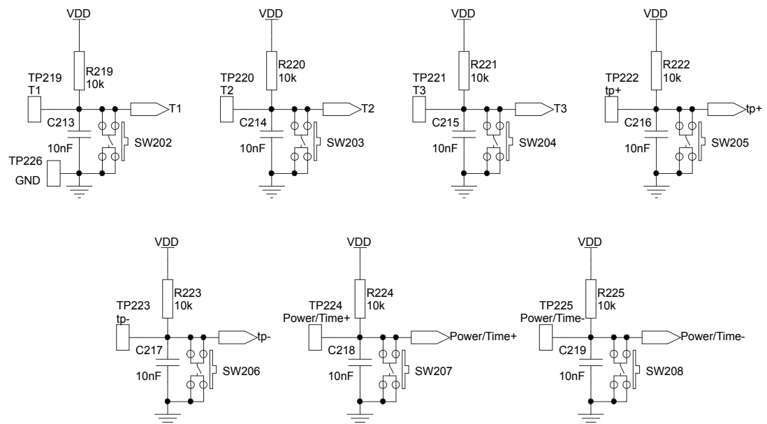
Figure 36. STEVAL-GLA001V1 - Commands/parameters push buttons
