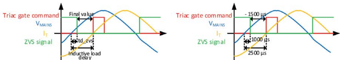
Figure 26. Parameters in case of inductive load (example on the right)
