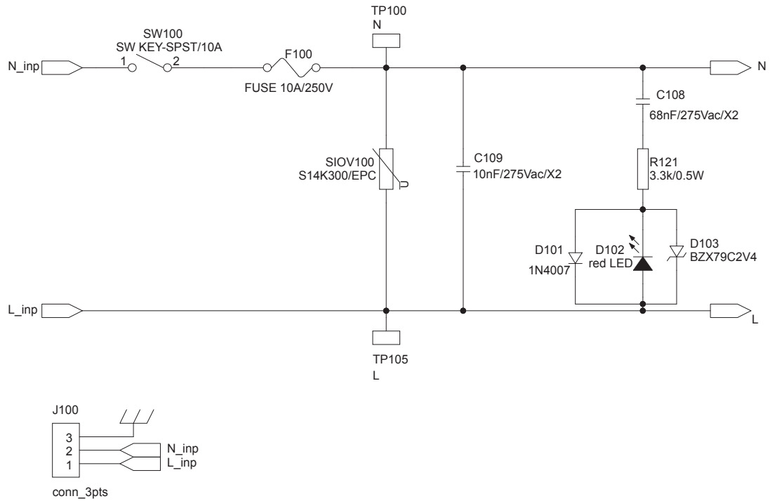
Figure 30. STEVAL-GLA001V1 - AC input
