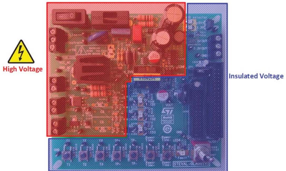
Figure 4. High voltage and insulated voltage on STEVAL-GLA001V1 evaluation board
