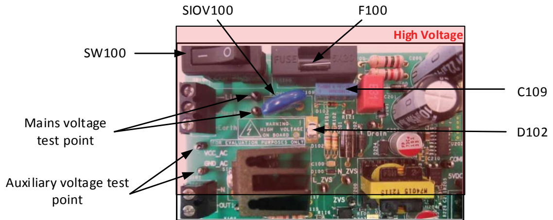
Figure 7. STEVAL-GLA001V1 evaluation board power supply primary side components
