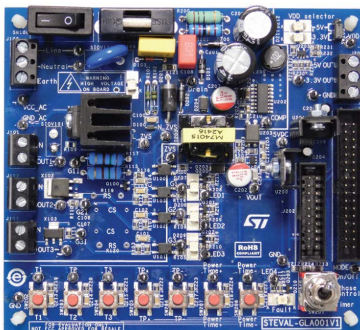
Figure 1. STEVAL-GLA001V1 evaluation board (top view)
