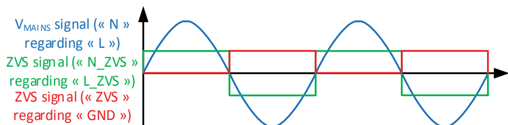
Figure 15. ZVS signal versus mains voltage
