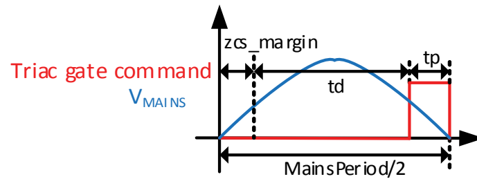
Figure 27. Parameters for phase control mode
