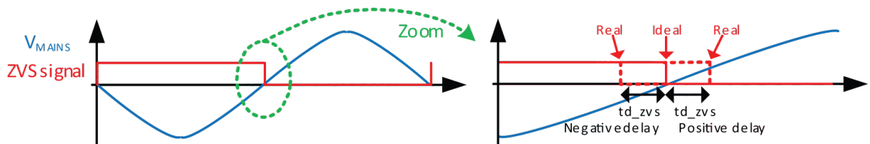
Figure 25. ZVS signal versus mains voltage (zoom on the right)
