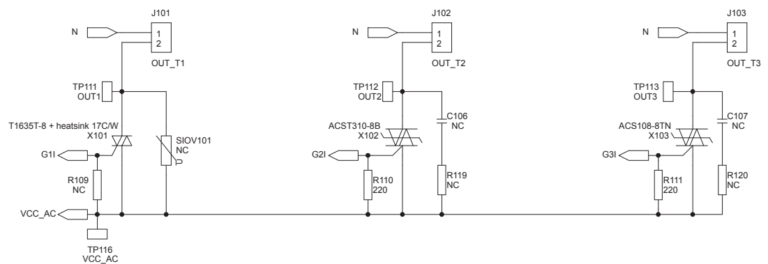
Figure 33. STEVAL-GLA001V1 - Triacs/ACS connection
