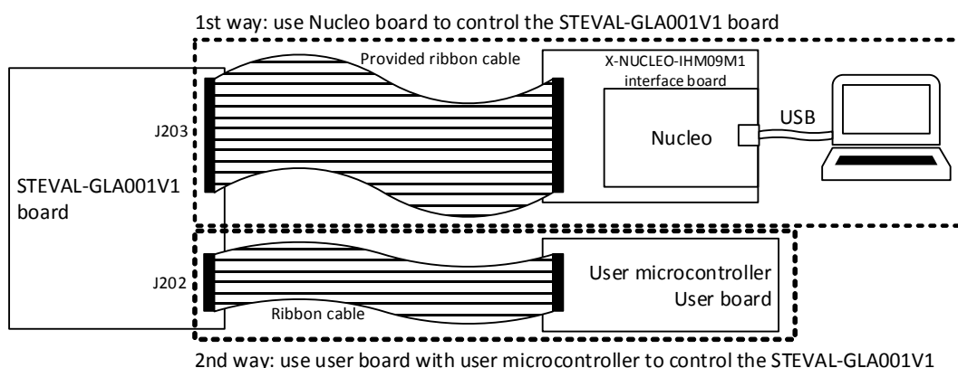
Figure 17. Ways to control the STEVAL-GLA001V1 evaluation board
