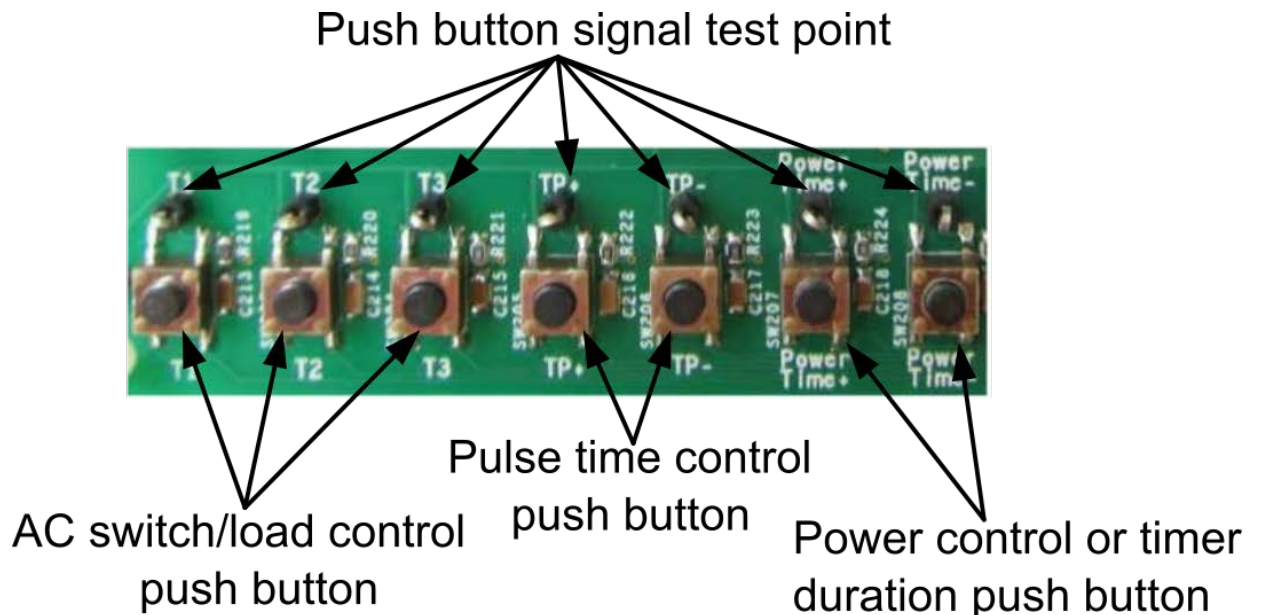
Figure 10. STEVAL-GLA001V1 evaluation board push button components
