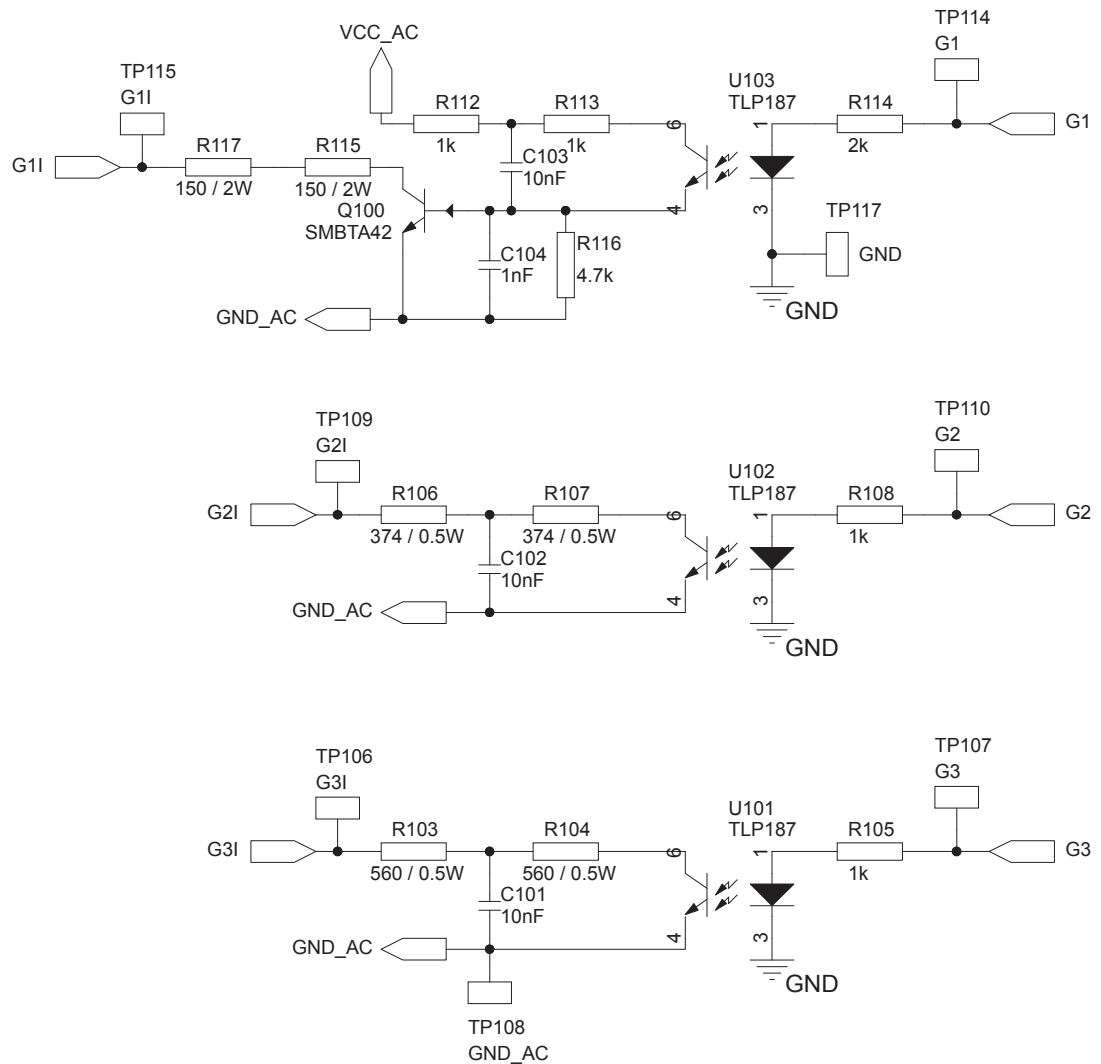
Figure 32. STEVAL-GLA001V1 - Triac gate control
