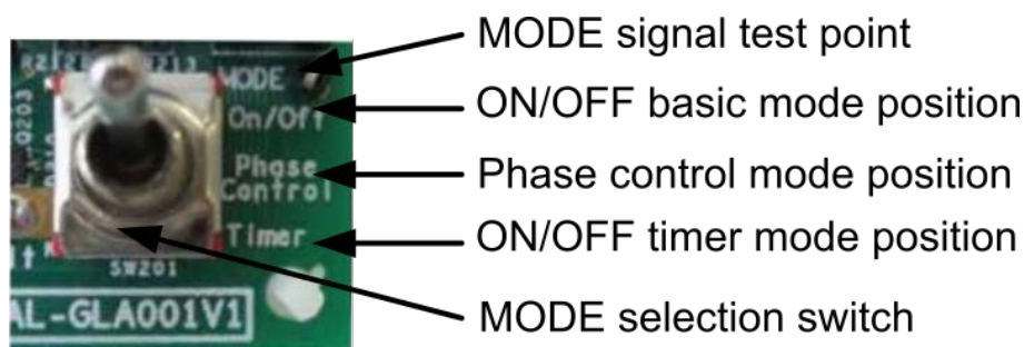
Figure 12. STEVAL-GLA001V1 evaluation board mode components
