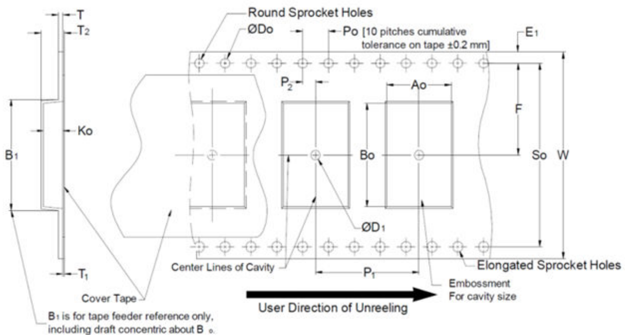
Figure 6. Embossed carrier tape (32 mm widths)
