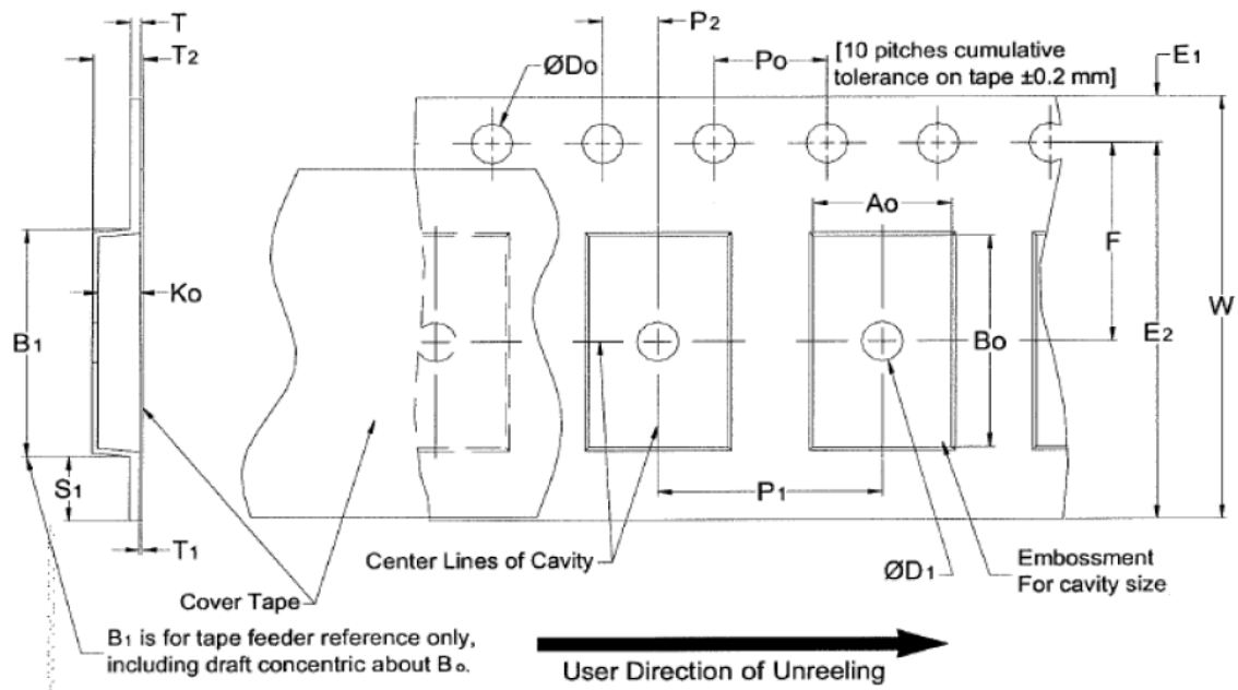
Figure 5. Embossed carrier tape (12 mm, 16 mm, and 24 mm widths)
