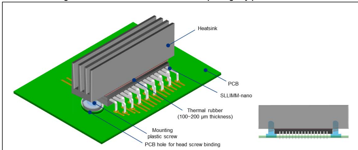
Figure 14. Large heatsink bonded on the package by plastic screws
