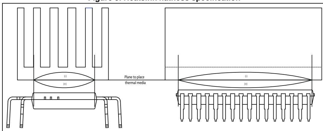
Figure 3. Heatsink flatness specification
