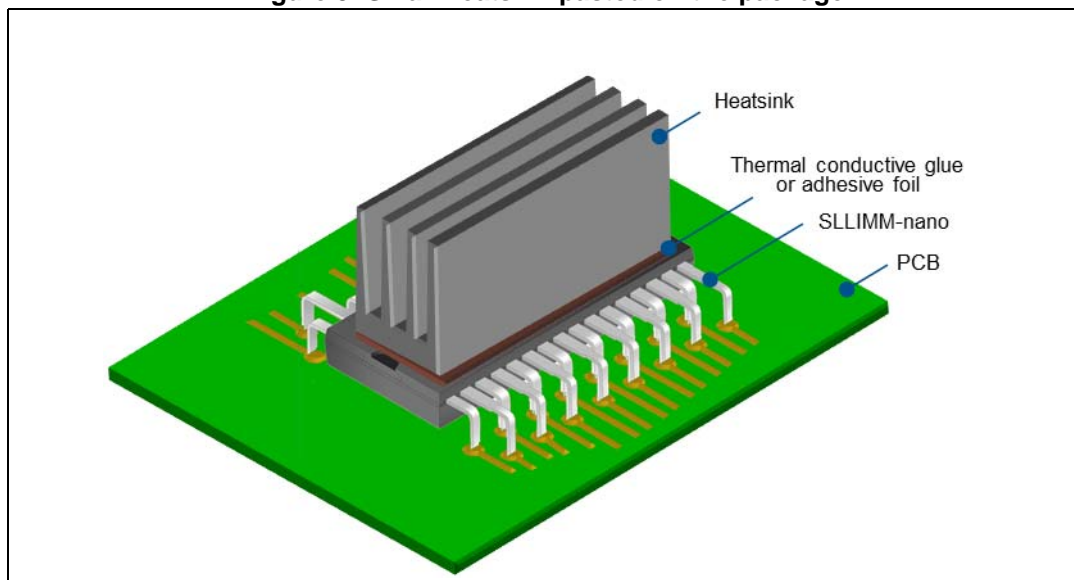
Figure 9. Small heatsink pasted on the package
