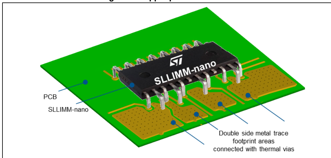
Figure 8. Copper plate on the PCB
