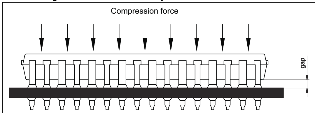
Figure 4. Heatsink force delivery to the leads of SLLIMM-nano
