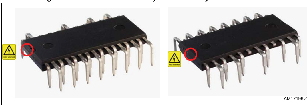
Figure 6. Heatsink force delivery onto the body of SLLIMM-nano
