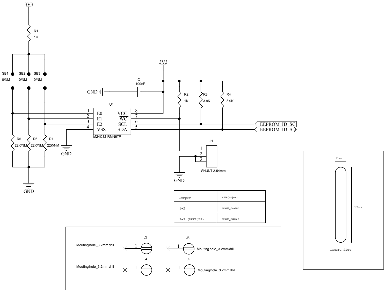
Figure 2. X-STM32MP-RBT01 circuit schematics (2 of 10)
