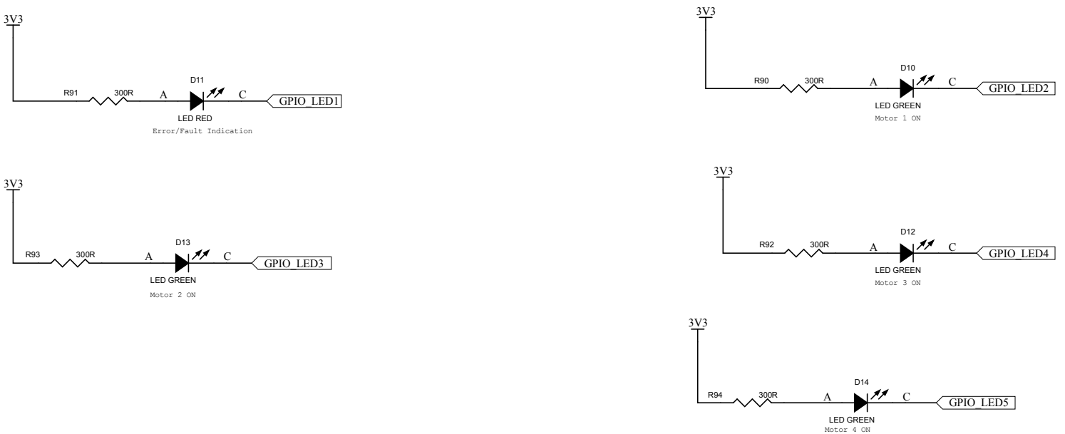
Figure 10. X-STM32MP-RBT01 circuit schematics (10 of 10)
