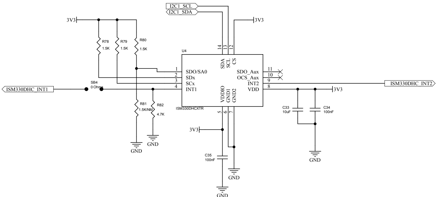
Figure 6. X-STM32MP-RBT01 circuit schematics (6 of 10)
