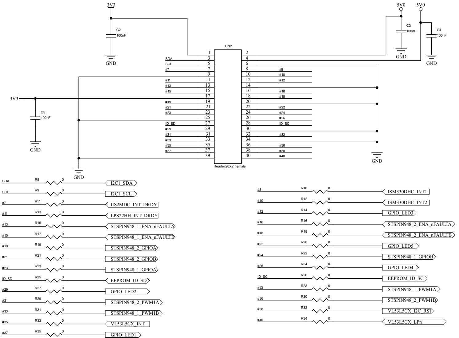
Figure 3. X-STM32MP-RBT01 circuit schematics (3 of 10)
