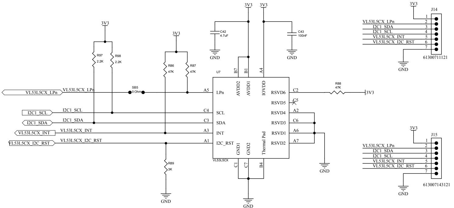
Figure 9. X-STM32MP-RBT01 circuit schematics (9 of 10)
