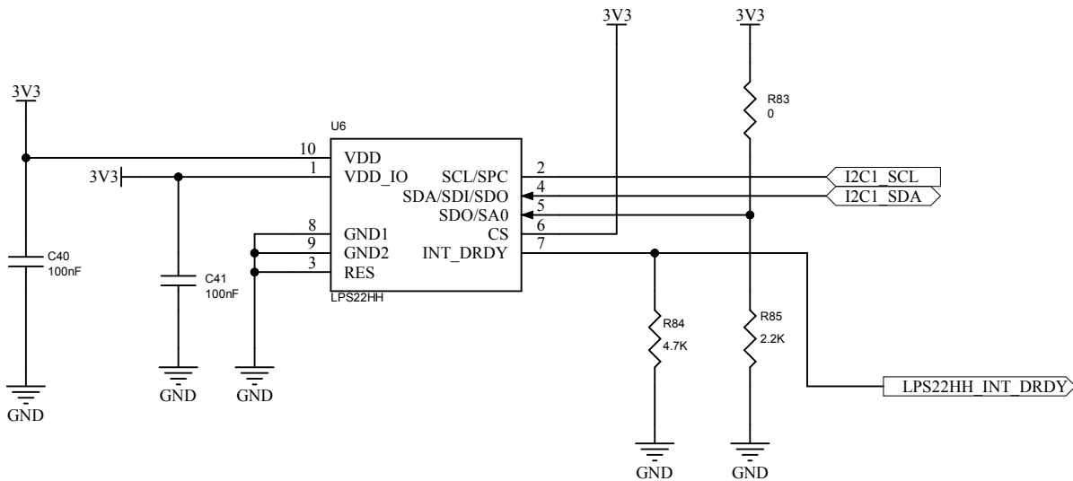
Figure 8. X-STM32MP-RBT01 circuit schematics (8 of 10)
