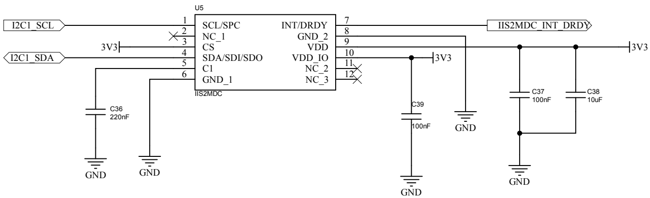
Figure 7. X-STM32MP-RBT01 circuit schematics (7 of 10)
