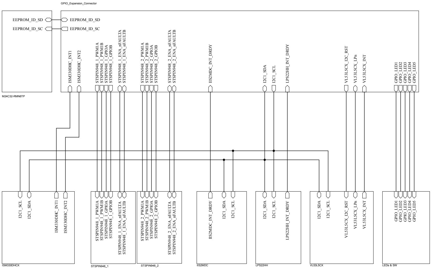
Figure 1. X-STM32MP-RBT01 circuit schematics (1 of 10)
