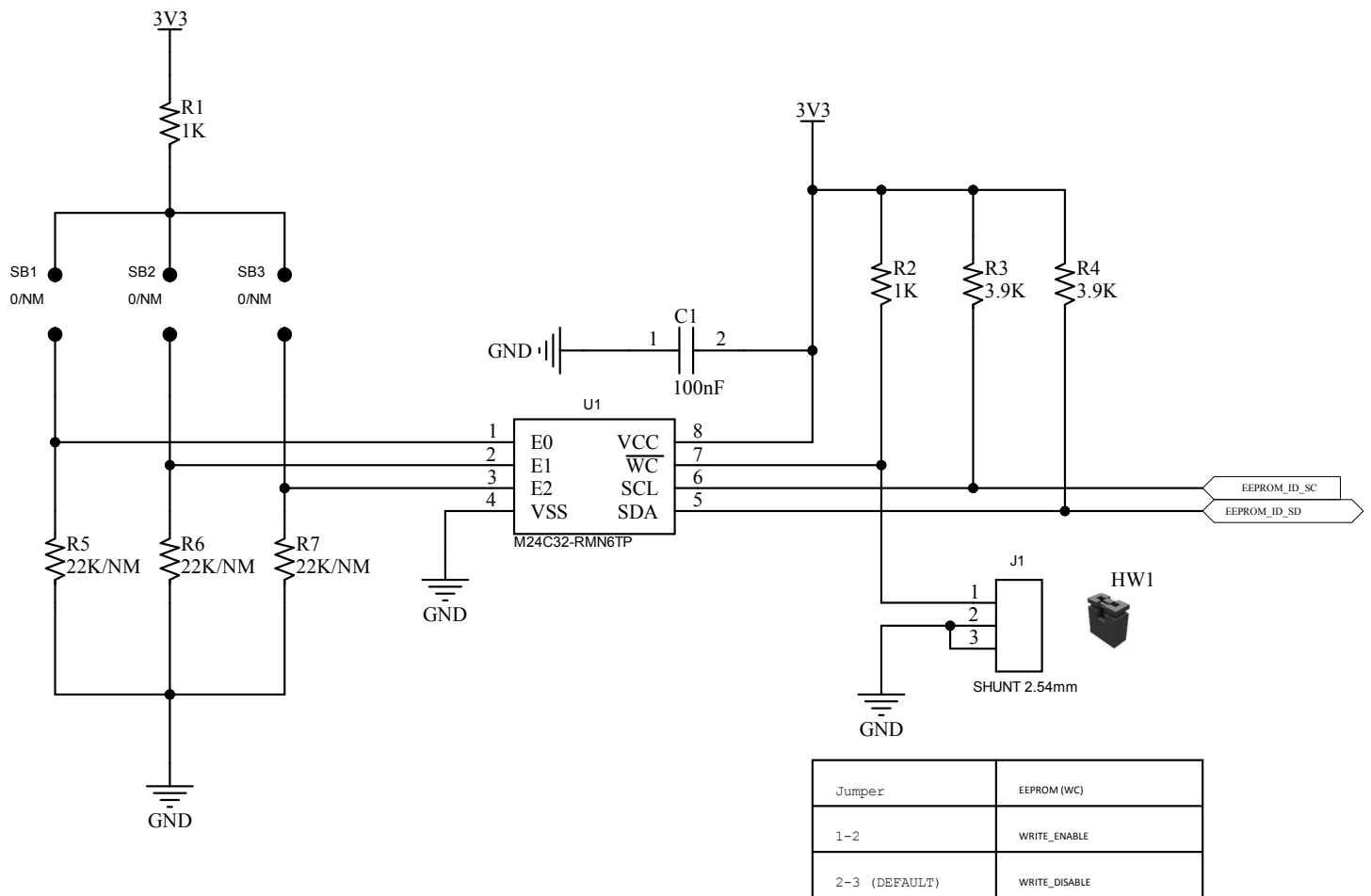
Figure 2. X-STM32MP-IGTW1 circuit schematic (2 of 10)
