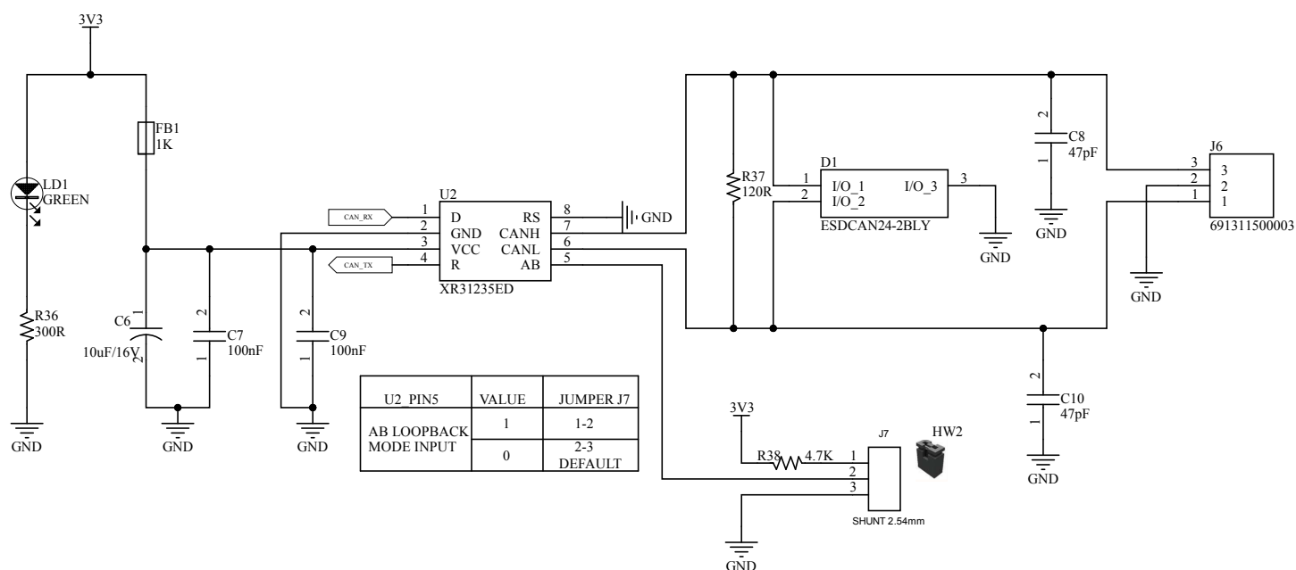
Figure 4. X-STM32MP-IGTW1 circuit schematic (4 of 10)
