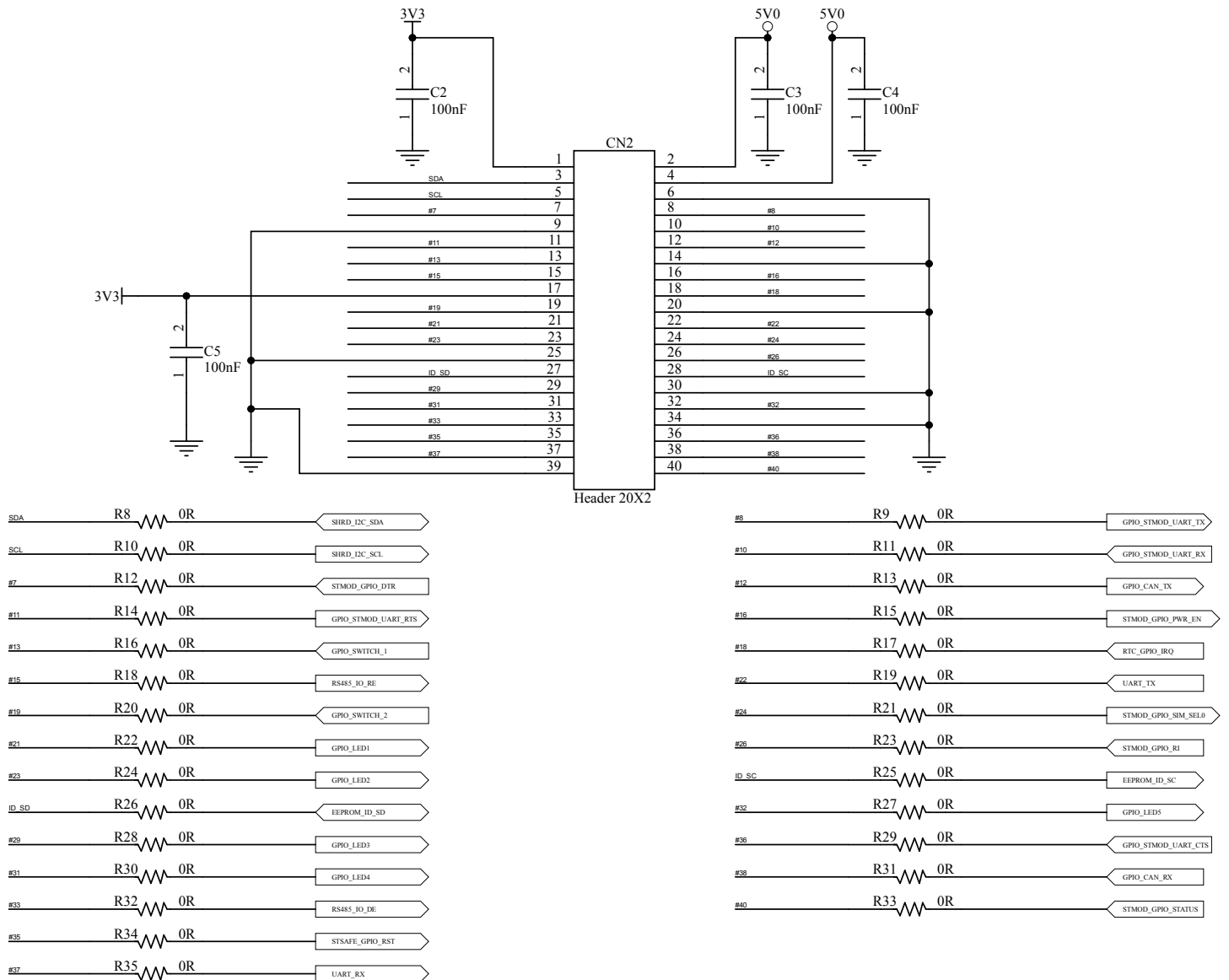
Figure 3. X-STM32MP-IGTW1 circuit schematic (3 of 10)
