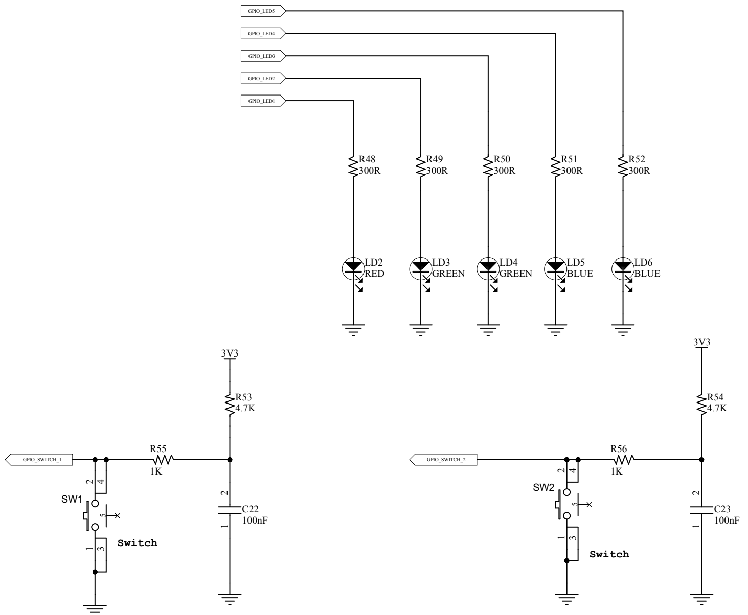
Figure 9. X-STM32MP-IGTW1 circuit schematic (9 of 10)
