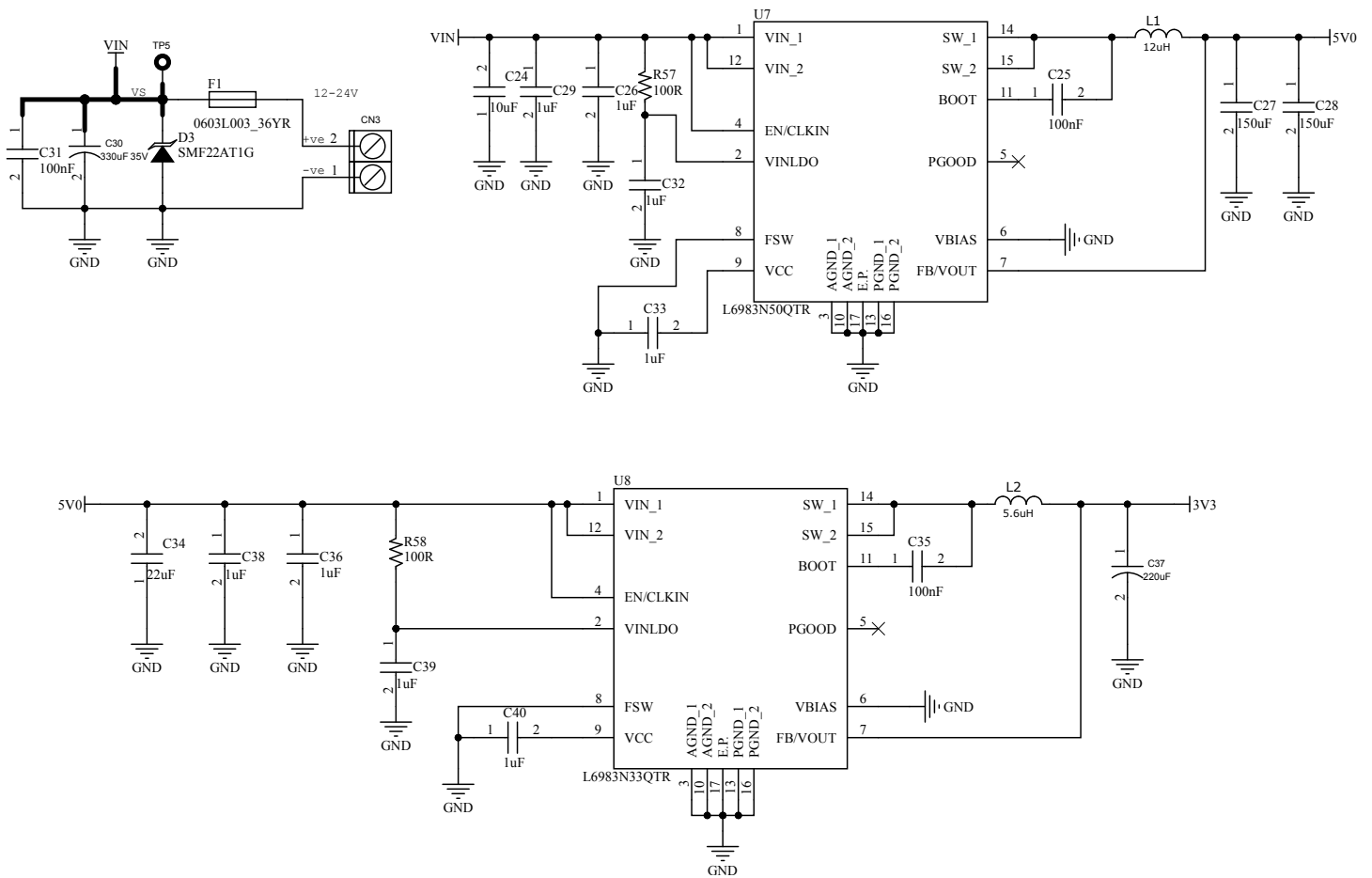
Figure 10. X-STM32MP-IGTW1 circuit schematic (10 of 10)
