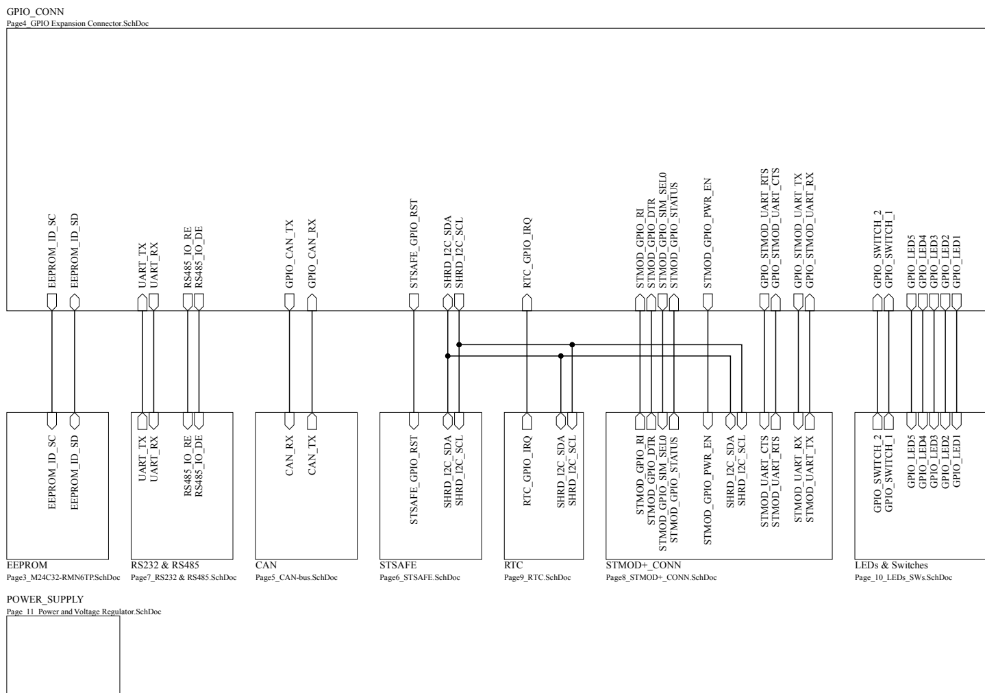
Figure 1. X-STM32MP-IGTW1 circuit schematic (1 of 10)
