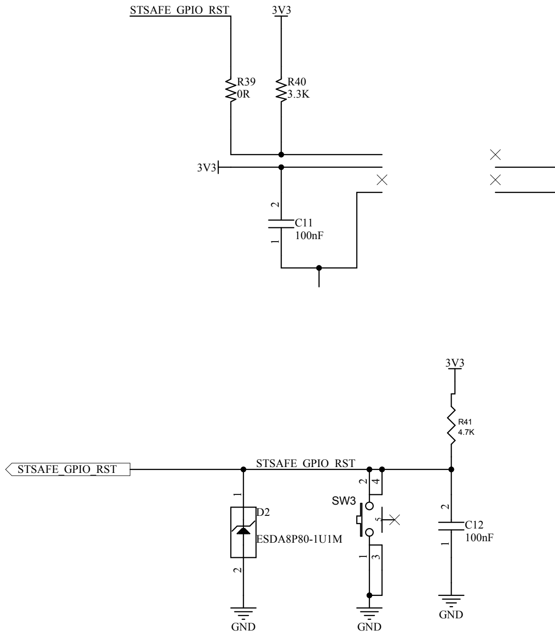
Figure 5. X-STM32MP-IGTW1 circuit schematic (5 of 10)
