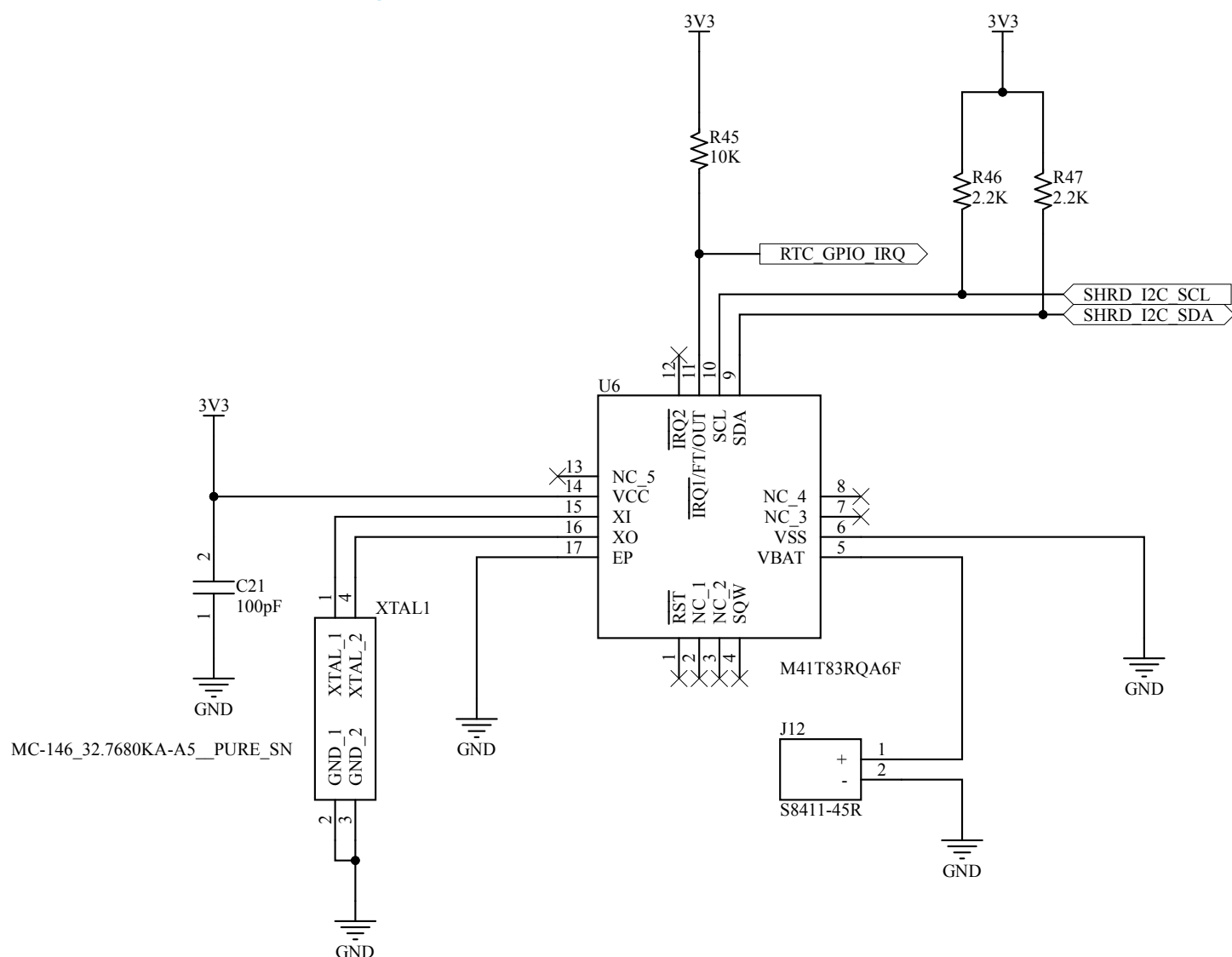
Figure 8. X-STM32MP-IGTW1 circuit schematic (8 of 10)
