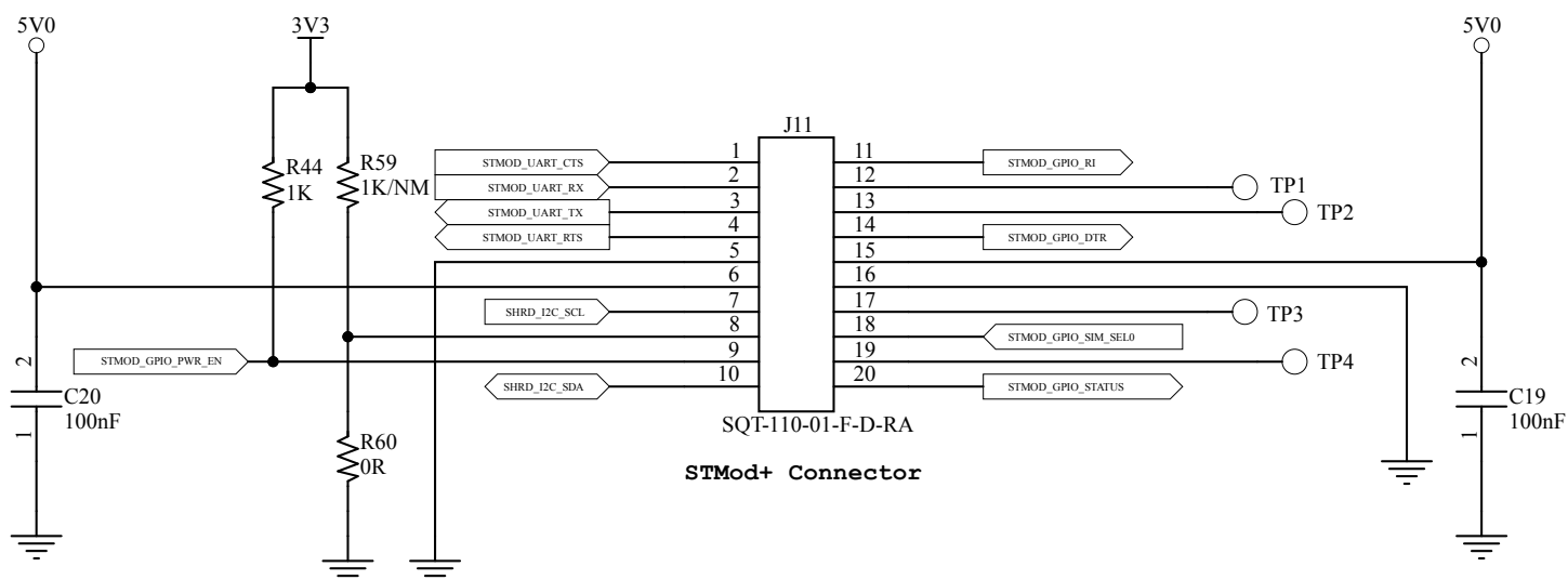
Figure 7. X-STM32MP-IGTW1 circuit schematic (7 of 10)
