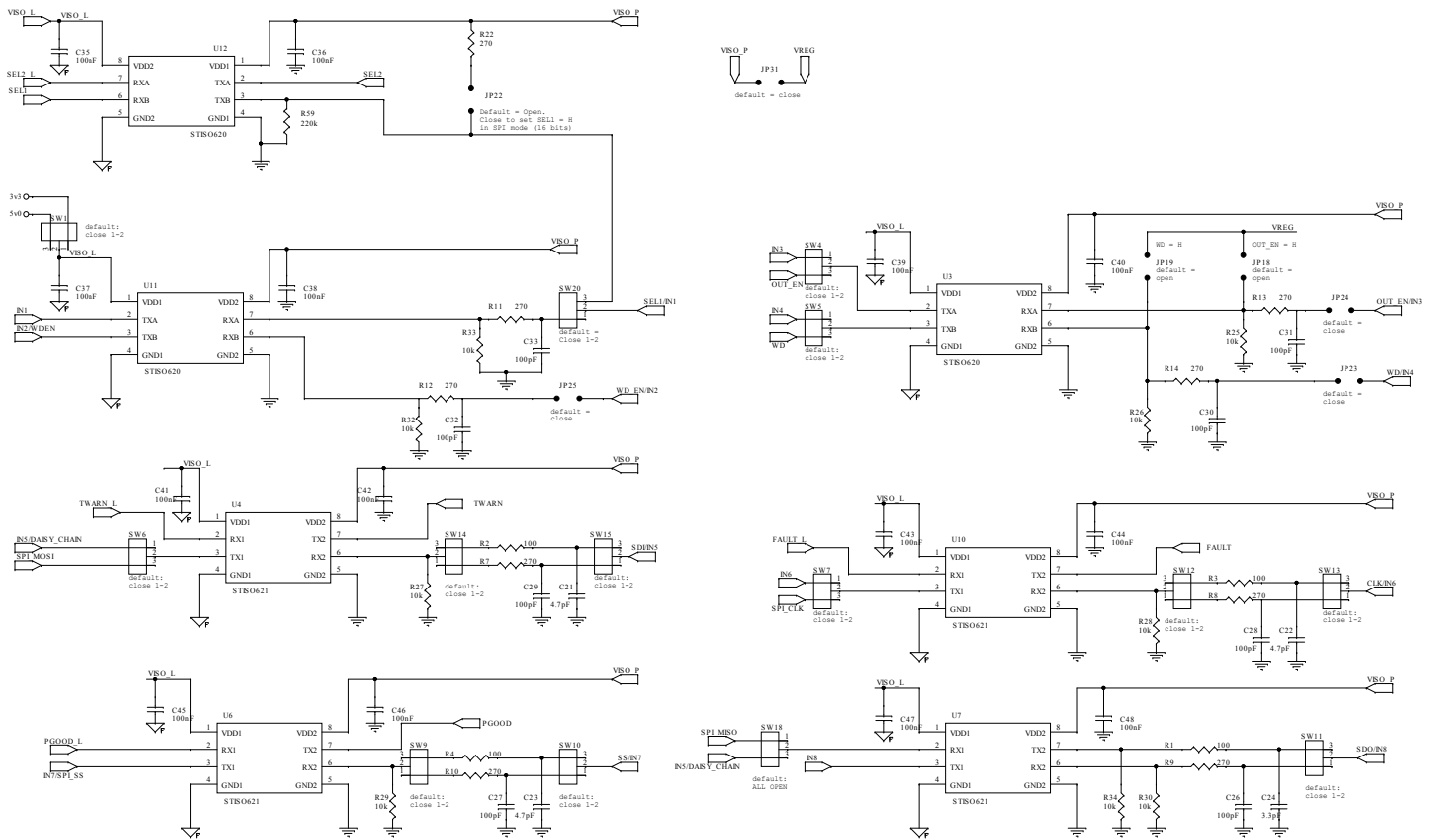
Figure 2. X-NUCLEO-OUT16A1 circuit schematic (2 of 3)
