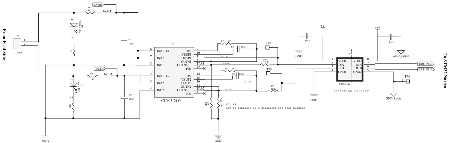
Figure 2. X-NUCLEO-ISO1A1 circuit schematic (2 of 4)
