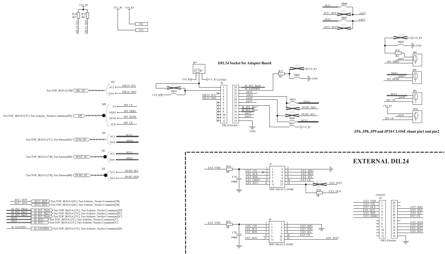
Figure 4. X-NUCLEO-IKS5A1 circuit schematic (4 of 4)
