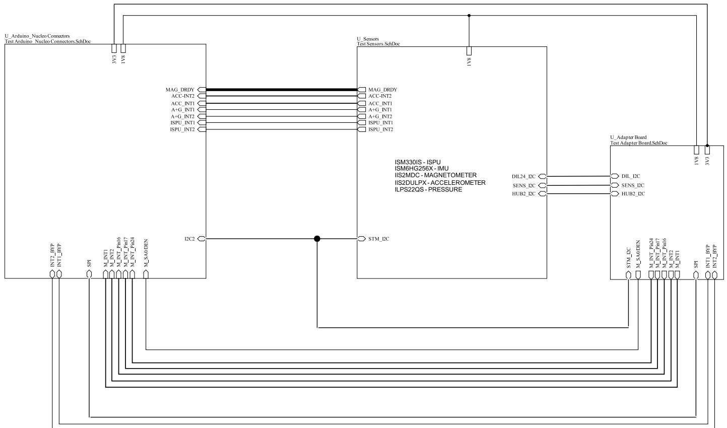
Figure 1. X-NUCLEO-IKS5A1 circuit schematic (1 of 4)
