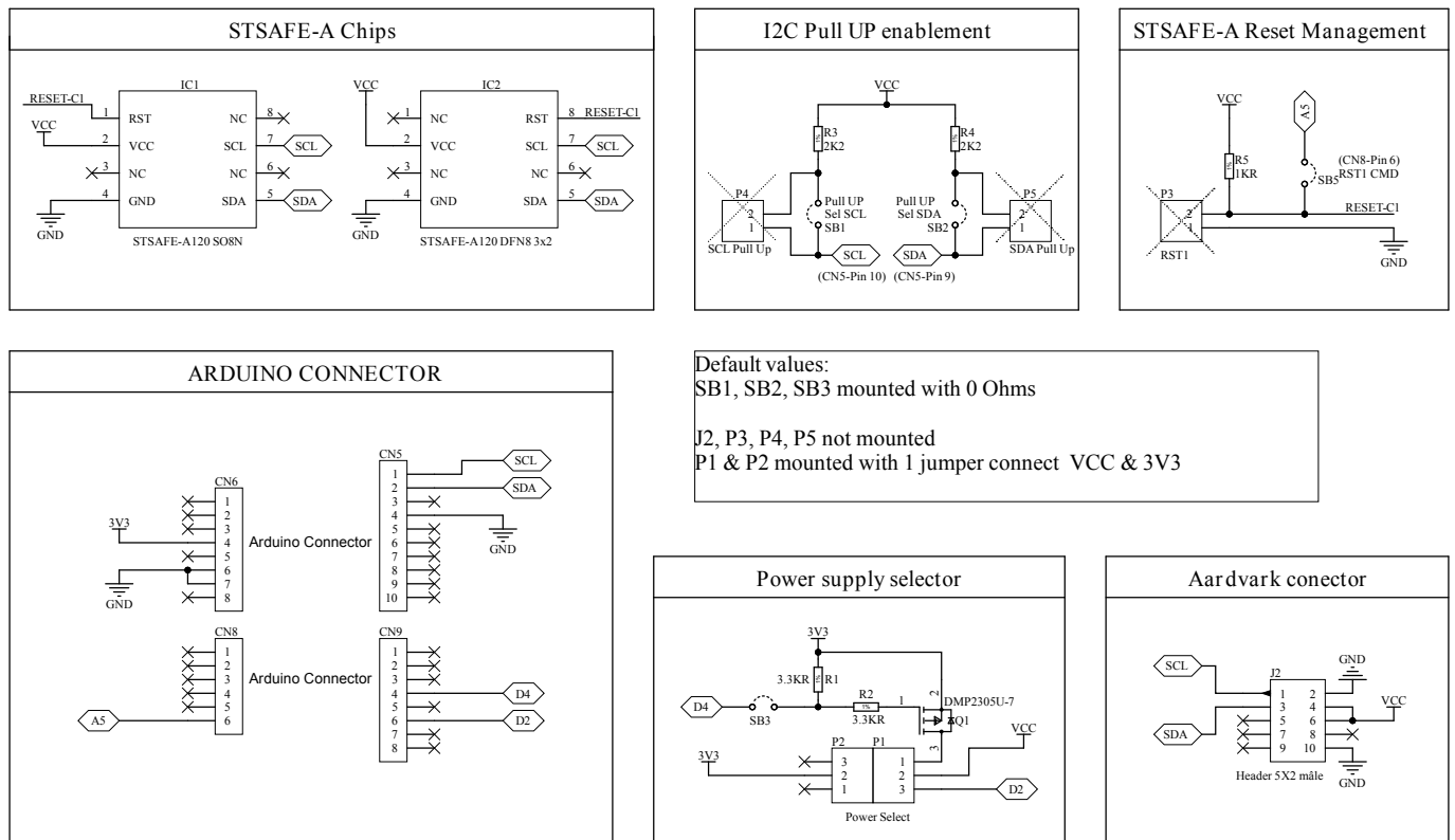
Figure 1. X-NUCLEO-ESE01A1 circuit schematic
