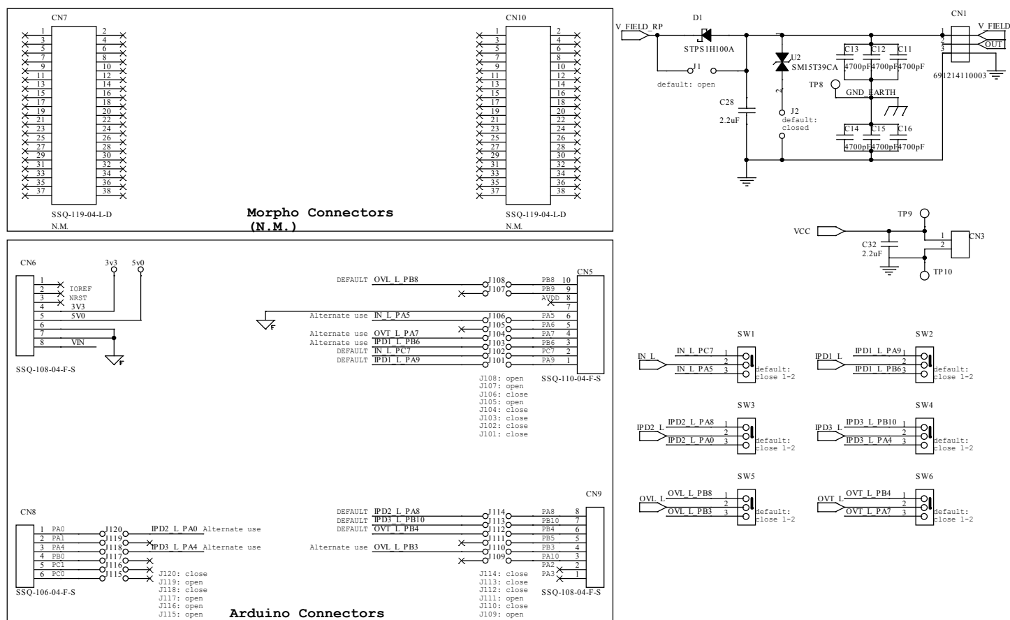
Figure 1. X-NUCLEO-DOL10A1 circuit schematic (1 of 2)
