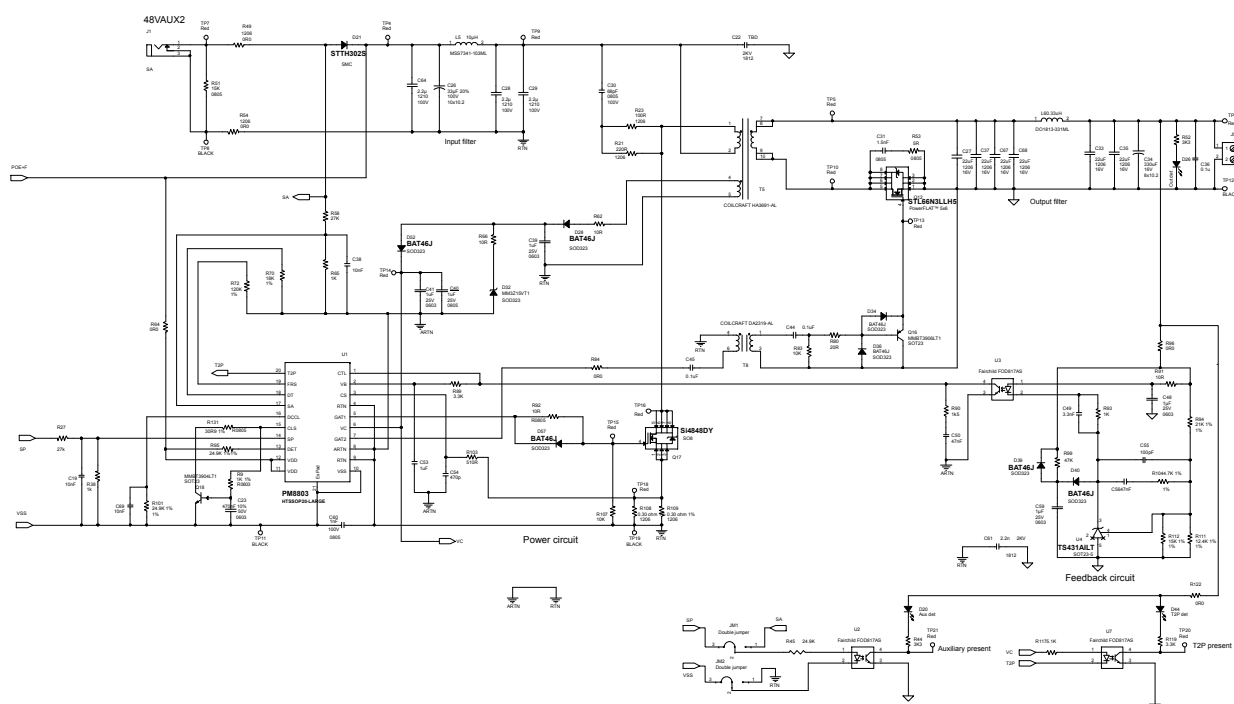
Figure 2. STEVAL-TSP004V2 circuit schematic (2 of 2)
