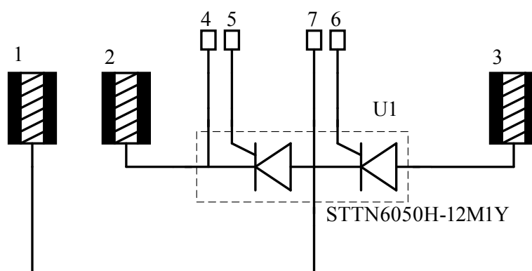
Figure 1. STEVAL-TO240SCR schematic
