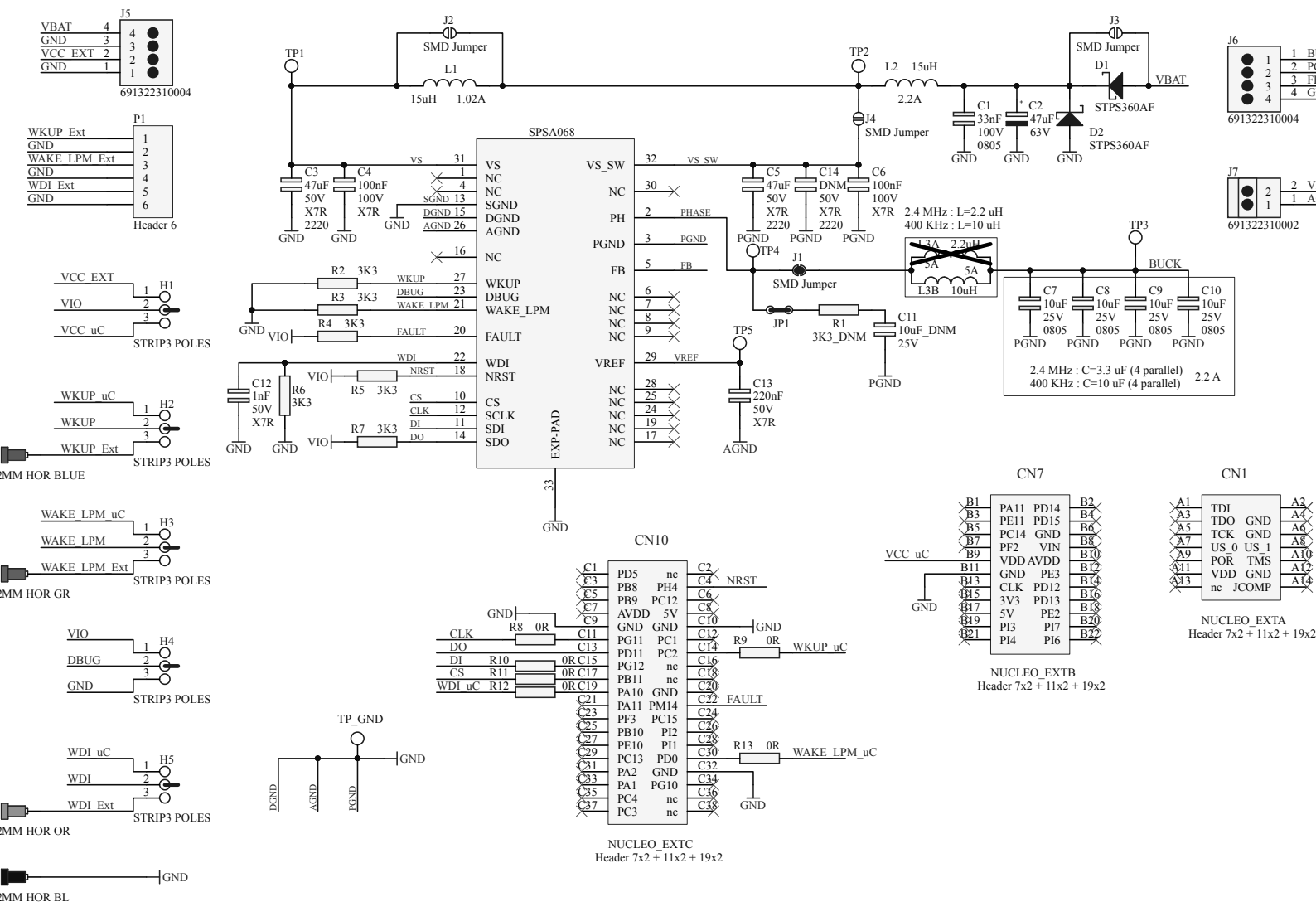
Figure 1. STEVAL-SPSA068 schematic
