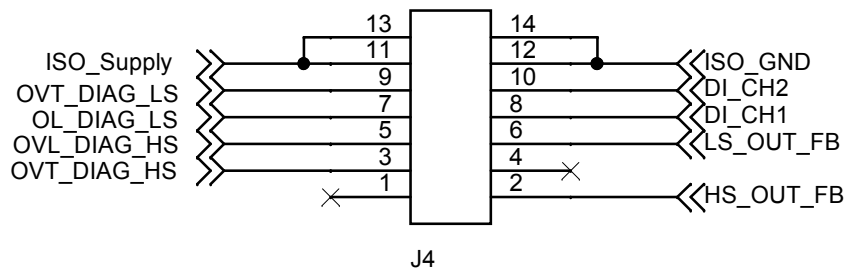
Figure 23. STEVAL-SILKTB01 circuit schematic (2 of 12)
