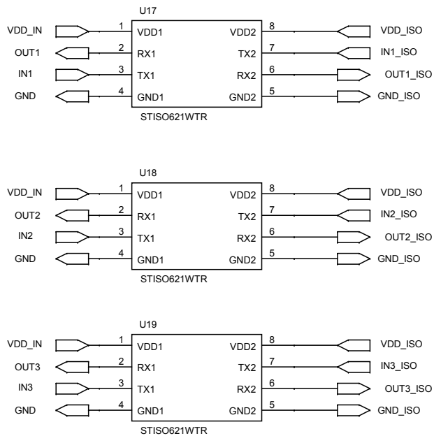
Figure 17. STEVAL-SILKTA01 circuit schematic (17 of 21)
