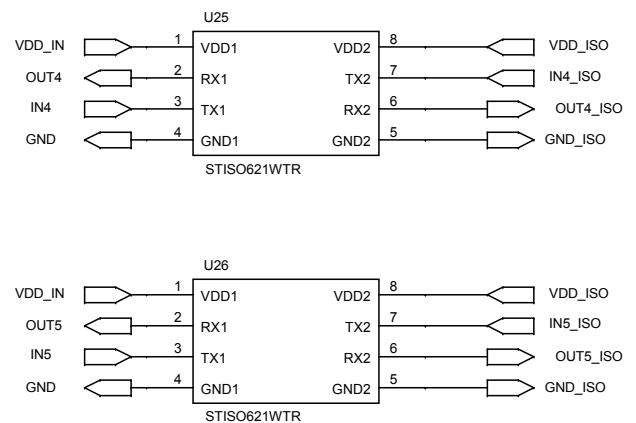
Figure 17. STEVAL-SILKTA01 circuit schematic (17 of 21)
