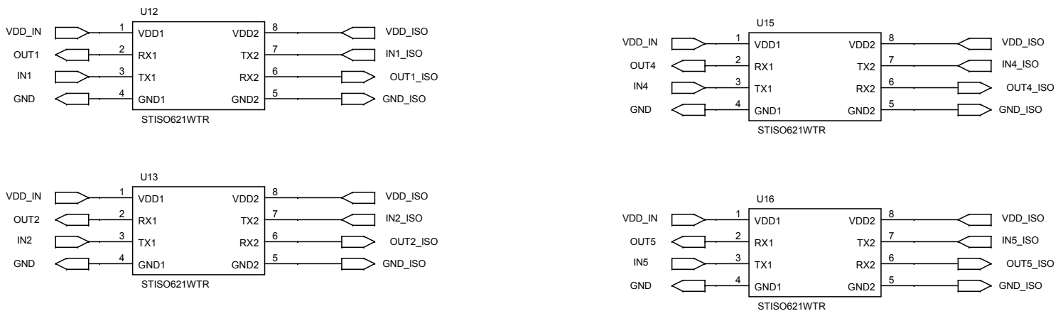
Figure 15. STEVAL-SILKTA01 circuit schematic (15 of 21)
