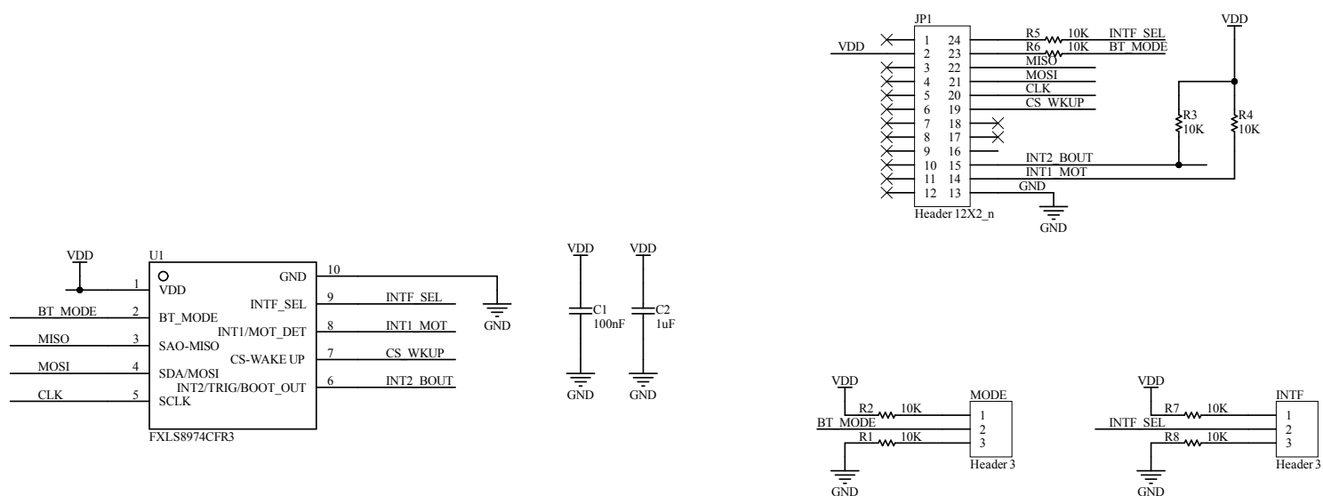
Figure 1. STEVAL-MKI265A schematic
