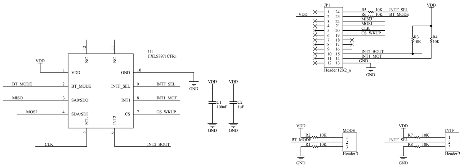
Figure 1. STEVAL-MKI264A schematic
