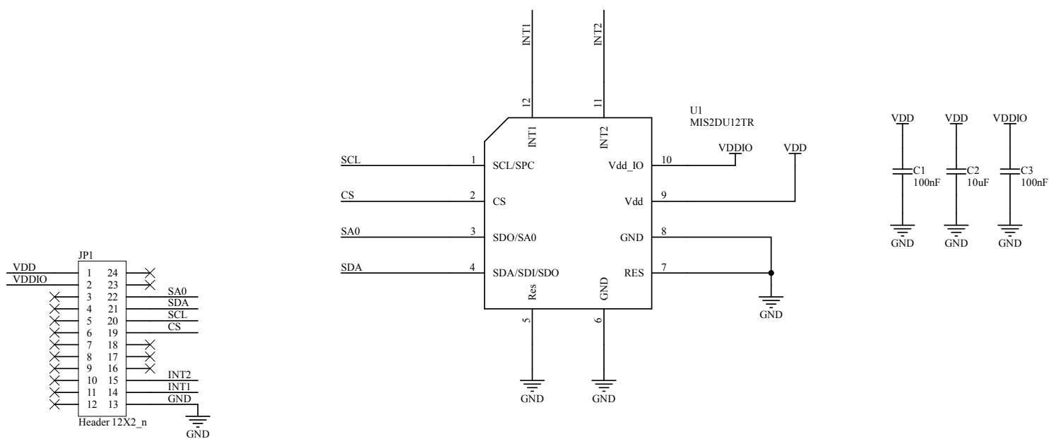
Figure 1. STEVAL-MKI255A schematic
