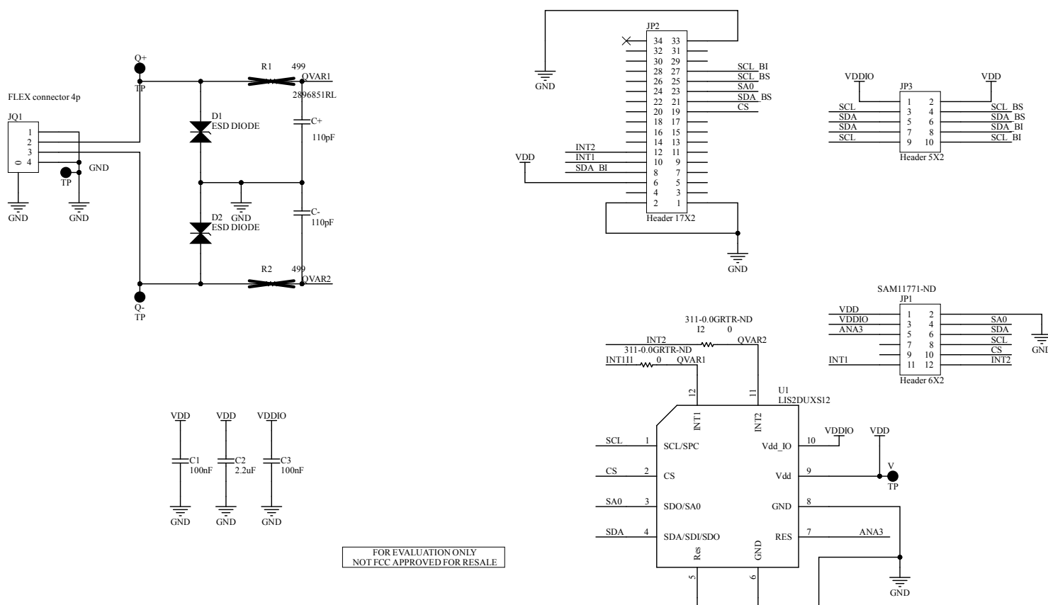
Figure 2. STEVAL-MKI246A schematic
