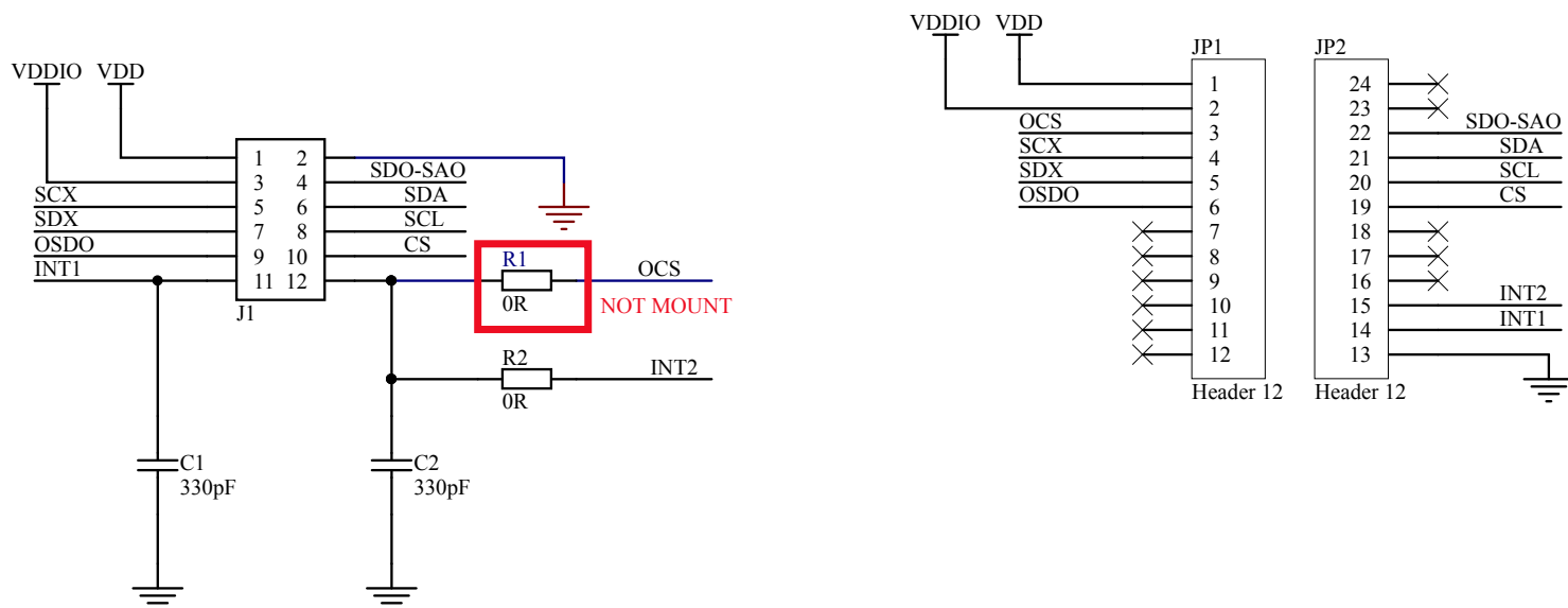
Figure 1. STEVAL-MKIGIBV5 schematic
