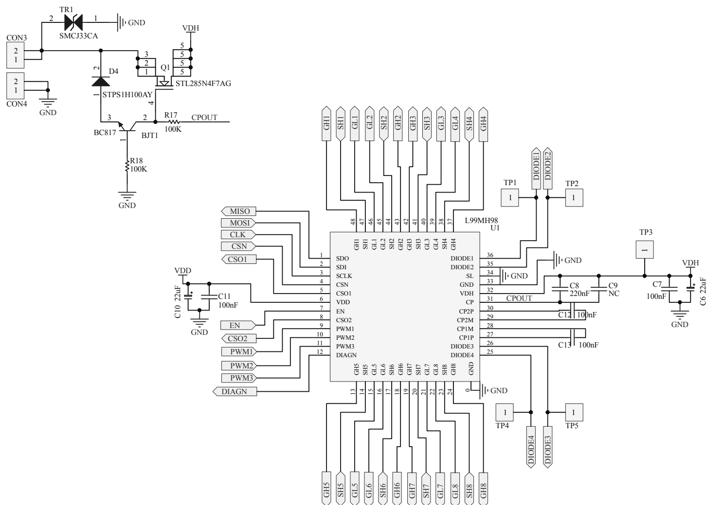
Figure 1. STEVAL-L99MH98 schematic diagram - [1 of 3]
