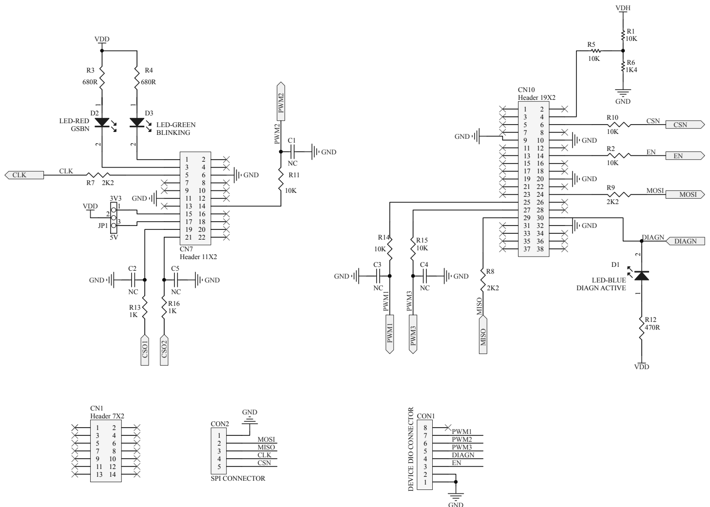
Figure 2. STEVAL-L99MH98 schematic diagram - [2 of 3]
