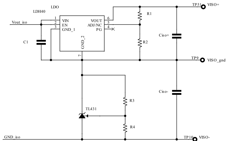
Figure 2. STEVAL-L6983IV1 circuit schematic (2 of 2) - post regulation (not mounted, bottom side)
