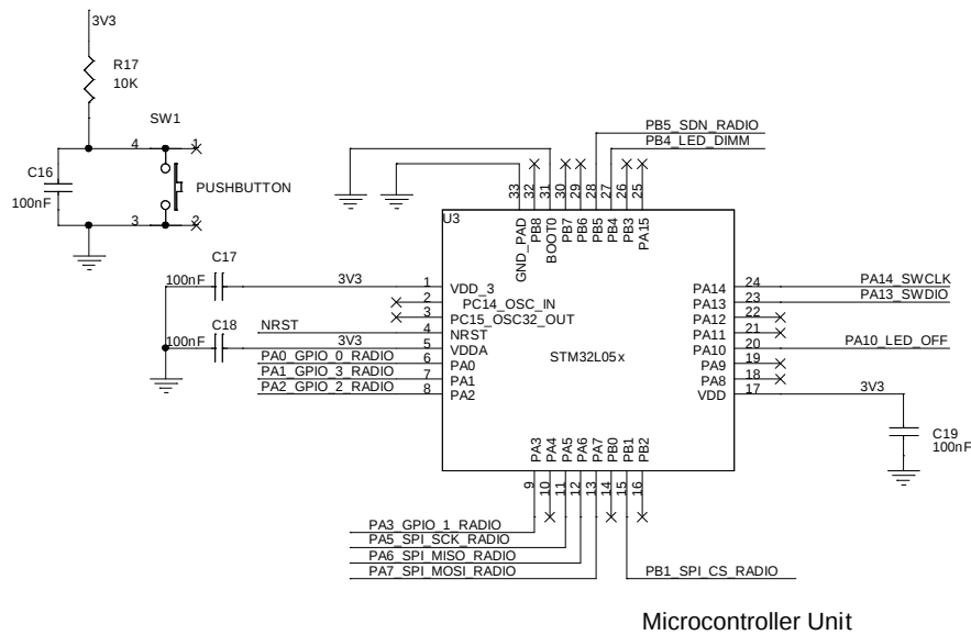
Figure 1: STEVAL-ILL083V1 circuit schematic (1 of 3)
