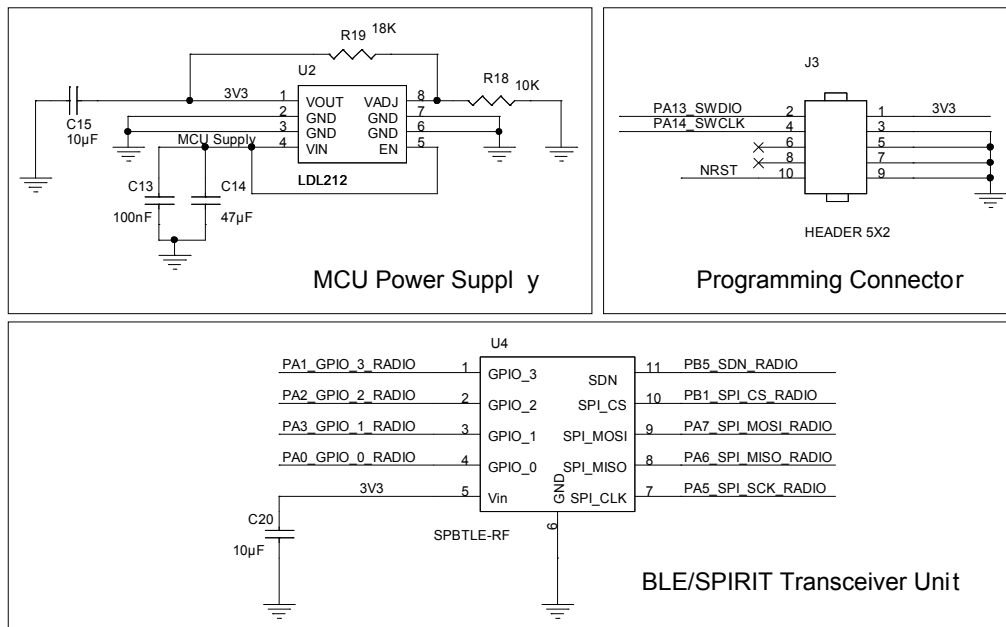
Figure 2: STEVAL-ILL083V1 circuit schematic (2 of 3)
