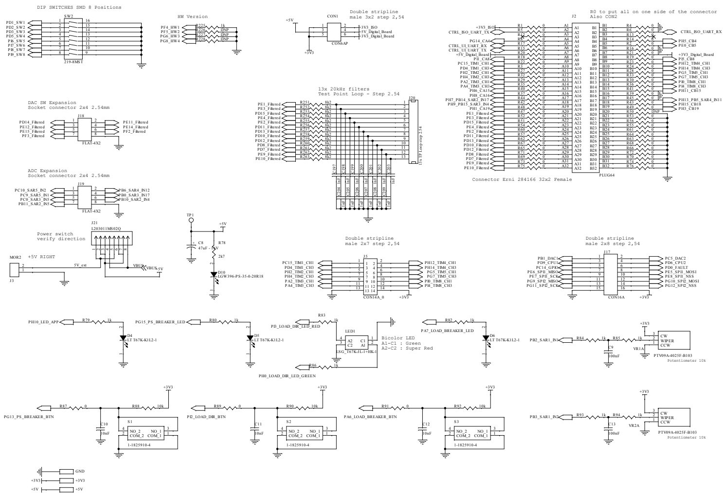
Figure 1. STEVAL-HILE1V1 - HIL board circuit schematic (1 of 6)
