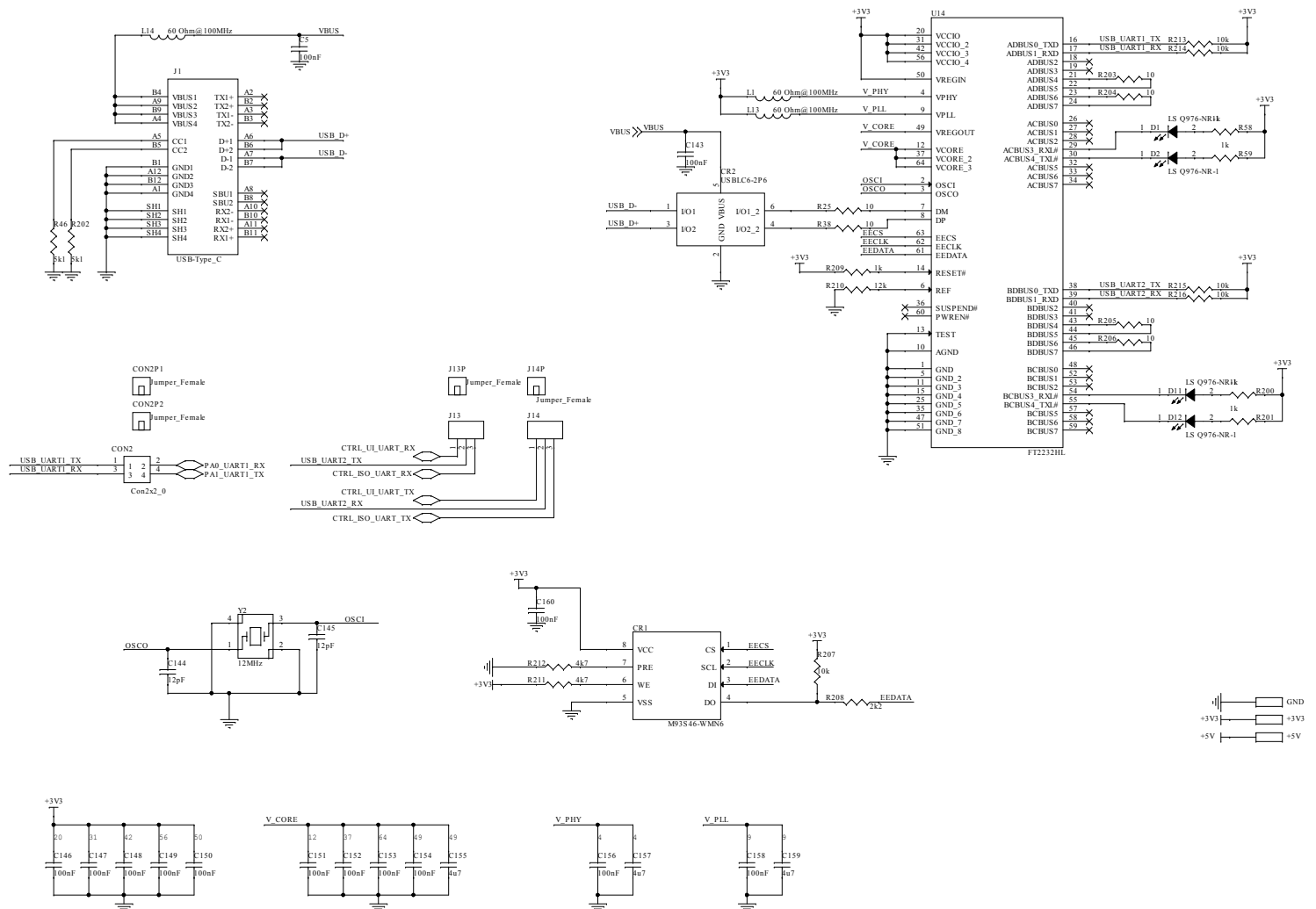
Figure 2. STEVAL-HILE1V1 - HIL board circuit schematic (2 of 6)
