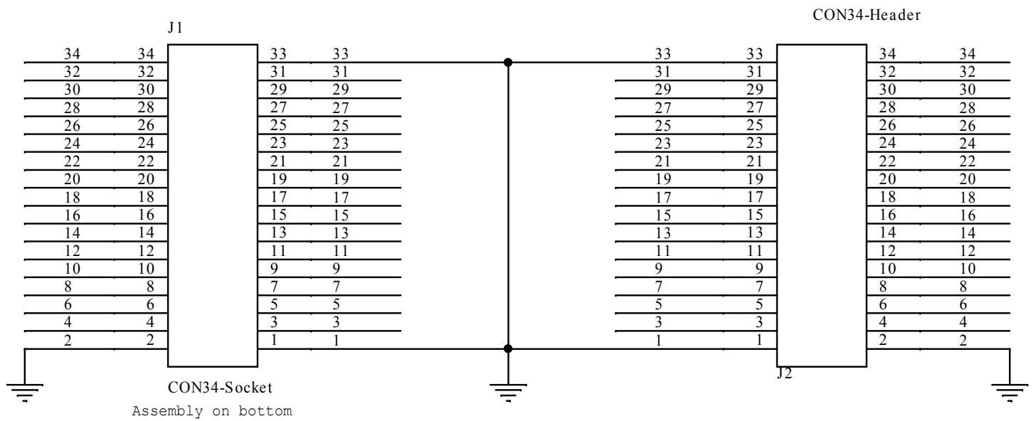
Figure 2. STEVAL-FLTCB05 circuit schematic
