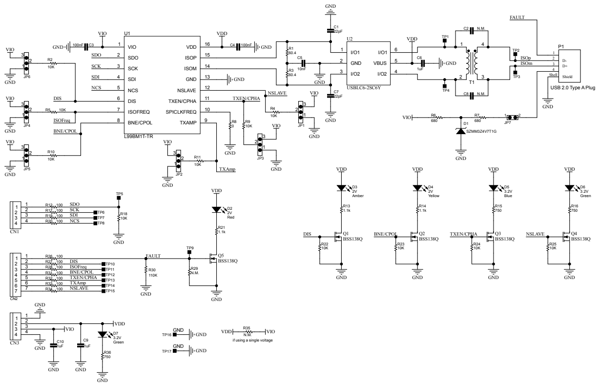
Figure 1. STEVAL-BMS1T circuit schematic
