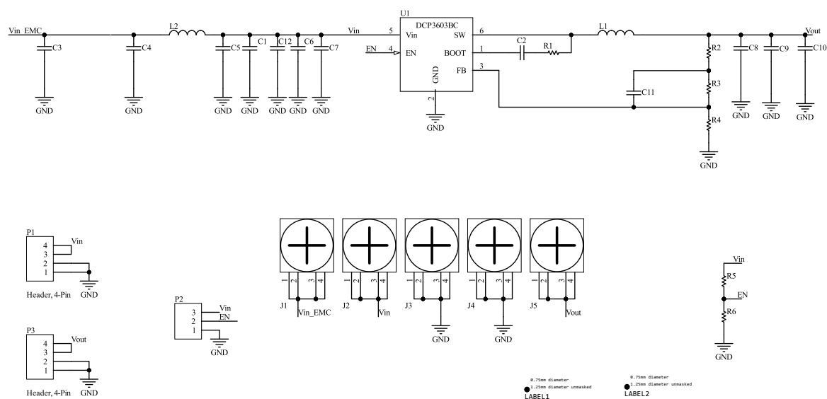
Figure 1. STEVAL-3603BC1 circuit schematic
