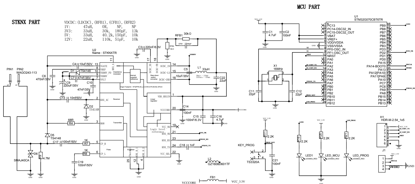
Figure 1. STDES-HARMONYKNX circuit schematic
