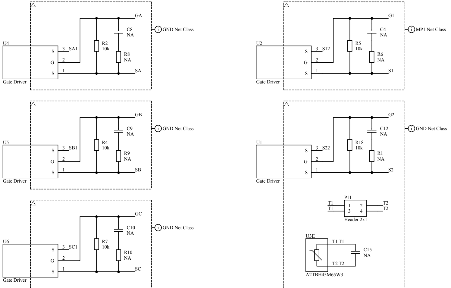
Figure 4. STDES-A2TBH45M65 synchronous iso-buck circuit schematic
