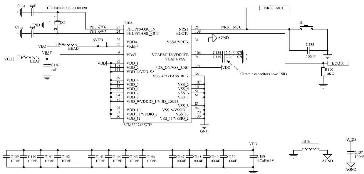
Figure 2. STDES-8PIOLM4P circuit schematic (2 of 12)
