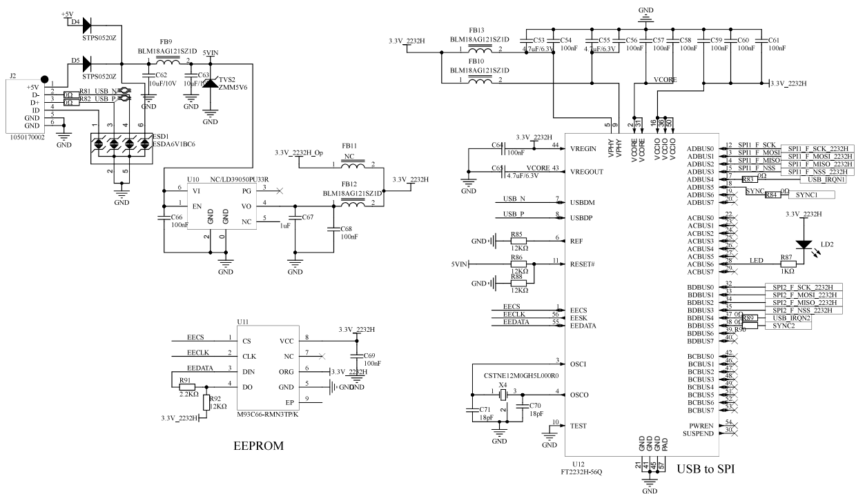
Figure 6. STDES-8PIOLM4P circuit schematic (6 of 12)
