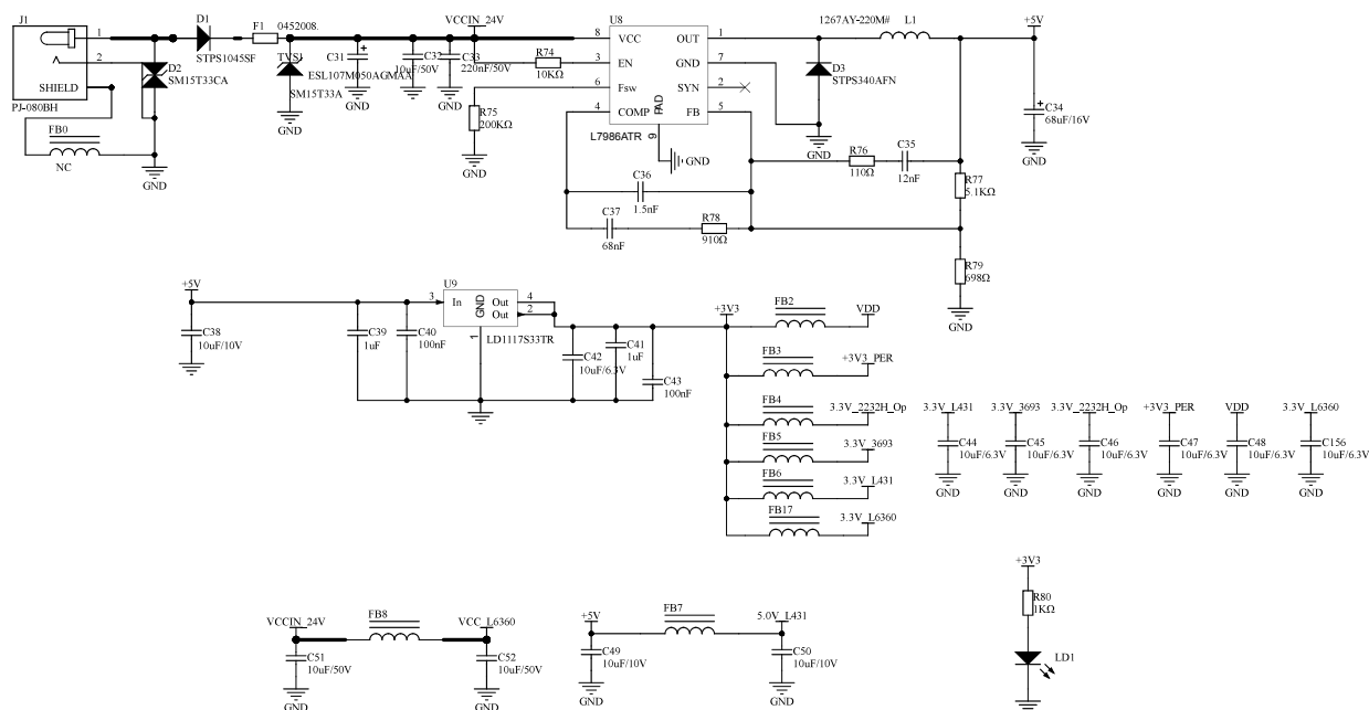
Figure 2. STDES-8PIOLM4P circuit schematic (2 of 12)
