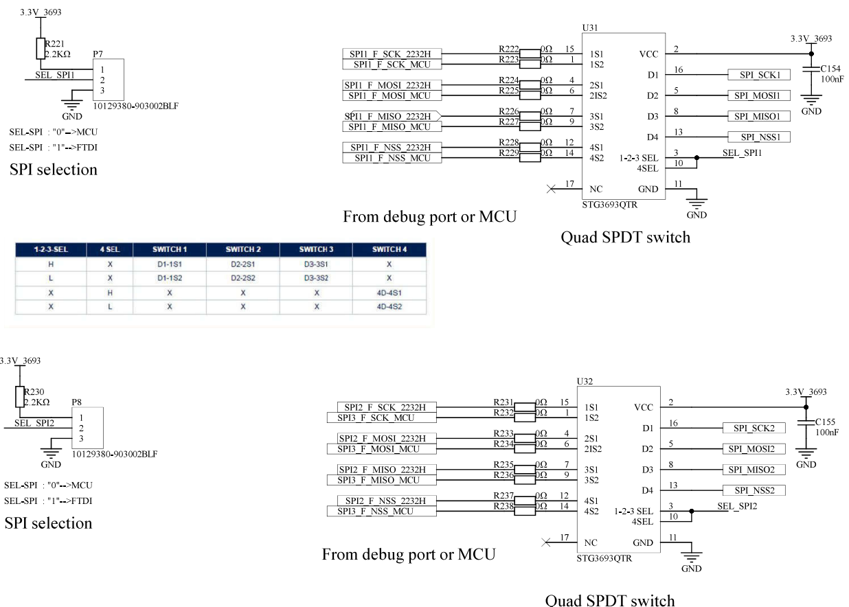
Figure 6. STDES-8PIOLM4P circuit schematic (6 of 12)
