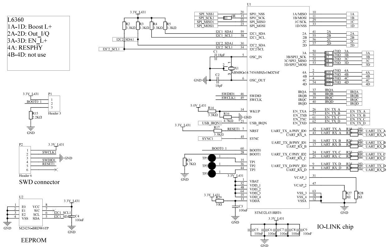
Figure 7. STDES-8PIOLM4P circuit schematic (7 of 12)
