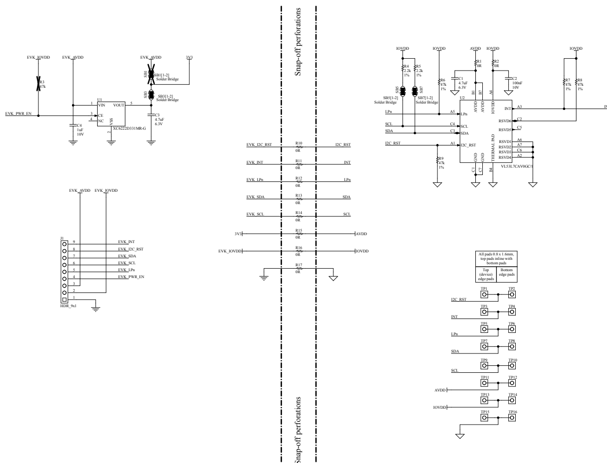
Figure 1. SATEL-VL53L7 circuit schematic
