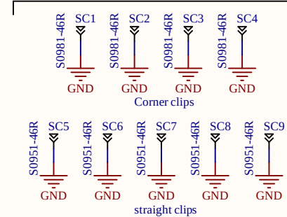
Socket for Metallic Shield
