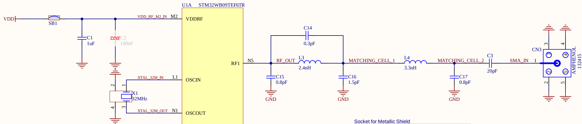
Socket for Metallic Shield
