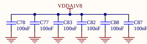
Level shifter VDDA1V8 voltage decoupling capacitors
