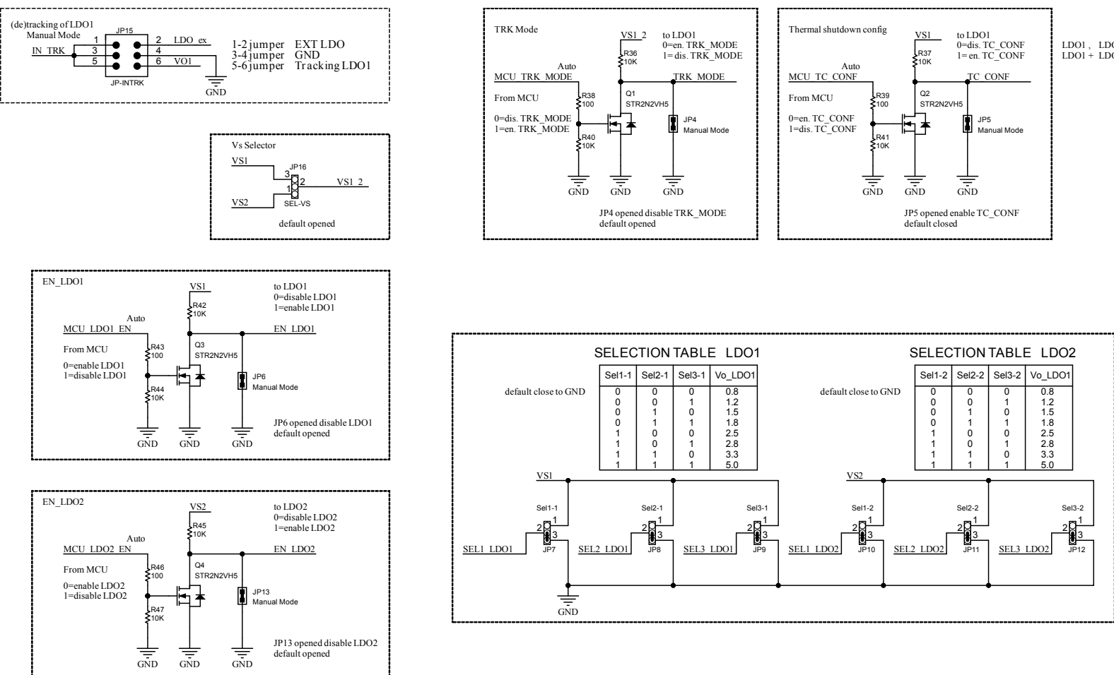
Figure 3. AEK-POW-LDOV02X circuit schematic (3 of 3)
