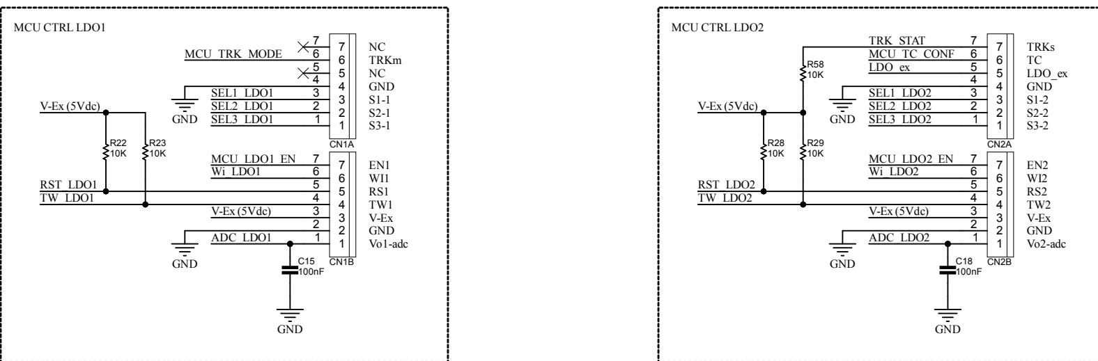
Figure 2. AEK-POW-LDOV02X circuit schematic (2 of 3)
