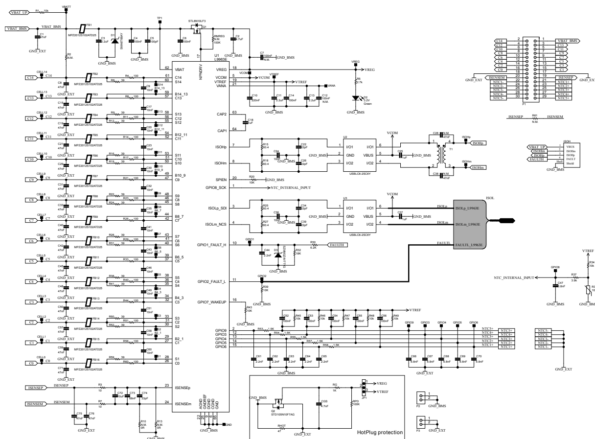
Figure 1. AEK-POW-BMSWTX circuit schematic (1 of 2)
