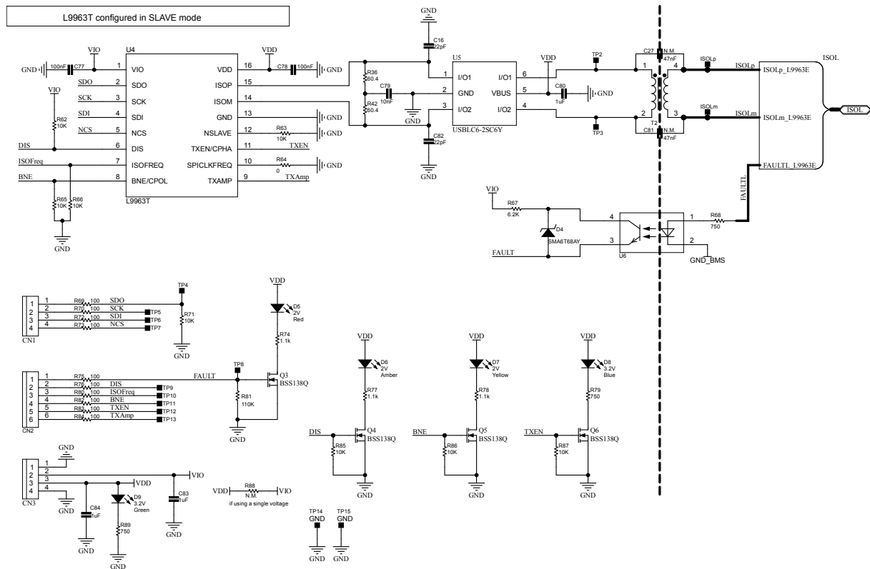
Figure 2. AEK-POW-BMSWTX circuit schematic (2 of 2)
