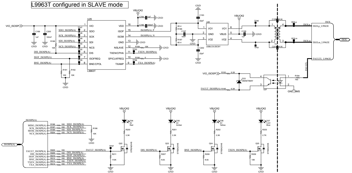
Figure 9. AEK-POW-BMS63EM schematic diagrams (9 of 12)
