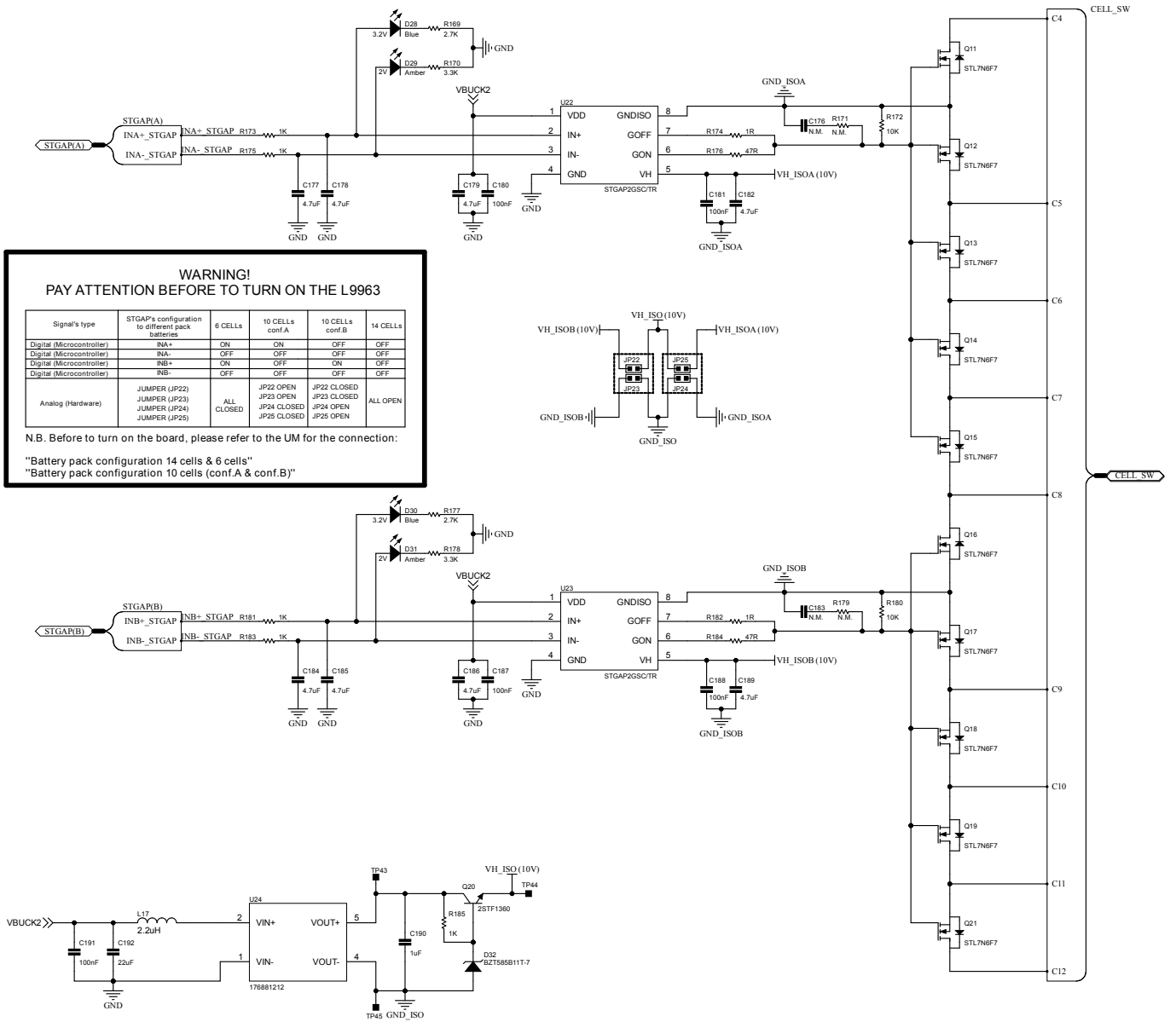
Figure 8. AEK-POW-BMS63EM schematic diagrams (8 of 12)
