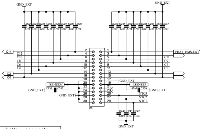
Figure 12. AEK-POW-BMS63EM schematic diagrams (12 of 12)
