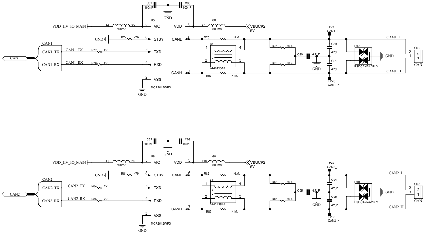
Figure 5. AEK-POW-BMS63EM schematic diagrams (5 of 12)
