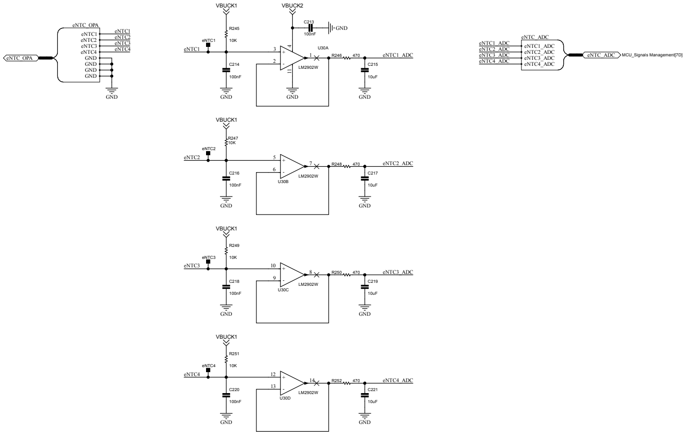
Figure 11. AEK-POW-BMS63EM schematic diagrams (11 of 12)
