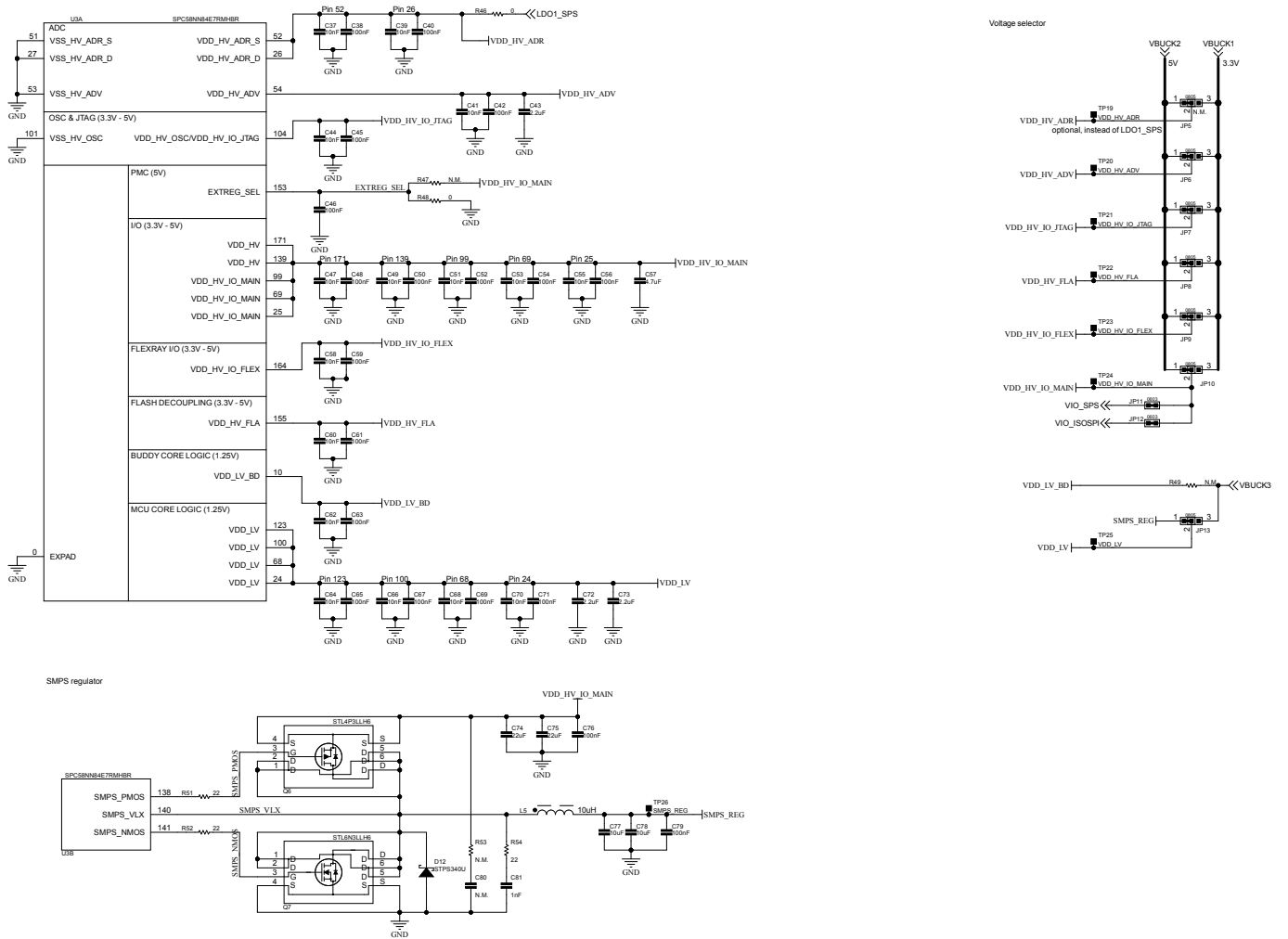
Figure 2. AEK-POW-BMS63EM schematic diagrams (2 of 12)
