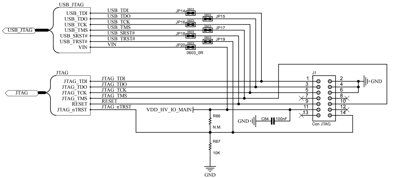
Figure 4. AEK-POW-BMS63EM schematic diagrams (4 of 12)
