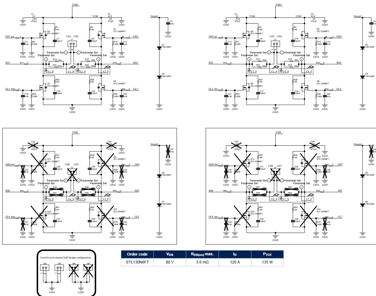
Figure 2. AEK-MOT-4DCMH94 circuit schematic (2 of 4)
