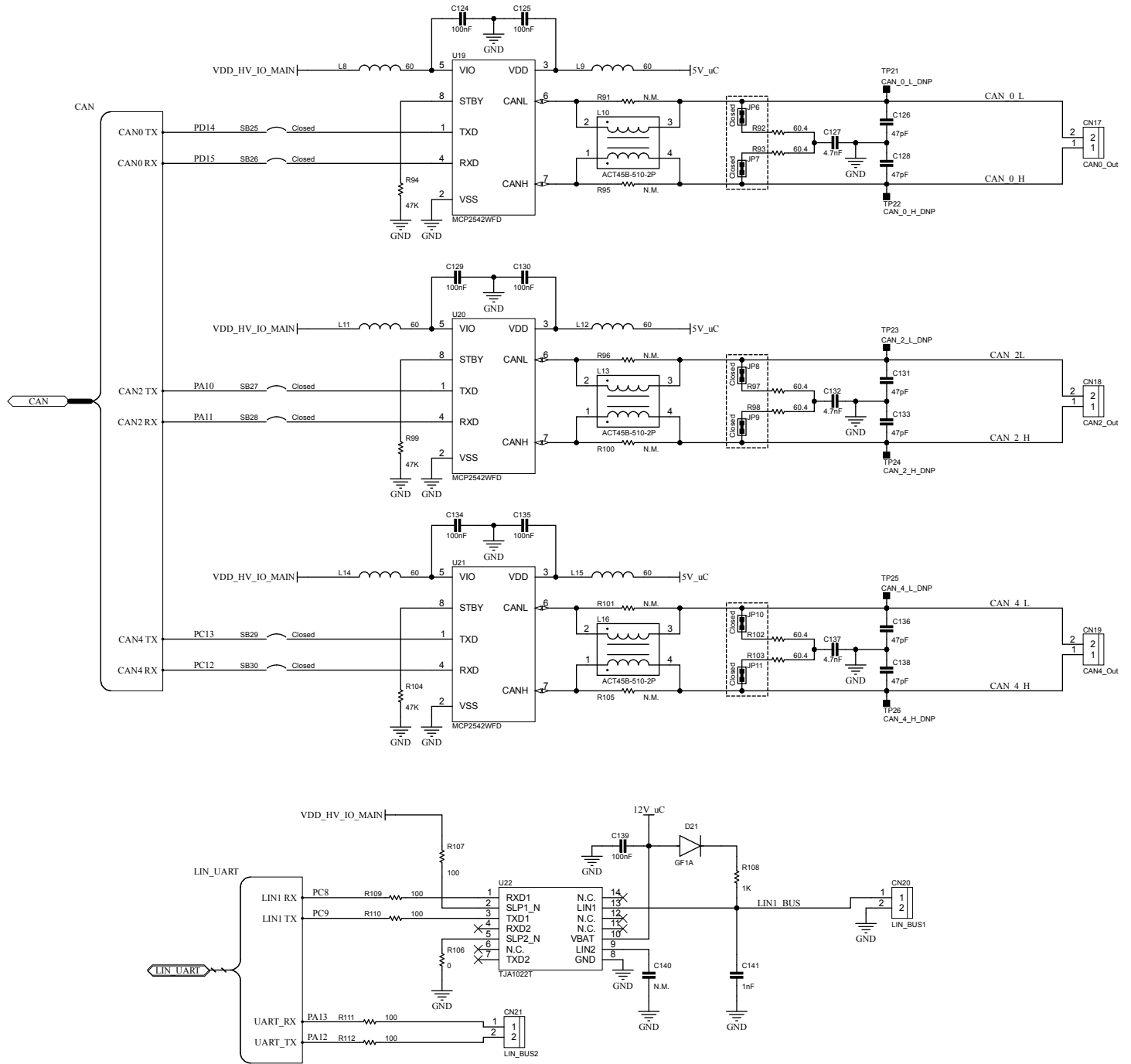
Figure 8. AEK-MCU-C4MINI1 circuit schematic (8 of 12)
