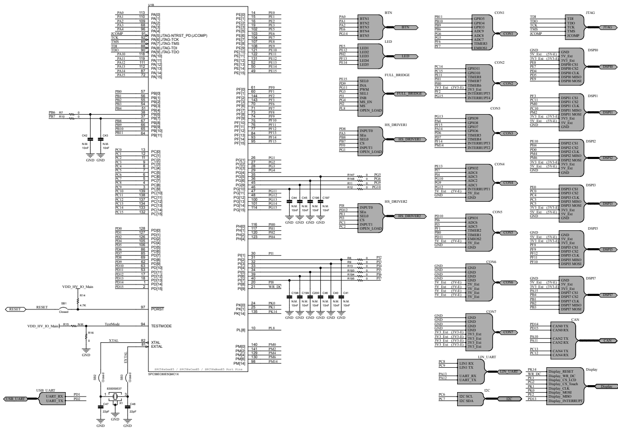
Figure 4. AEK-MCU-C4MINI1 circuit schematic (4 of 12)
