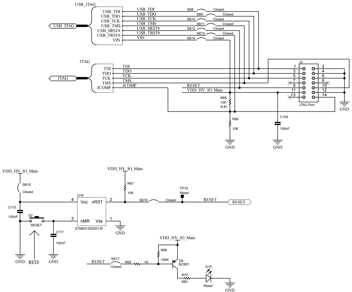
Figure 6. AEK-MCU-C4MINI1 circuit schematic (6 of 12)
