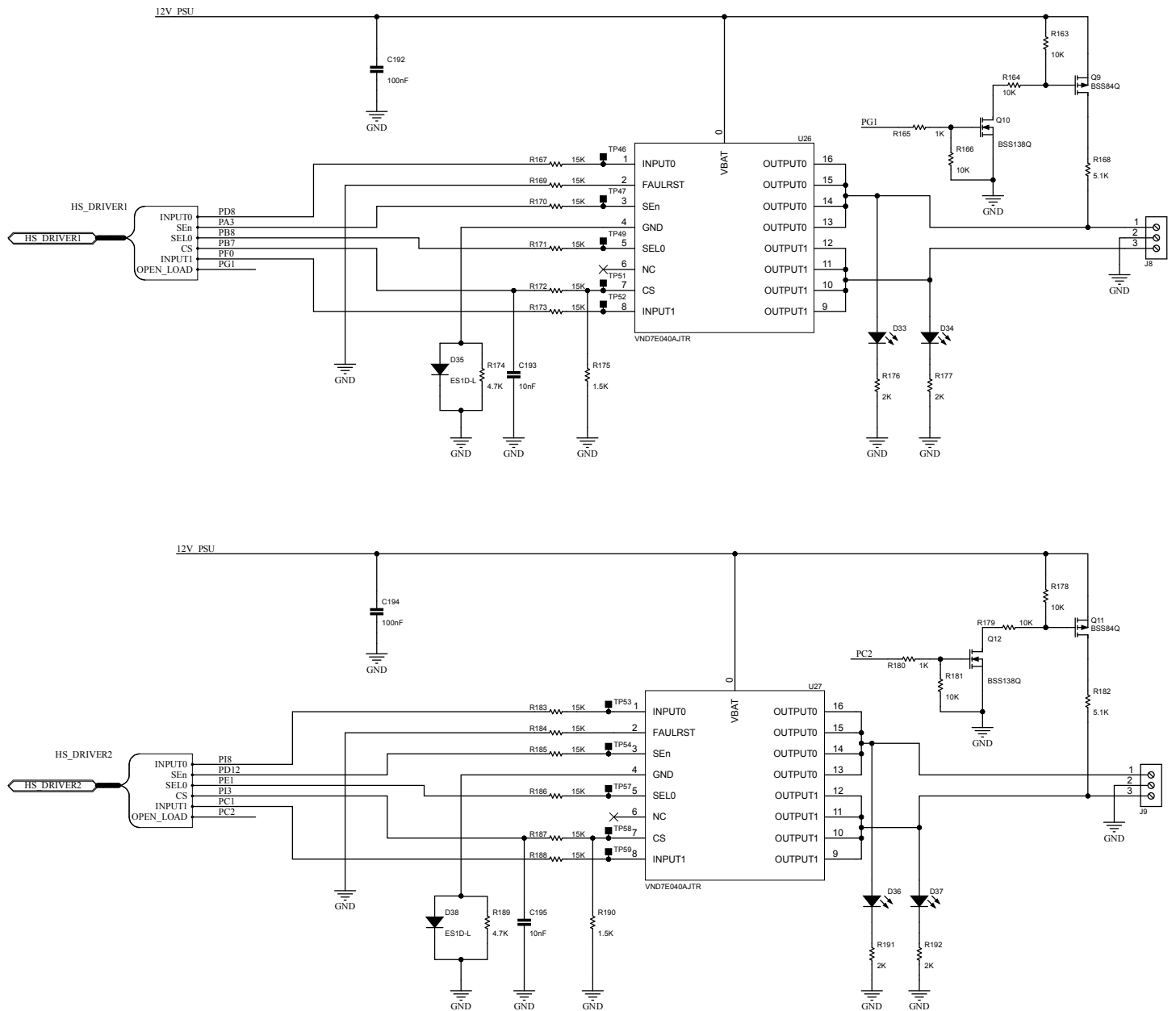
Figure 11. AEK-MCU-C4MINI1 circuit schematic (11 of 12)
