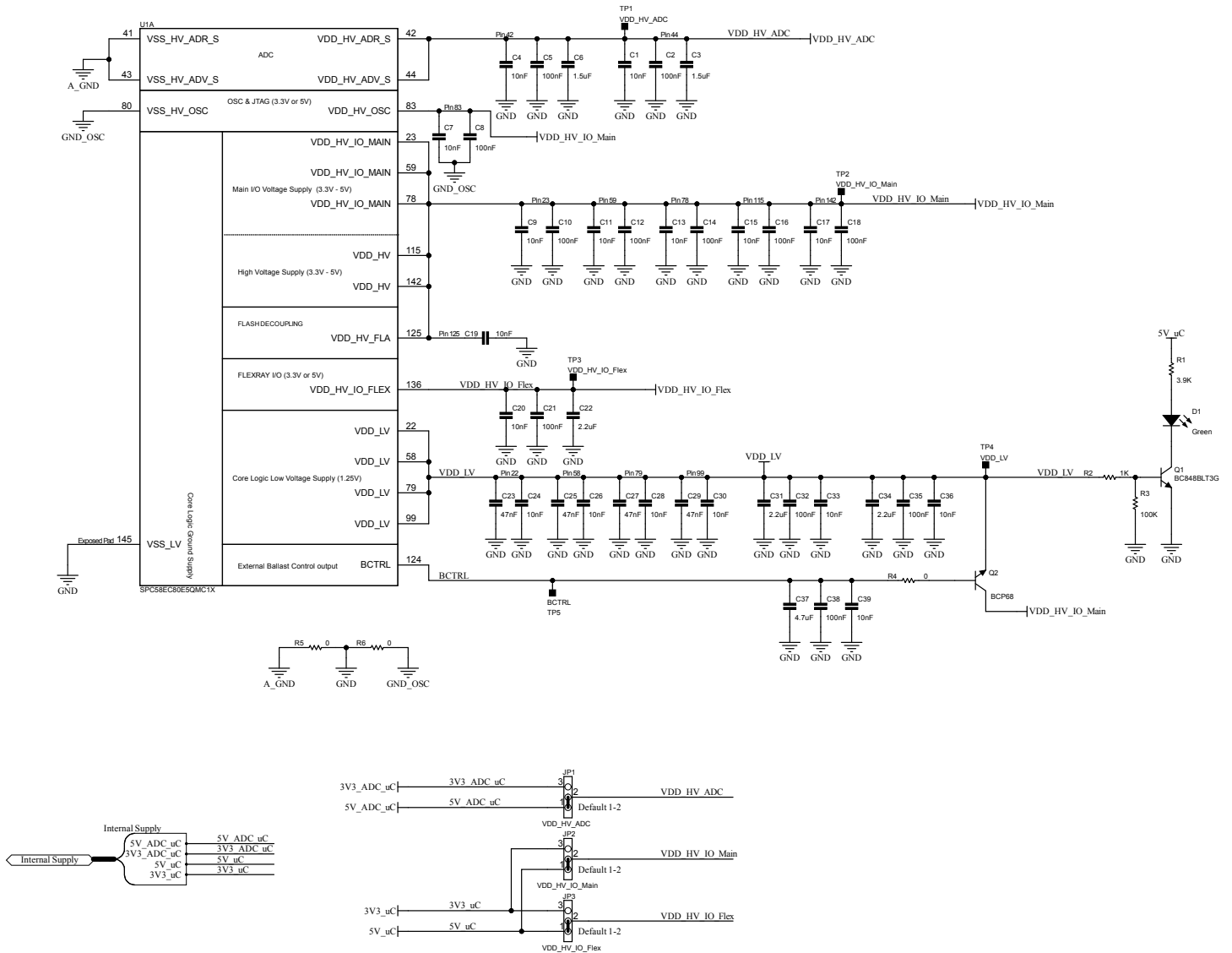
Figure 3. AEK-MCU-C4MINI1 circuit schematic (3 of 12)
