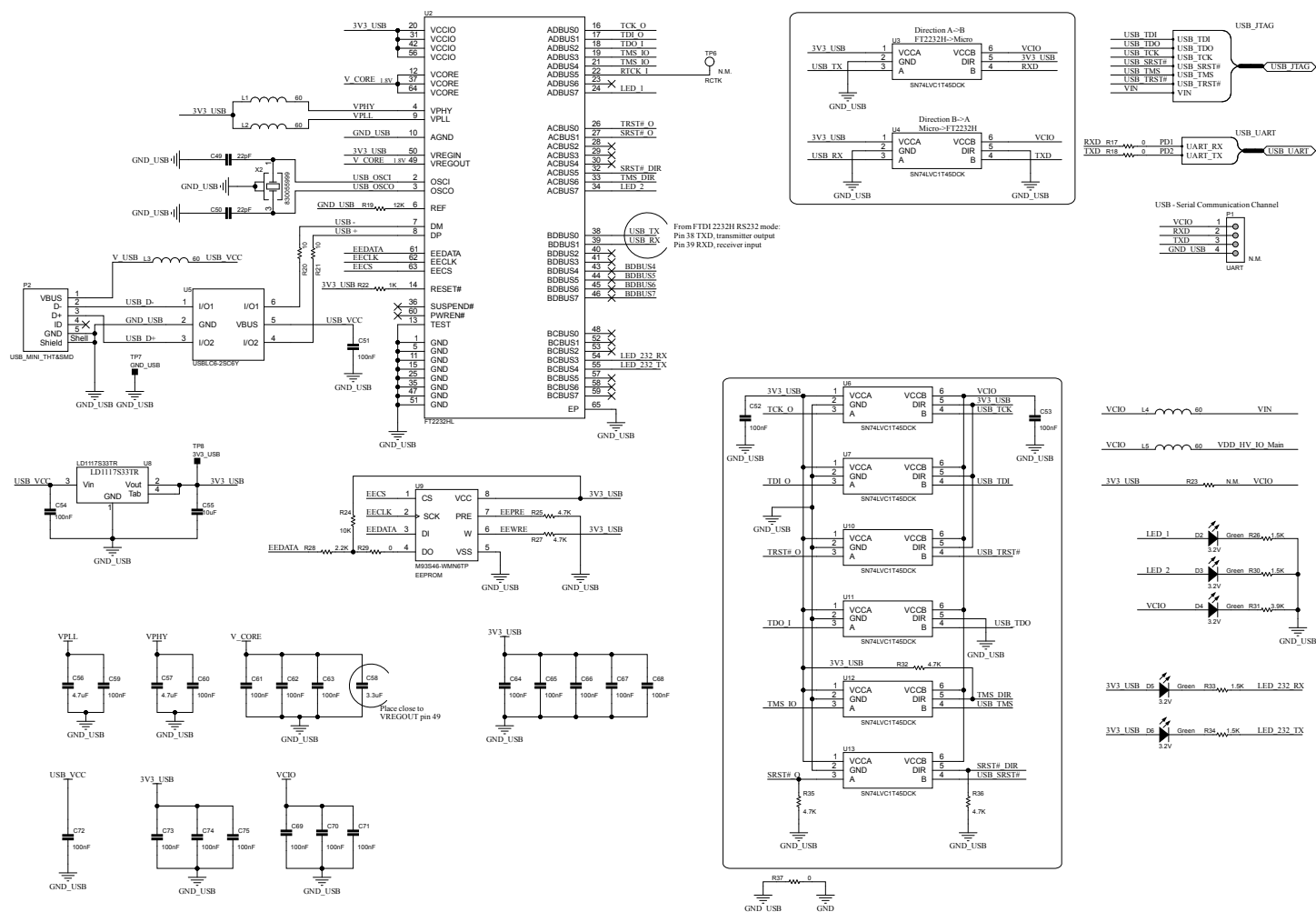
Figure 5. AEK-MCU-C4MINI1 circuit schematic (5 of 12)
