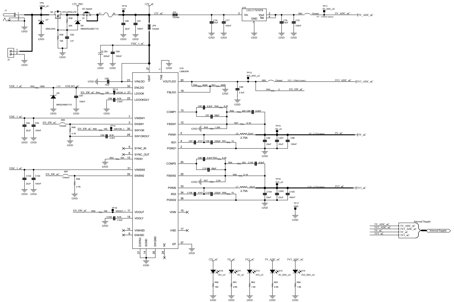
Figure 2. AEK-MCU-C4MINI1 circuit schematic (2 of 12)
