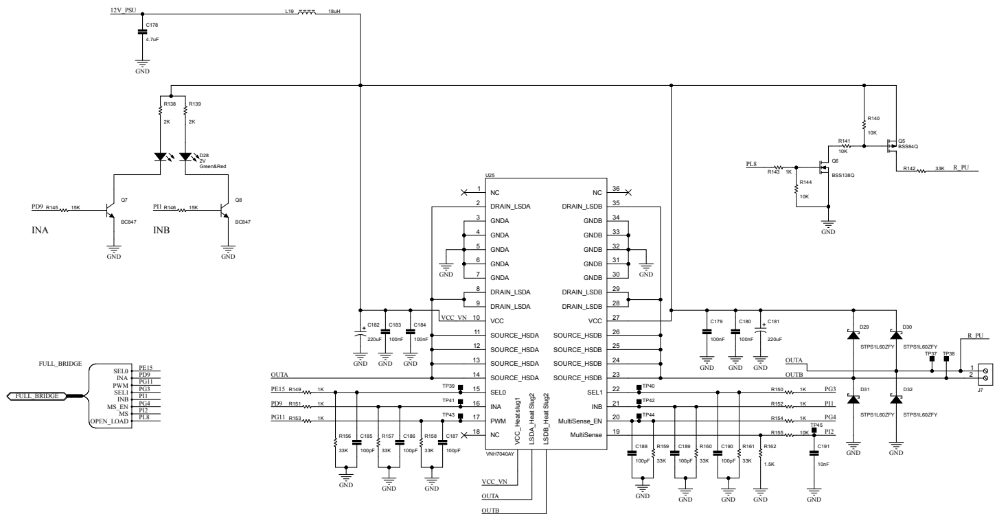
Figure 10. AEK-MCU-C4MINI1 circuit schematic (10 of 12)
