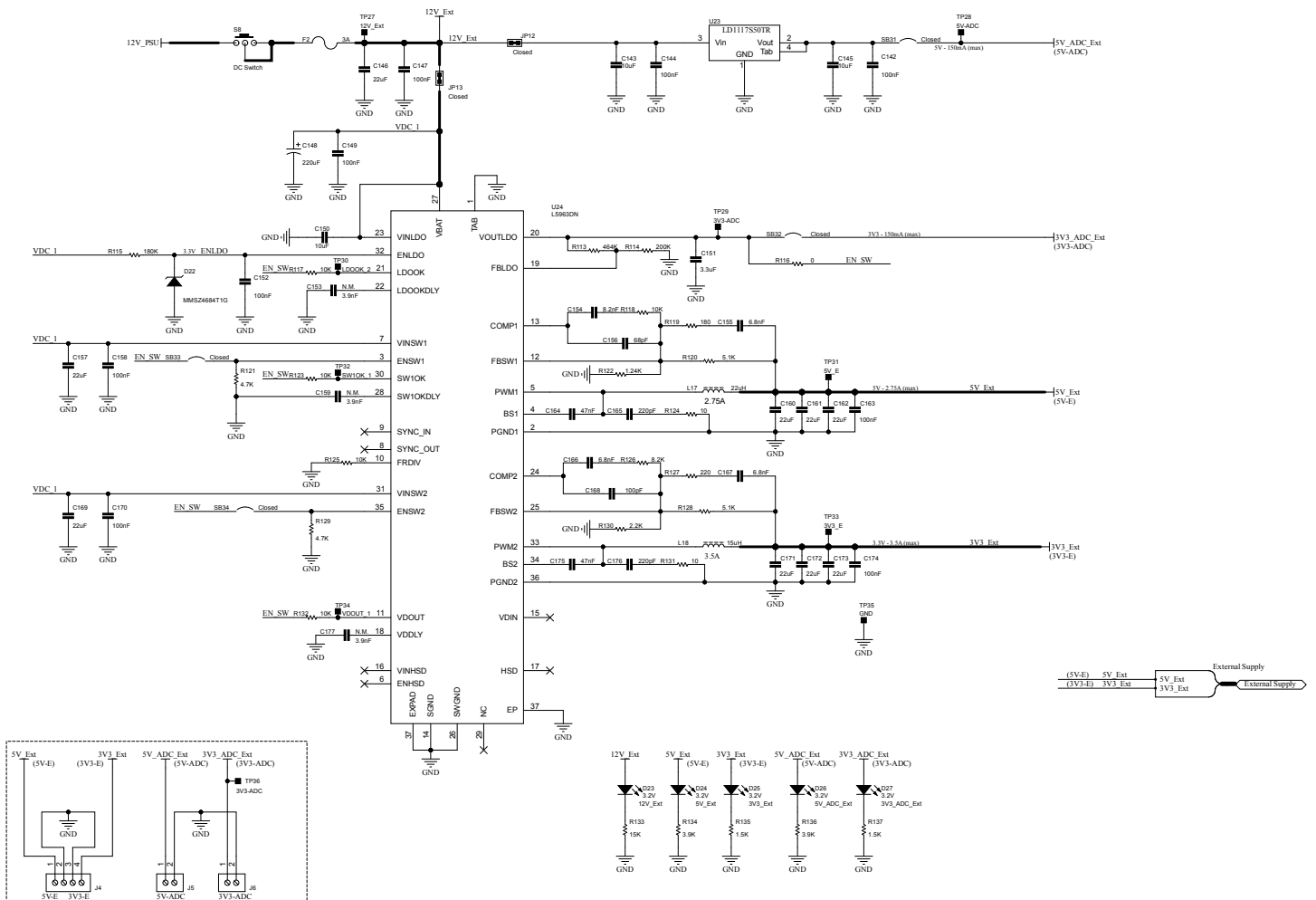
Figure 9. AEK-MCU-C4MINI1 circuit schematic (9 of 12)
