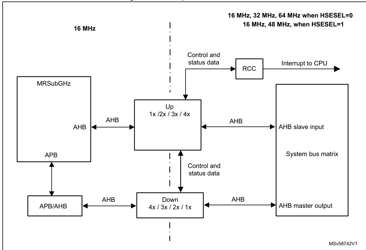
Figure 3. AHB up/down converter
