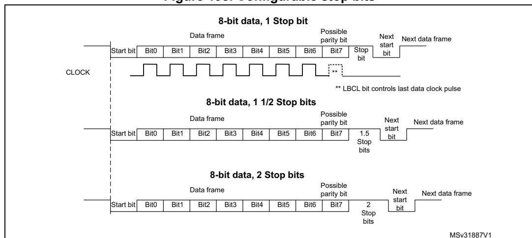
Figure 198. Configurable stop bits
