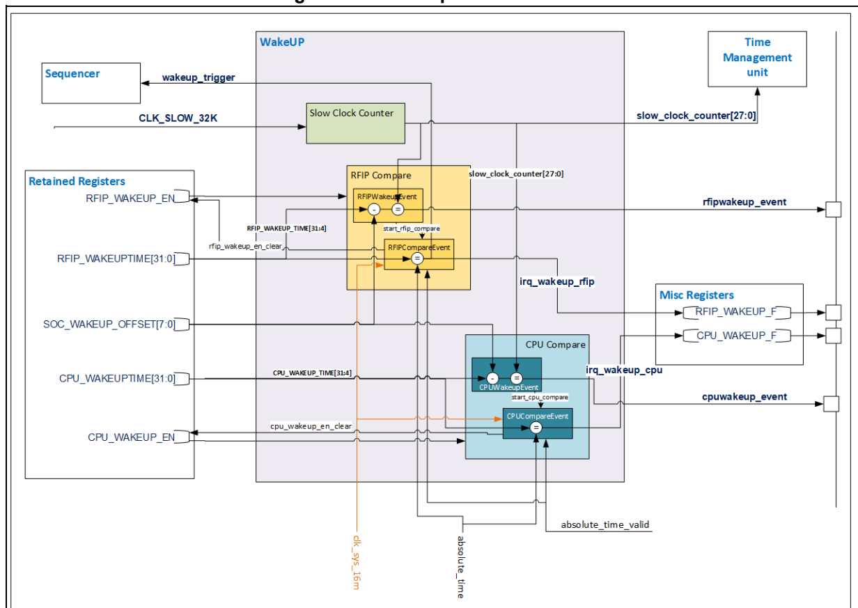
Figure 271. Wakeup block overview
