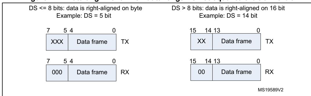
Figure 214. Data alignment when data length is not equal to 8-bit or 16-bit
