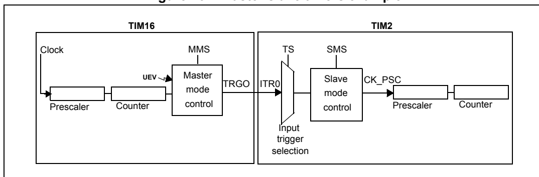
Figure 134. Master/slave timers example
