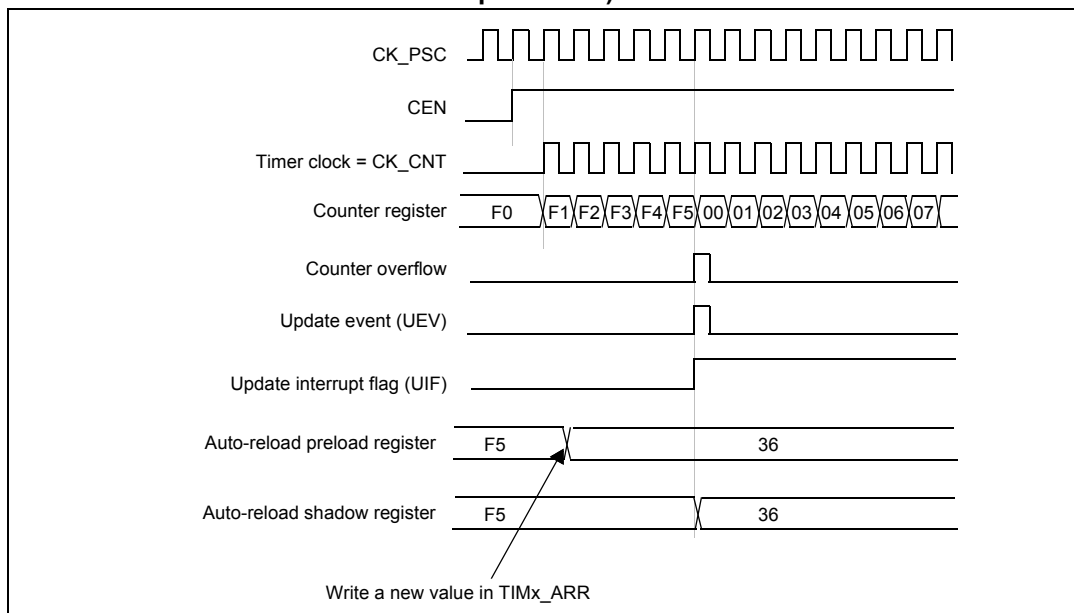
Figure 62. Counter timing diagram, update event when ARPE=1 (TIMx_ARR preloaded)
