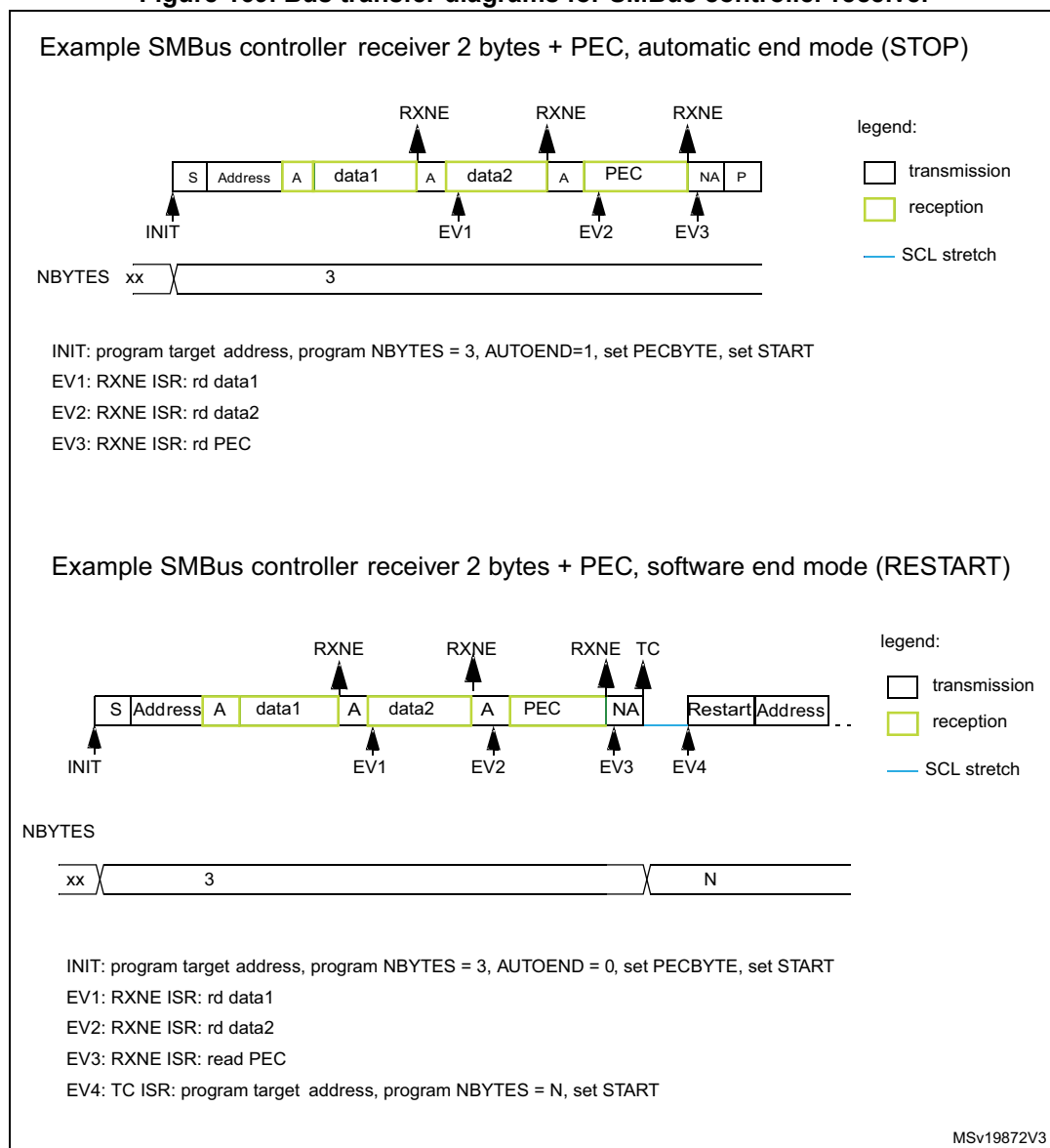
Figure 169. Bus transfer diagrams for SMBus controller receiver
