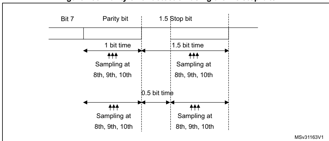
Figure 188. Parity error detection using the 1.5 stop bits
