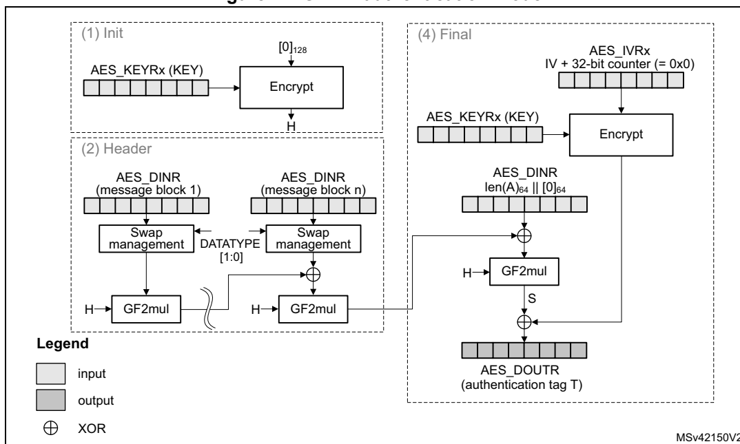
Figure 47. GMAC authentication mode
