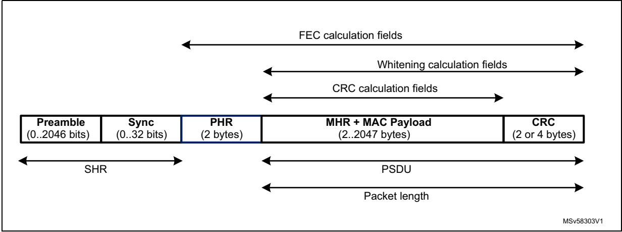
Figure 244. 802.15.4 packet format
