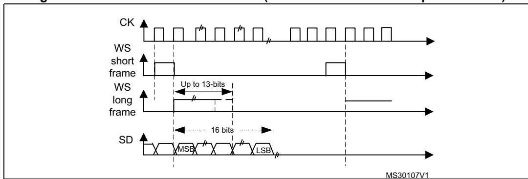
Figure 239. PCM standard waveforms (16-bit extended to 32-bit packet frame)
