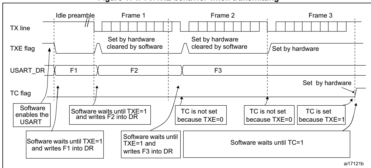
Figure 174. TC/TXE behavior when transmitting
