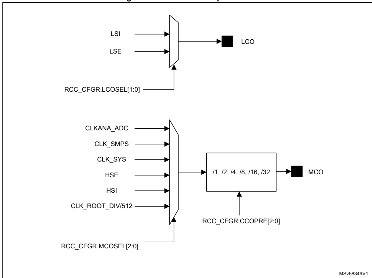
Figure 15. LCO / MCO output clocks
