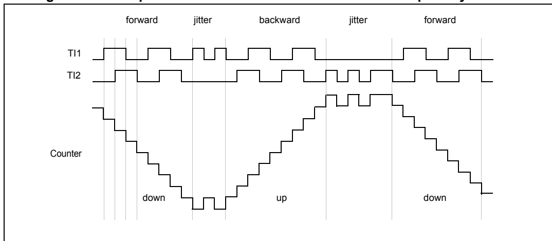
Figure 95. Example of encoder interface mode with TI1FP1 polarity inverted.
