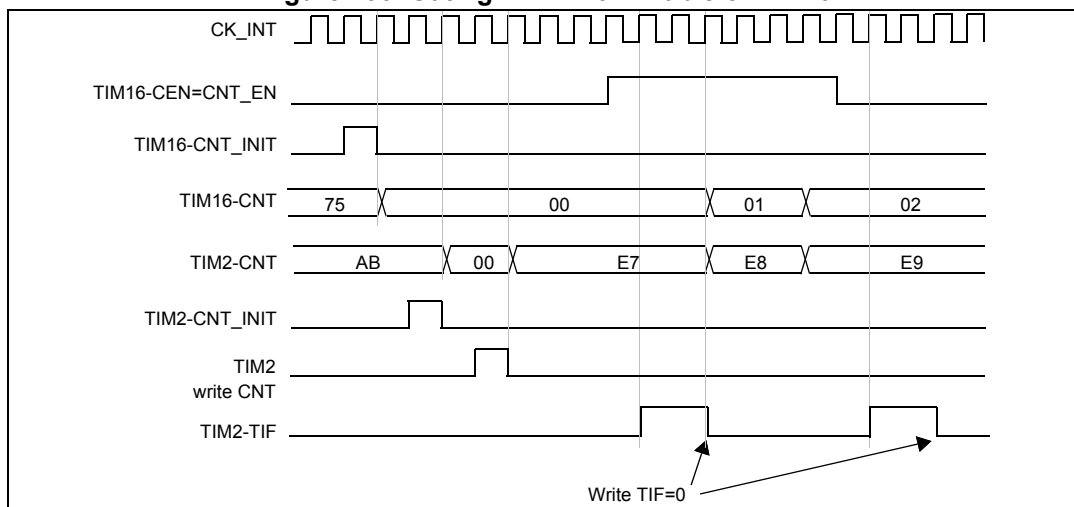
Figure 136. Gating TIM2 with Enable of TIM16
