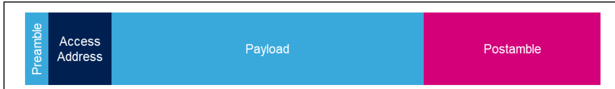
Figure 259. W-MBUS frame format
