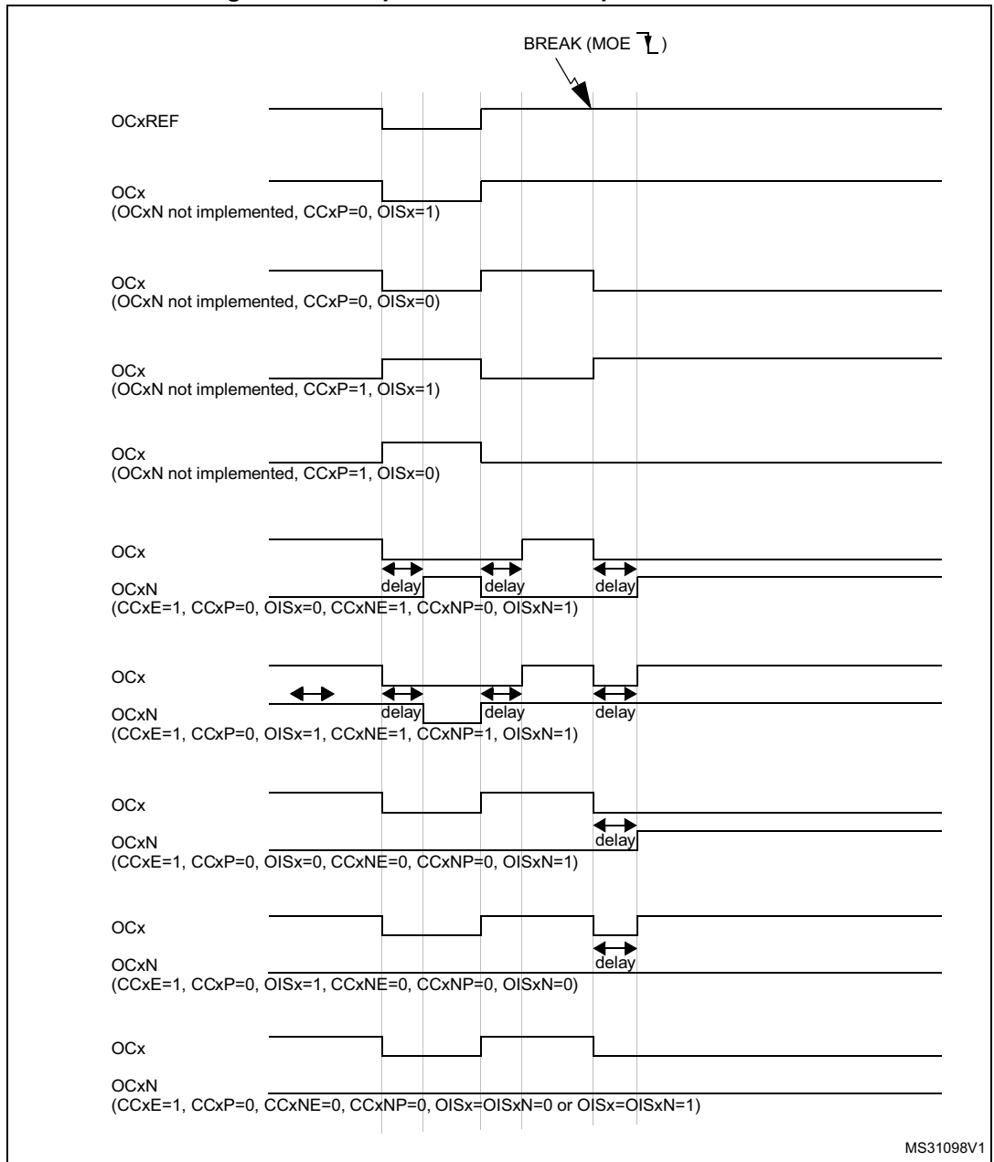
Figure 127. Output behavior in response to a break
