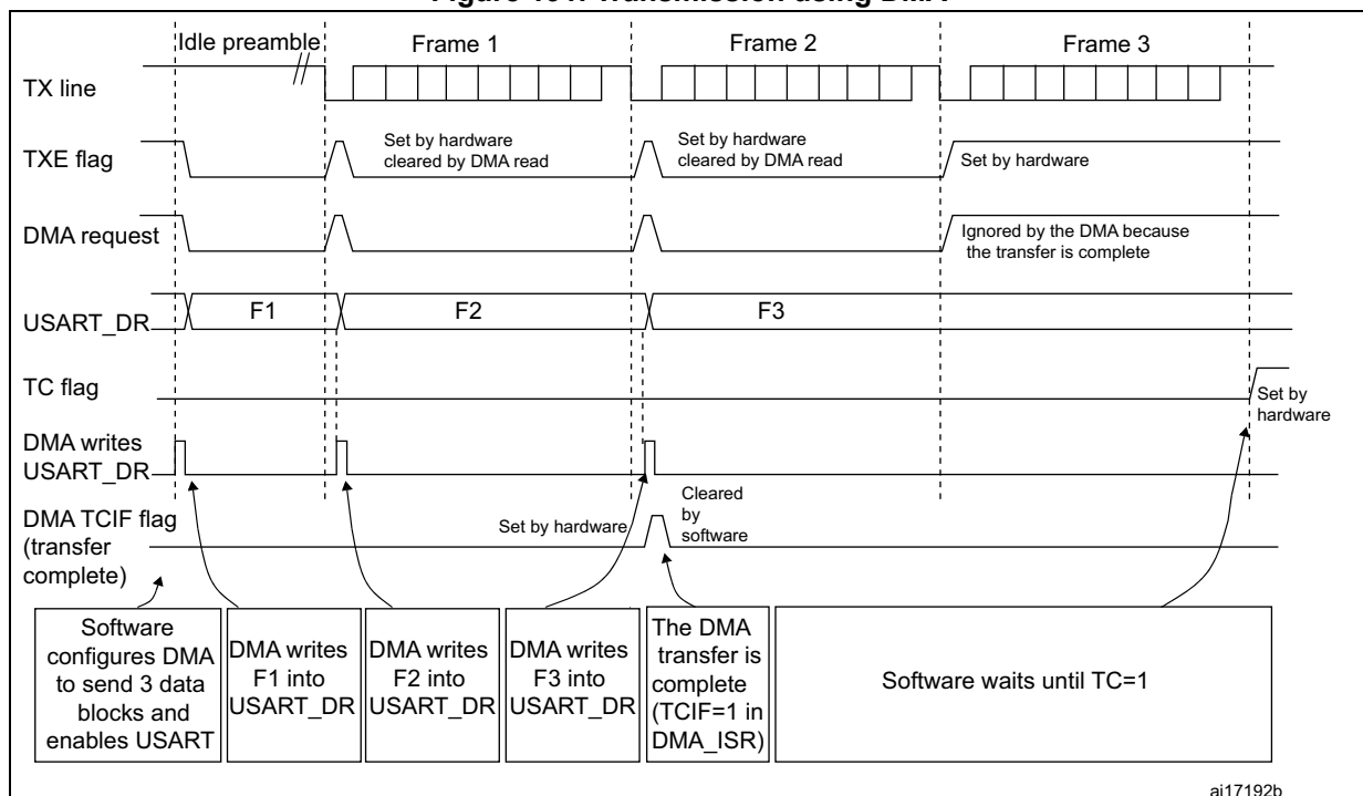
Figure 191. Transmission using DMA
