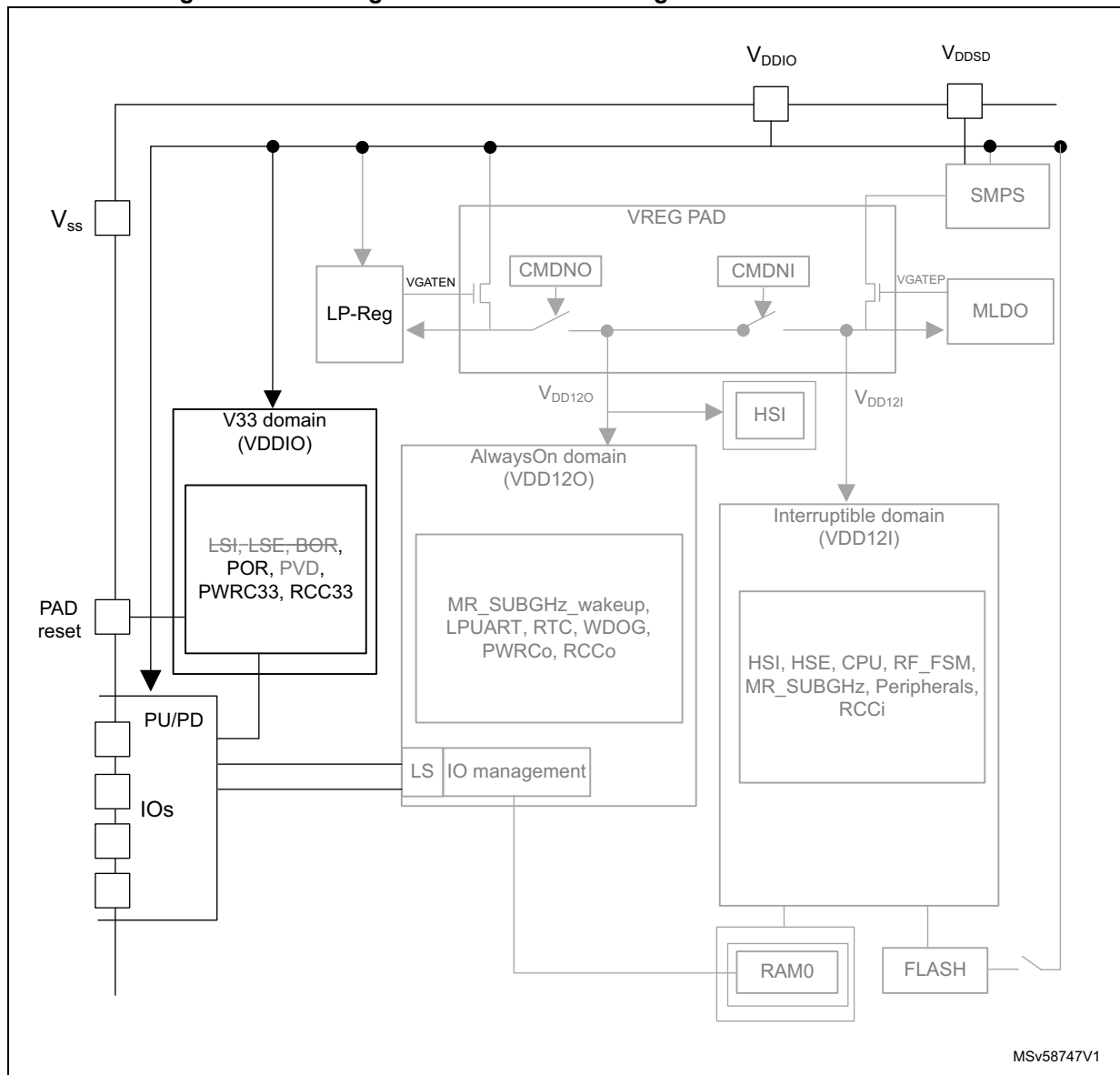
Figure 9. Power regulators and SMPS configuration in Shutdown mode
