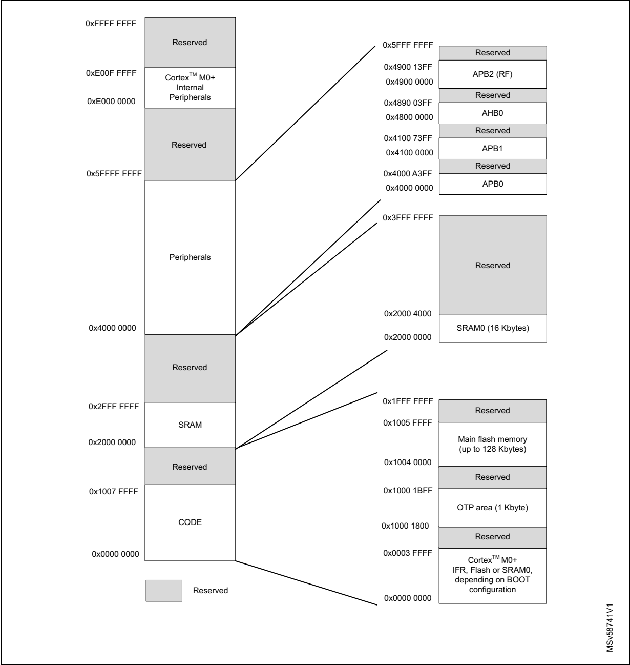
Figure 2. Memory map
