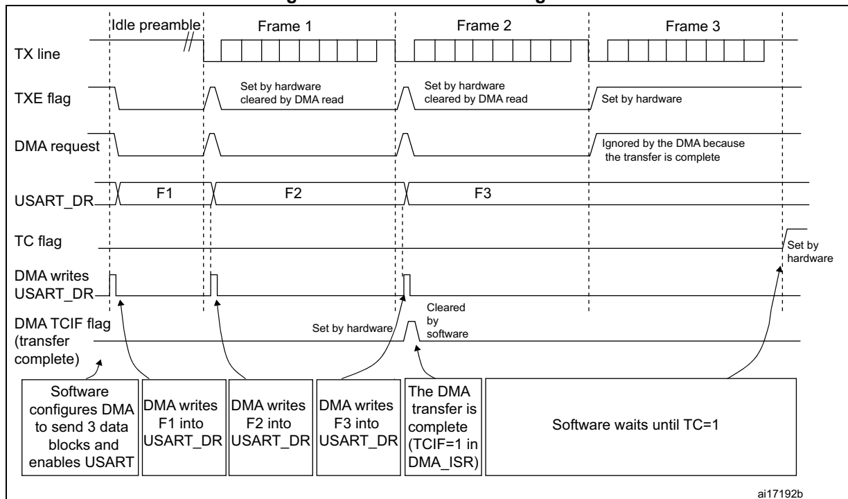
Figure 202. Transmission using DMA
