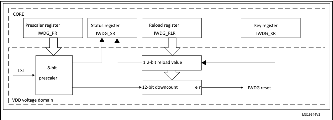
Figure 140. Independent watchdog block diagram
