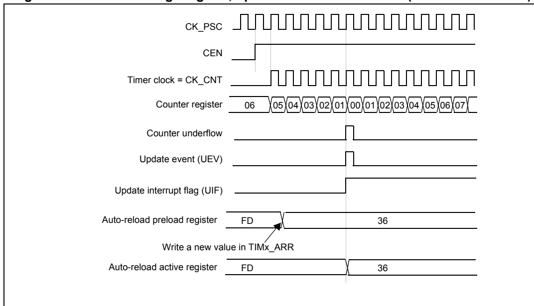
Figure 72. Counter timing diagram, update event with ARPE=1 (counter underflow)
