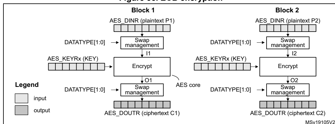
Figure 35. ECB encryption
