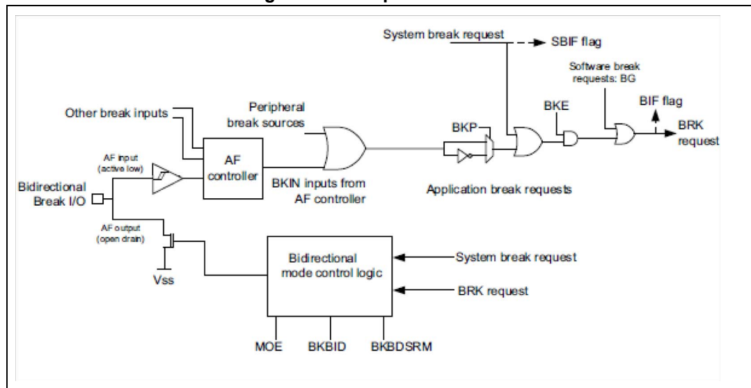
Figure 128. Output redirection
