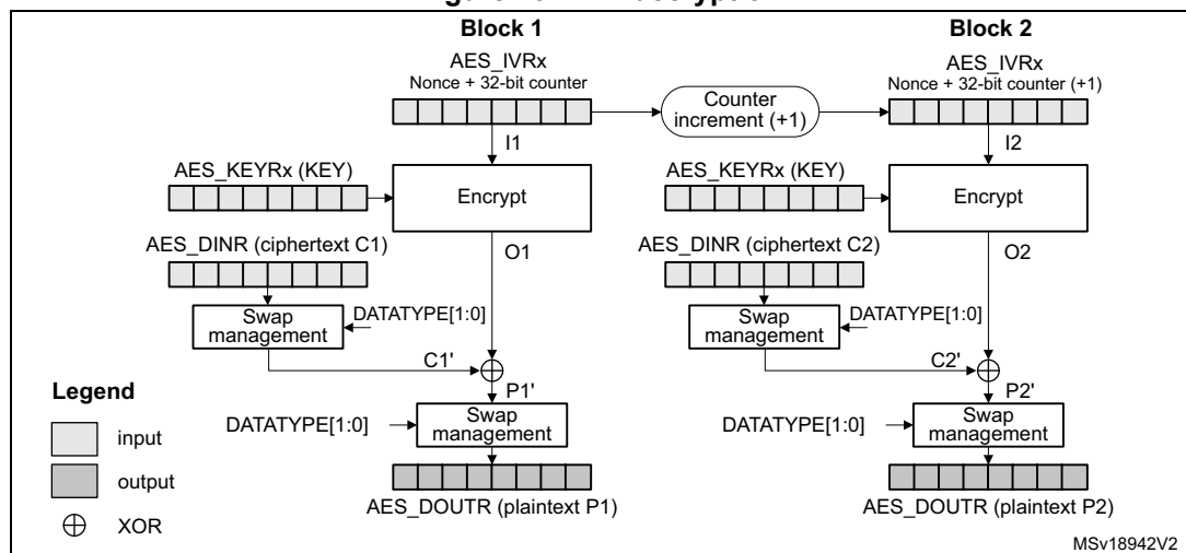
Figure 43. CTR decryption
