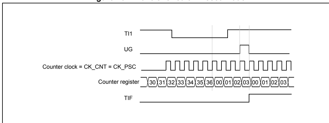
Figure 131. Control circuit in reset mode
