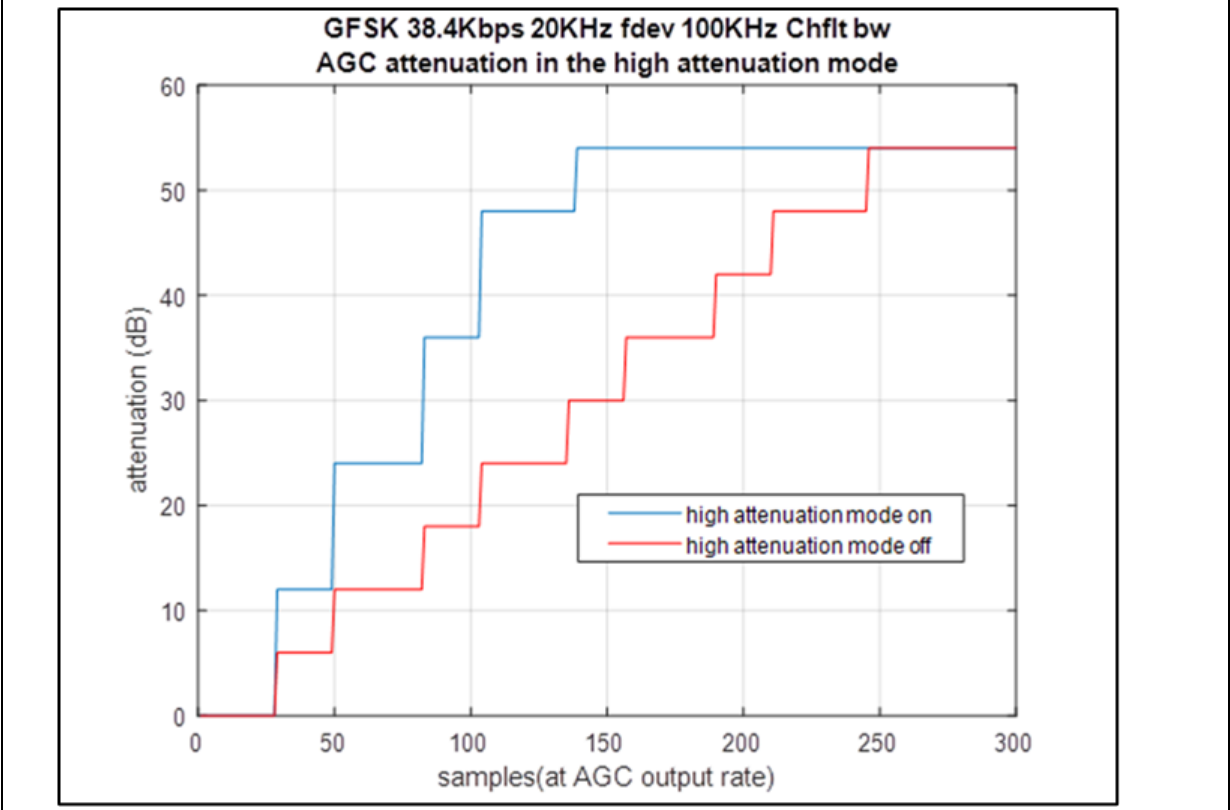
Figure 262. AGC high attenuation mode versus normal mode
