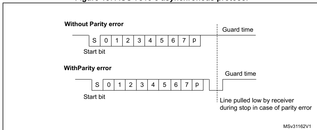
Figure 187. ISO 7816-3 asynchronous protocol
