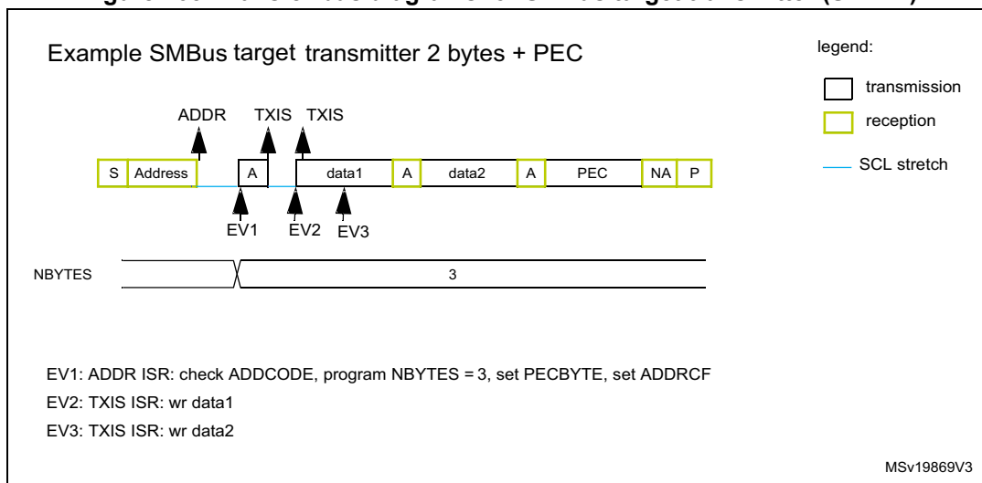
Figure 165. Transfer bus diagrams for SMBus target transmitter (SBC=1)
