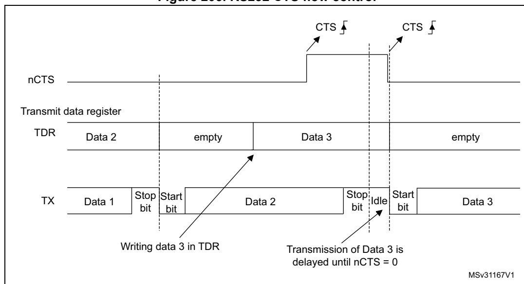
Figure 206. RS232 CTS flow control
