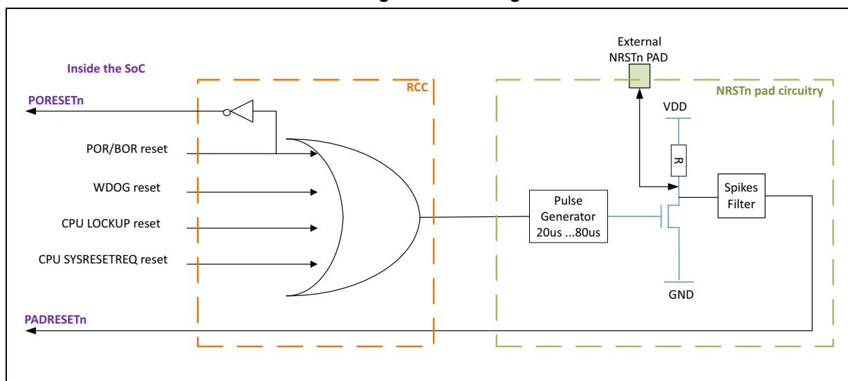
Figure 13. Reset generation
