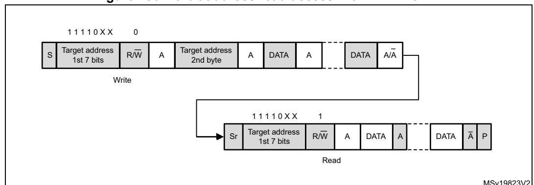
Figure 156. 10-bit address read access with HEAD10R=1
