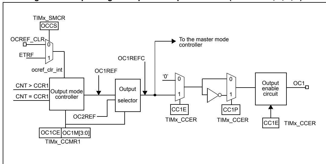
Figure 84. Output stage of capture/compare channel (channels 1, 2, 3, 4)
