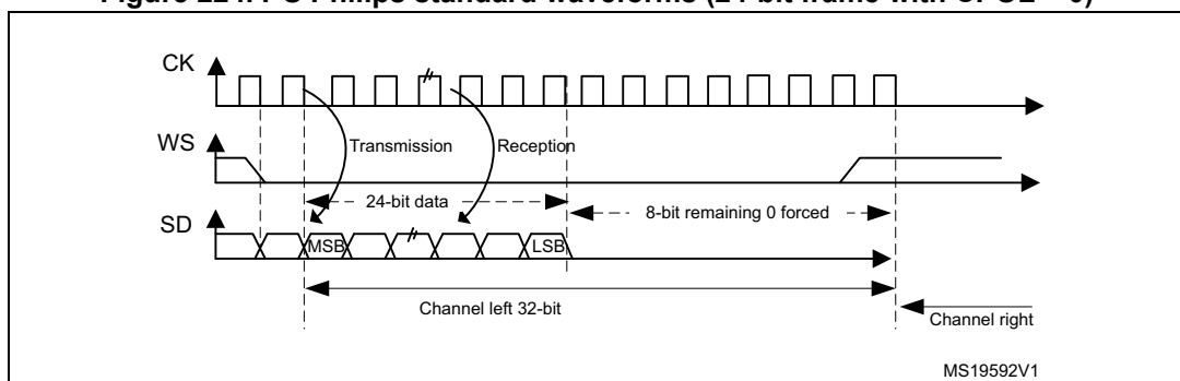
Figure 224. I 2 S Philips standard waveforms (24-bit frame with CPOL = 0)
