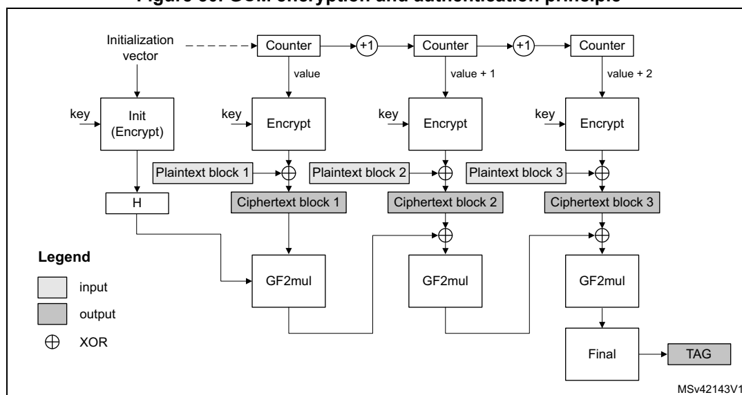
Figure 30. GCM encryption and authentication principle
