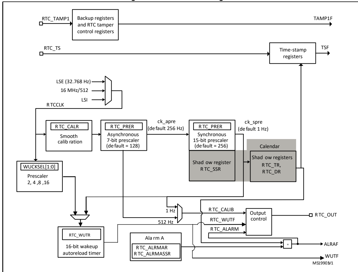
Figure 139. RTC block diagram
