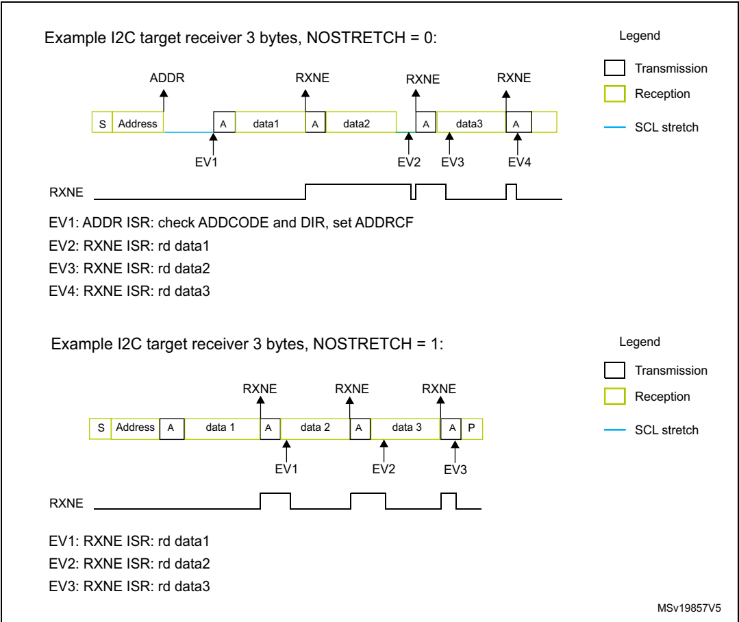
Figure 153. Transfer bus diagrams for I2C target receiver
