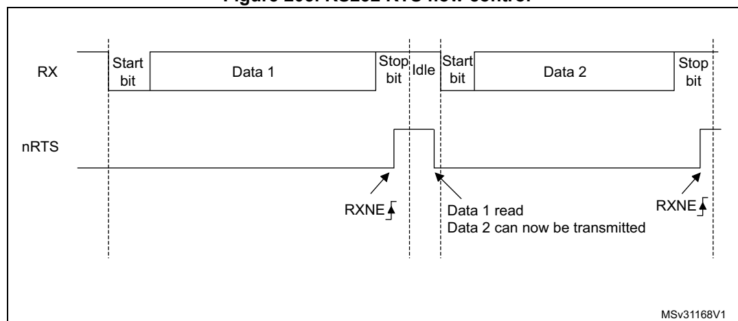
Figure 205. RS232 RTS flow control
