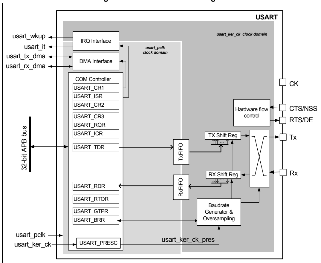
Figure 196. LPUART Block diagram
