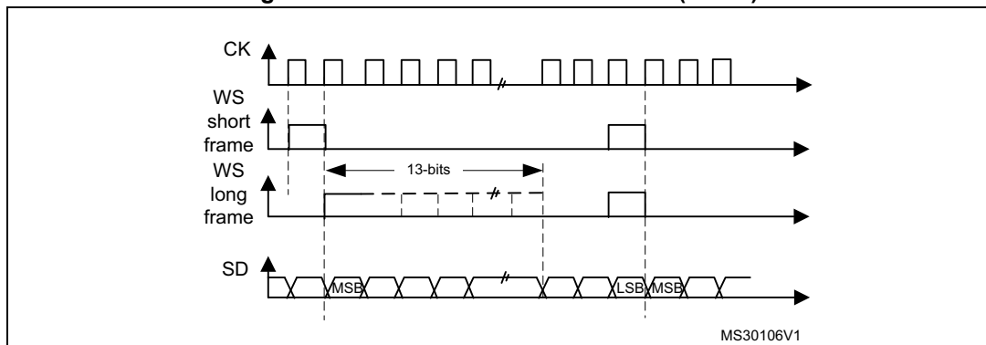
Figure 238. PCM standard waveforms (16-bit)
