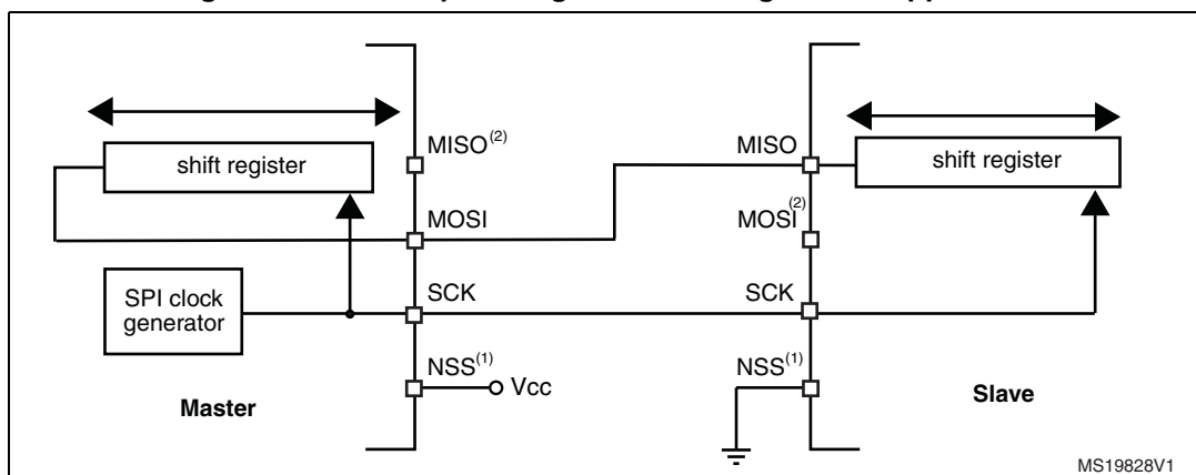
Figure 209. Half-duplex single master/ single slave application
