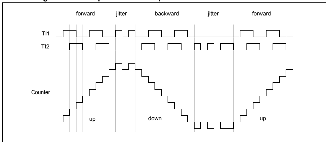
Figure 94. Example of counter operation in encoder interface mode.
