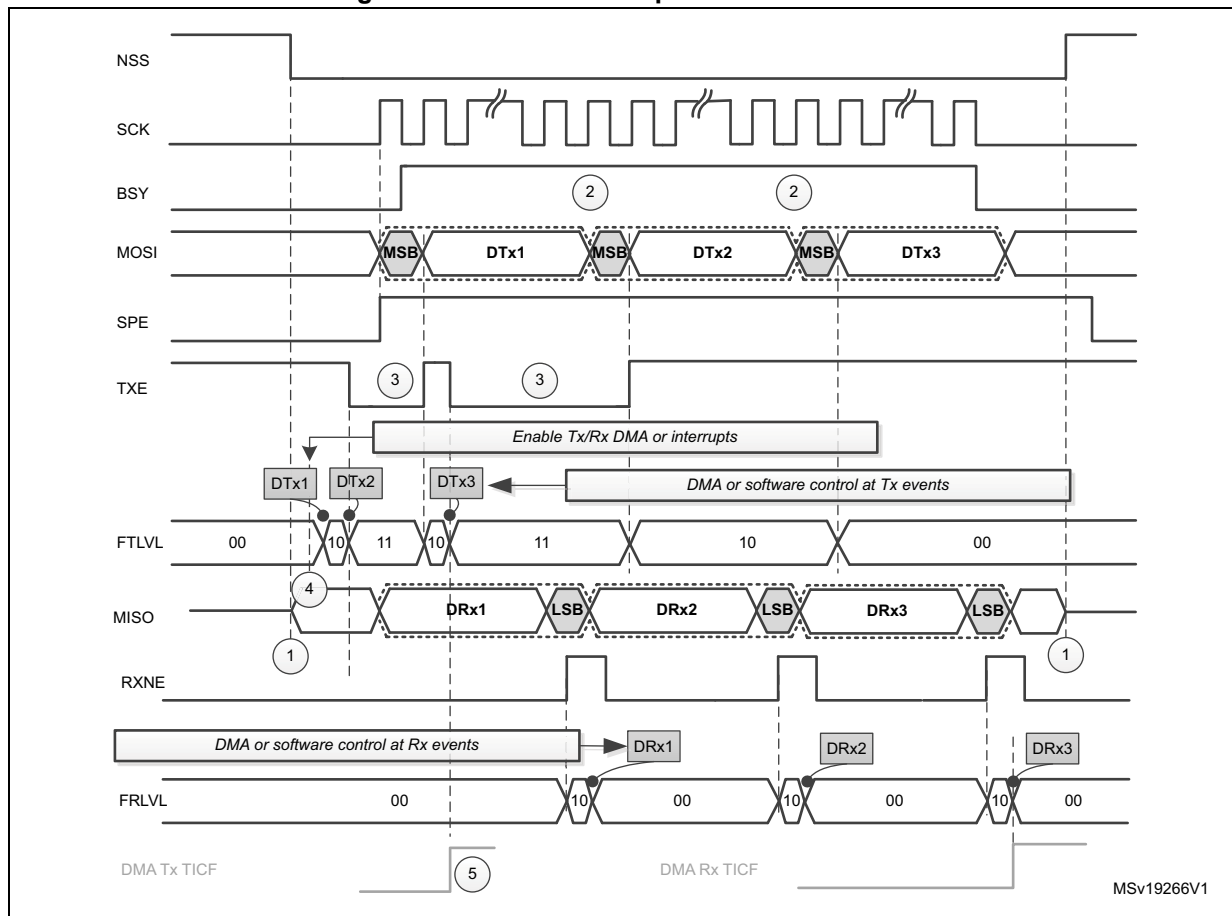
Figure 216. Master full duplex communication
