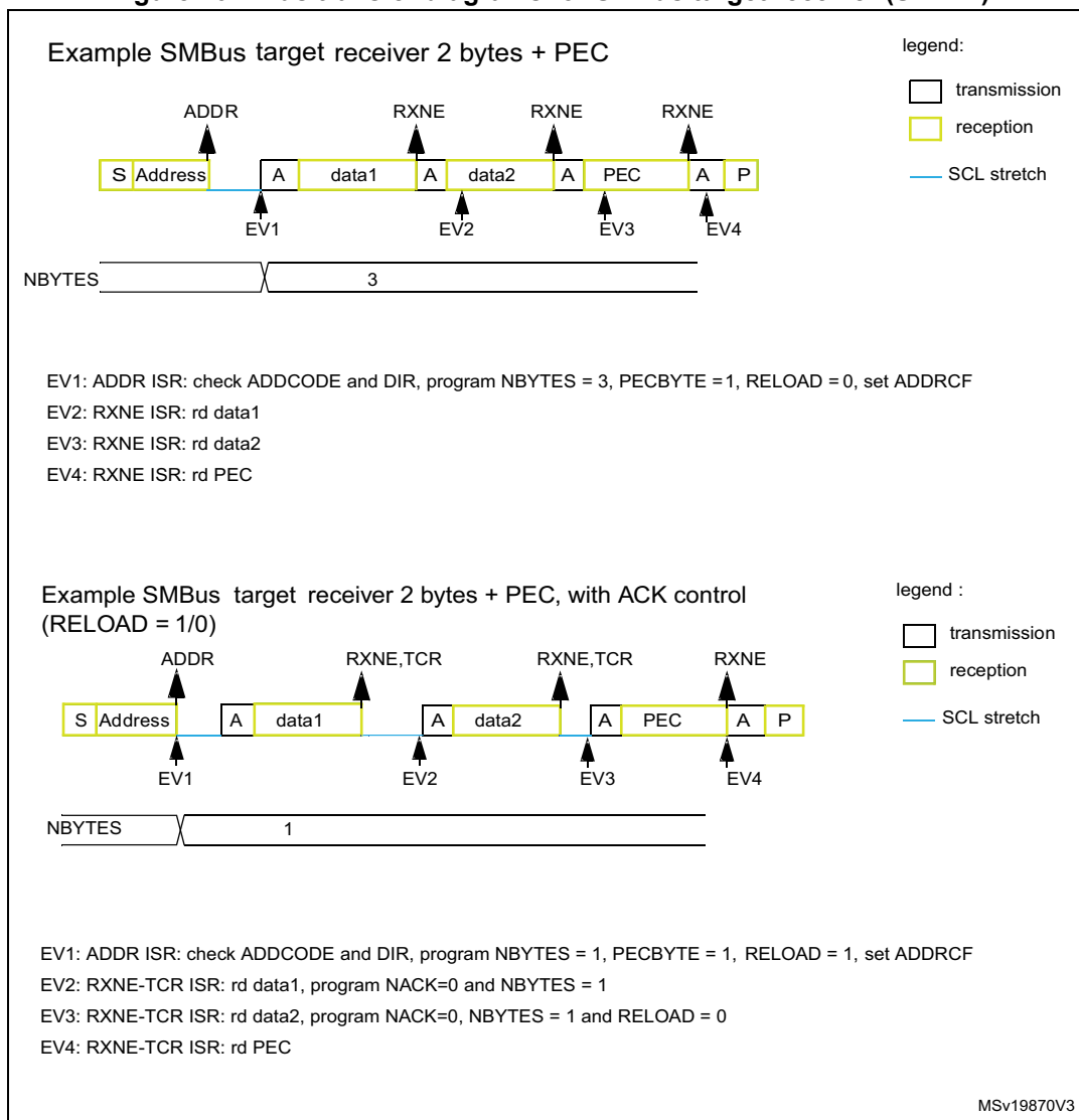
Figure 167. Bus transfer diagrams for SMBus target receiver (SBC=1)
