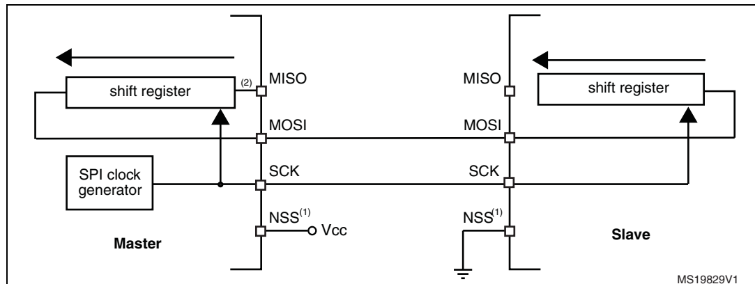
Figure 210. Simplex single master/single slave application (master in transmit-only/ slave in receive-only mode)
