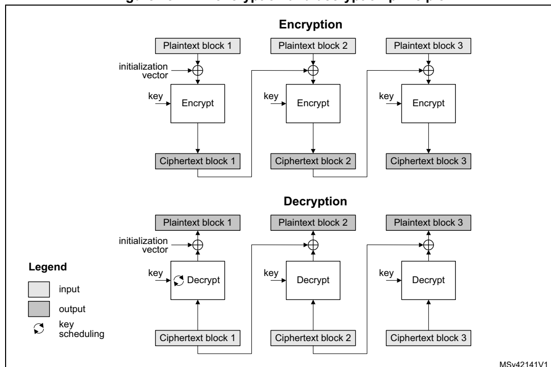
Figure 28. CBC encryption and decryption principle
