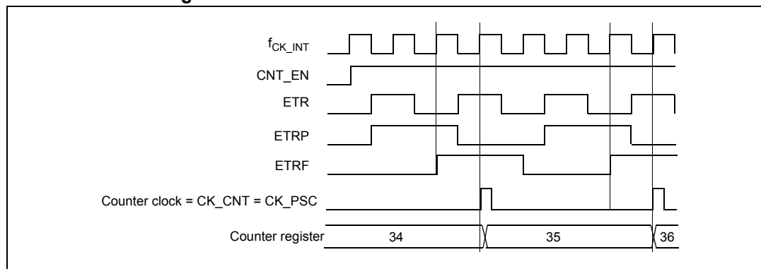
Figure 81. Control circuit in external clock mode 2
