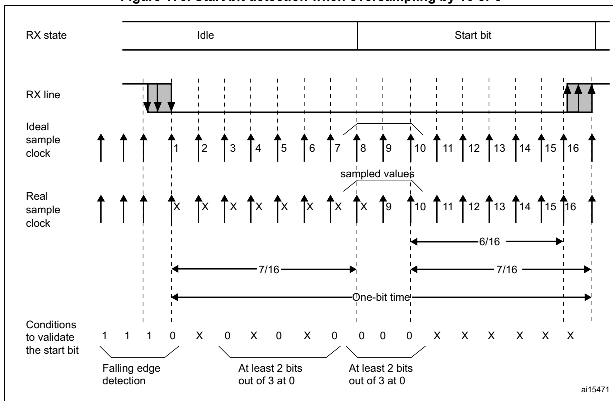
Figure 175. Start bit detection when oversampling by 16 or 8
