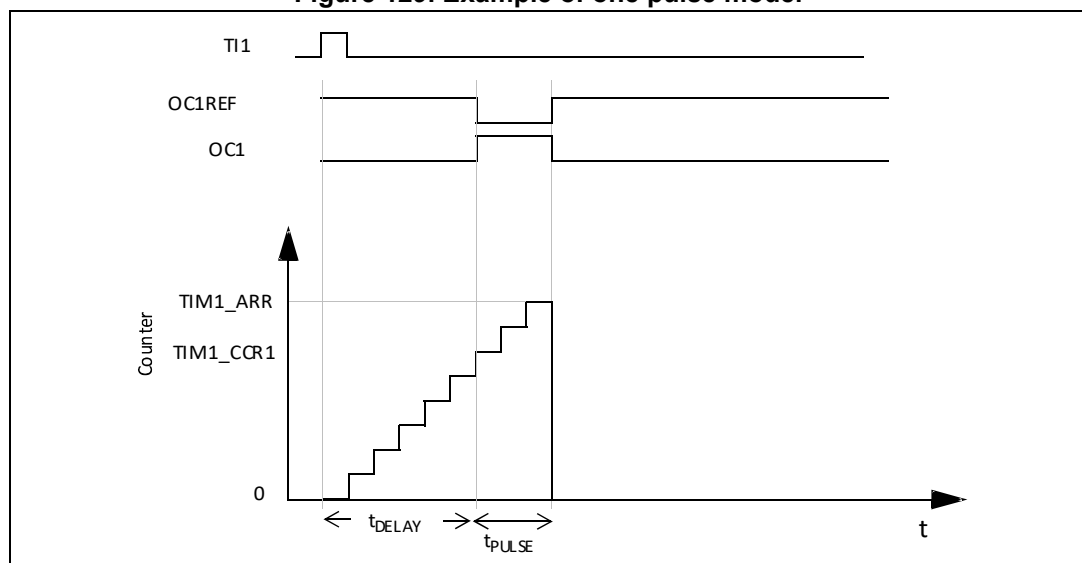
Figure 129. Example of one pulse mode.
