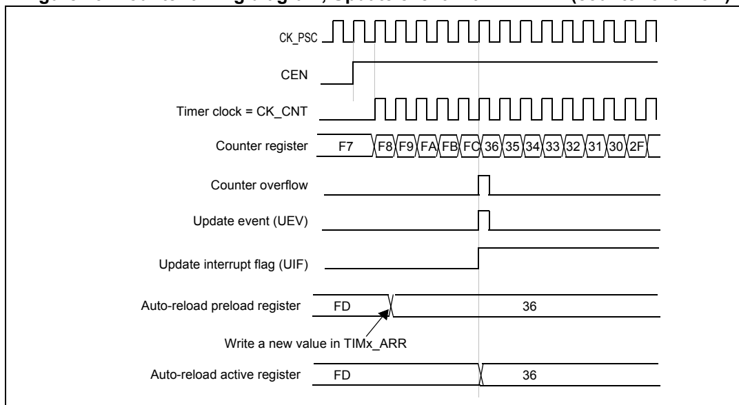
Figure 73. Counter timing diagram, Update event with ARPE=1 (counter overflow)
