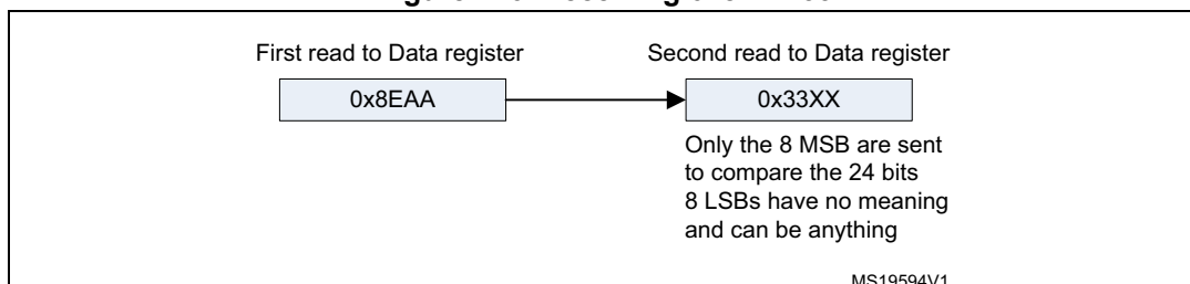
Figure 226. Receiving 0x8EAA33
