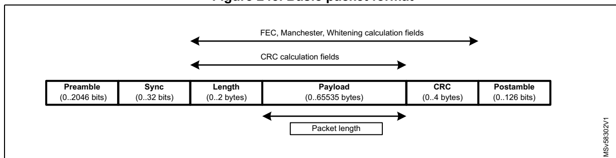
Figure 243. Basic packet format
