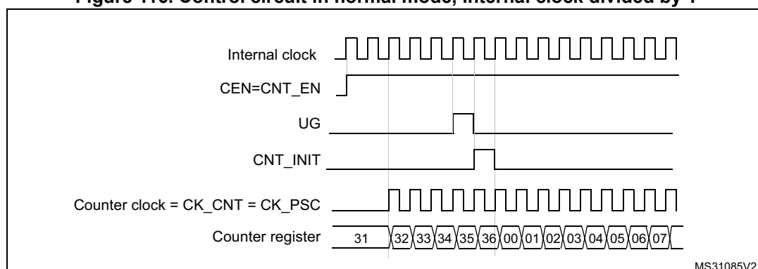
Figure 116. Control circuit in normal mode, internal clock divided by 1
