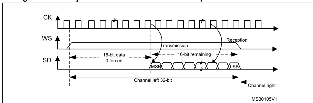
Figure 236. LSB justified 16-bit extended to 32-bit packet frame with CPOL = 0
