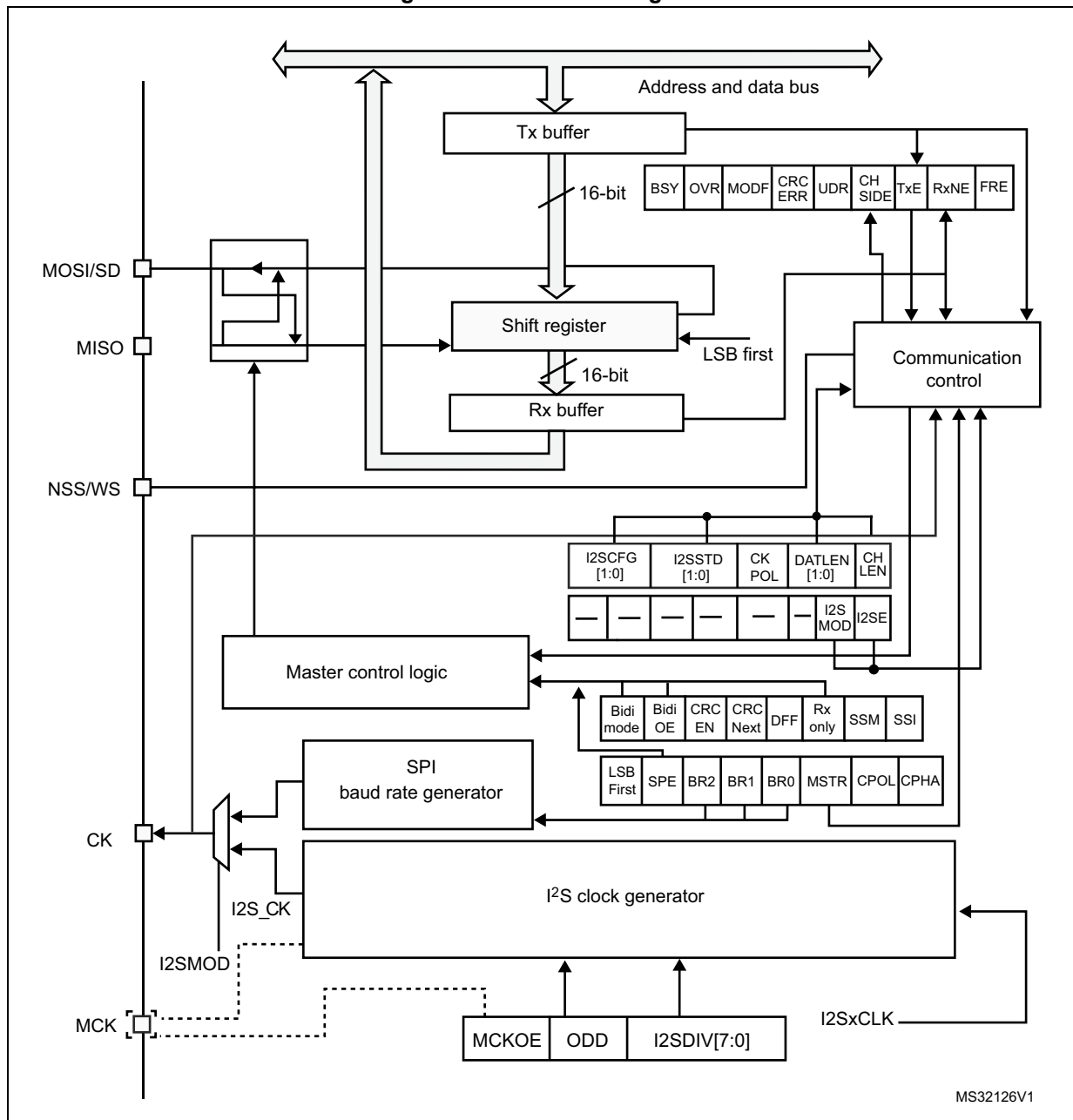
Figure 222. I 2 S block diagram
