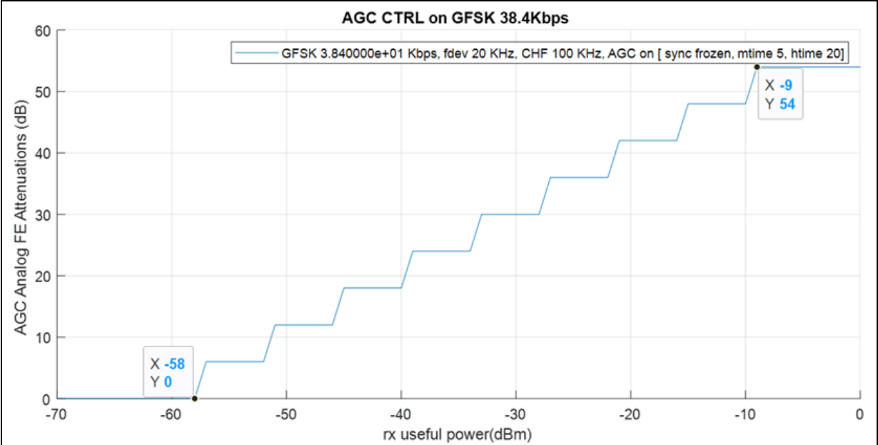
Figure 261. AGC attenuation example
