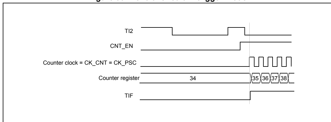
Figure 99. Control circuit in trigger mode
