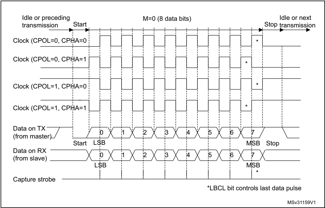
Figure 184. USART data clock timing diagram (M=0)
