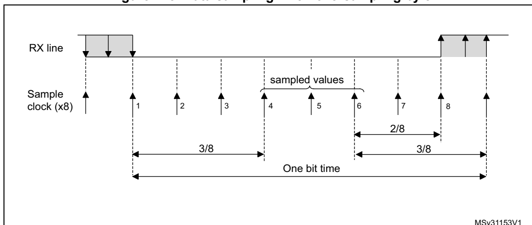
Figure 178. Data sampling when oversampling by 8
