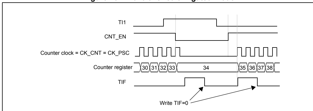
Figure 132. Control circuit in gated mode
