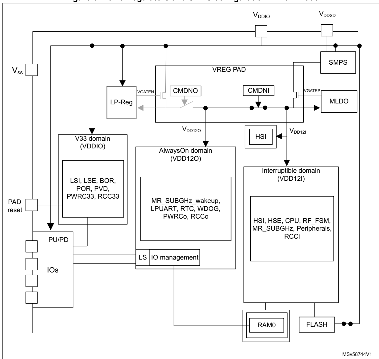
Figure 6. Power regulators and SMPS configuration in Run mode
