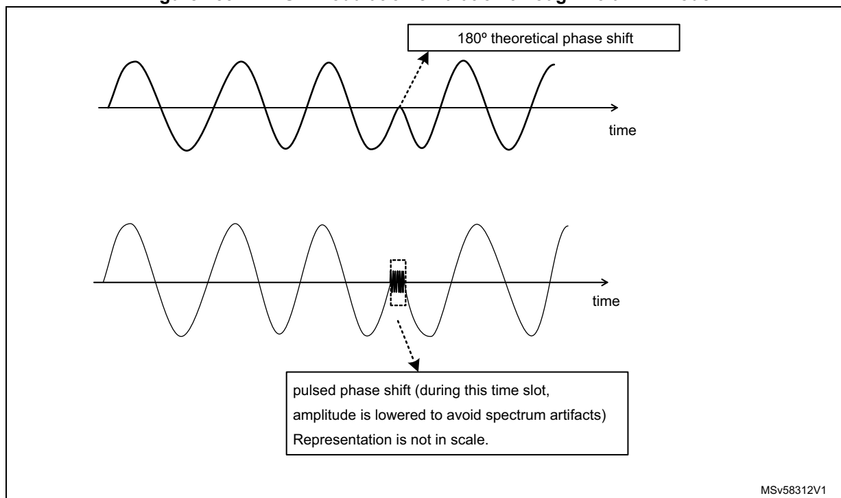
Figure 253. DBPSK modulation emulation through Polar TX mode
