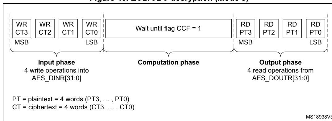
Figure 40. ECB/CBC decryption (Mode 3)
