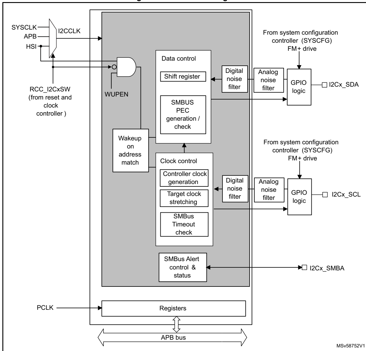
Figure 141. I2C block diagram
