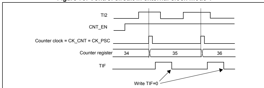
Figure 79. Control circuit in external clock mode 1
