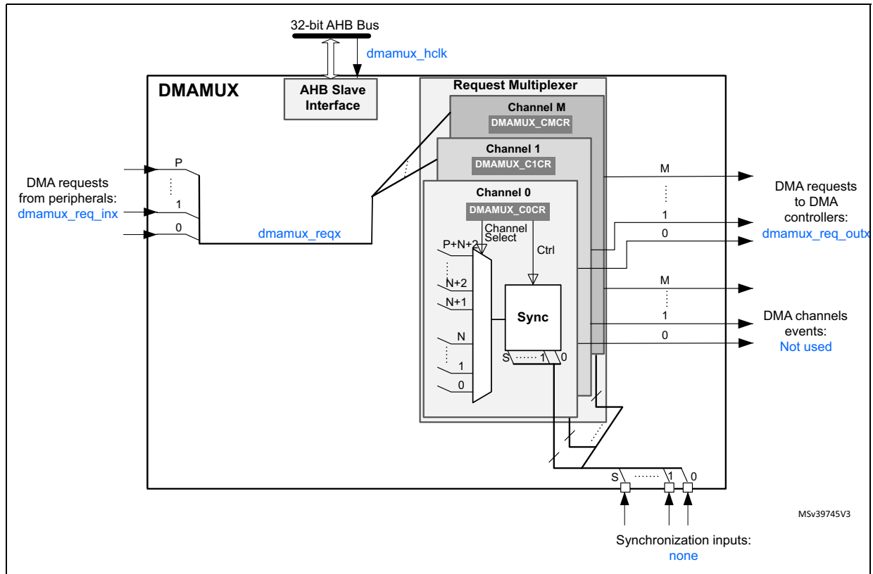
Figure 22. DMAMUX block diagram
