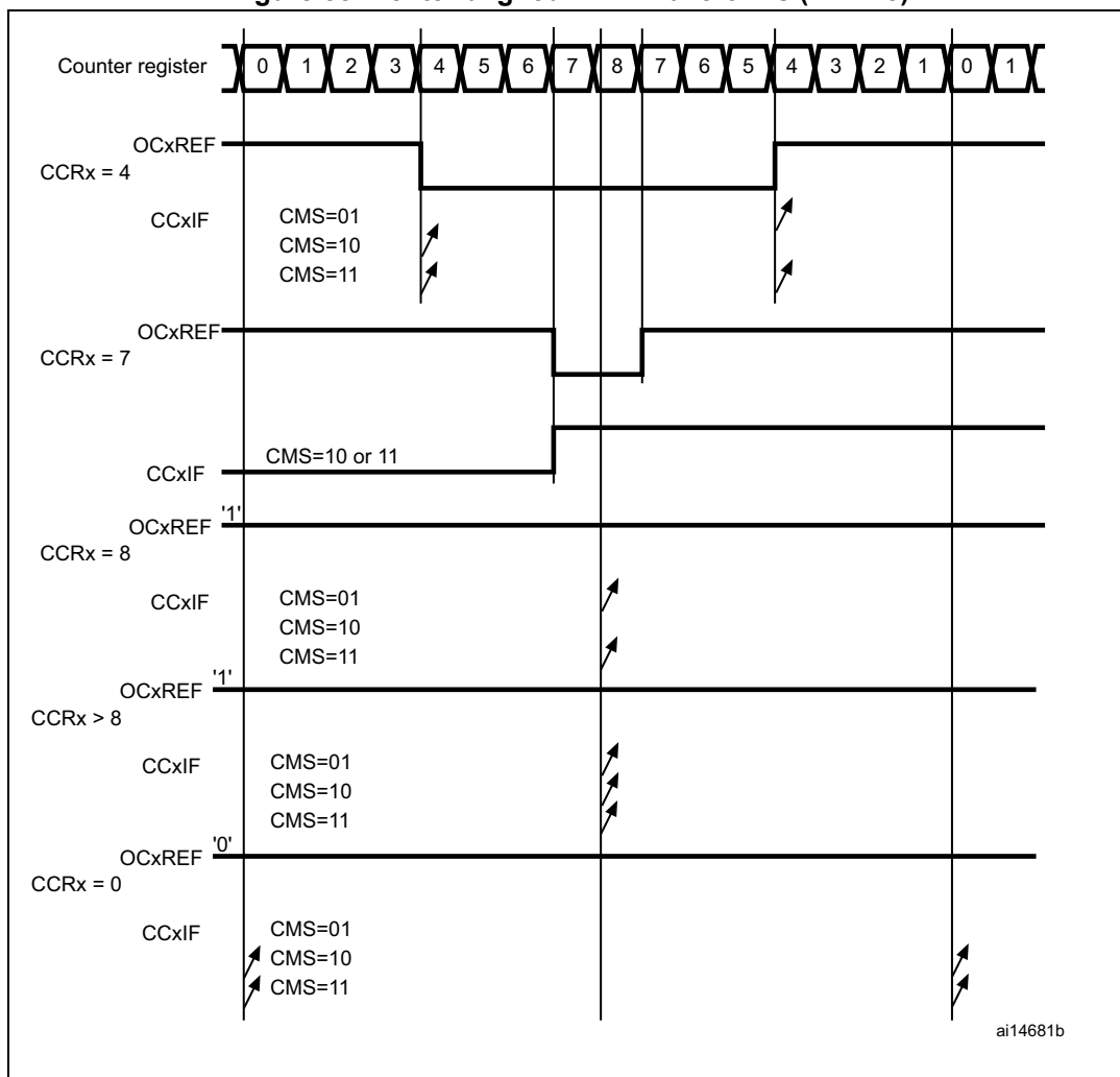
Figure 88. Center-aligned PWM waveforms (ARR=8)
