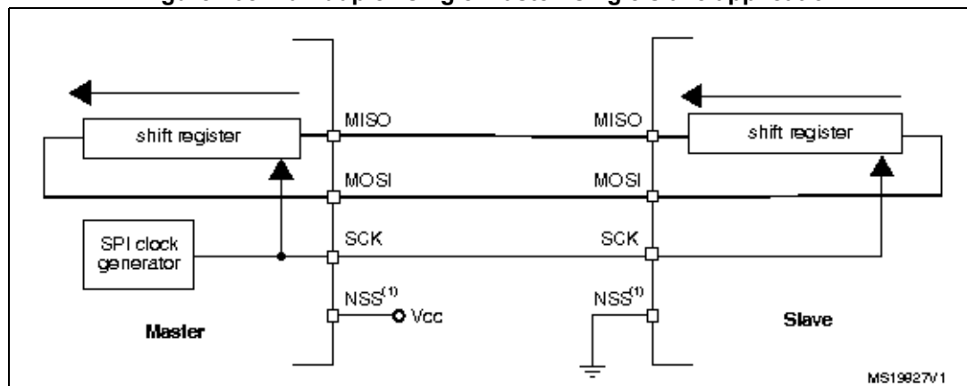
Figure 208. Full-duplex single master/ single slave application
