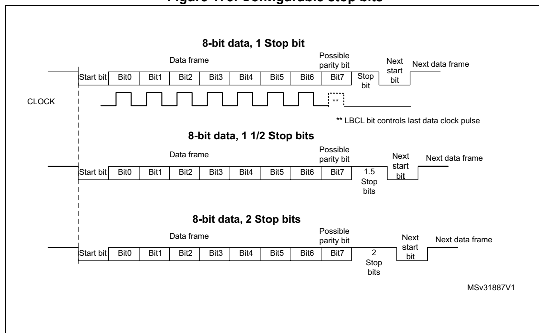
Figure 173. Configurable stop bits
