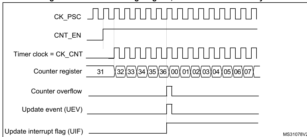
Figure 109. Counter timing diagram, internal clock divided by 1
