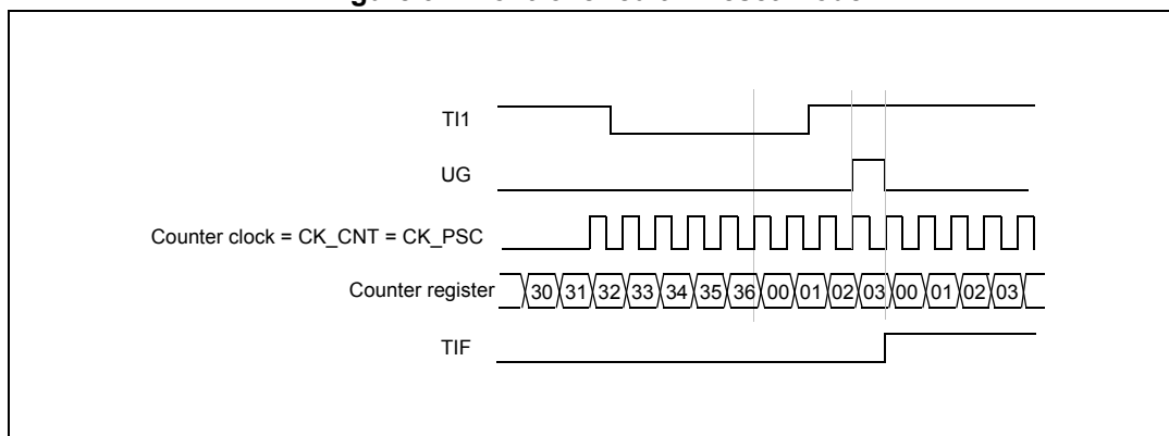
Figure 97. Control circuit in reset mode
