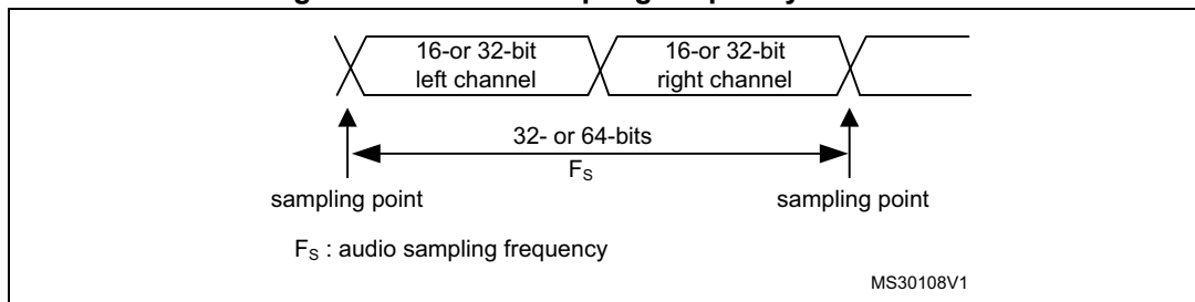
Figure 240. Audio sampling frequency definition
