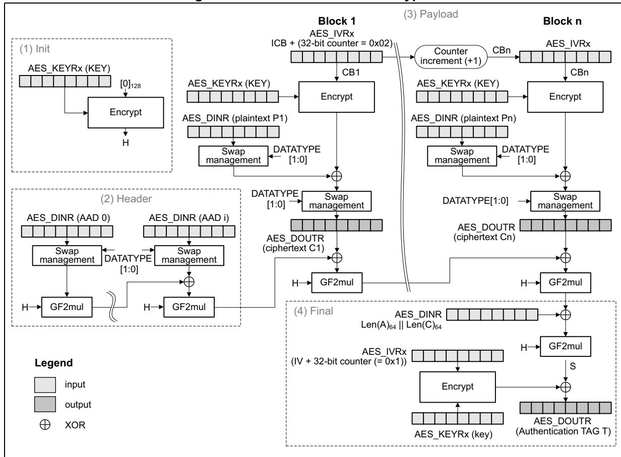
Figure 45. GCM authenticated encryption
