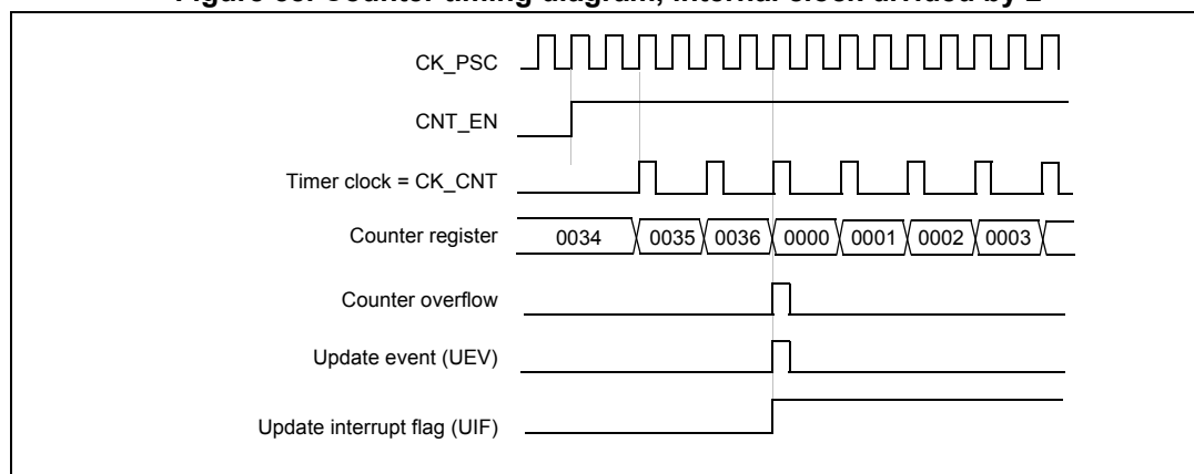
Figure 58. Counter timing diagram, internal clock divided by 2
