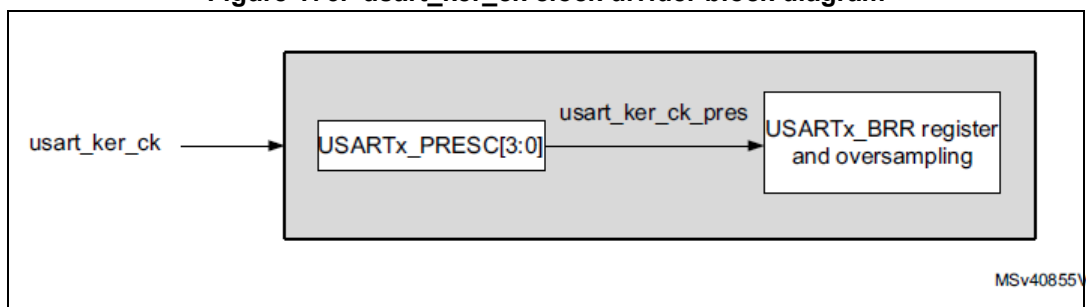
Figure 176. usart_ker_ck clock divider block diagram
