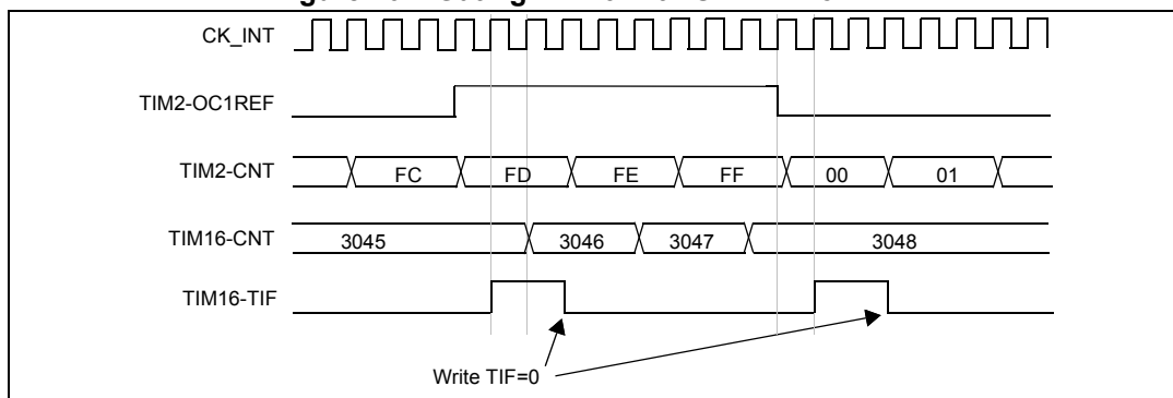
Figure 102. Gating TIM16 with OC1REF of TIM2
