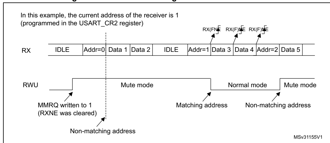
Figure 201. Mute mode using address mark detection
