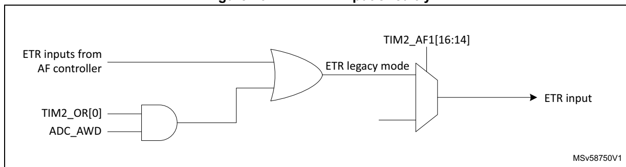
Figure 76. TIM2 ETR input circuitry
