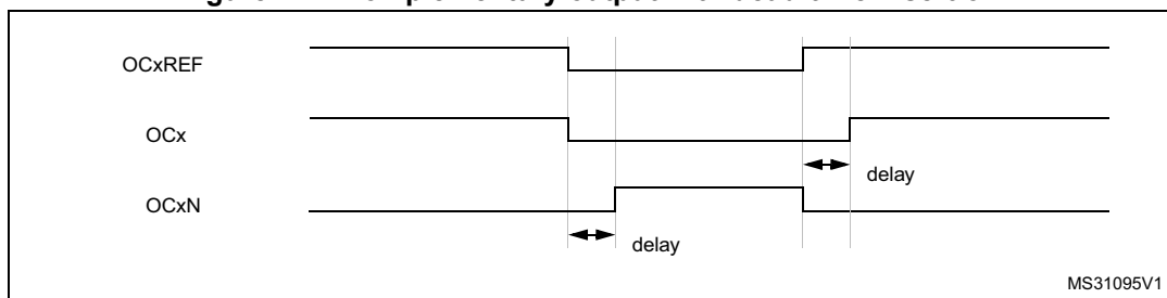
Figure 124. Complementary output with dead-time insertion.
