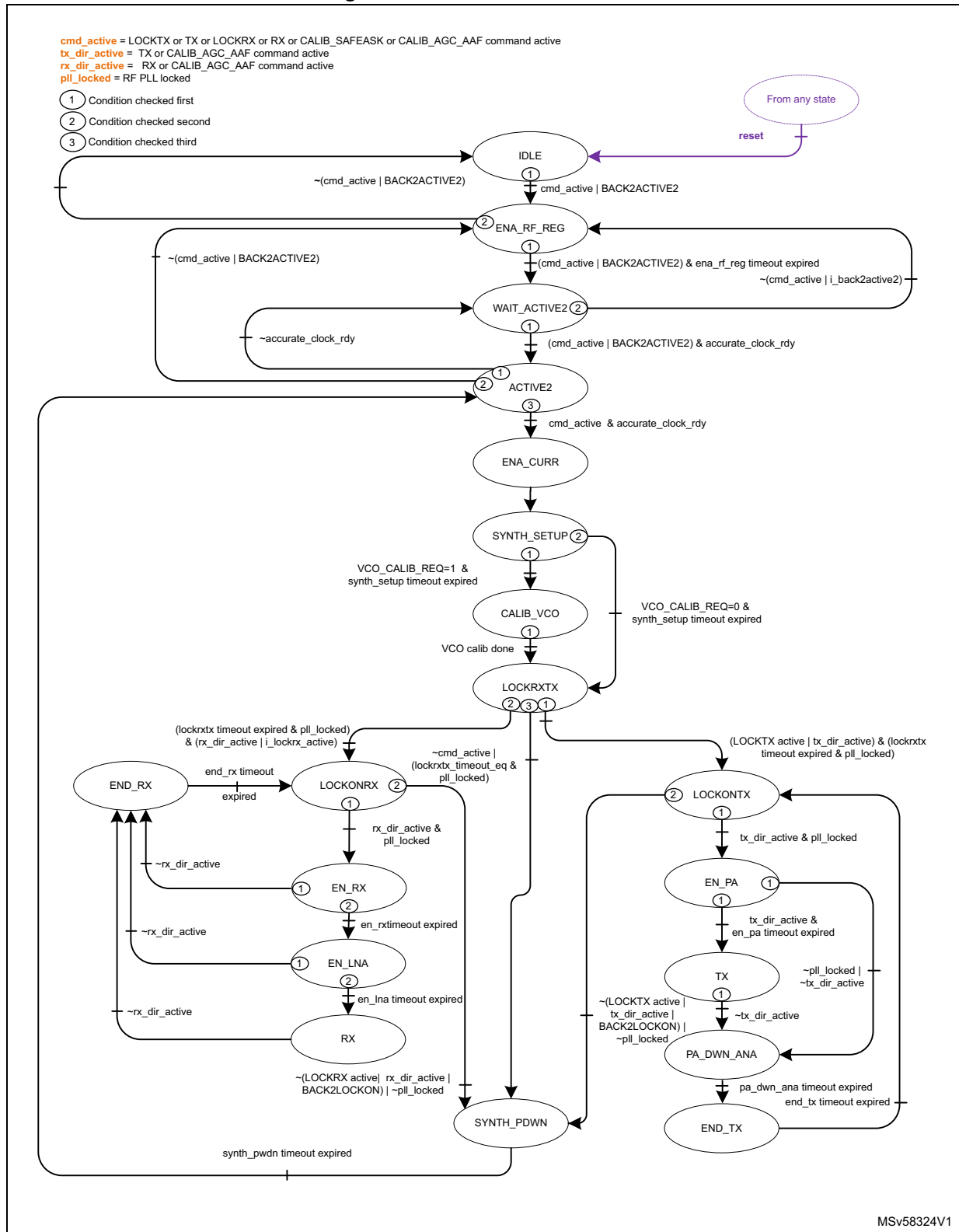
Figure 265. Radio FSM overview
