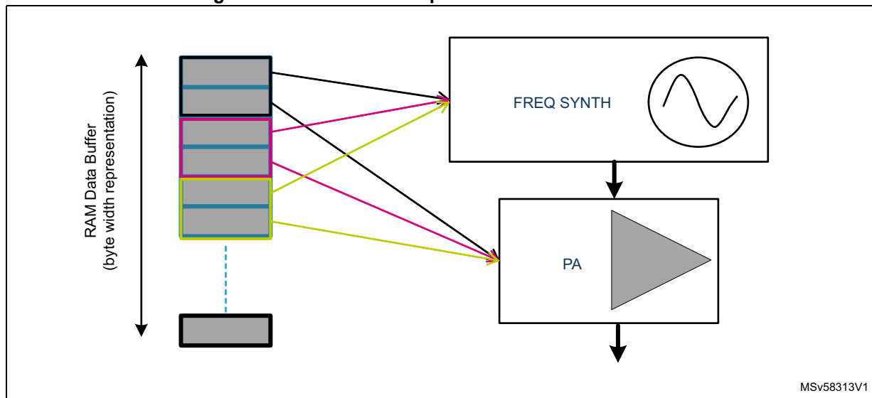
Figure 254. Transmission path for Polar TX modulation
