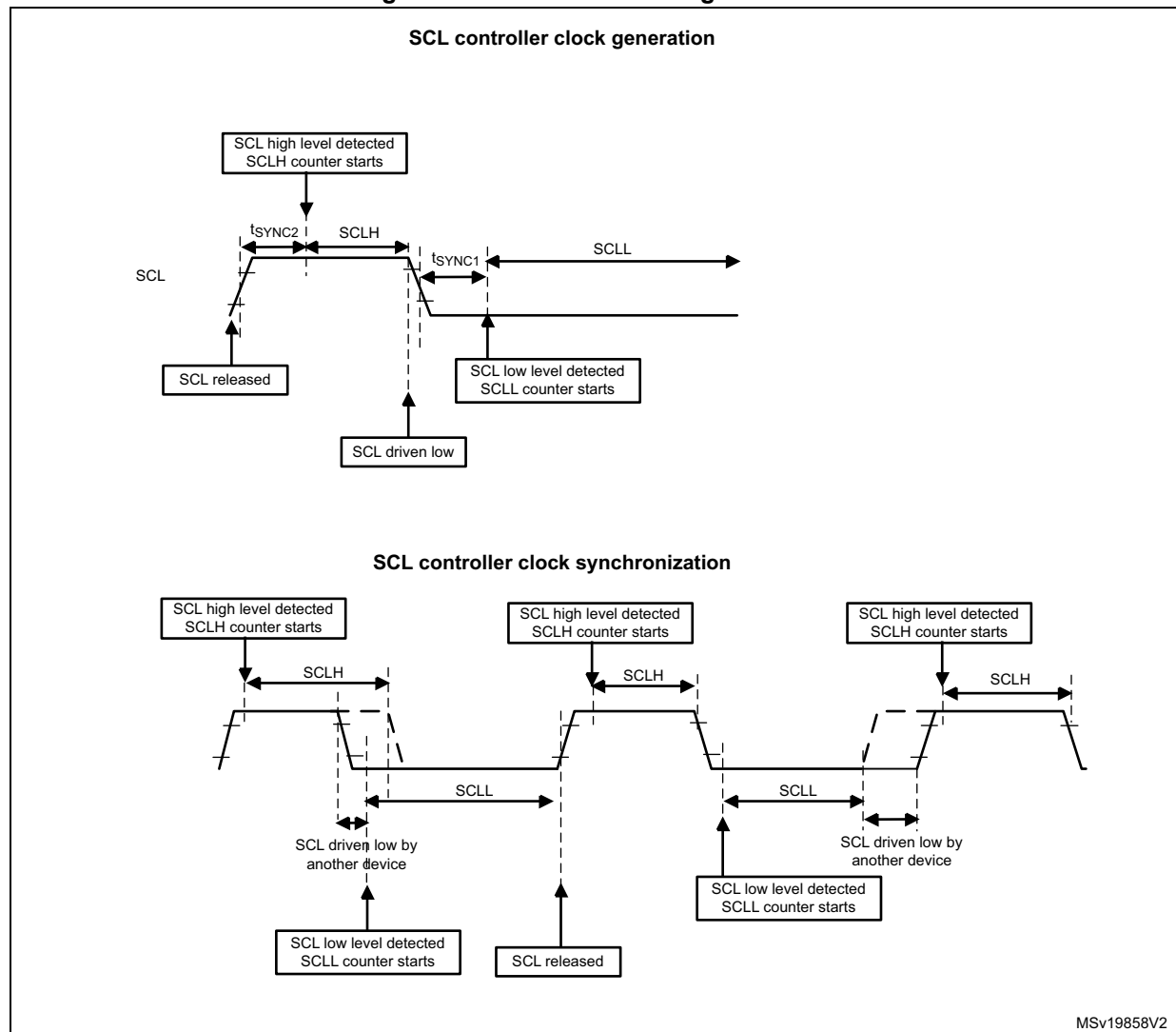
Figure 154. Controller clock generation
