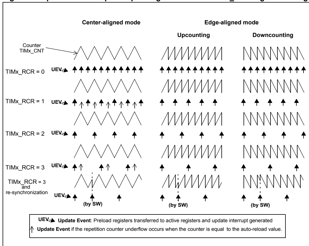
Figure 74. Update rate examples depending on mode and TIMx_RCR register settings
