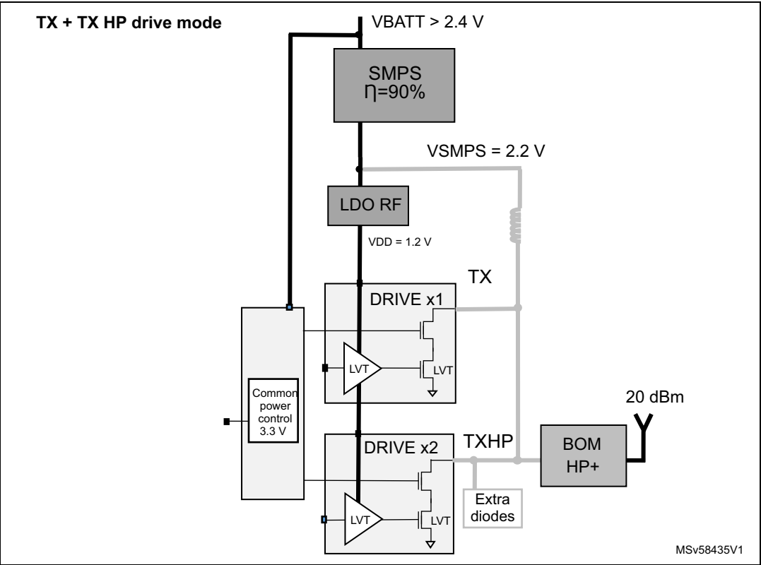
Figure 257. TX and TX HP pin connections, TX + TX HP PA drive mode, VBATT > 2.4 V
