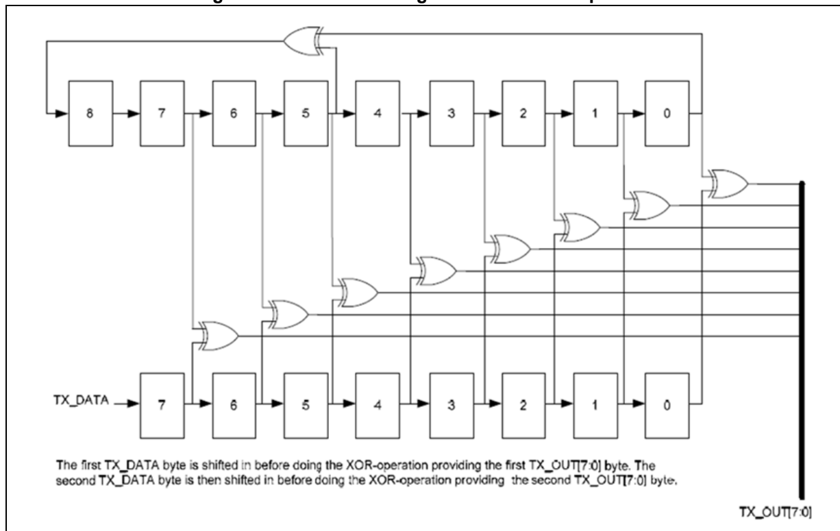
Figure 245. Data whitening scheme for Basic packets
