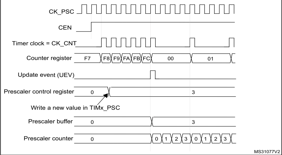
Figure 108. Counter timing diagram with prescaler division change from 1 to 4
