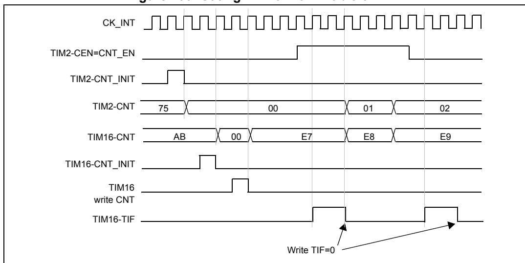
Figure 103. Gating TIM16 with Enable of TIM2
