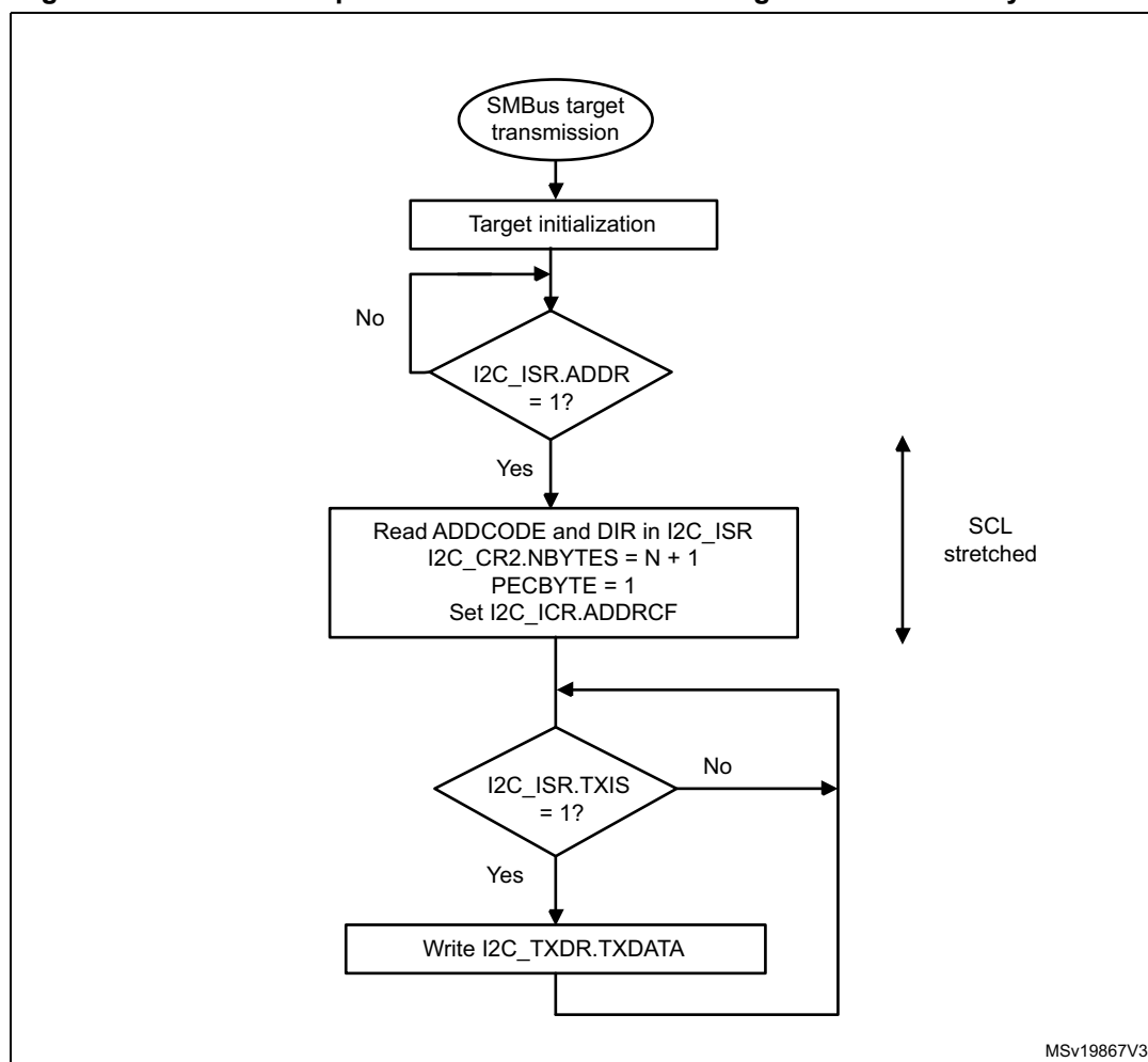
Figure 164. Transfer sequence flowchart for SMBus target transmitter N bytes + PEC
