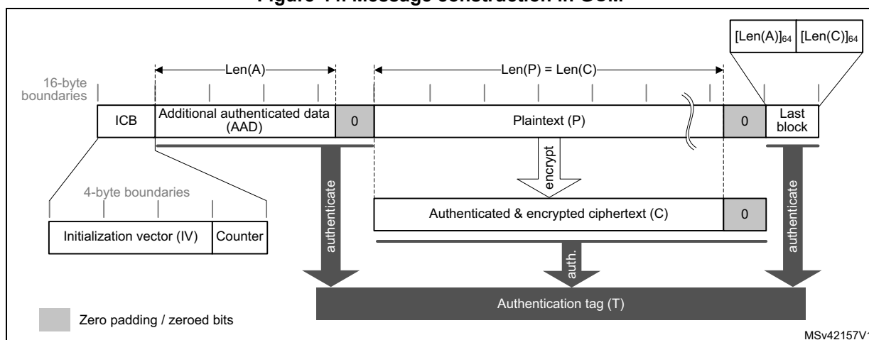
Figure 44. Message construction in GCM
