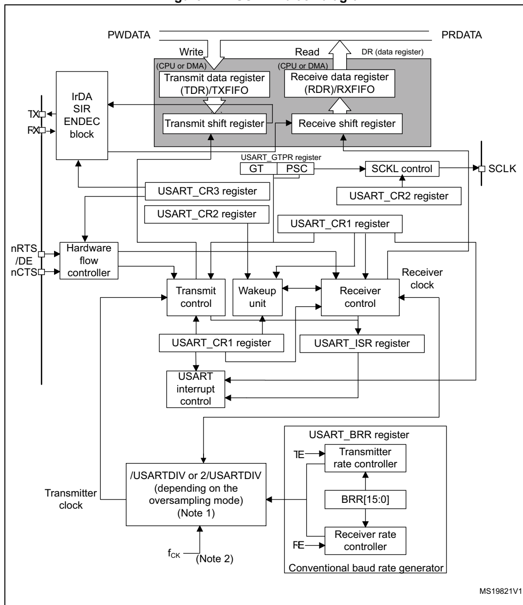
Figure 171. USART block diagram
