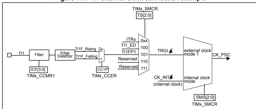
Figure 117. TI1 external clock connection example
