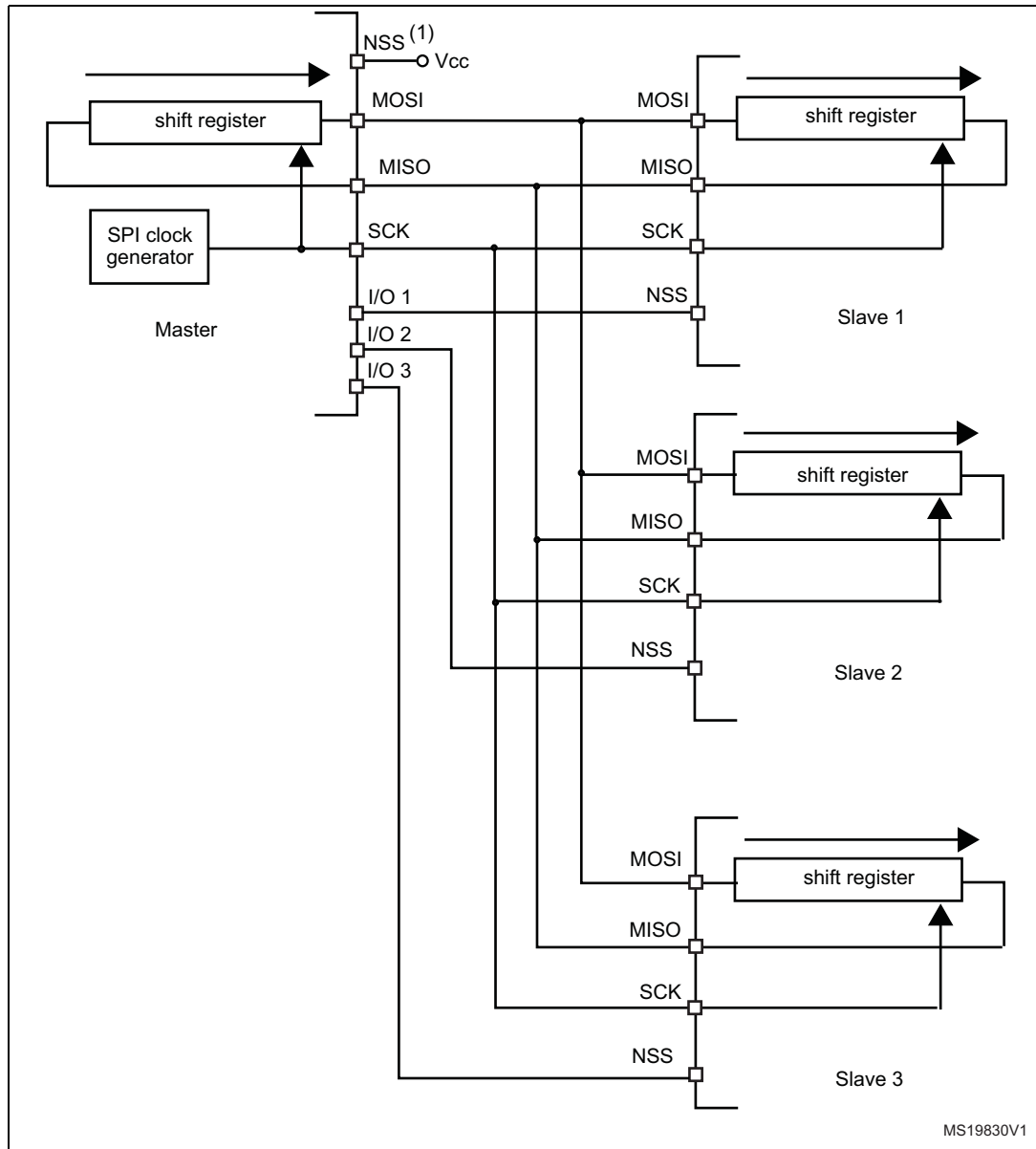
Figure 211. Master and three independent slaves
