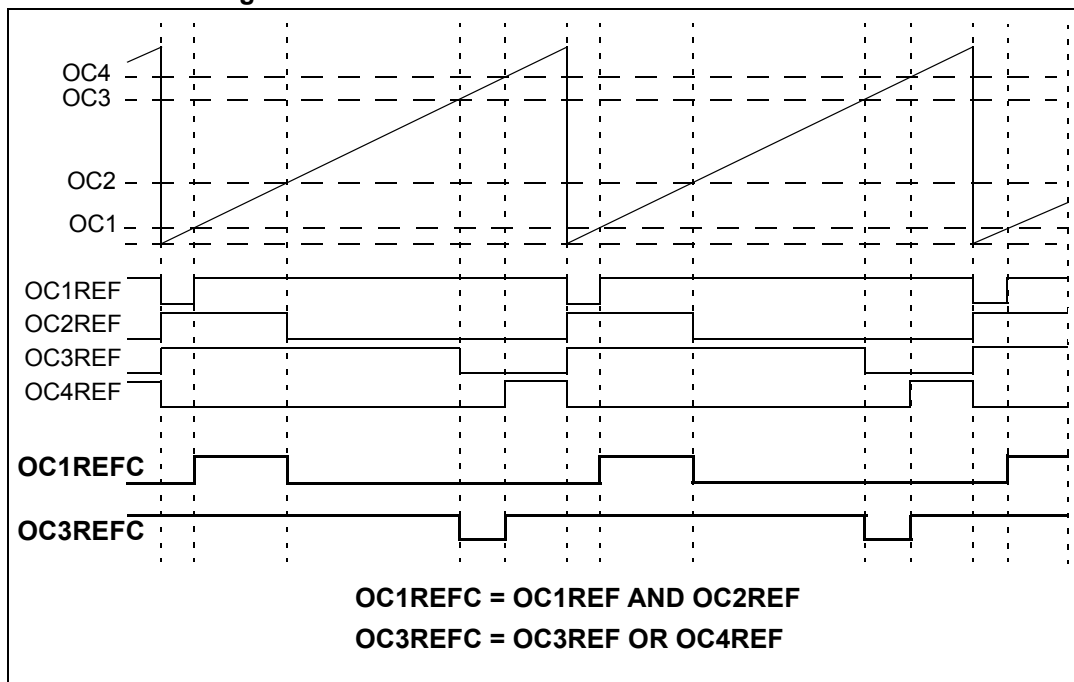
Figure 90. Combined PWM mode on channel 1 and 3
