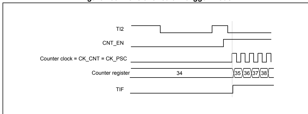
Figure 133. Control circuit in trigger mode
