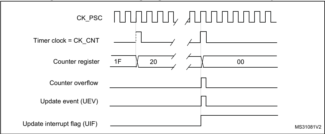
Figure 112. Counter timing diagram, internal clock divided by N
