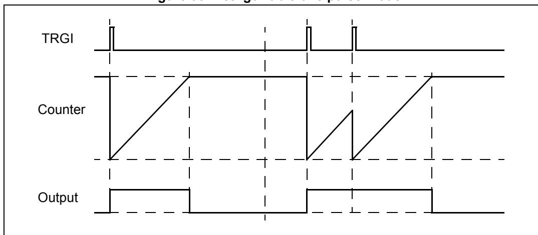
Figure 93. Retriggerable one pulse mode
