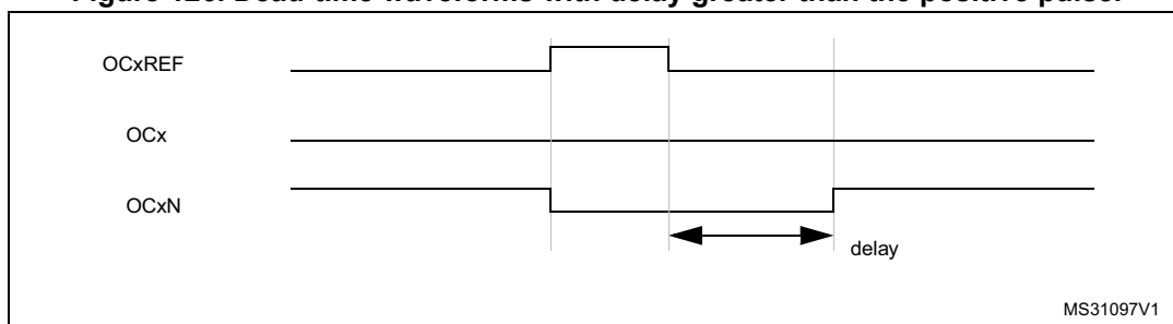
Figure 126. Dead-time waveforms with delay greater than the positive pulse.
