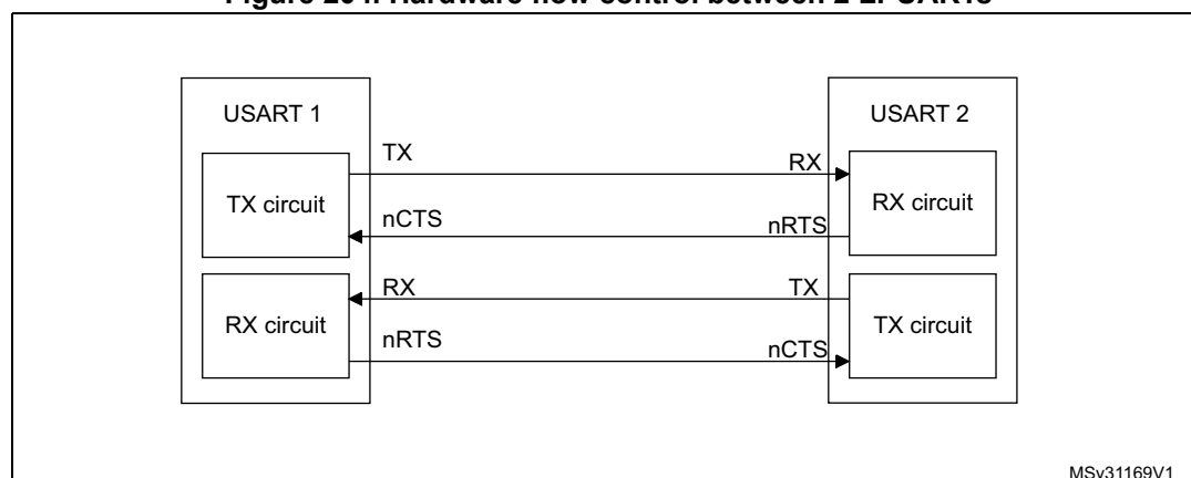
Figure 204. Hardware flow control between 2 LPUARTs
