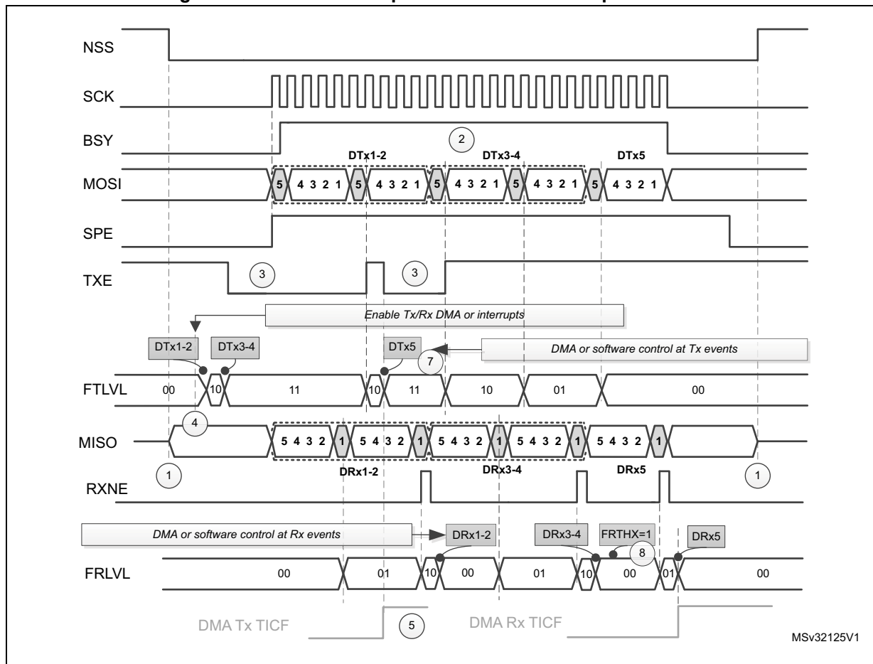
Figure 219. Master full duplex communication in packed mode
