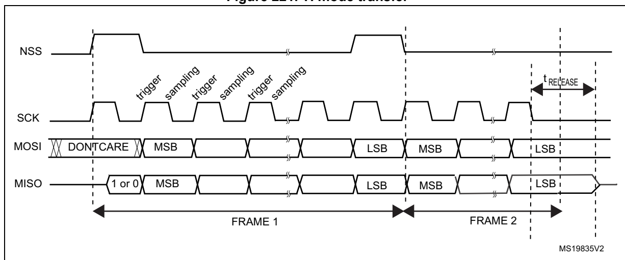
Figure 221. TI mode transfer
