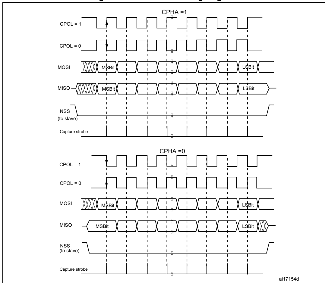
Figure 213. Data clock timing diagram
