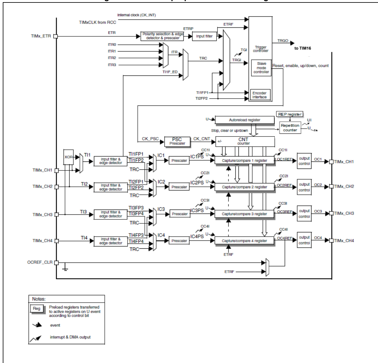
Figure 54. General purpose timer block diagram
