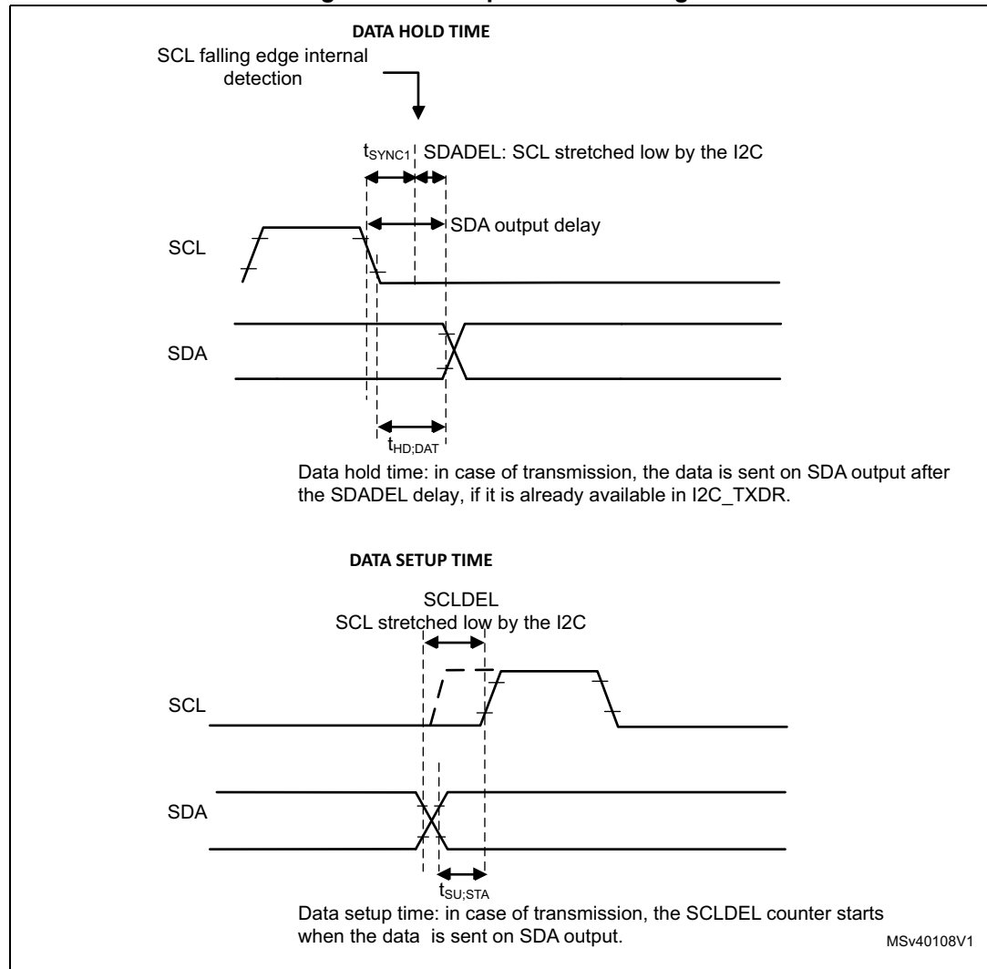
Figure 143. Setup and hold timings
