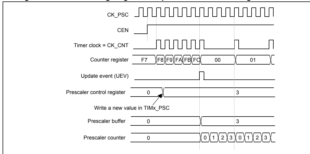
Figure 56. Counter timing diagram with prescaler division change from 1 to 4
