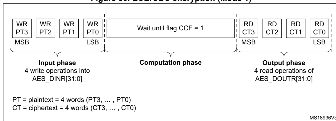
Figure 39. ECB/CBC encryption (Mode 1)
