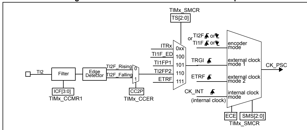
Figure 78. TI2 external clock connection example
