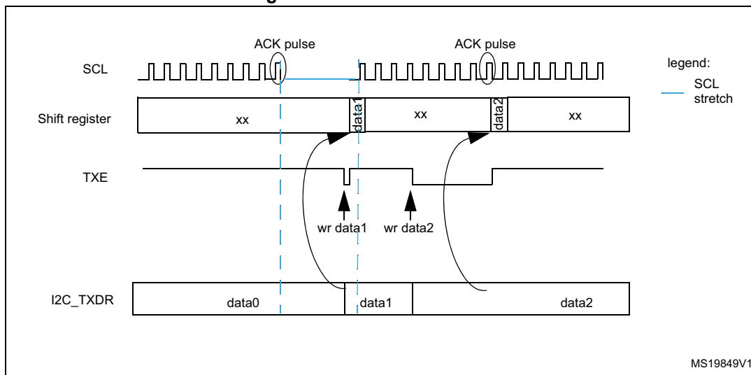
Figure 146. Data transmission
