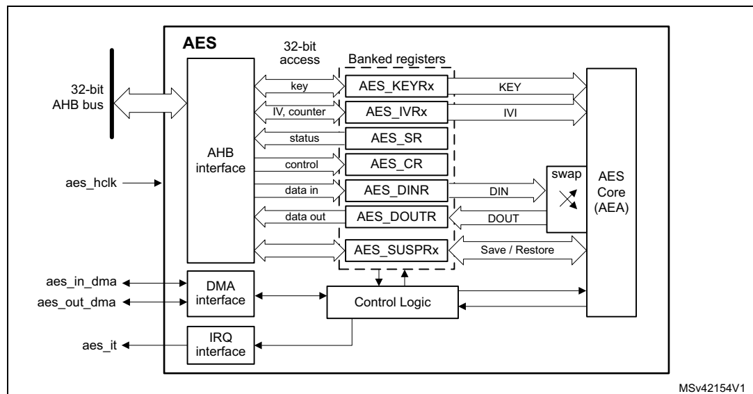
Figure 26. AES block diagram
