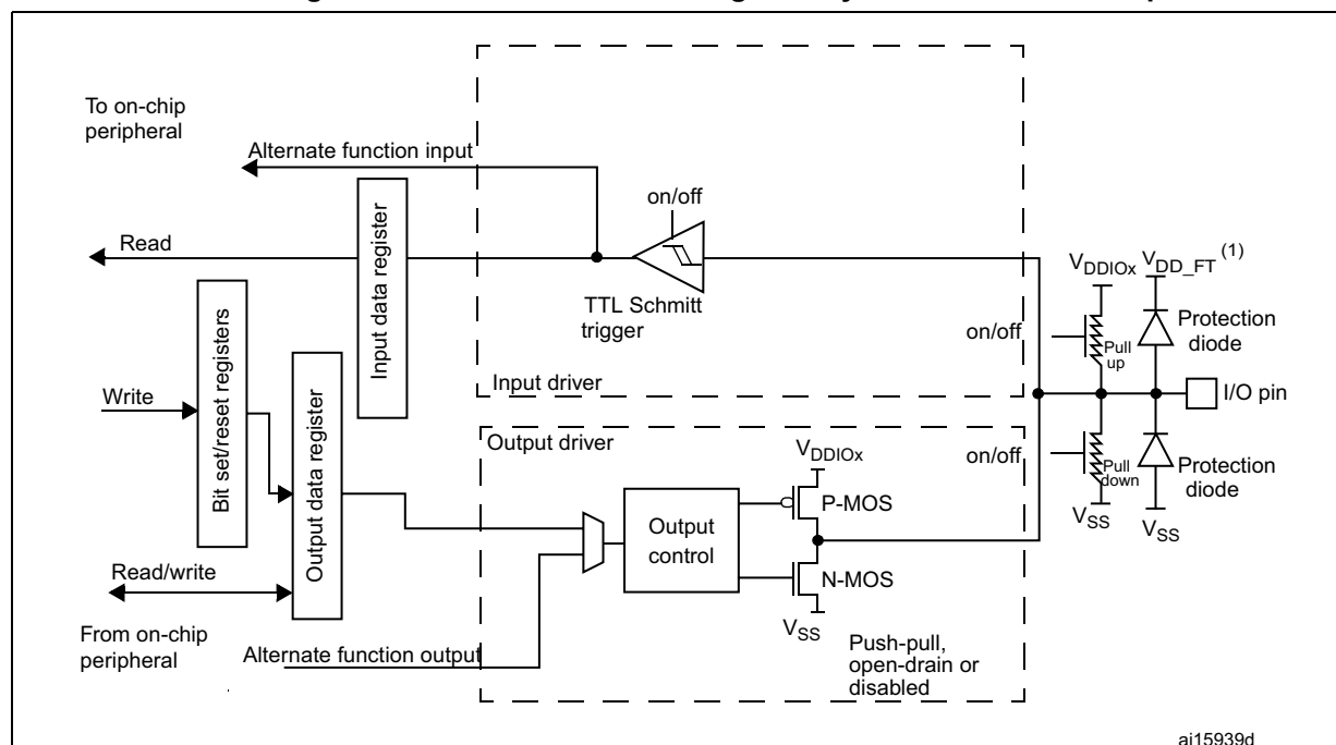
Figure 17. Basic structure of a digital only five-volt tolerant I/O port bit
