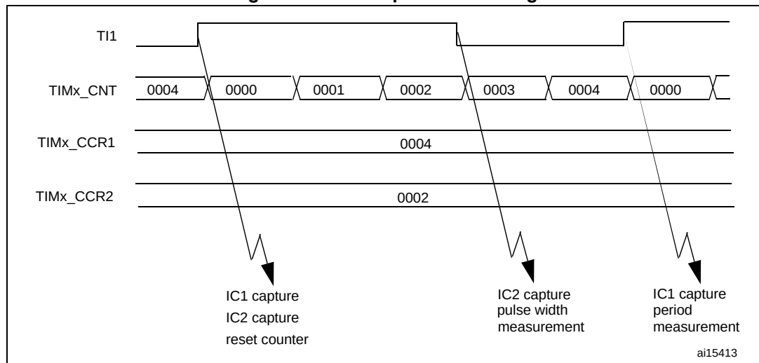
Figure 85. PWM input mode timing
