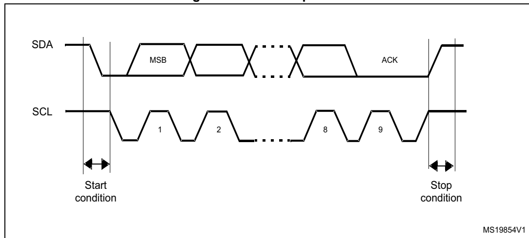
Figure 142. I 2 C bus protocol
