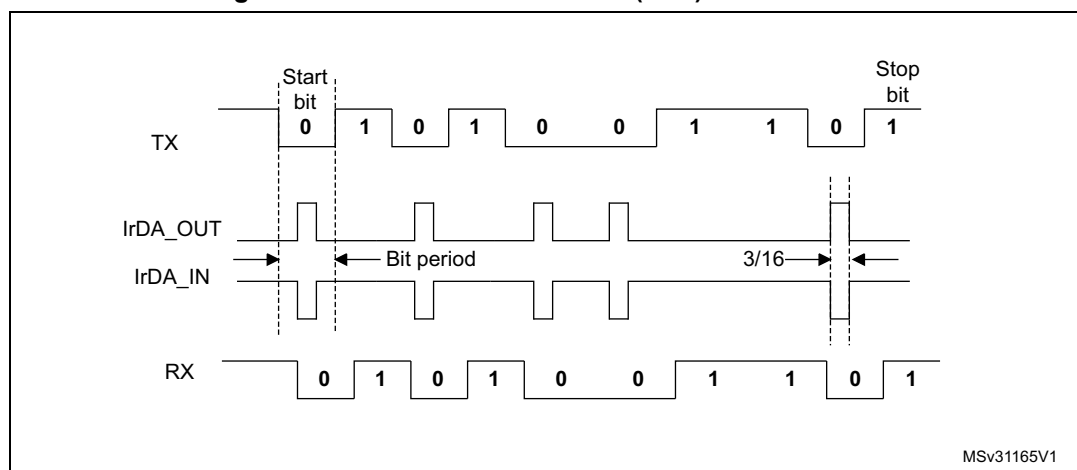
Figure 190. IrDA data modulation (3/16) -Normal Mode
