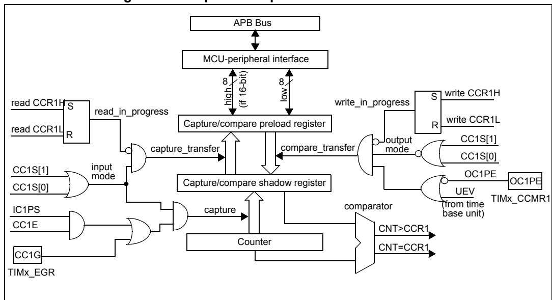
Figure 120. Capture/compare channel 1 main circuit
