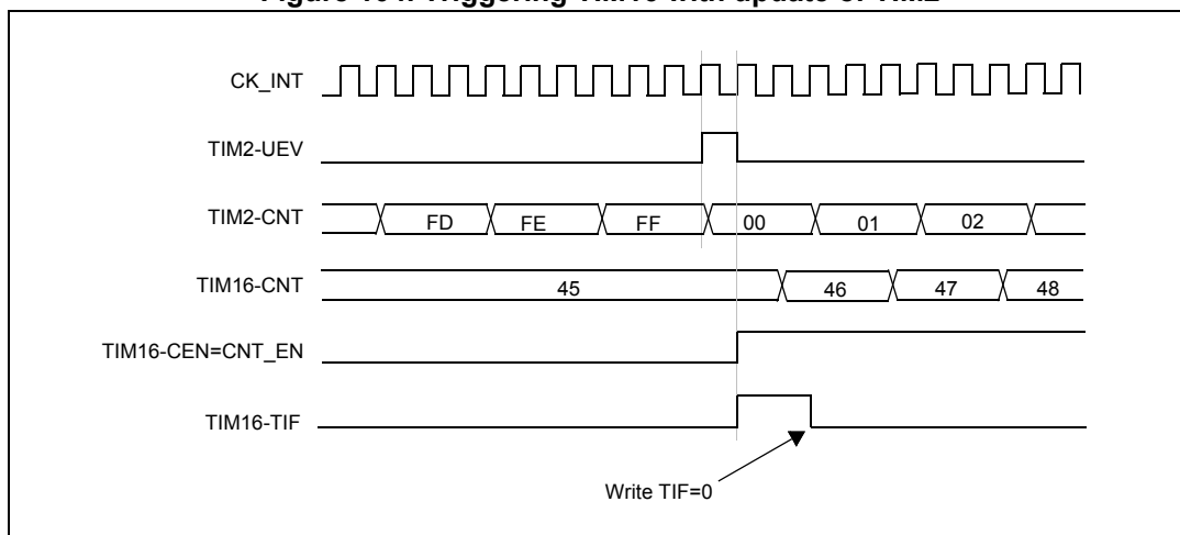
Figure 104. Triggering TIM16 with update of TIM2
