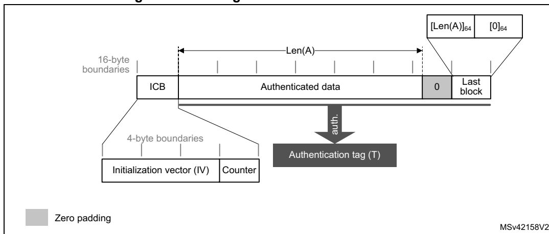
Figure 46. Message construction in GMAC mode
