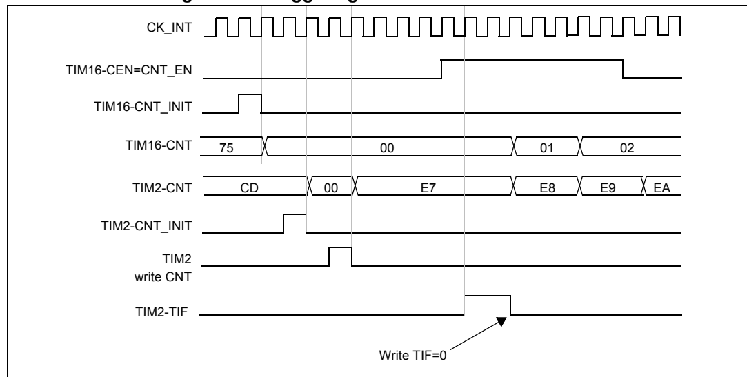
Figure 138. Triggering TIM2 with Enable of TIM16
