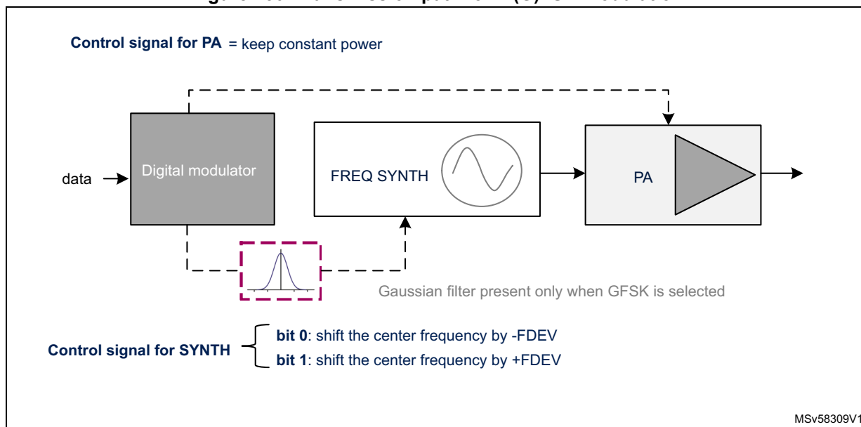
Figure 250. Transmission path for 2-(G)FSK modulation
