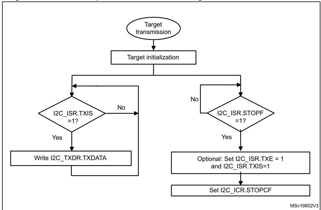
Figure 149. Transfer sequence flowchart for I2C target transmitter, NOSTRETCH=1
