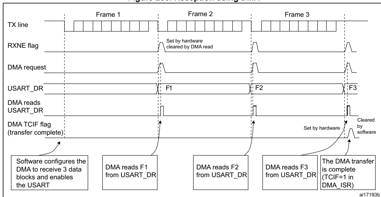
Figure 203. Reception using DMA
