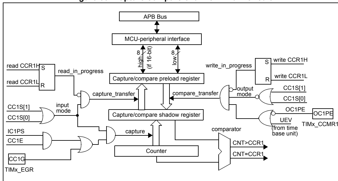
Figure 83. Capture/compare channel 1 main circuit
