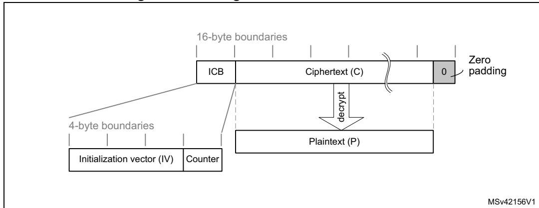
Figure 41. Message construction in CTR mode
