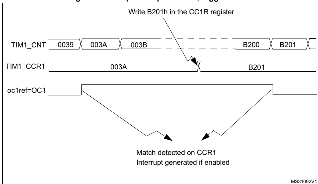
Figure 122. Output compare mode, toggle on OC1
