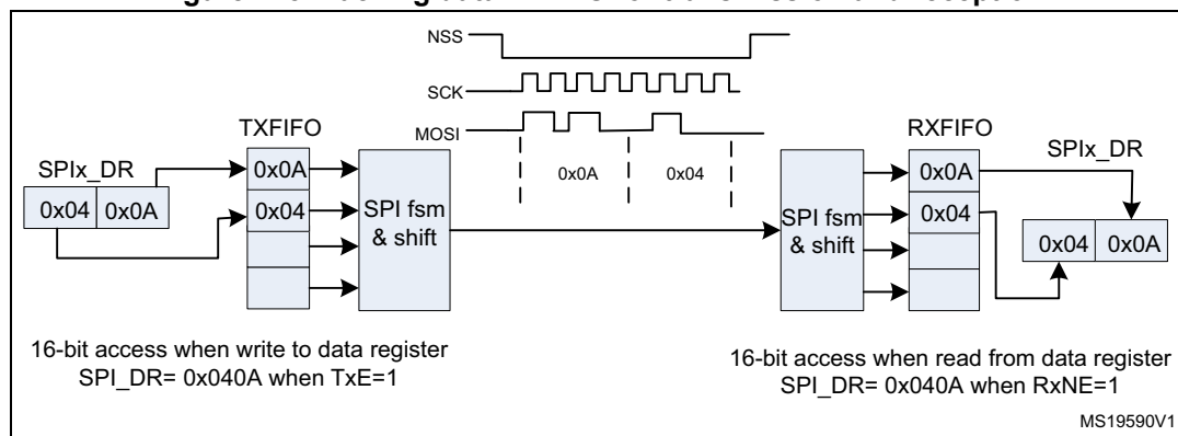
Figure 215. Packing data in FIFO for transmission and reception
