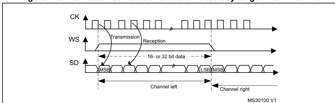
Figure 229. MSB Justified 16-bit or 32-bit full-accuracy length with CPOL = 0
