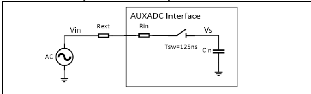
Figure 25. Effect of analog source resistance
