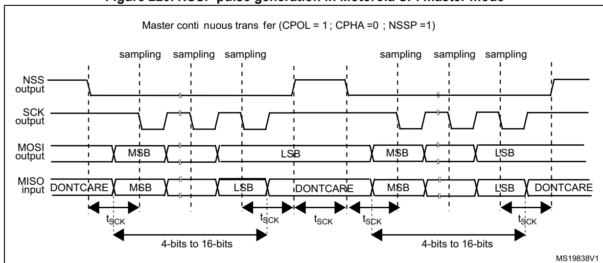
Figure 220. NSSP pulse generation in Motorola SPI master mode
