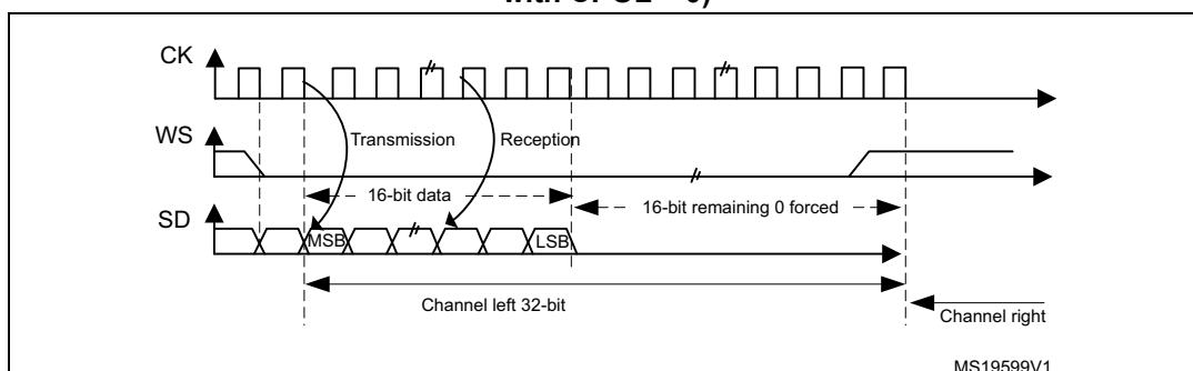
Figure 227. I 2 S Philips standard (16-bit extended to 32-bit packet frame with CPOL = 0)
