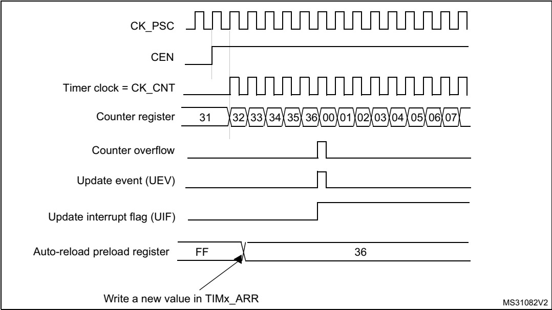
Figure 113. Counter timing diagram, update event when ARPE=0 (TIMx_ARR not preloaded)
