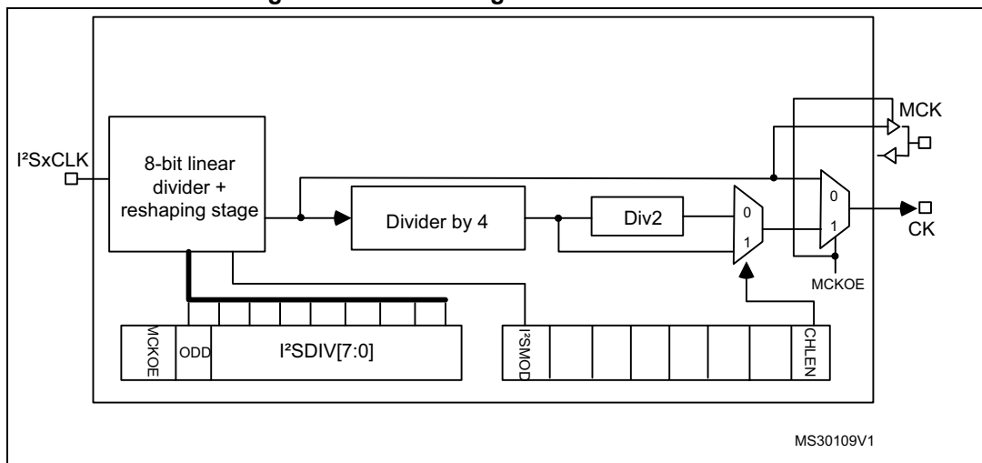
Figure 241. I 2 S clock generator architecture
