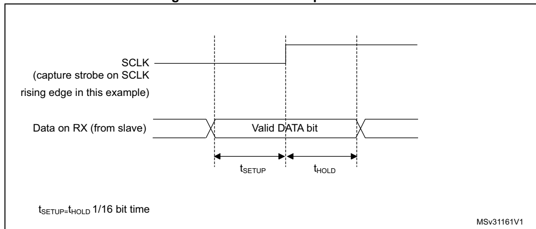
Figure 186. RX data setup/hold time
