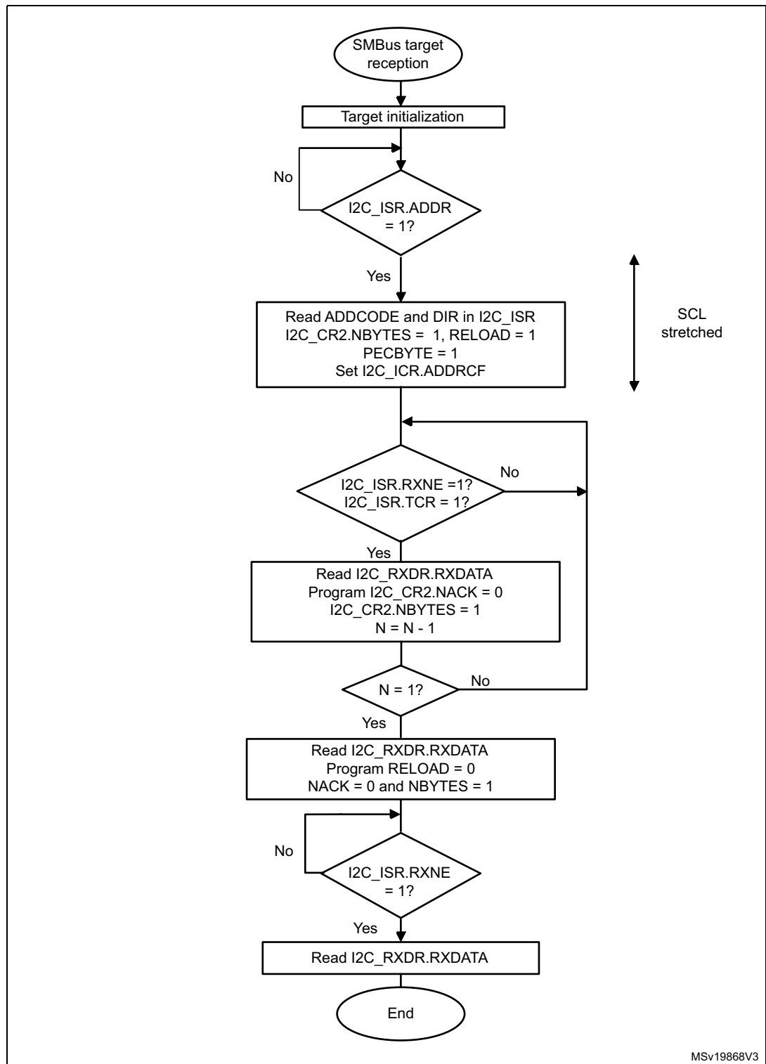
Figure 166. Transfer sequence flowchart for SMBus target receiver N Bytes + PEC
