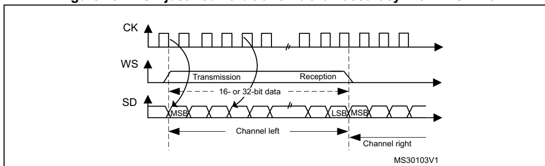
Figure 232. LSB justified 16-bit or 32-bit full-accuracy with CPOL = 0
