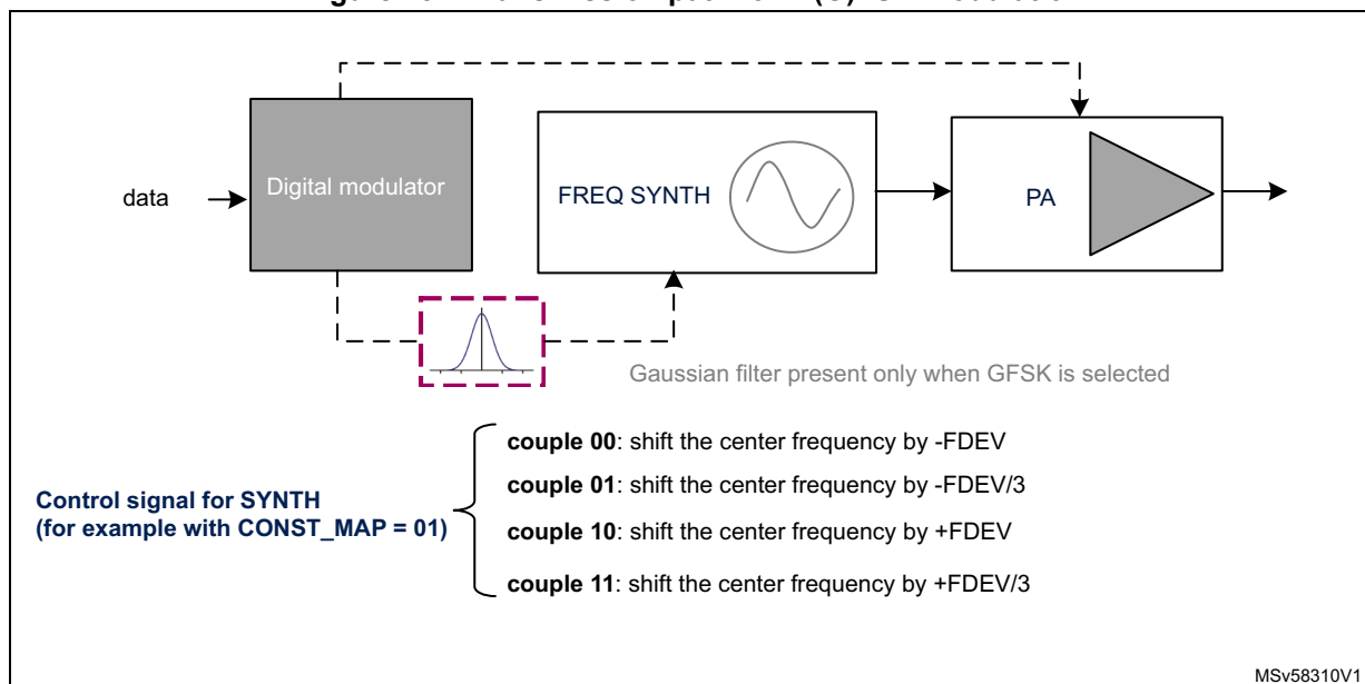
Figure 251. Transmission path for 4-(G)FSK modulation
