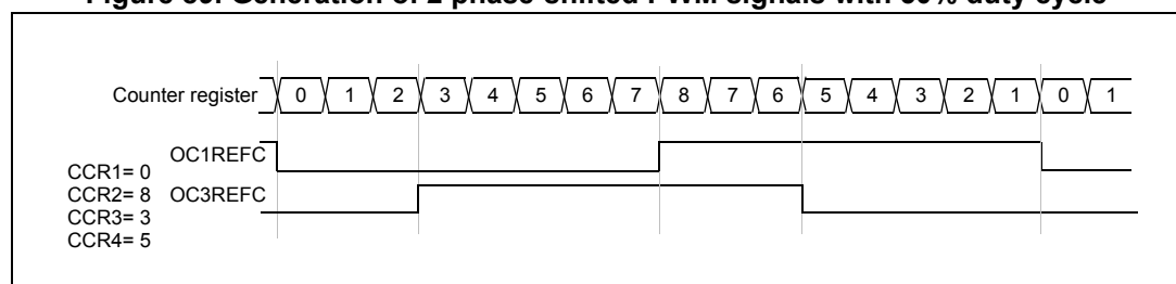
Figure 89. Generation of 2 phase-shifted PWM signals with 50% duty cycle
