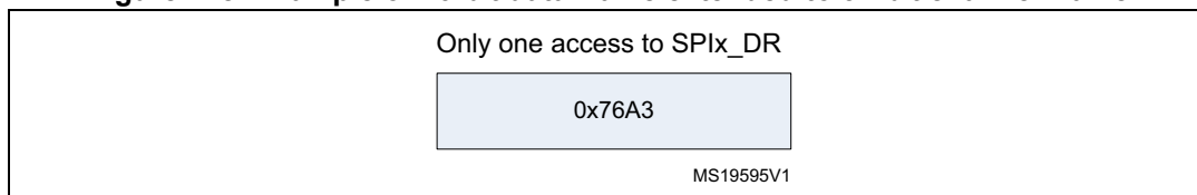
Figure 228. Example of 16-bit data frame extended to 32-bit channel frame
