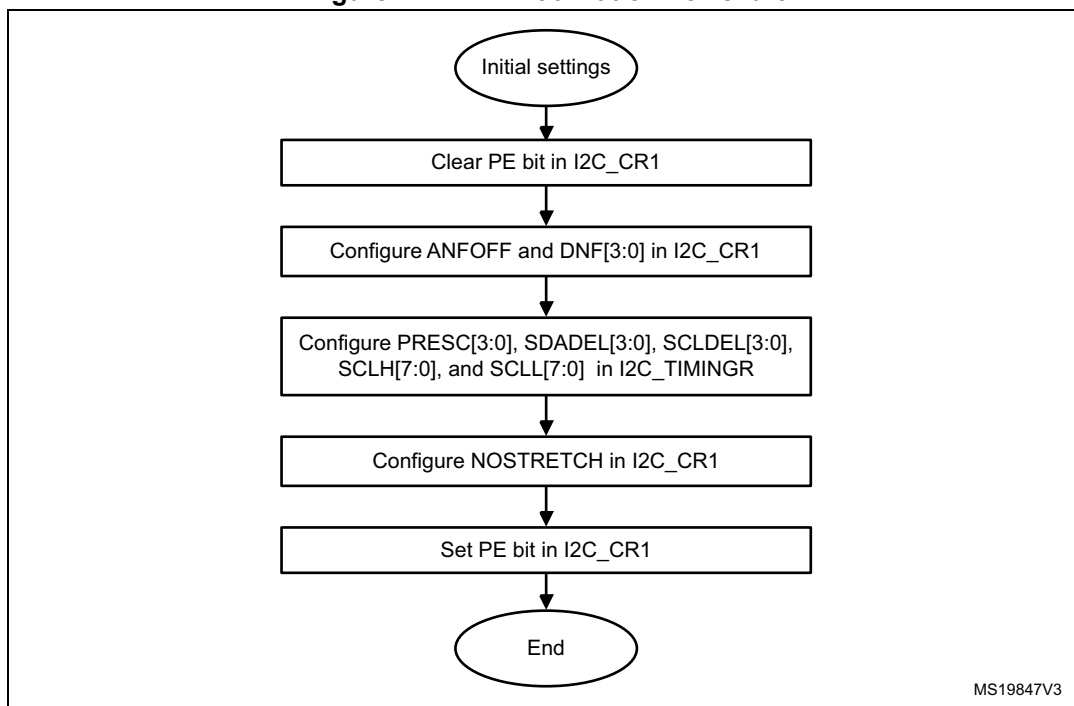
Figure 144. I2C initialization flowchart
