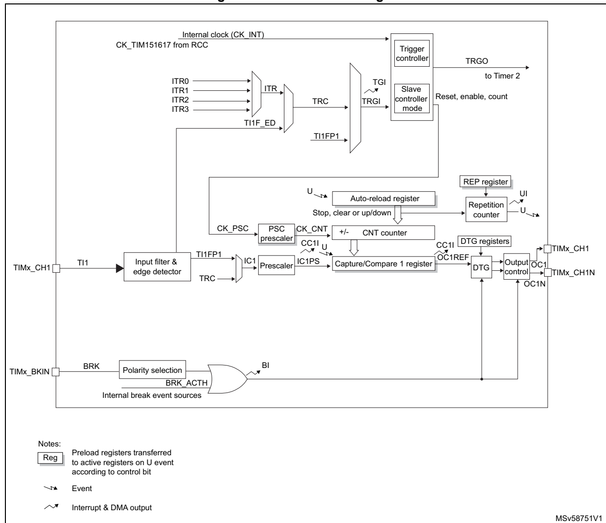
Figure 106. TIM16 block diagram
