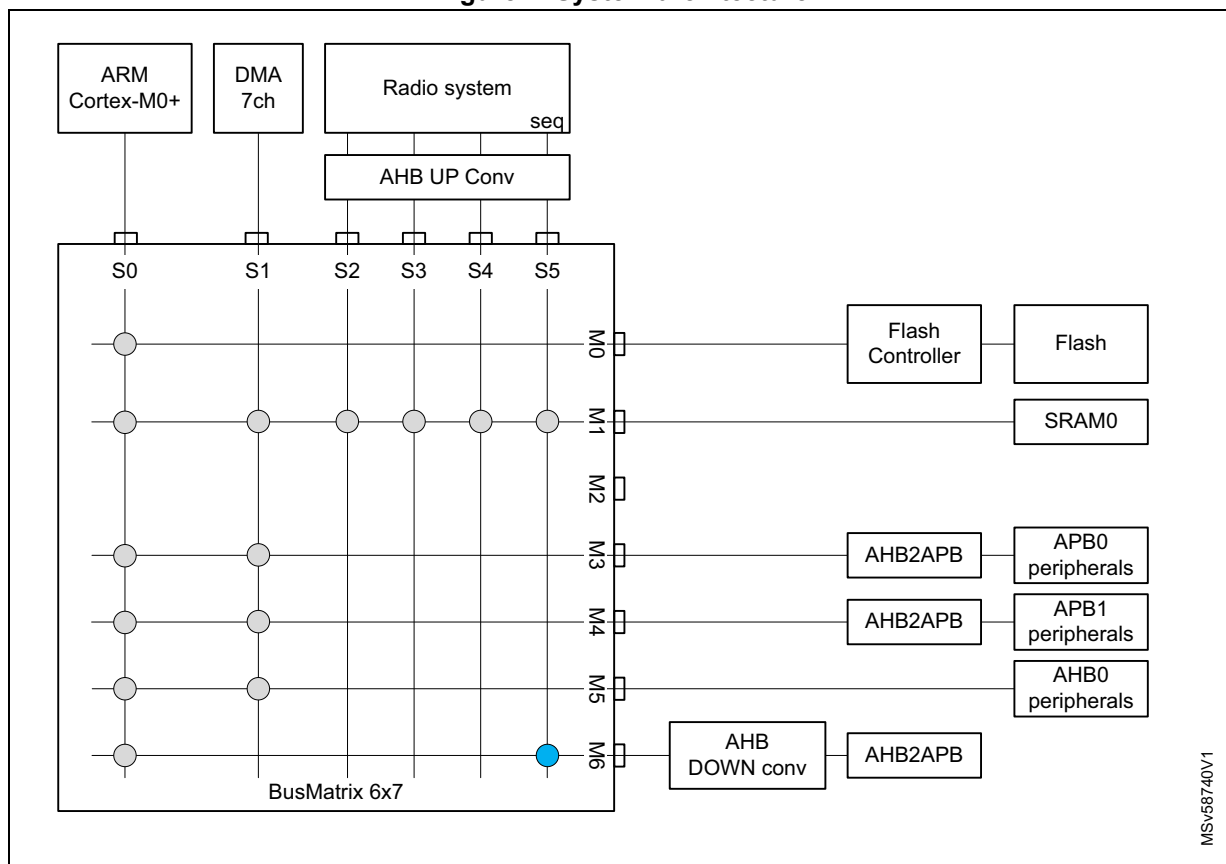
Figure 1. System architecture
