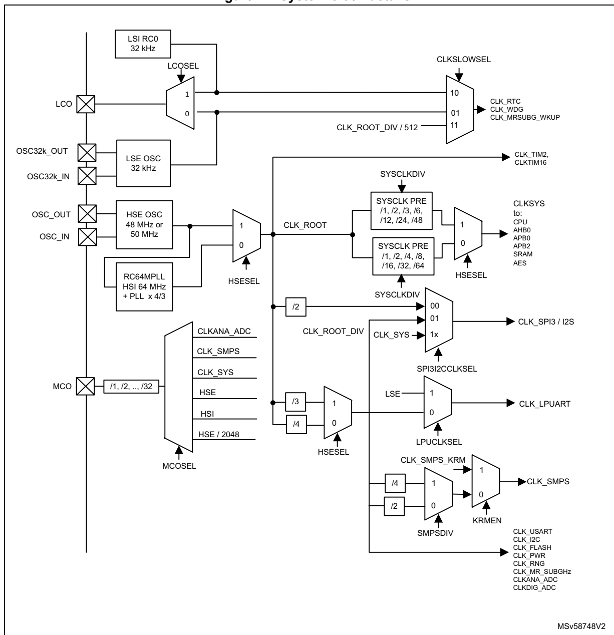
Figure 14. System clock details
