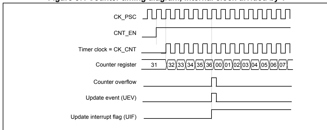
Figure 57. Counter timing diagram, internal clock divided by 1
