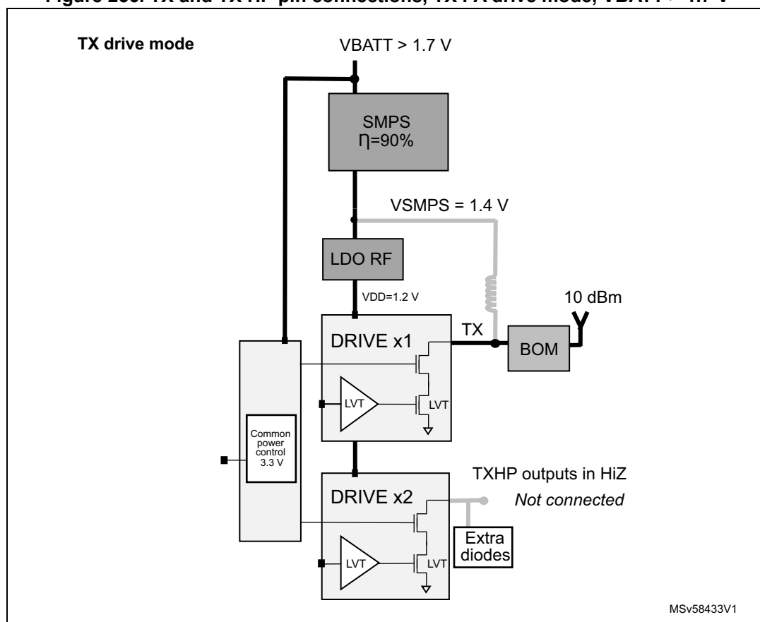
Figure 256. TX and TX HP pin connections, TX PA drive mode, VBATT > 1.7 V
