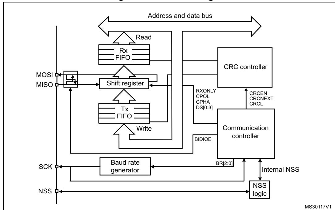
Figure 207. SPI block diagram
