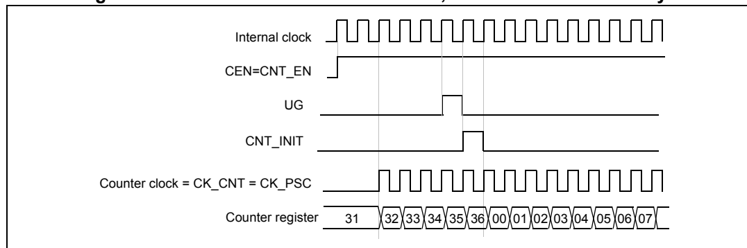
Figure 77. Control circuit in normal mode, internal clock divided by 1
