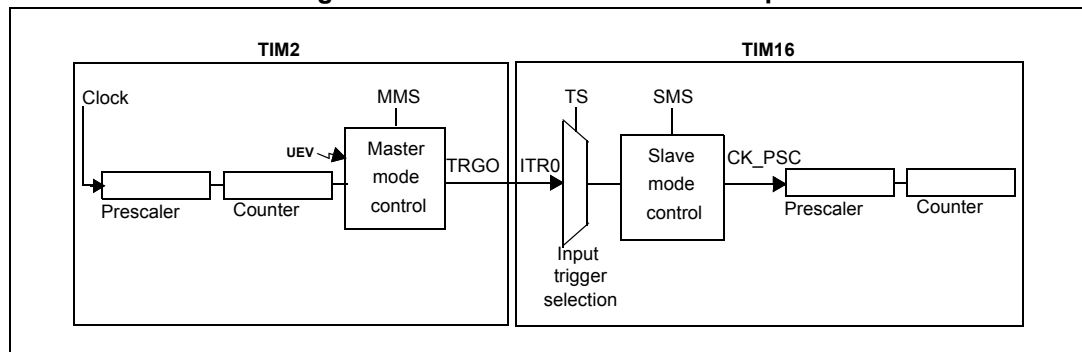
Figure 101. Master/slave timers example
