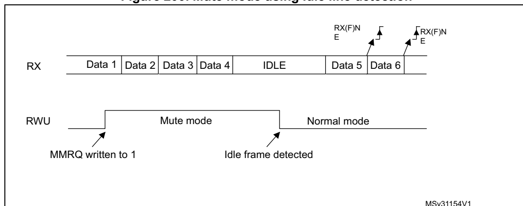
Figure 200. Mute mode using Idle line detection
