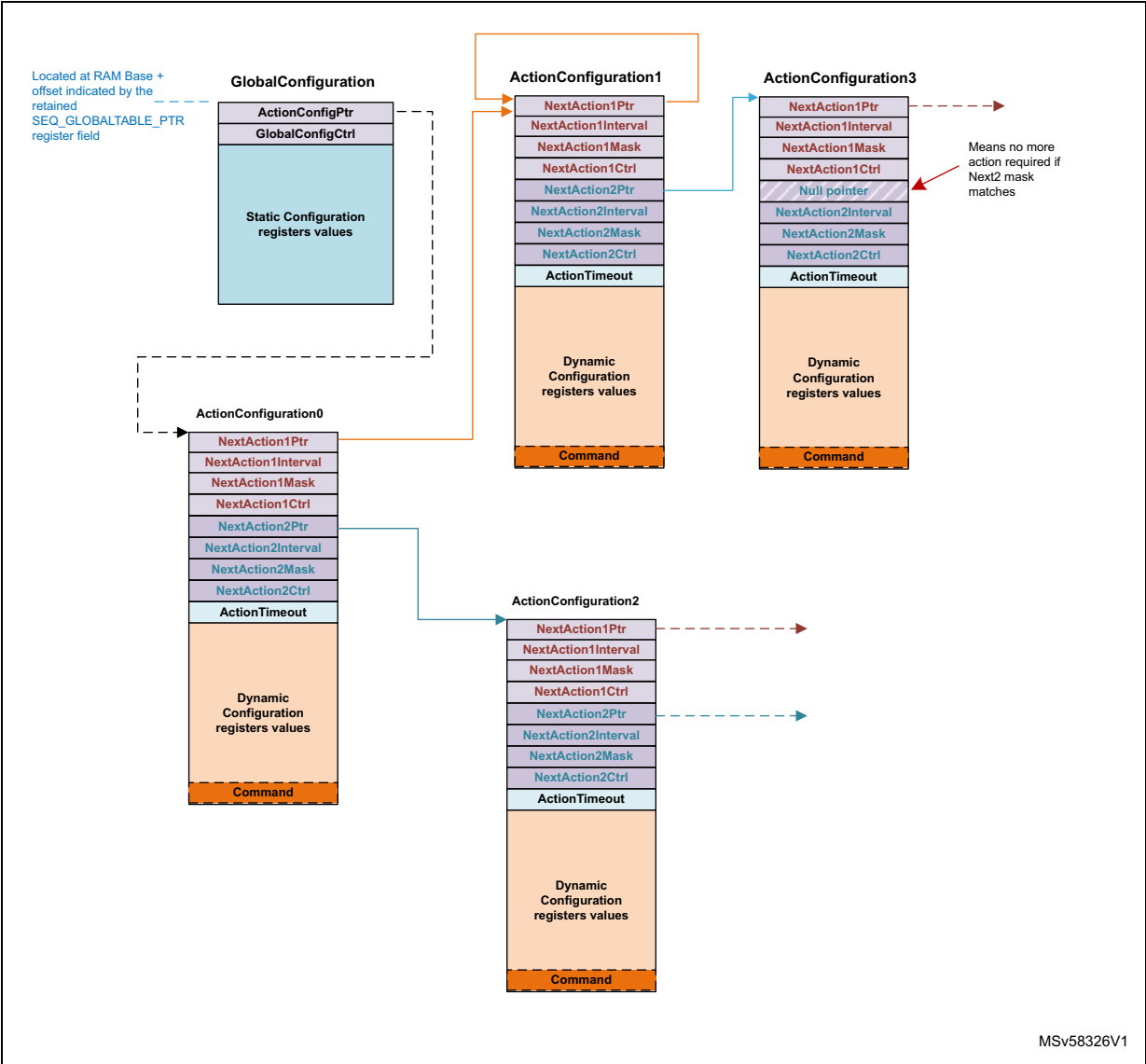
Figure 267. Sequencer actions list example
