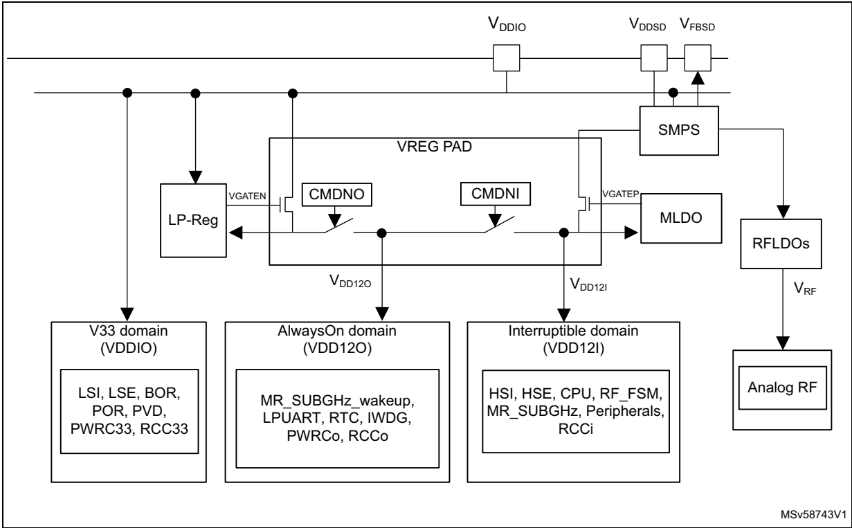
Figure 4. Power supply domain overview
