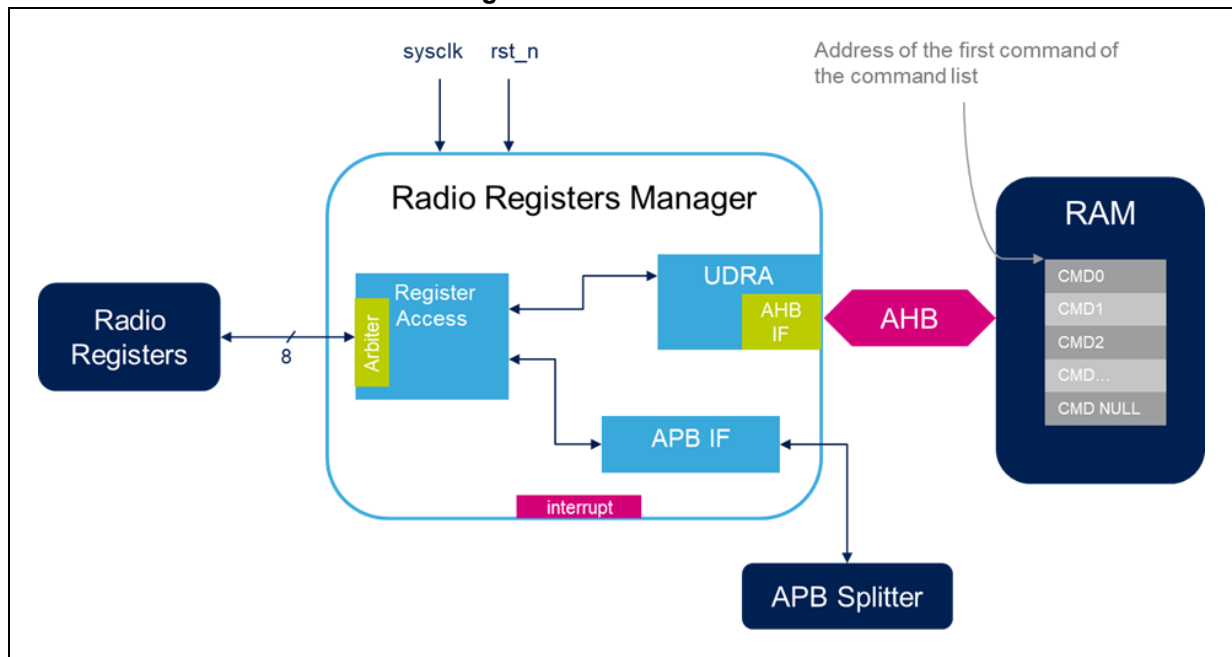
Figure 263. RRM overview
