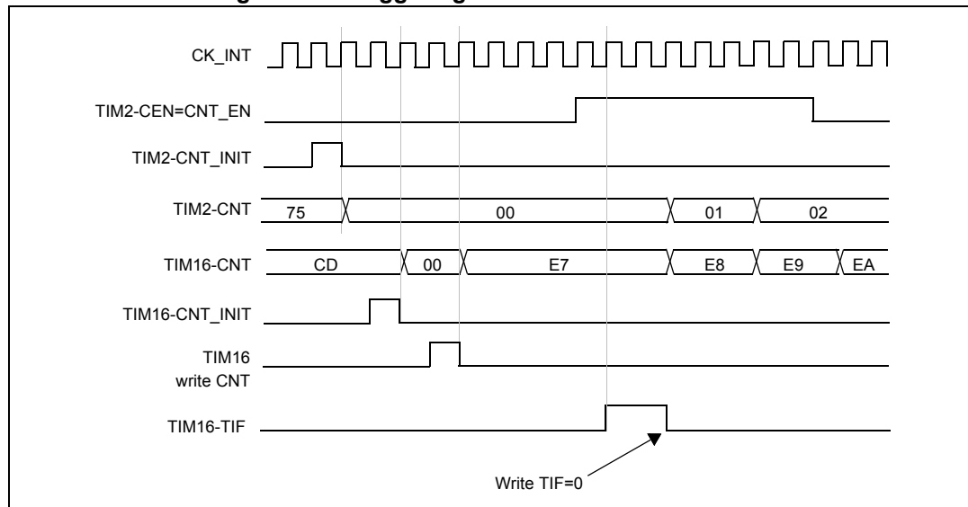
Figure 105. Triggering TIM16 with Enable of TIM2
