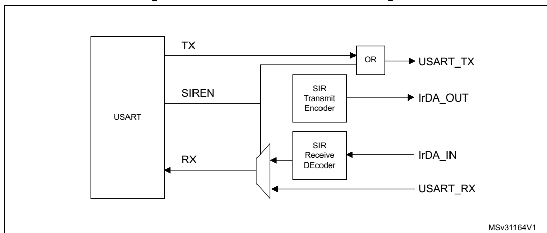
Figure 189. IrDA SIR ENDEC- block diagram
