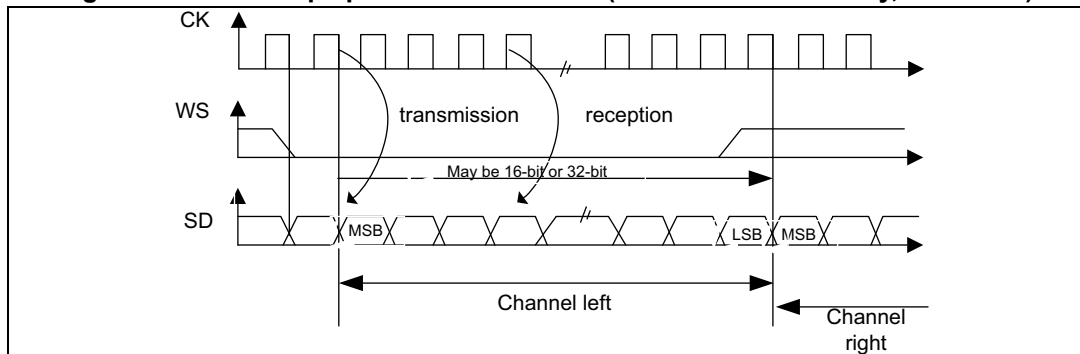
Figure 223. I 2 S Philips protocol waveforms (16/32-bit full accuracy, CPOL = 0)
