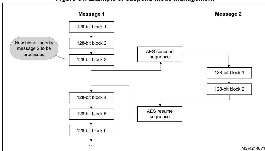
Figure 34. Example of suspend mode management
