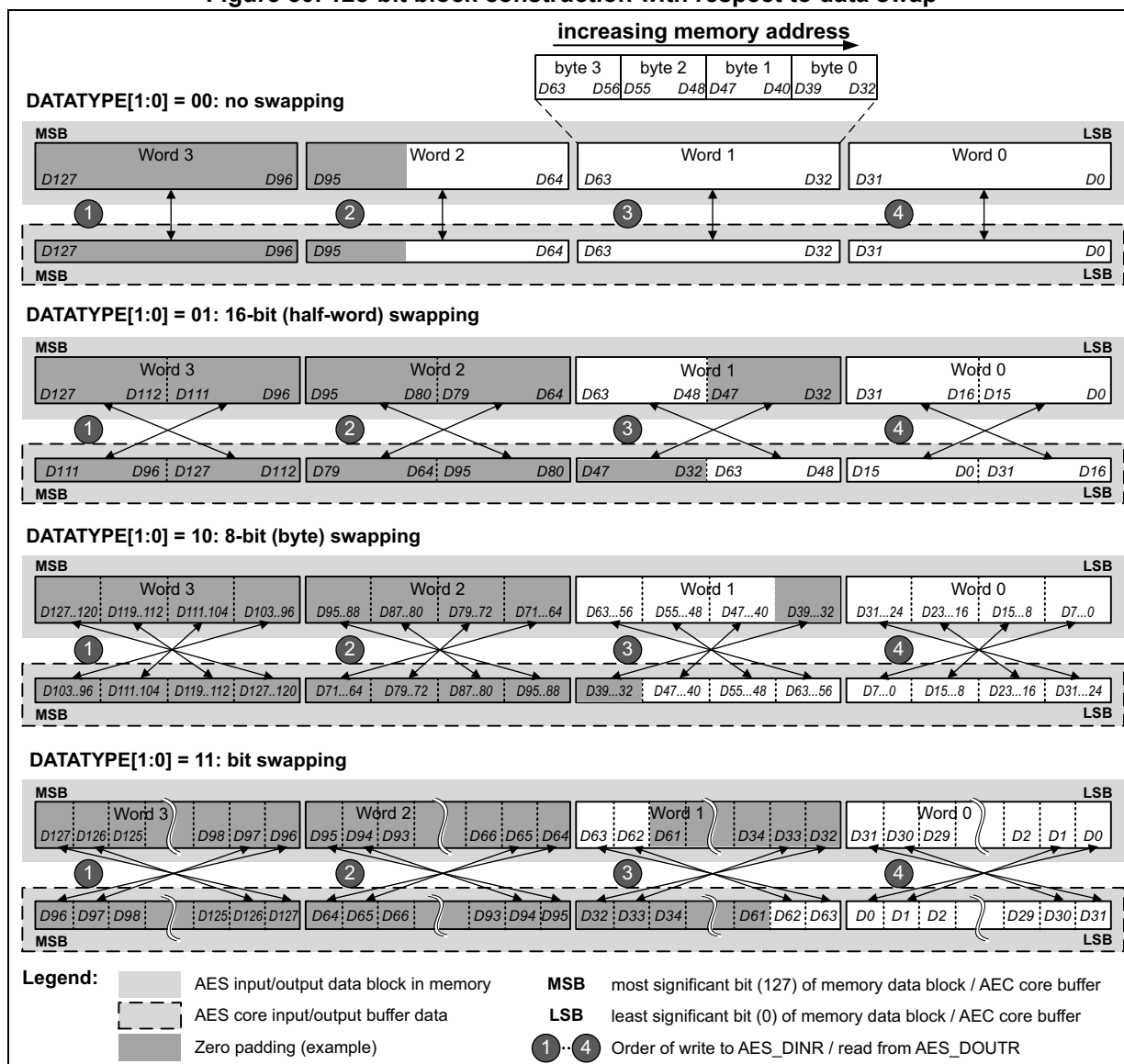
Figure 50. 128-bit block construction with respect to data swap
