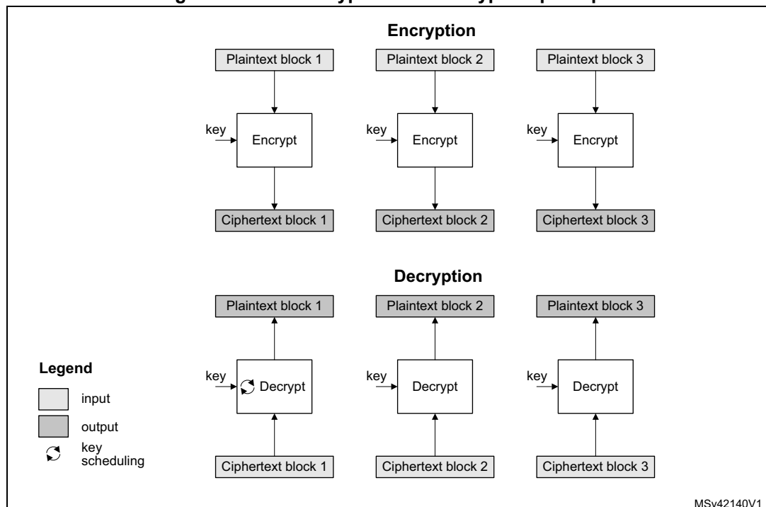
Figure 27. ECB encryption and decryption principle
