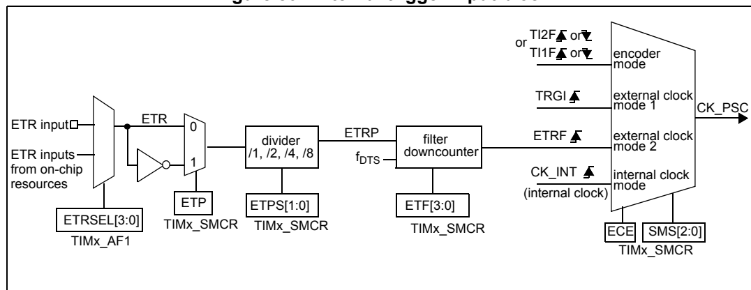
Figure 80. External trigger input block
