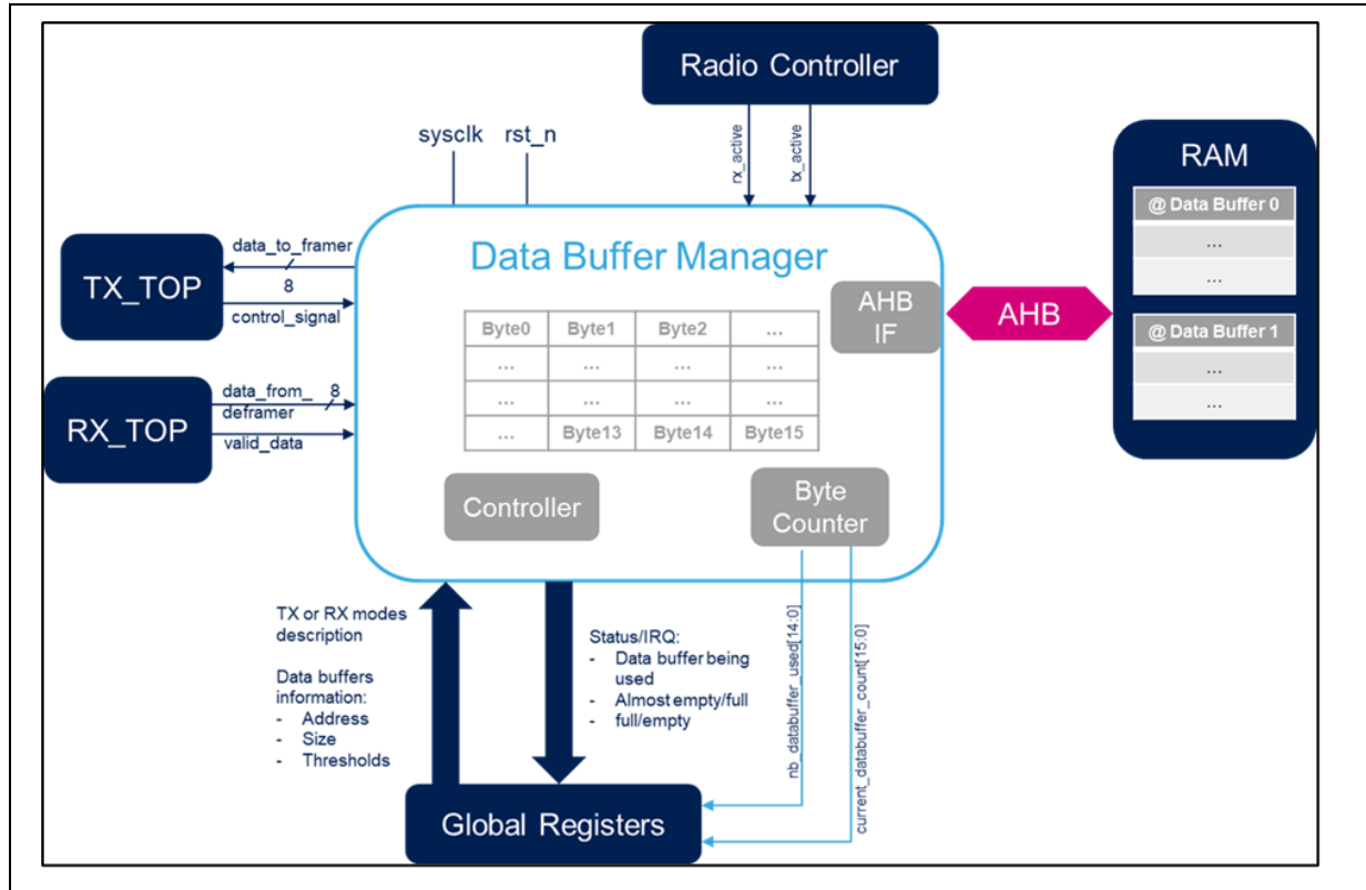
Figure 266. Data Buffer Manager overview
