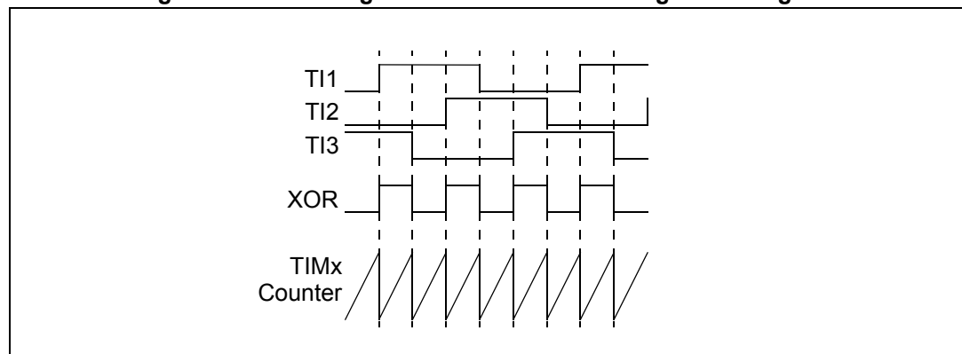
Figure 96. Measuring time interval between edges on 3 signals
