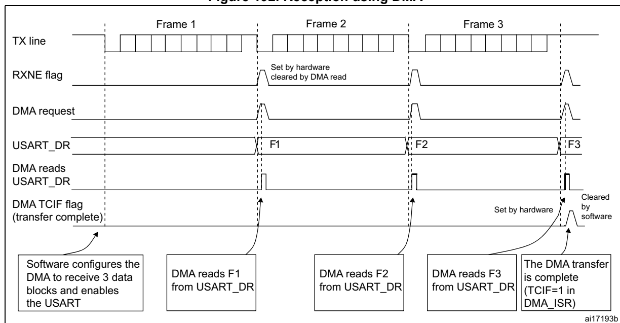
Figure 192. Reception using DMA
