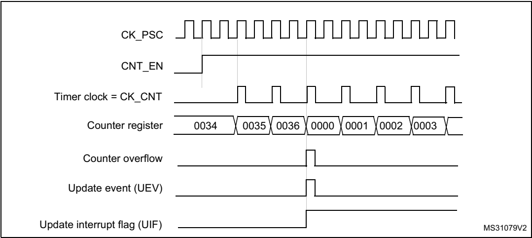
Figure 110. Counter timing diagram, internal clock divided by 2
