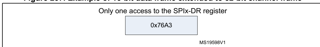
Figure 237. Example of 16-bit data frame extended to 32-bit channel frame
