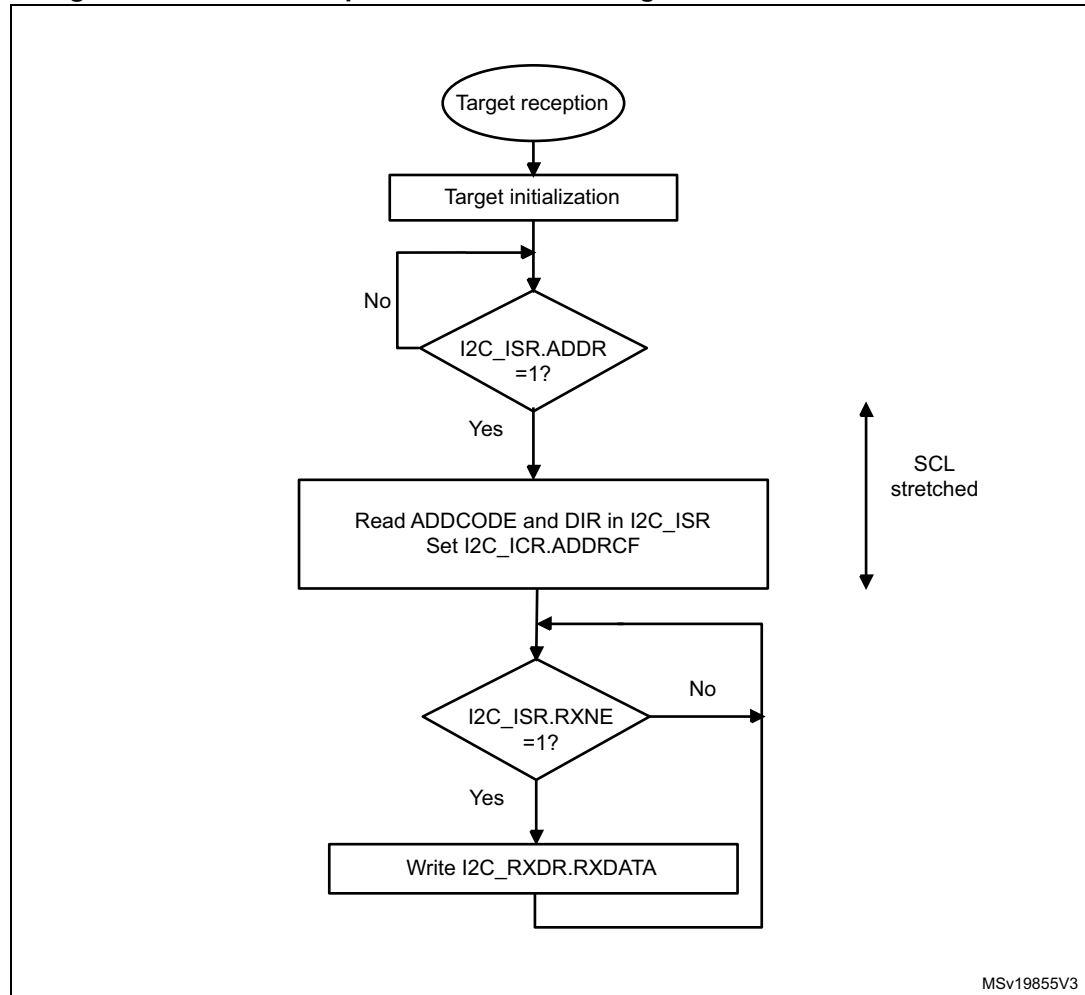
Figure 151. Transfer sequence flowchart for target receiver with NOSTRETCH=0
