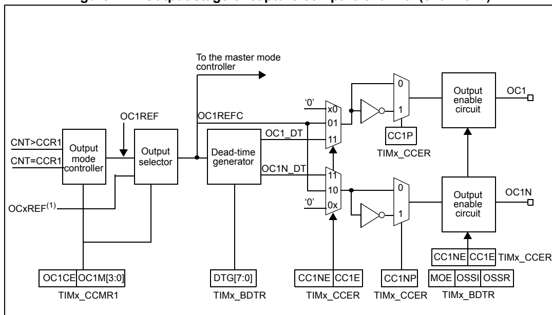
Figure 121. Output stage of capture/compare channel (channel 1)
