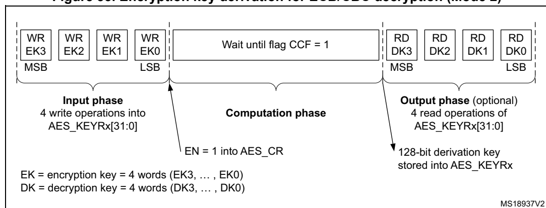
Figure 33. Encryption key derivation for ECB/CBC decryption (Mode 2)
