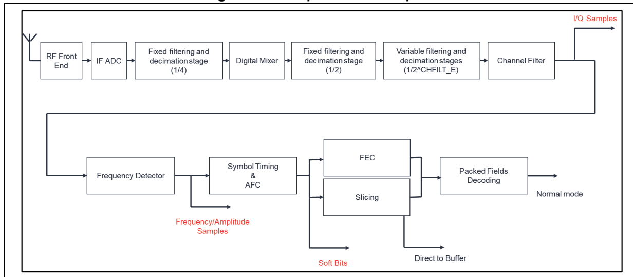
Figure 255. Simplified RX data path
