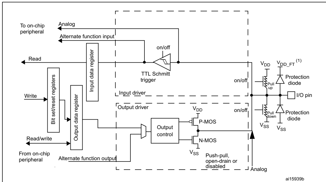
Figure 16. Basic structure of a mixed analog/digital five-volt tolerant I/O port bit
