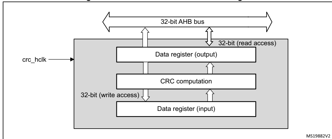
Figure 53. CRC calculation unit block diagram
