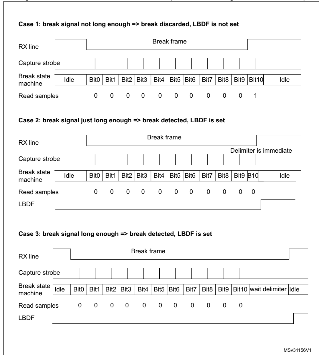
Figure 181. Break detection in LIN mode (11-bit break length - LBDL bit is set)
