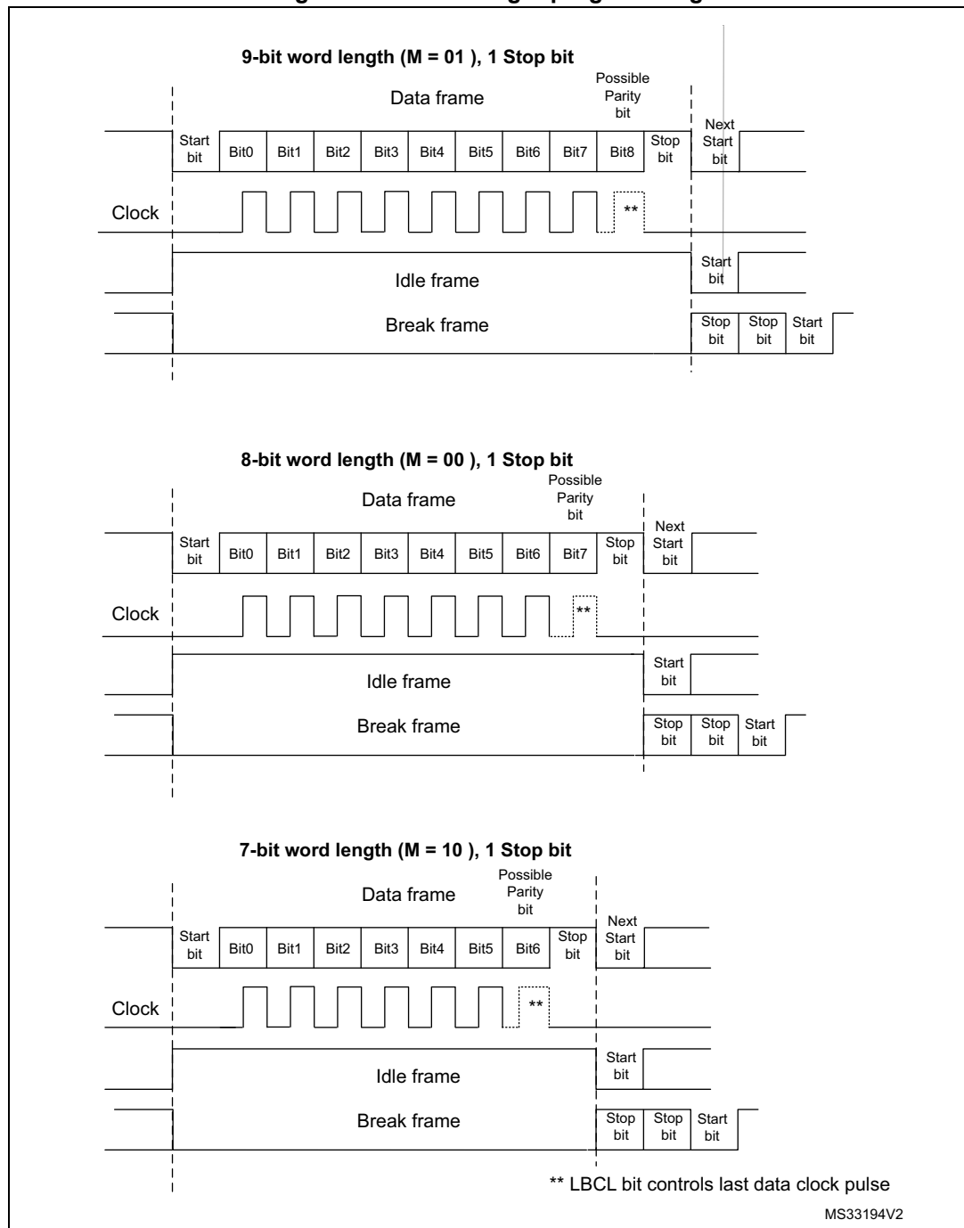
Figure 172. Word length programming
