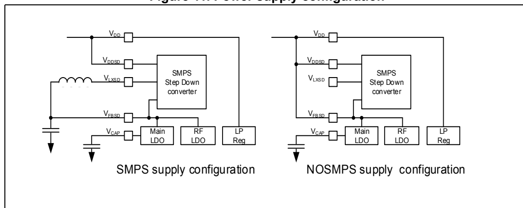
Figure 11. Power supply configuration
