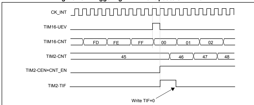
Figure 137. Triggering TIM2 with update of TIM16
