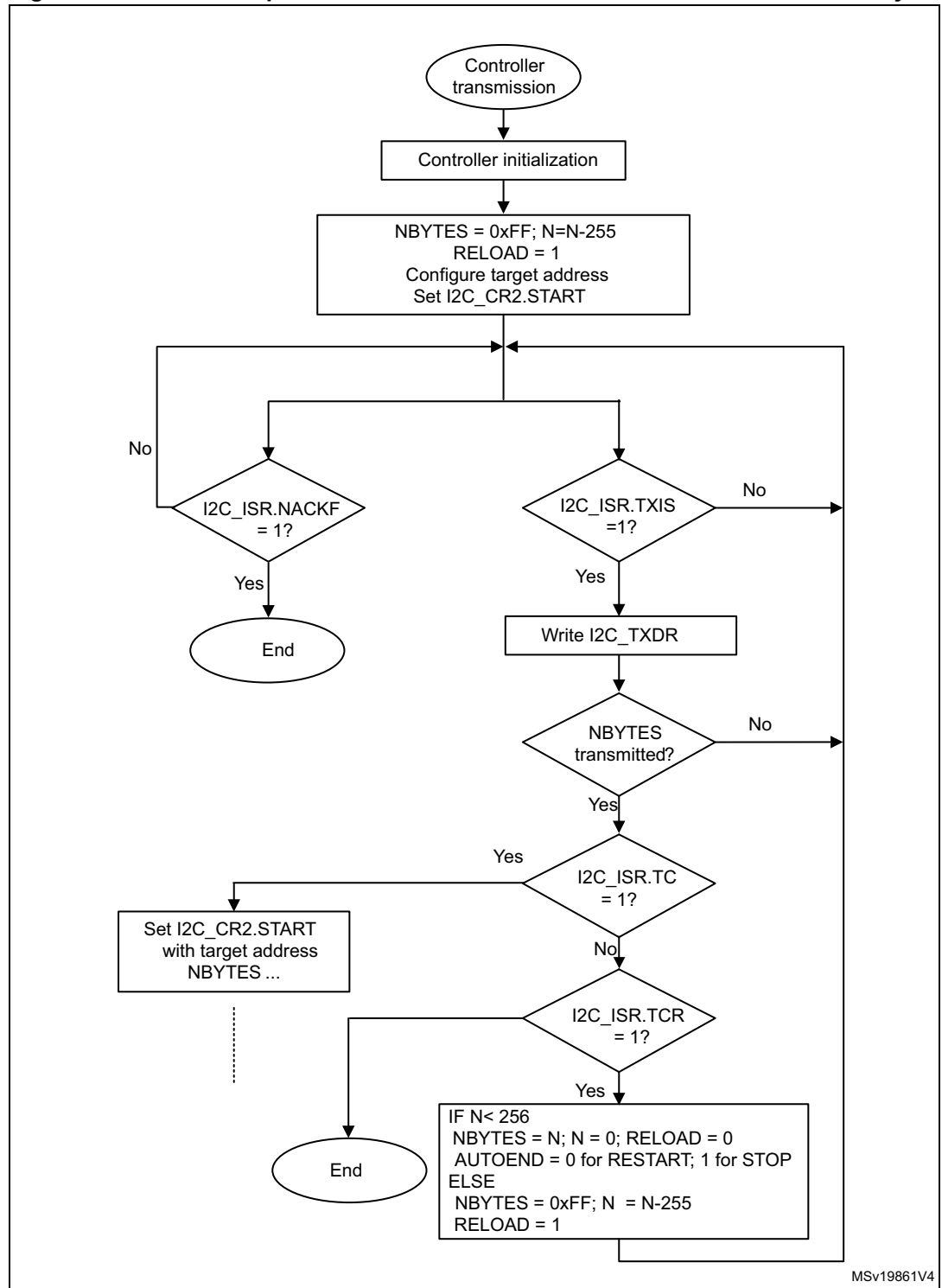
Figure 158. Transfer sequence flowchart for I2C controller transmitter for N&gt;255 bytes
