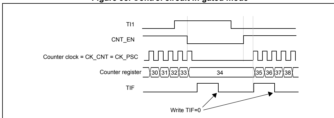
Figure 98. Control circuit in gated mode
