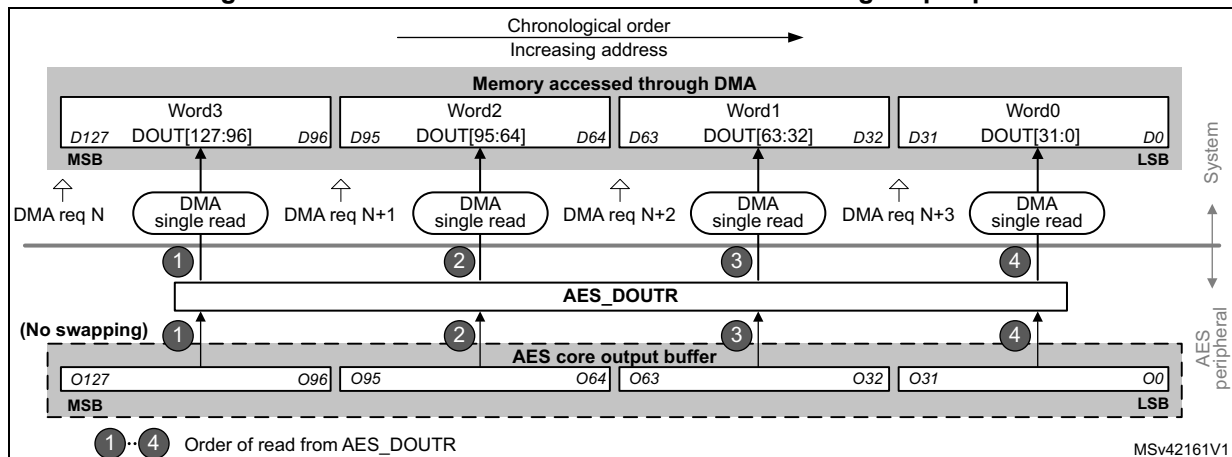
Figure 52. DMA transfer of a 128-bit data block during output phase
