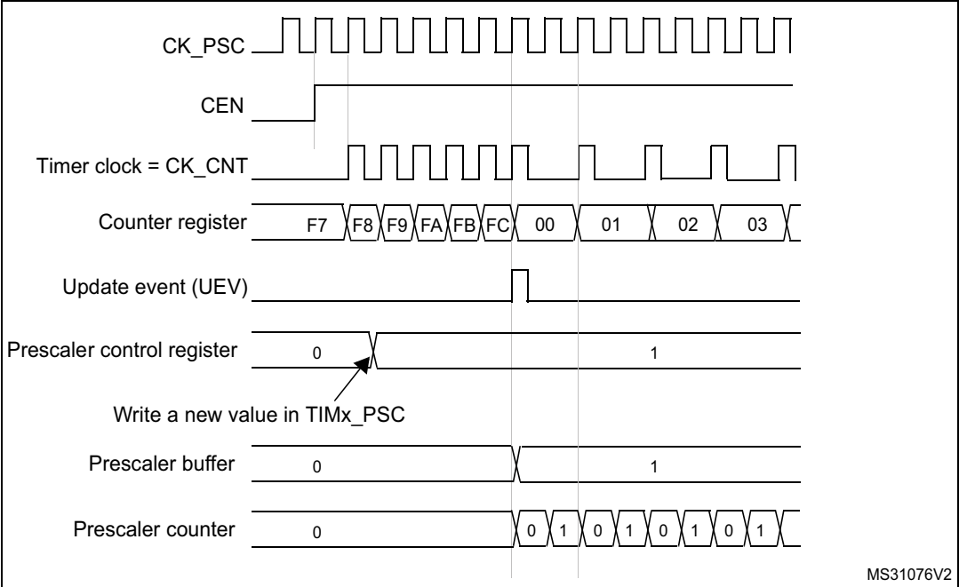
Figure 107. Counter timing diagram with prescaler division change from 1 to 2
