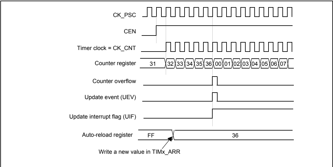
Figure 61. Counter timing diagram, update event when ARPE=0 (TIMx_ARR not preloaded)
