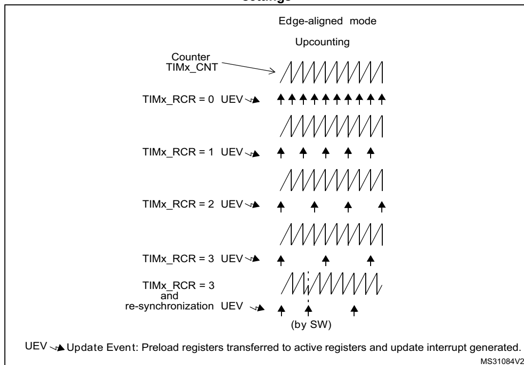
Figure 115. Update rate examples depending on mode and TIMx_RCR register settings
