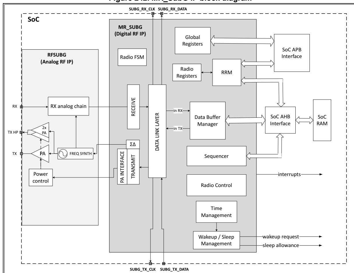
Figure 242. MR_SubG IP block diagram
