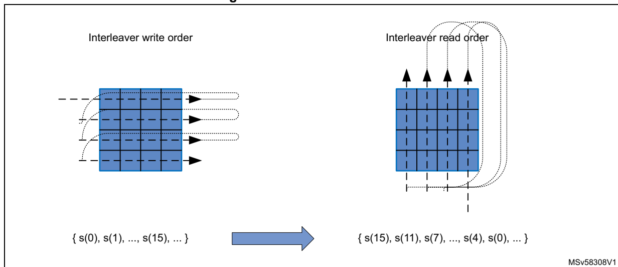
Figure 249. Interleave scheme
