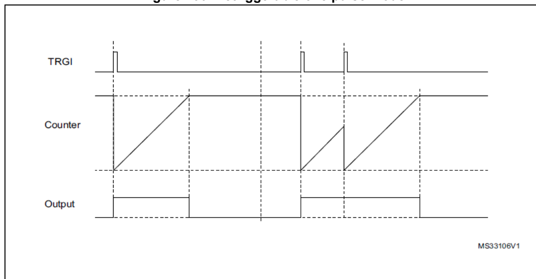
Figure 130. Retriggerable one pulse mode
