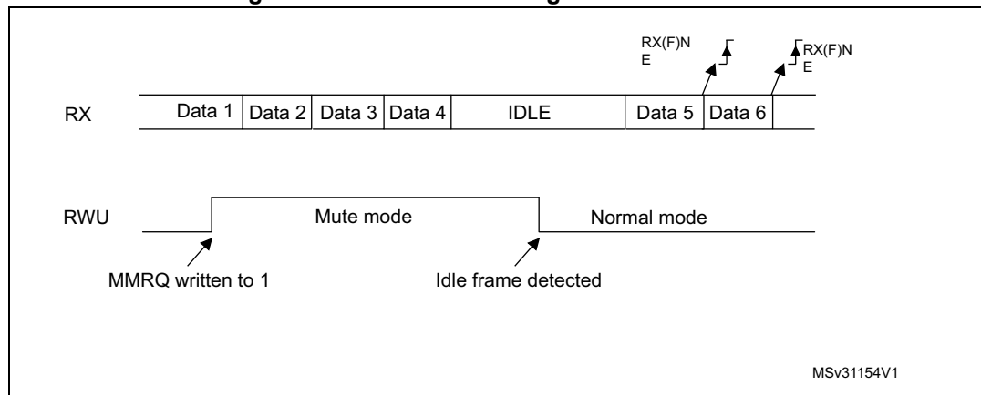
Figure 179. Mute mode using Idle line detection
