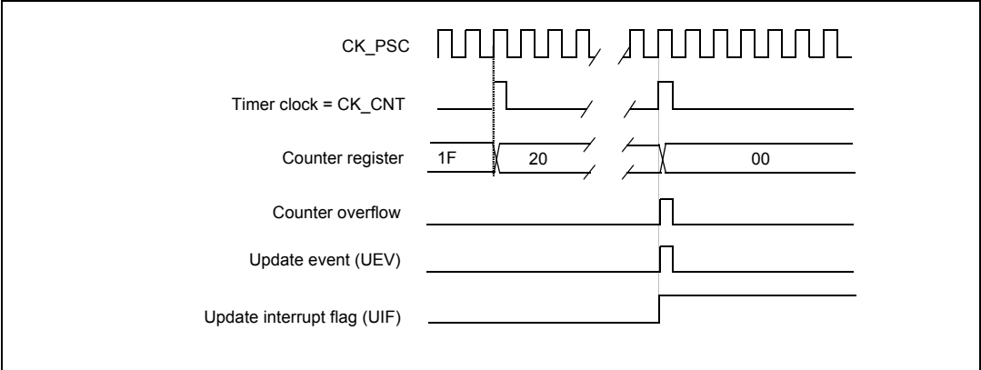
Figure 60. Counter timing diagram, internal clock divided by N
