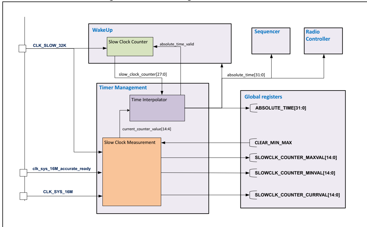
Figure 270. Time Management Unit overview
