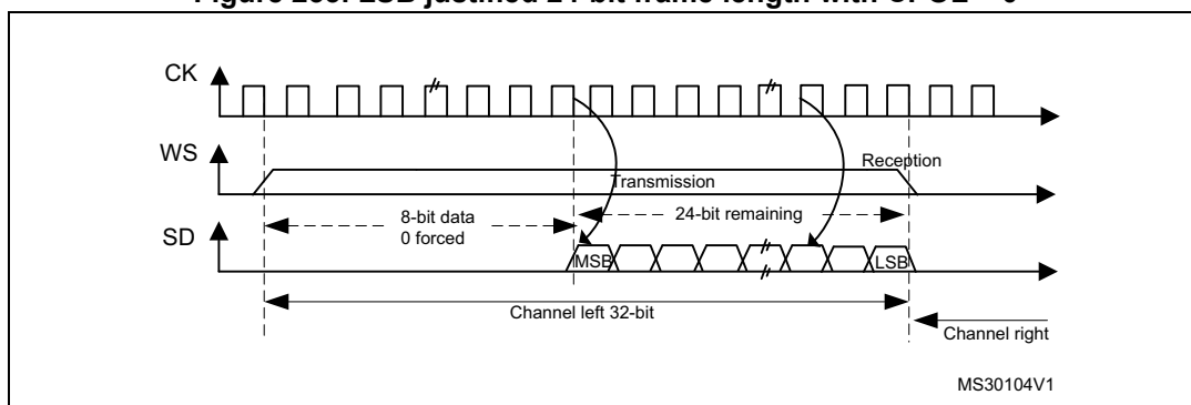
Figure 233. LSB justified 24-bit frame length with CPOL = 0
