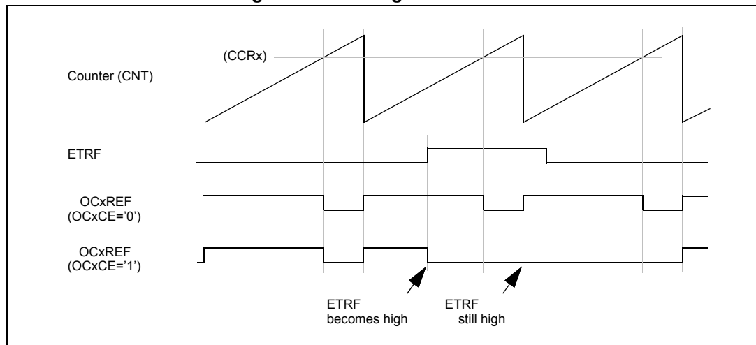
Figure 91. Clearing TIMx OCxREF
