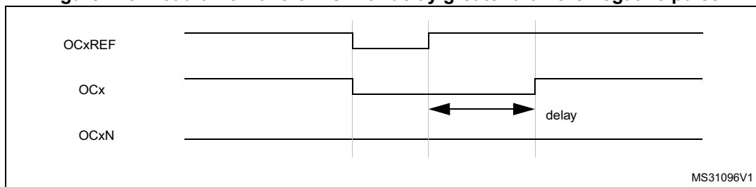
Figure 125. Dead-time waveforms with delay greater than the negative pulse.
