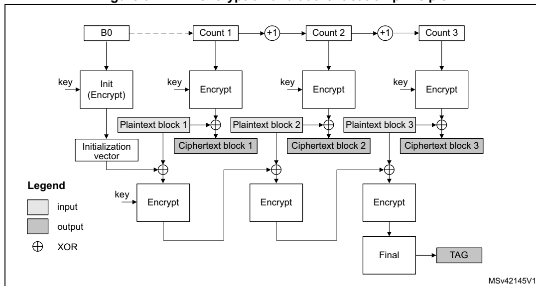
Figure 32. CCM encryption and authentication principle
