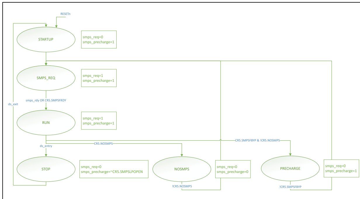
Figure 12. PWR SMPS state machine overview
