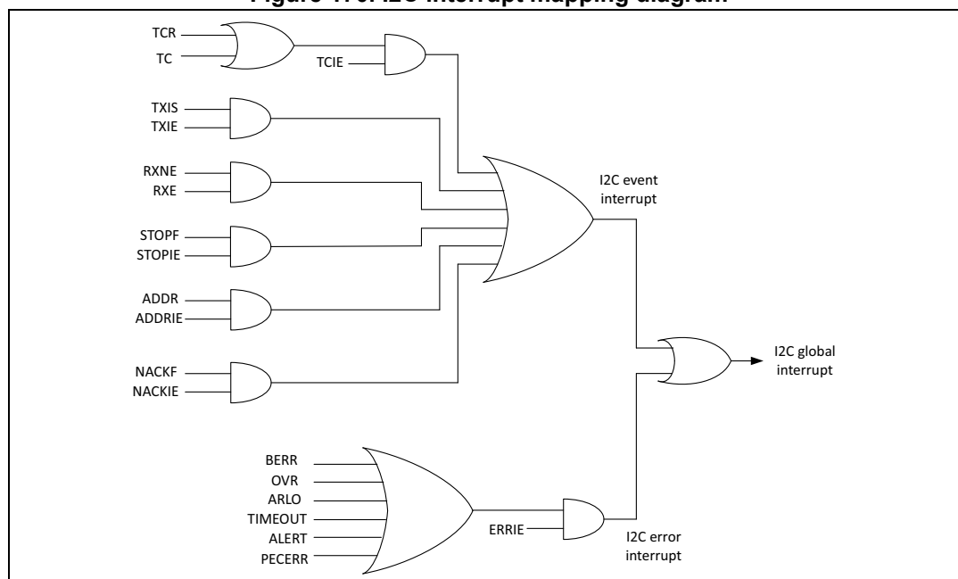
Figure 170. I2C interrupt mapping diagram
