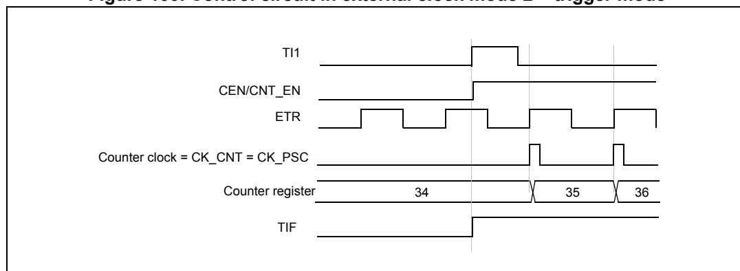
Figure 100. Control circuit in external clock mode 2 + trigger mode
