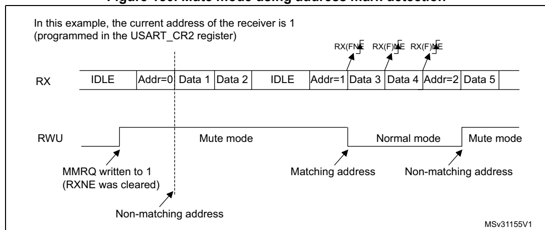
Figure 180. Mute mode using address mark detection
