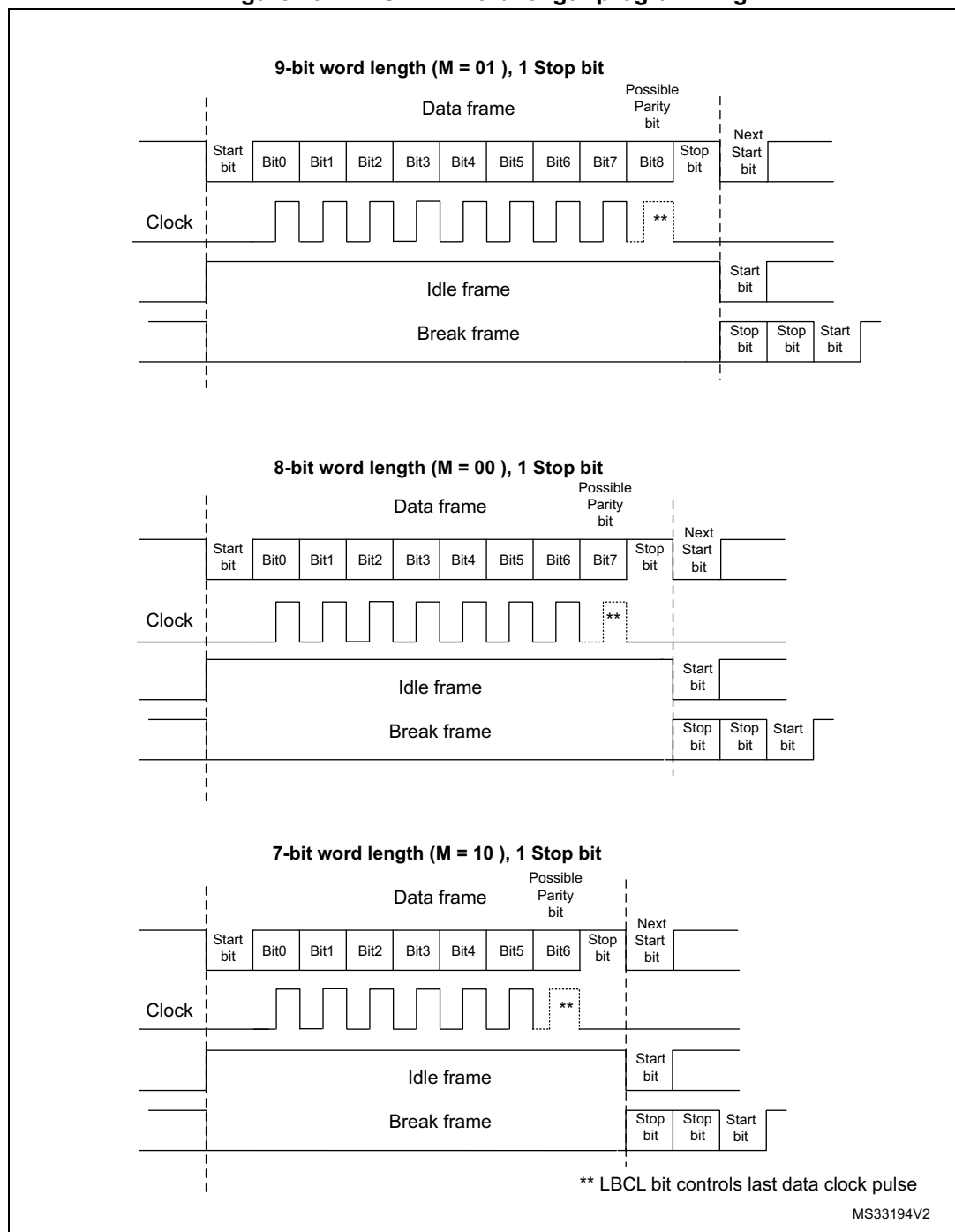
Figure 197. LPUART Word length programming
