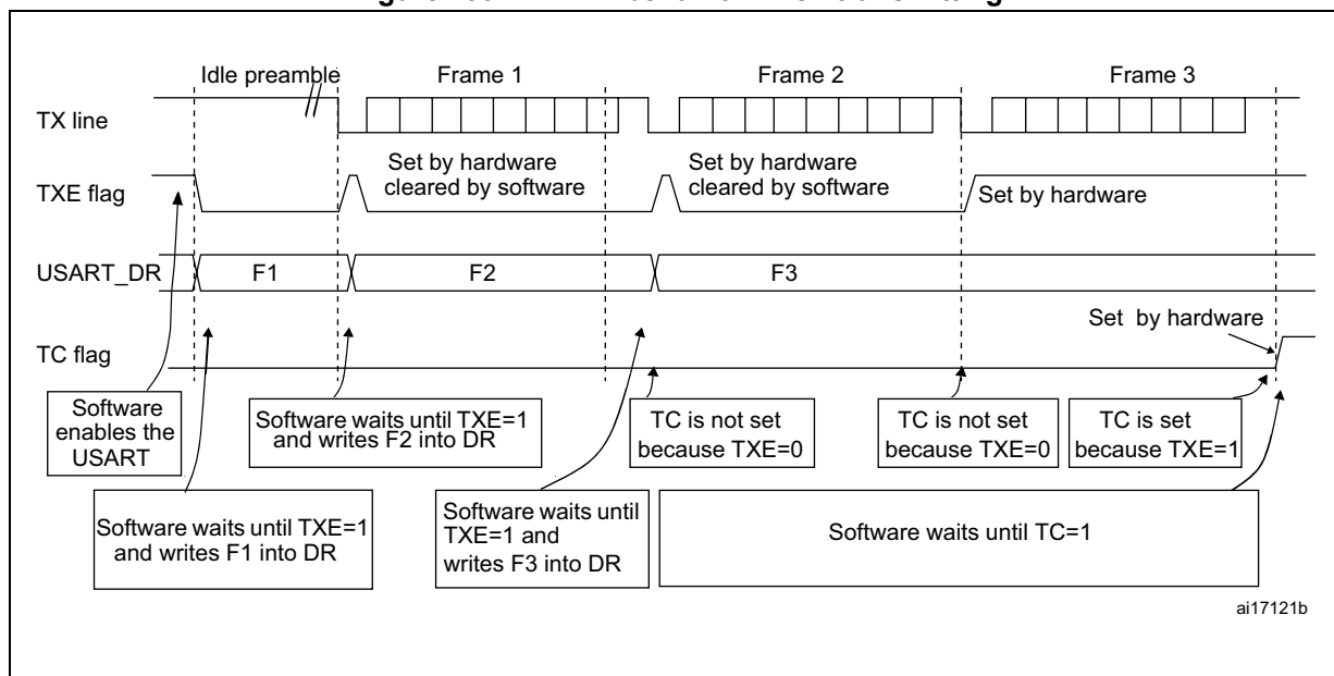
Figure 199. TC/TXE behavior when transmitting
