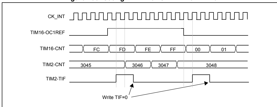
Figure 135. Gating TIM2 with OC1REF of TIM16
