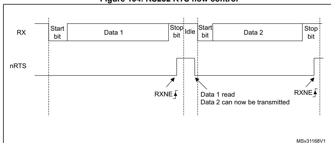
Figure 194. RS232 RTS flow control
