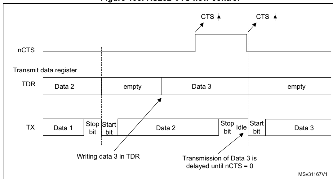
Figure 195. RS232 CTS flow control
