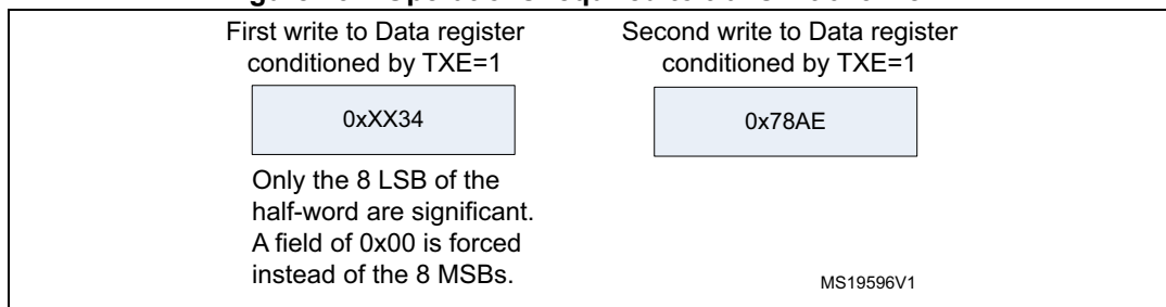
Figure 234. Operations required to transmit 0x3478AE
