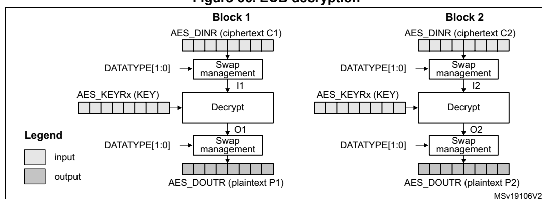
Figure 36. ECB decryption
