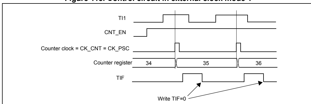
Figure 118. Control circuit in external clock mode 1
