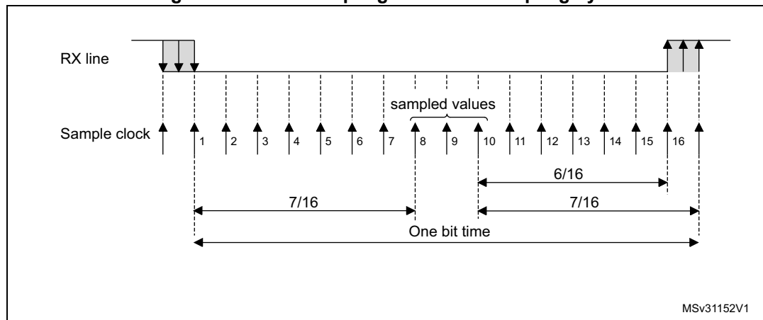
Figure 177. Data sampling when oversampling by 16
