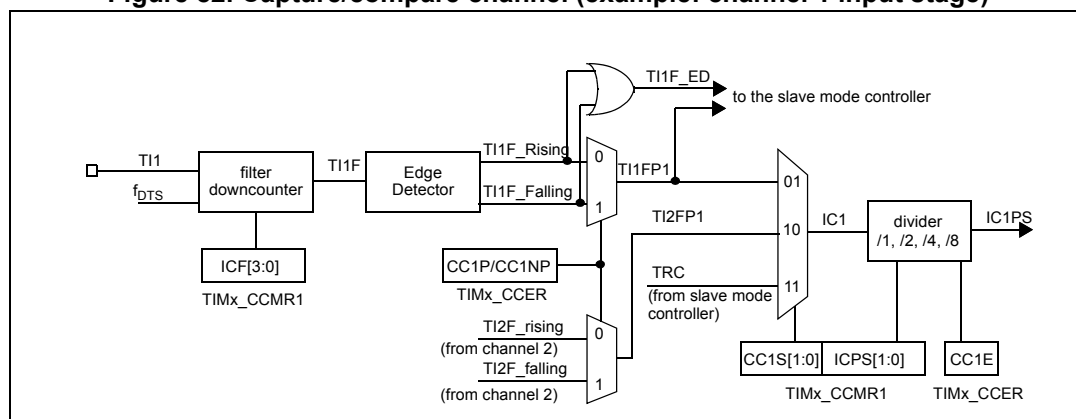
Figure 82. Capture/compare channel (example: channel 1 input stage)
