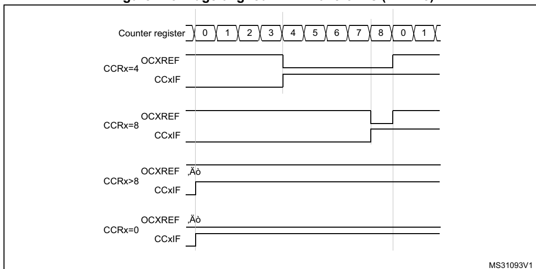
Figure 123. Edge-aligned PWM waveforms (ARR=8)
