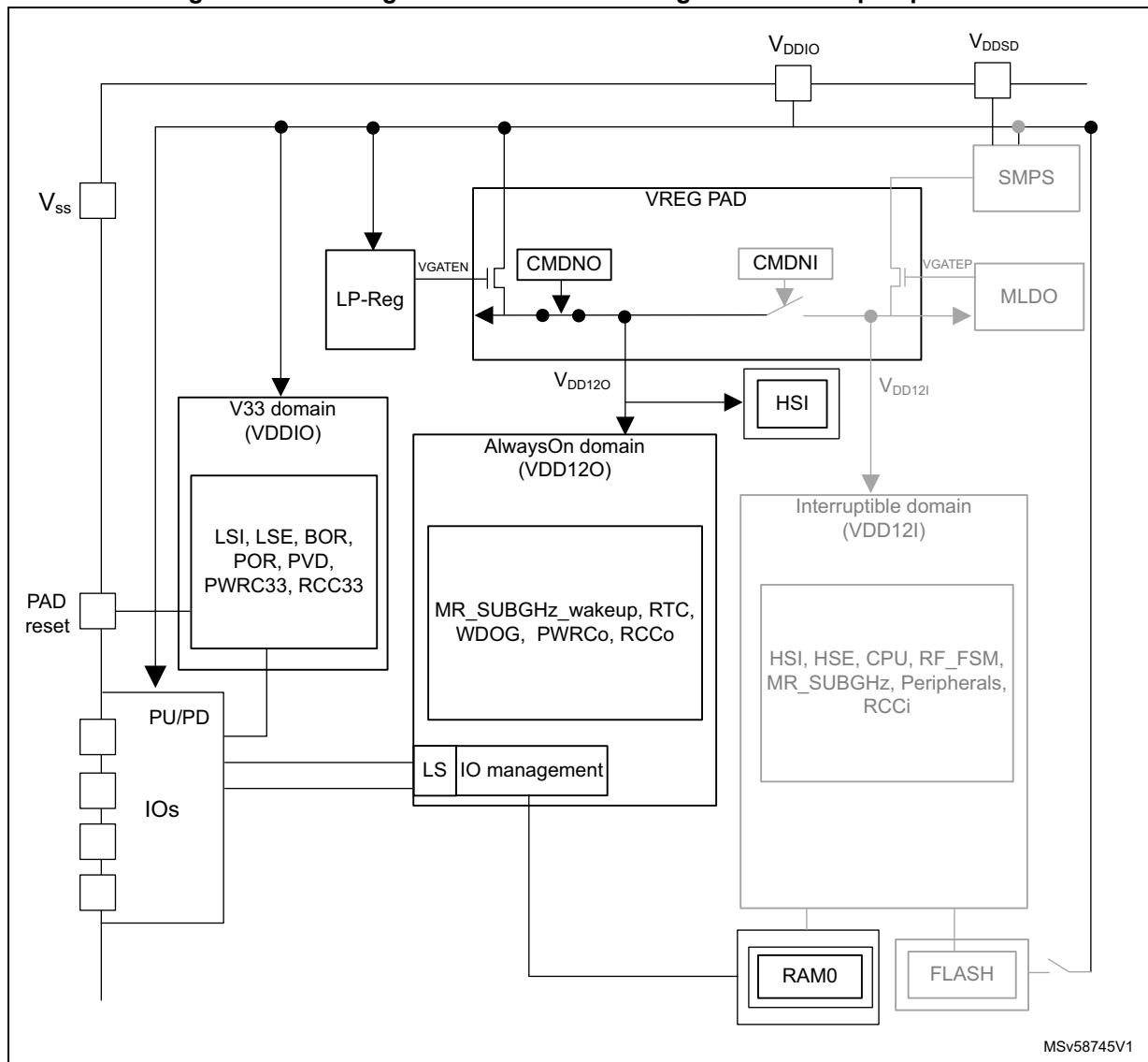
Figure 7. Power regulators and SMPS configuration in Deepstop mode
