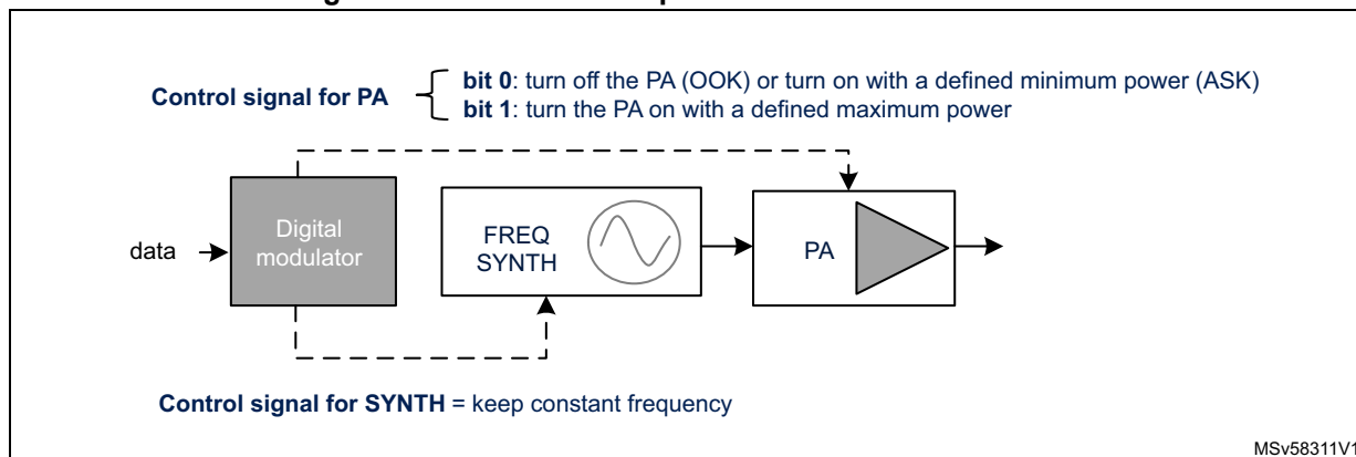
Figure 252. Transmission path for ASK/OOK modulation
