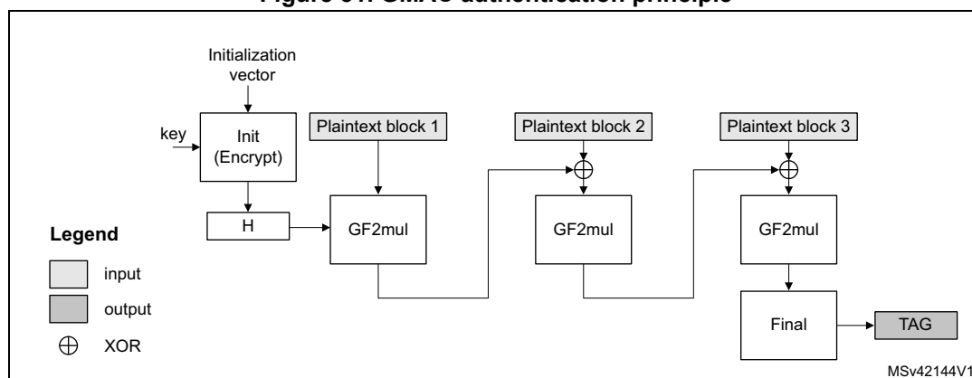
Figure 31. GMAC authentication principle
