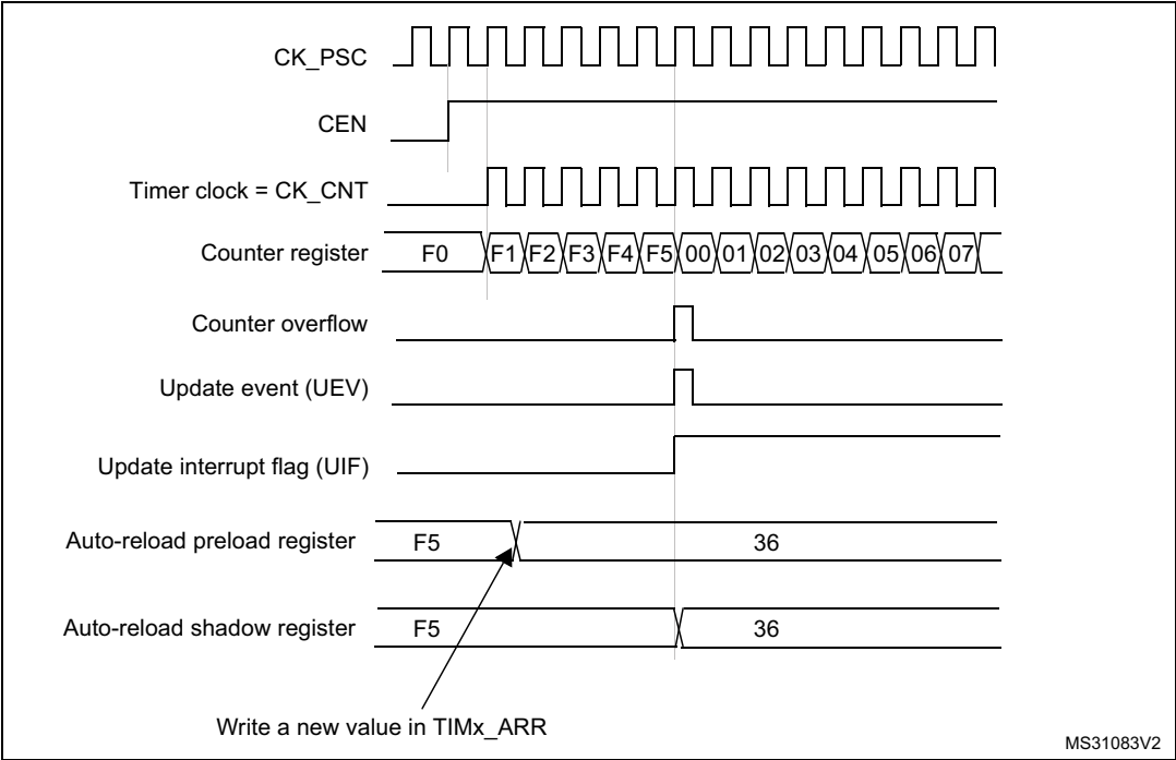
Figure 114. Counter timing diagram, update event when ARPE=1 (TIMx_ARR preloaded)
