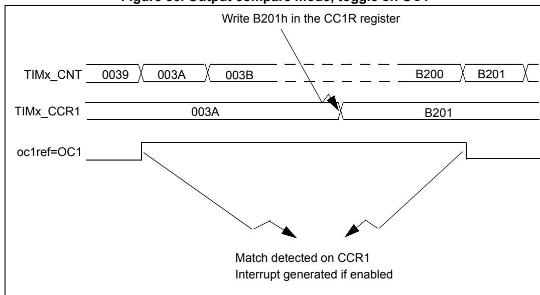
Figure 86. Output compare mode, toggle on OC1
