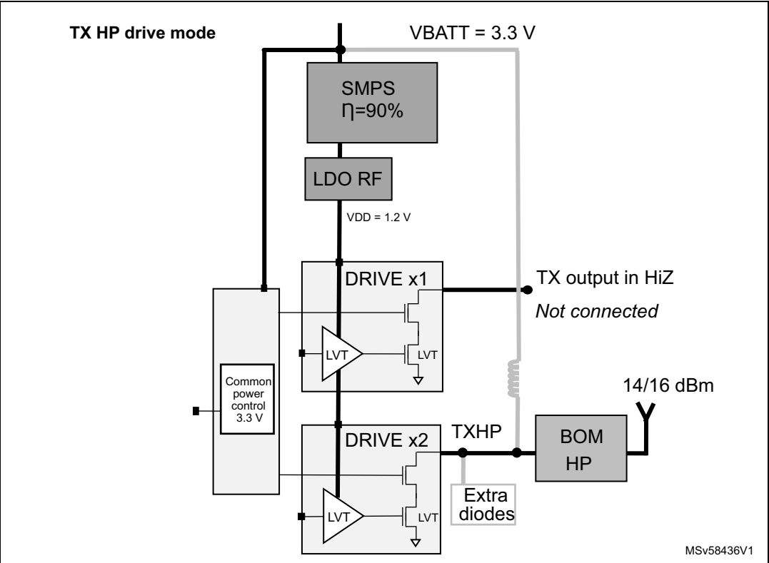
Figure 258. TX and TX HP pin connections, TX HP PA drive mode, VBATT = 3.3 V
