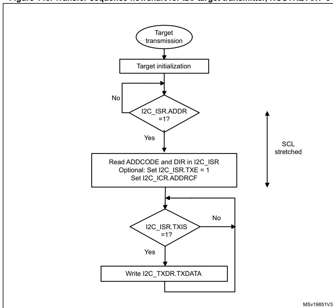
Figure 148. Transfer sequence flowchart for I2C target transmitter, NOSTRETCH=0
