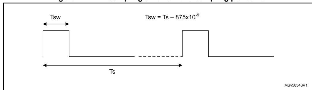
Figure 24. ADC sampling time T_{sw} and sampling period T_s
