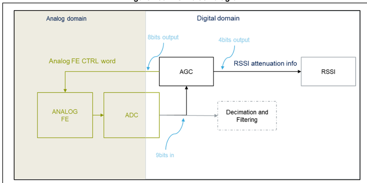
Figure 260. AGC block diagram
