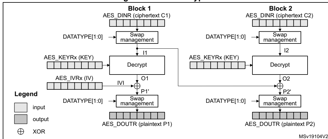
Figure 38. CBC decryption
