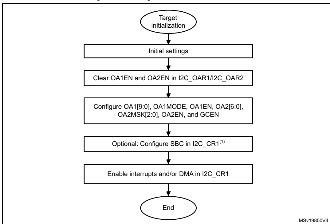
Figure 147. Target initialization flowchart
