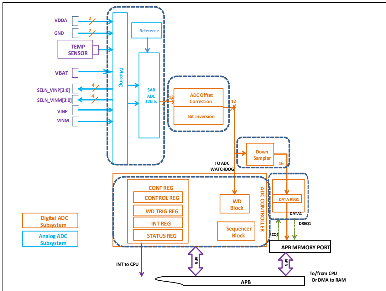
Figure 23. ADC top level diagram
