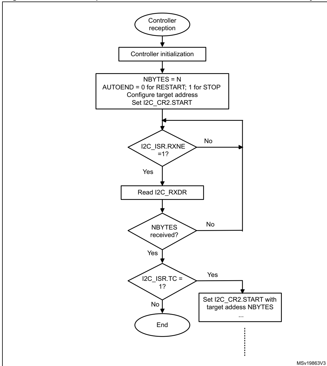
Figure 160. Transfer sequence flowchart for I2C controller receiver for N \leq 255 bytes
