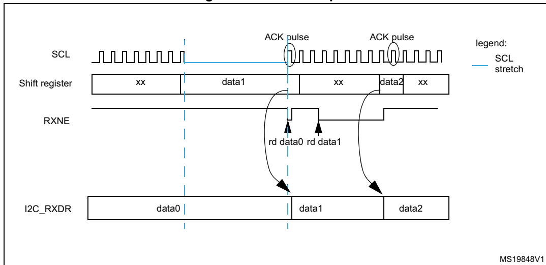
Figure 145. Data reception
