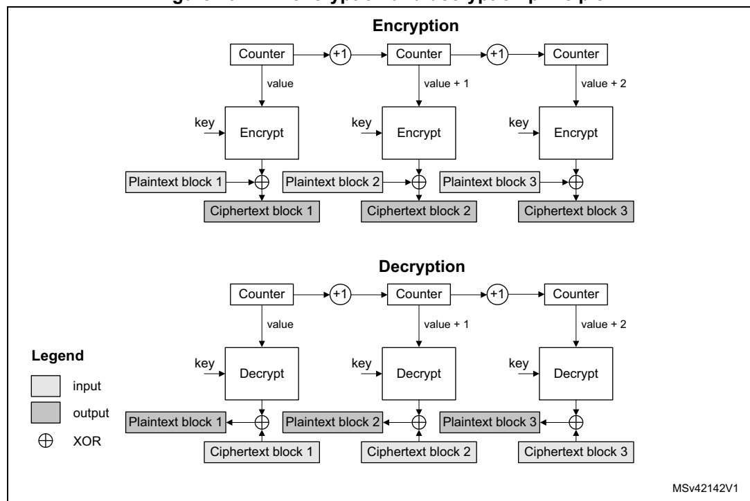
Figure 29. CTR encryption and decryption principle
