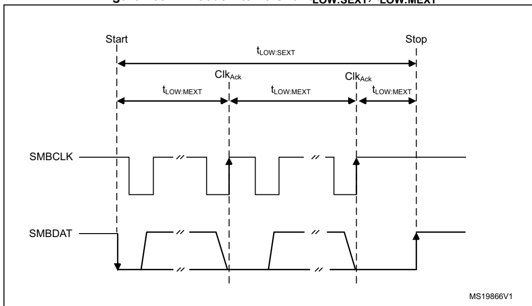
Figure 163. Timeout intervals for t_{\text{LOW:SEXT}} , t_{\text{LOW:MEXT}}
