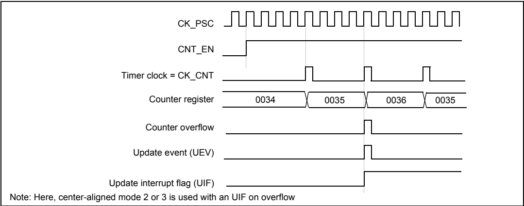
Figure 70. Counter timing diagram, internal clock divided by 4, TIMx_ARR=0x36
