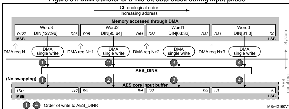
Figure 51. DMA transfer of a 128-bit data block during input phase
