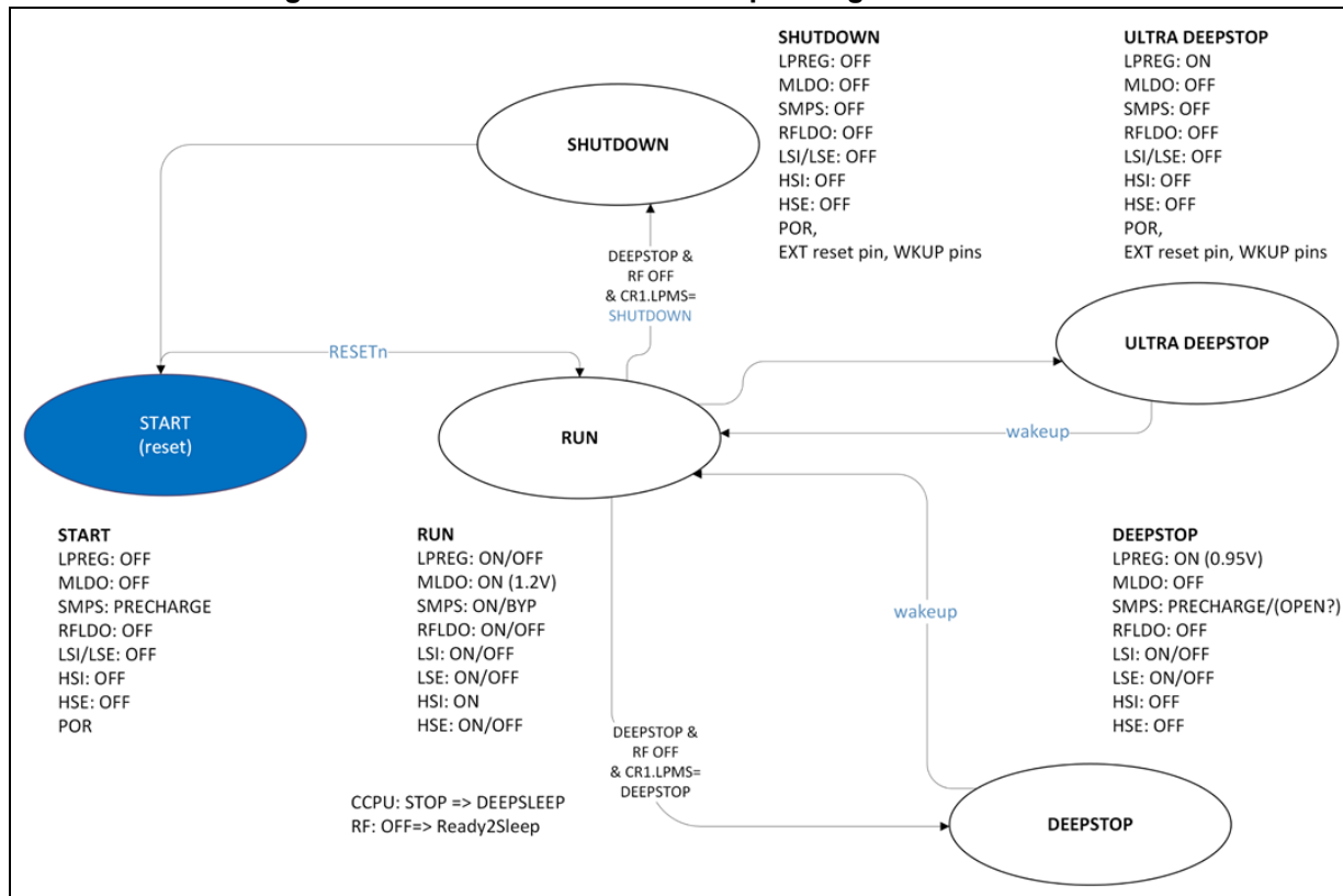
Figure 10. PWR state machine for operating mode transitions
