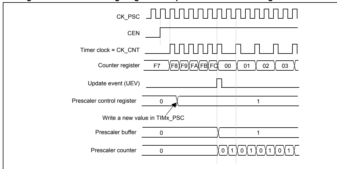
Figure 55. Counter timing diagram with prescaler division change from 1 to 2
