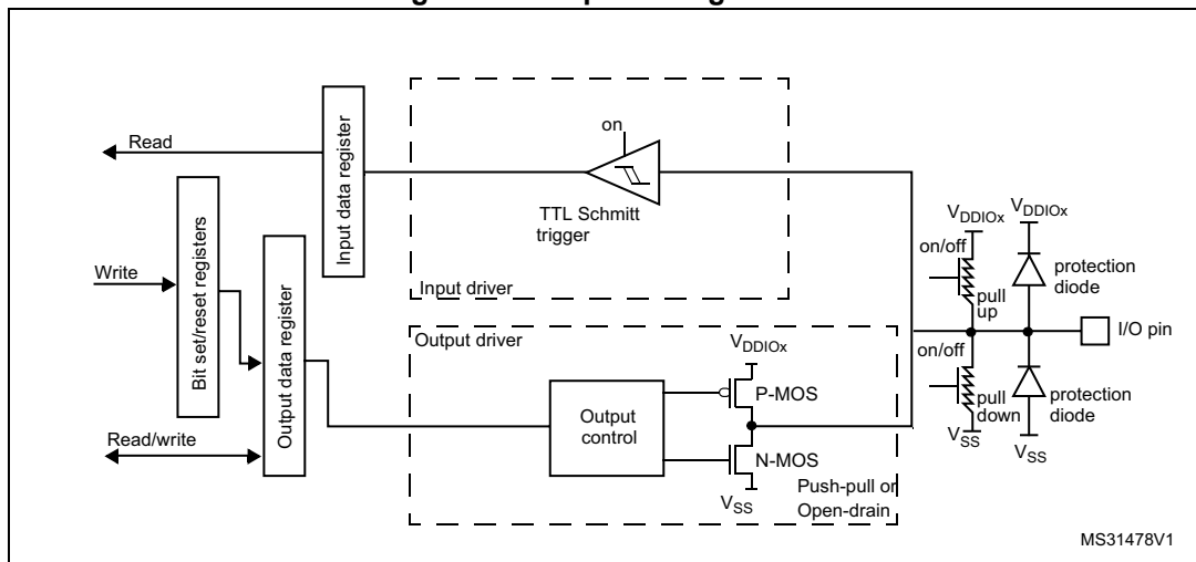
Figure 19. Output configuration
