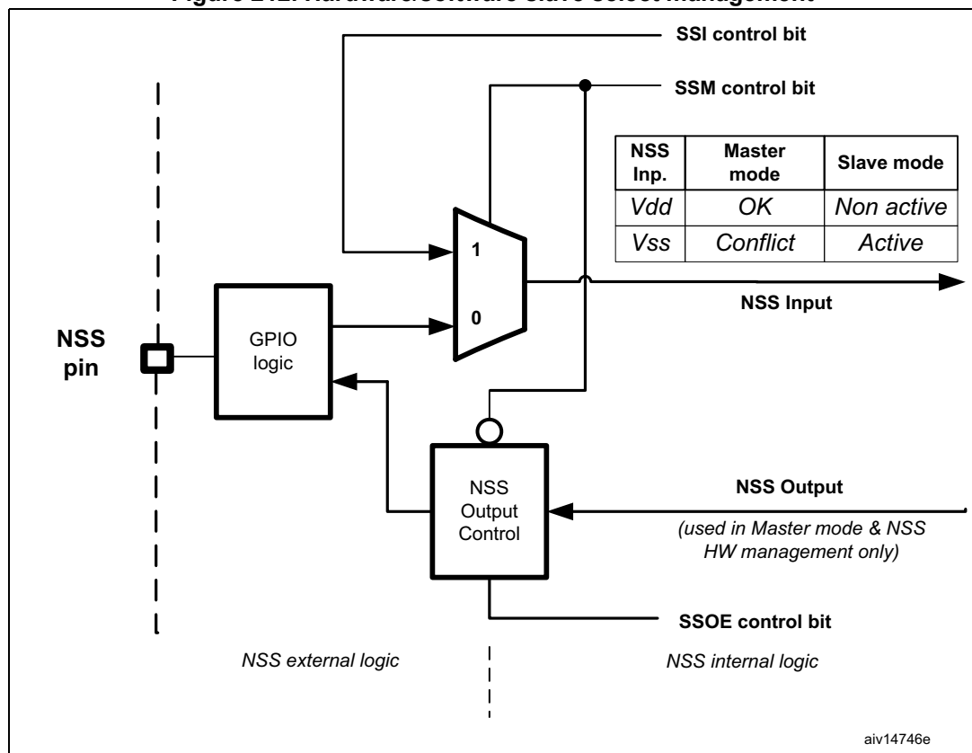
Figure 212. Hardware/software slave select management
