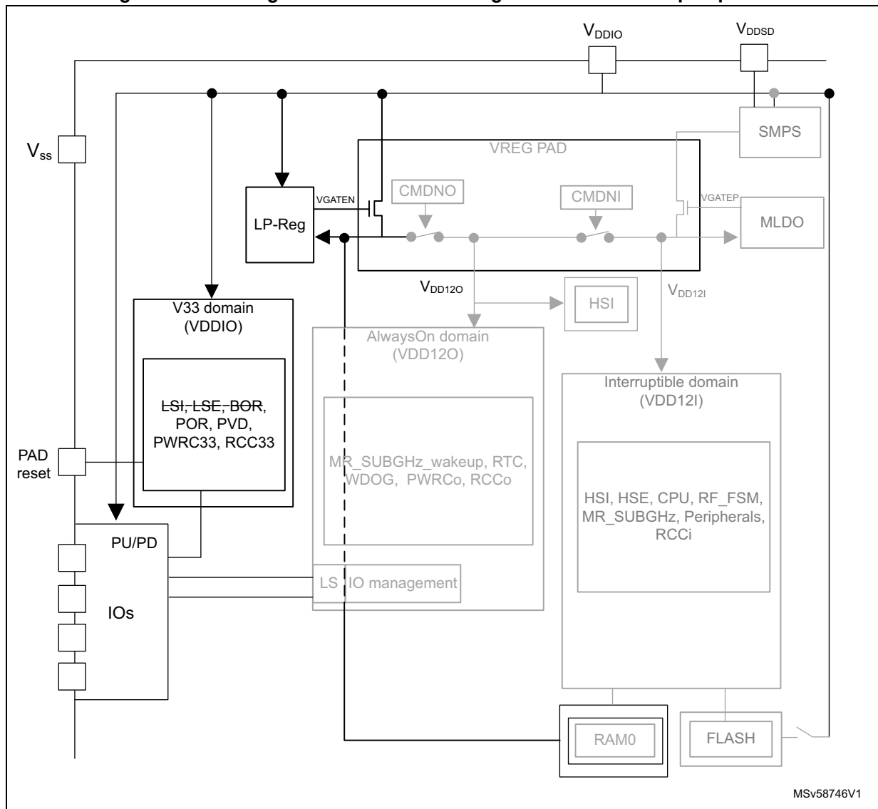
Figure 8. Power regulators and SMPS configuration in Ultra Deepstop mode
