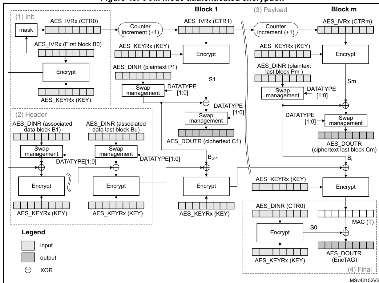
Figure 49. CCM mode authenticated encryption
