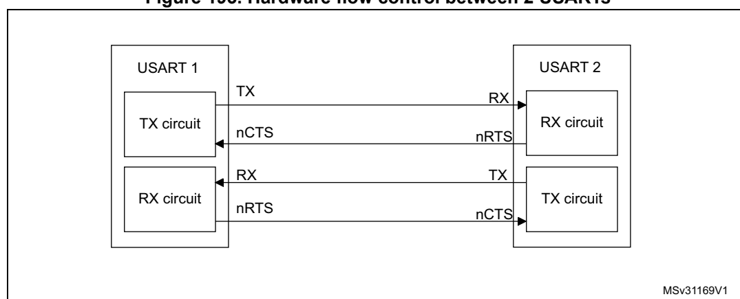
Figure 193. Hardware flow control between 2 USARTs
