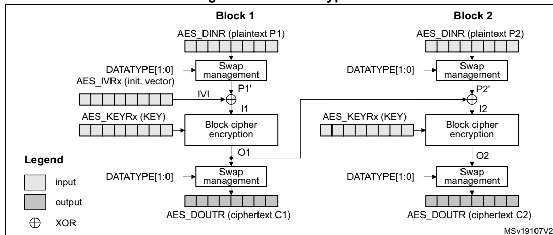
Figure 37. CBC encryption
