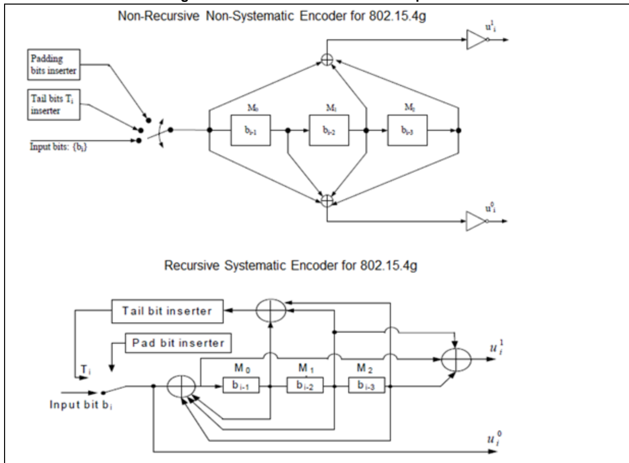
Figure 248. FEC schemes for 802.15.4 packets
