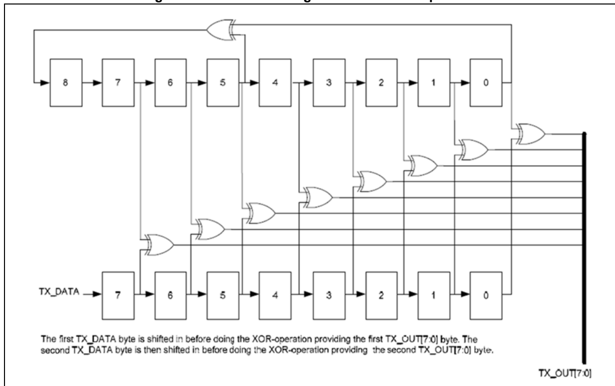
Figure 245. Data whitening scheme for Basic packets
