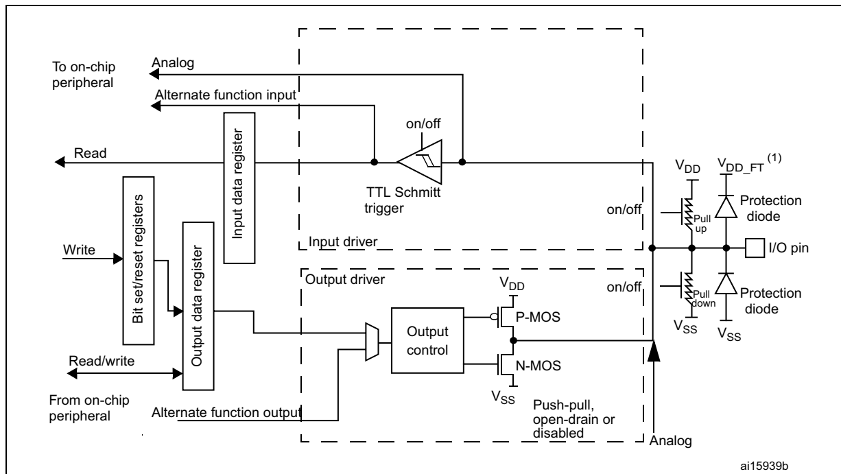
Figure 16. Basic structure of a mixed analog/digital five-volt tolerant I/O port bit
