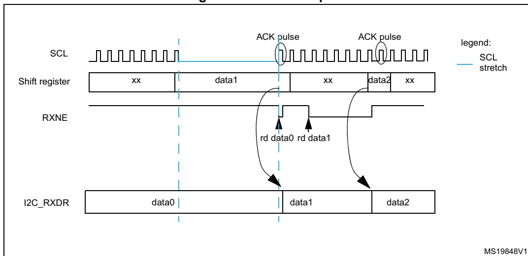
Figure 145. Data reception
