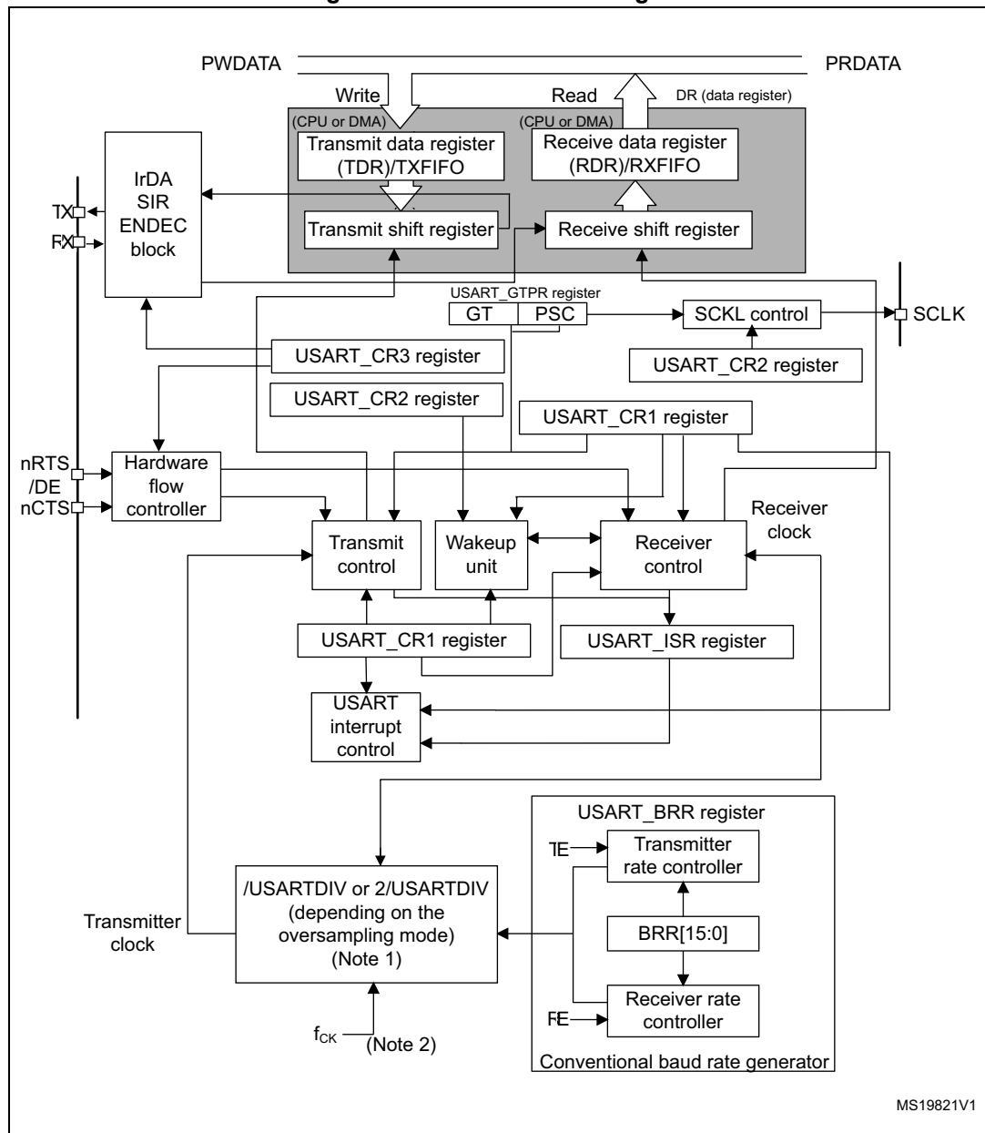
Figure 171. USART block diagram
