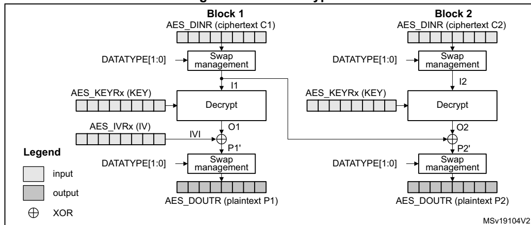
Figure 38. CBC decryption
