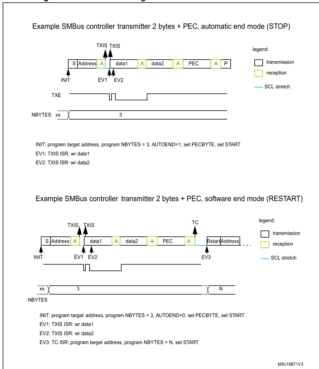
Figure 168. Bus transfer diagrams for SMBus controller transmitter
