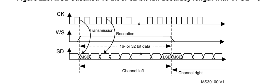
Figure 229. MSB Justified 16-bit or 32-bit full-accuracy length with CPOL = 0
