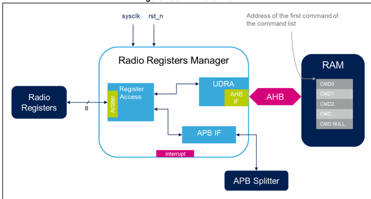
Figure 263. RRM overview
