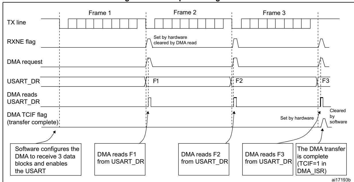
Figure 203. Reception using DMA
