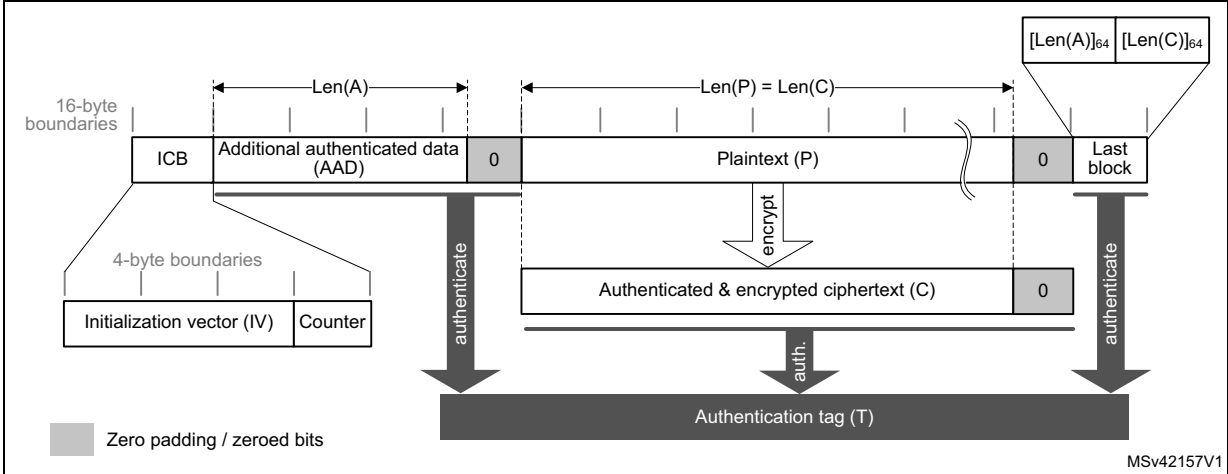
Figure 44. Message construction in GCM
