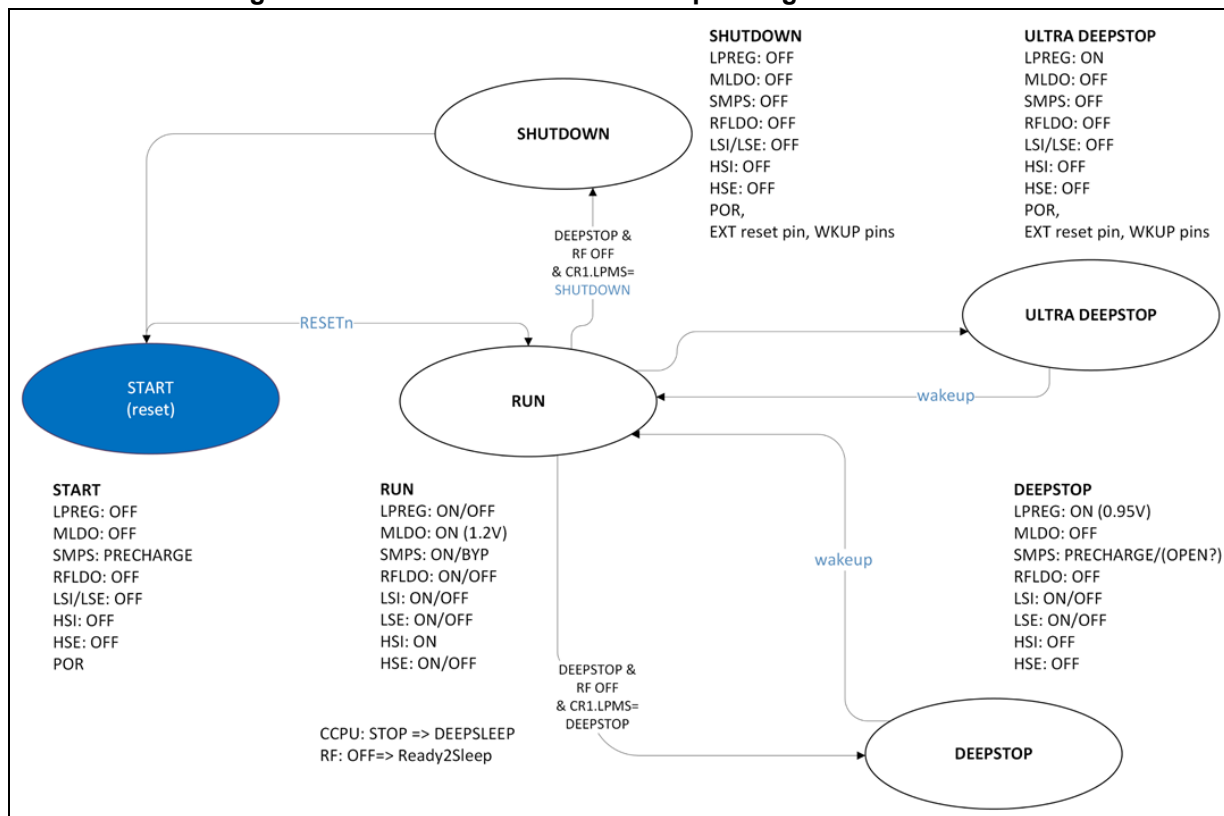
Figure 10. PWRC state machine for operating mode transitions
