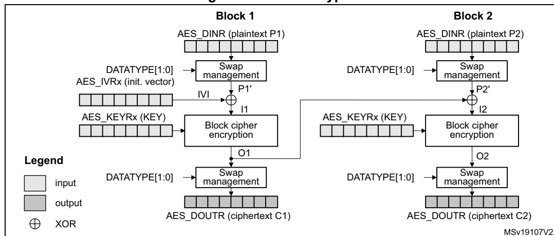
Figure 37. CBC encryption
