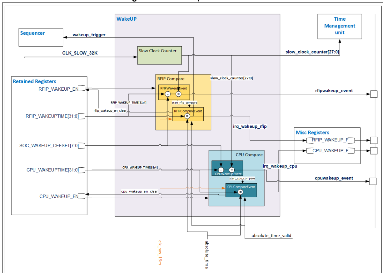
Figure 271. Wakeup block overview
