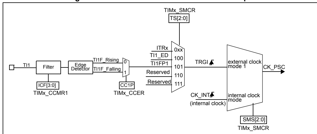
Figure 117. TI1 external clock connection example
