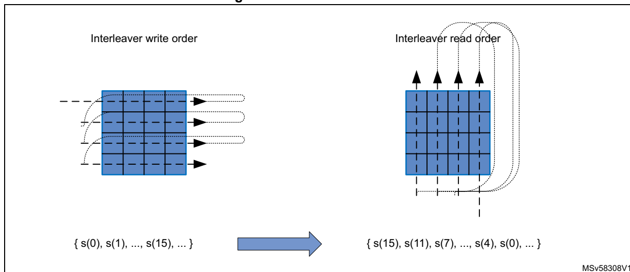
Figure 249. Interleave scheme
