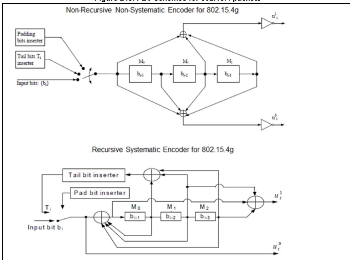
Figure 248. FEC schemes for 802.15.4 packets
