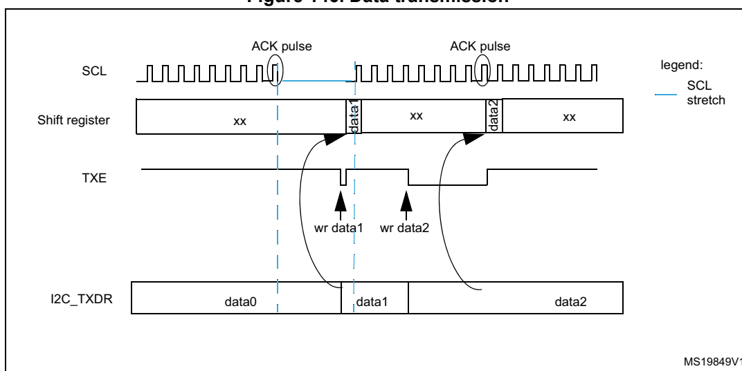
Figure 146. Data transmission
