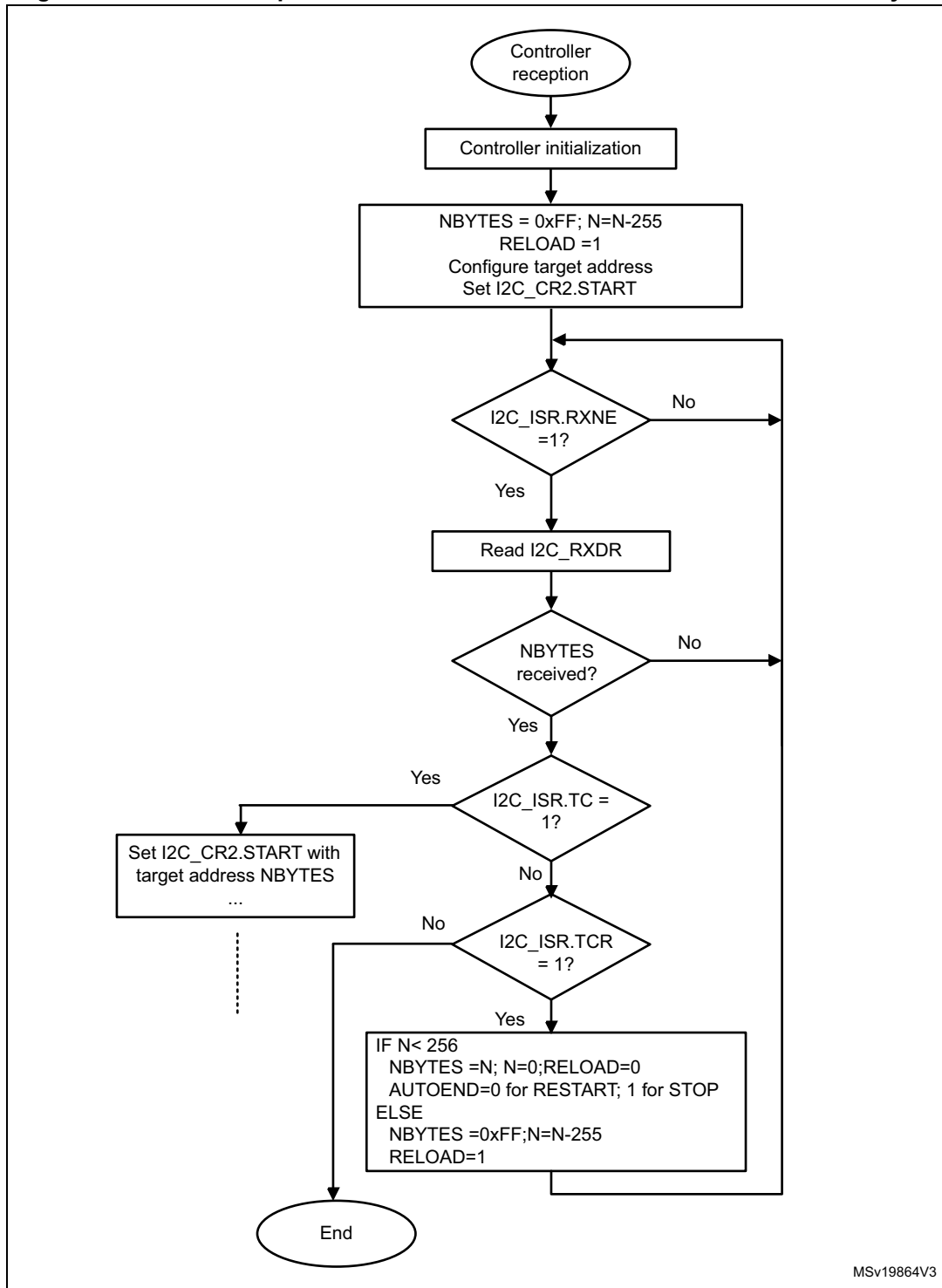
Figure 161. Transfer sequence flowchart for I2C controller receiver for N &gt; 255 bytes
